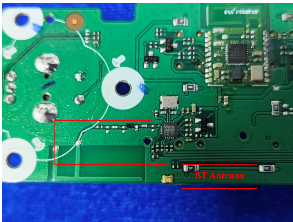
Photo 16: Internal View for BT Antenna
