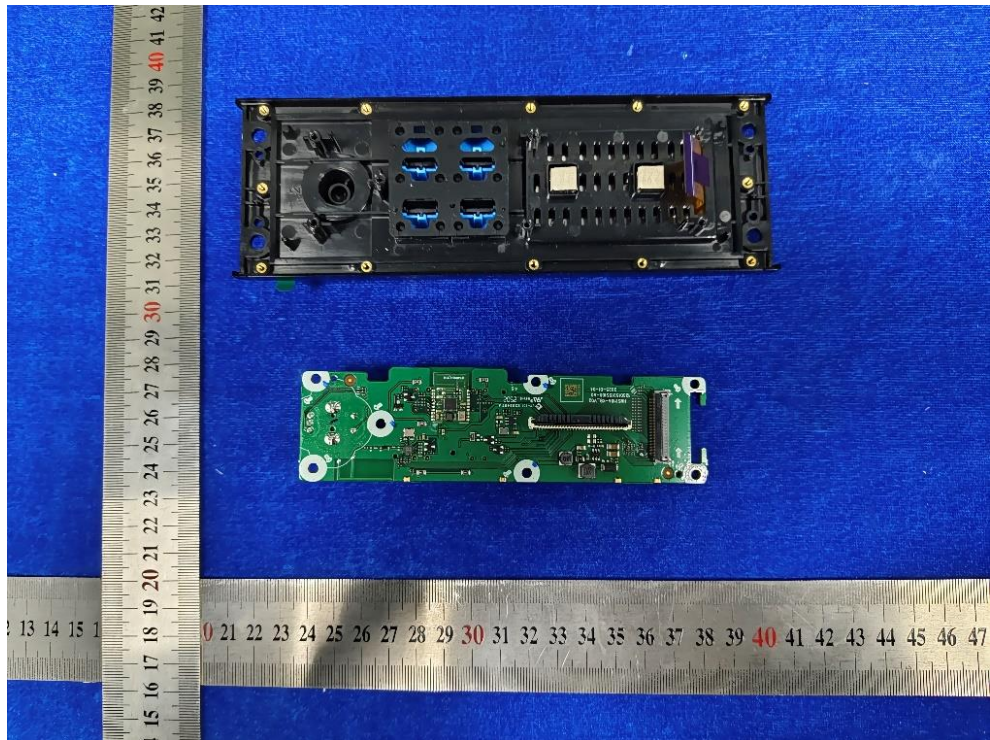
Photo 12: Internal View for PCB C
