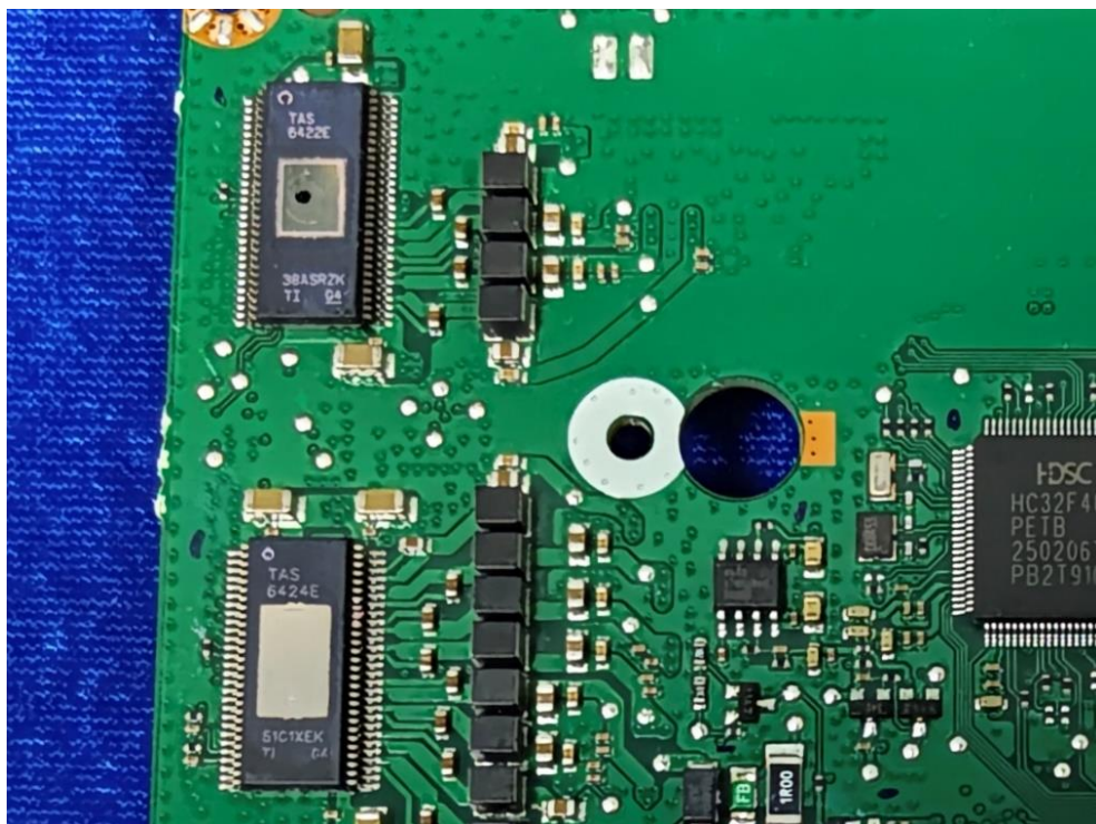
Photo 6: Internal View for PCB A
