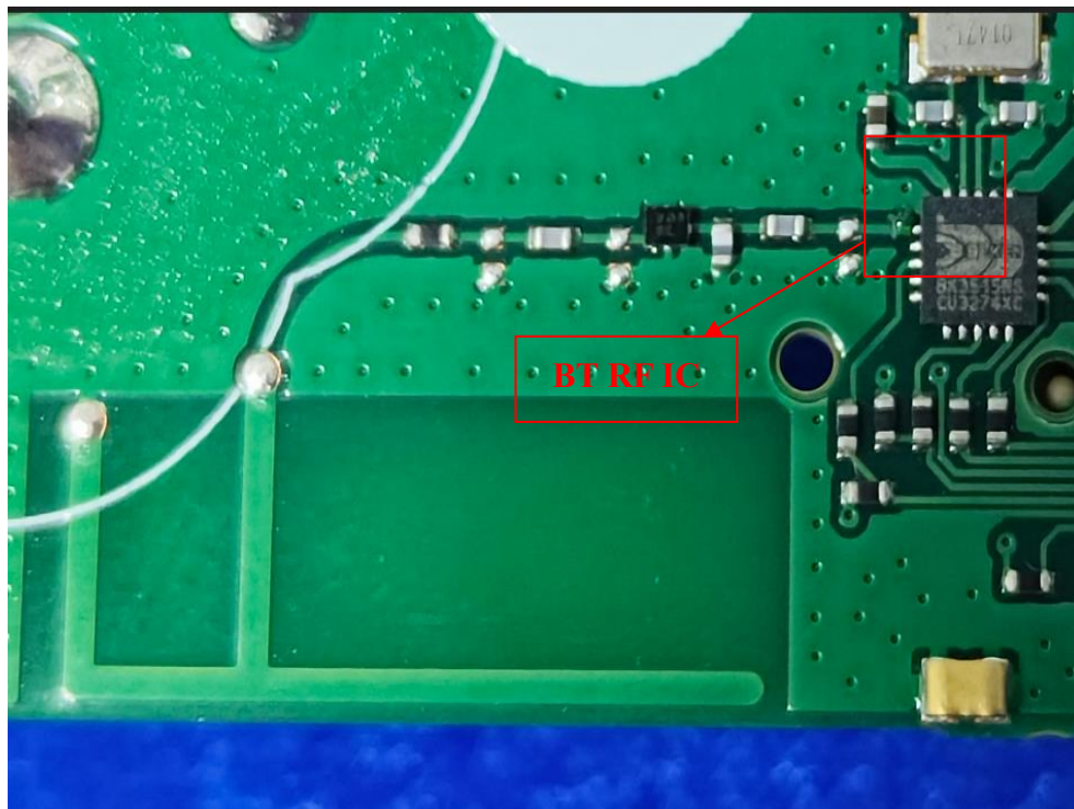
Photo 17: Internal View for BT RF IC
