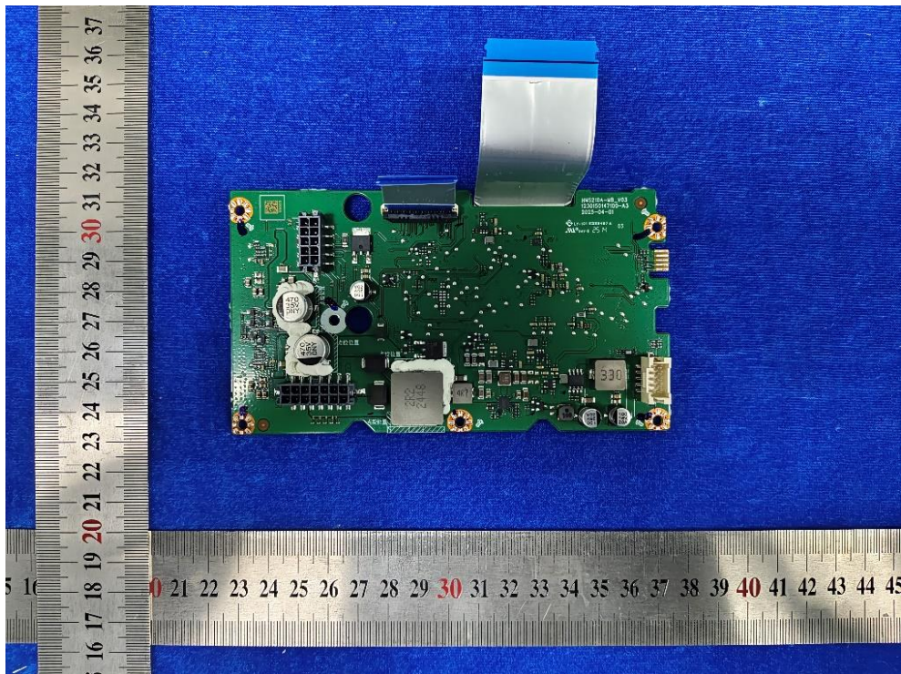
Photo 2: Internal View for PCB A
