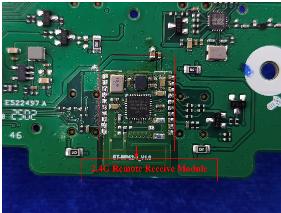
Photo 15: Internal View for PCB C
