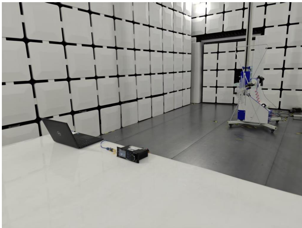
Description: RF Radiated Emission Test Setup for 30MHz ~ 1GHz
