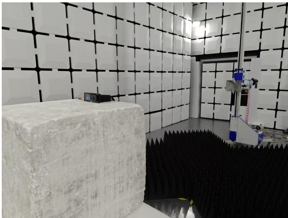
Description: RF Radiated Emission Test Setup for 1GHz ~ 18GHz
