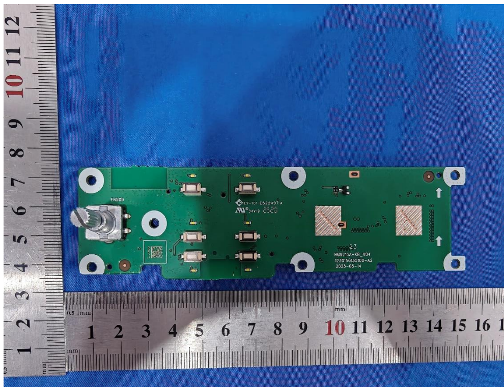
Photo 10: Internal View for PCB C
