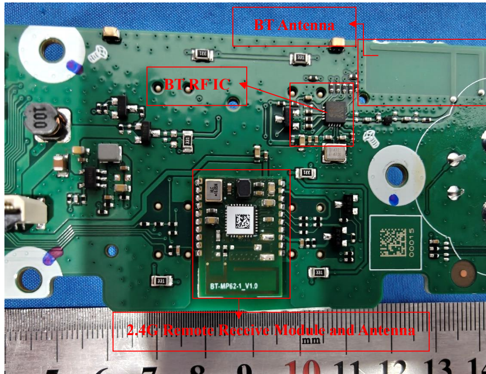
Photo 13: Internal View for Antenna
