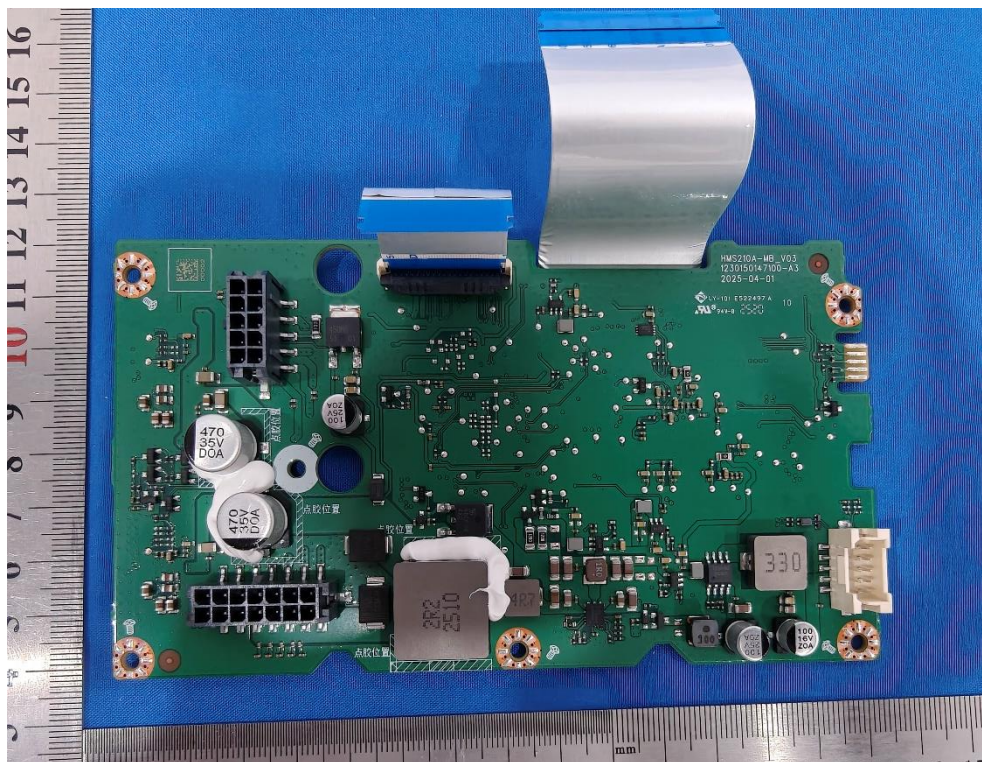
Photo 2: Internal View for PCB A
