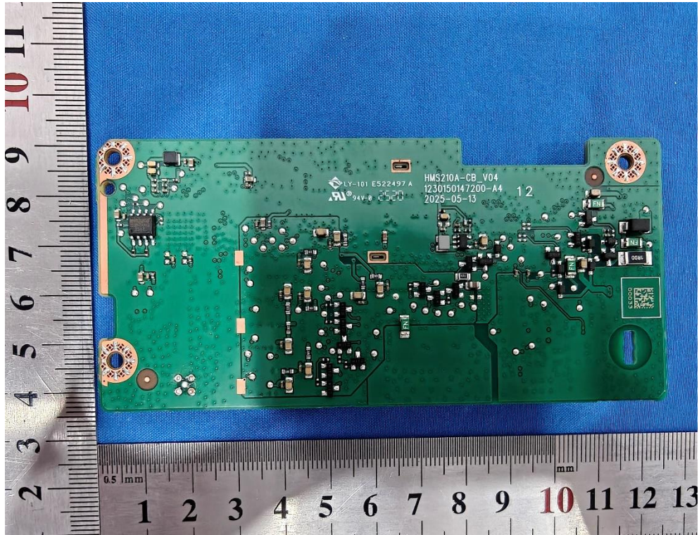
Photo 7: Internal View for PCB B
