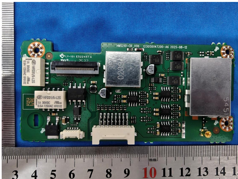
Photo 6: Internal View for PCB B
