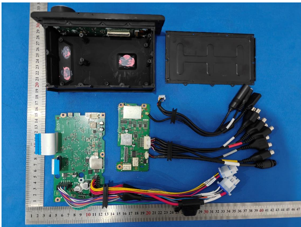
Photo 1: Internal View
