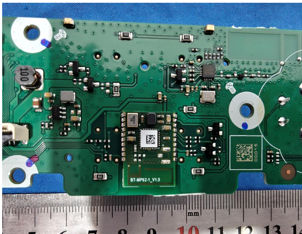
Photo 12: Internal View for PCB C
