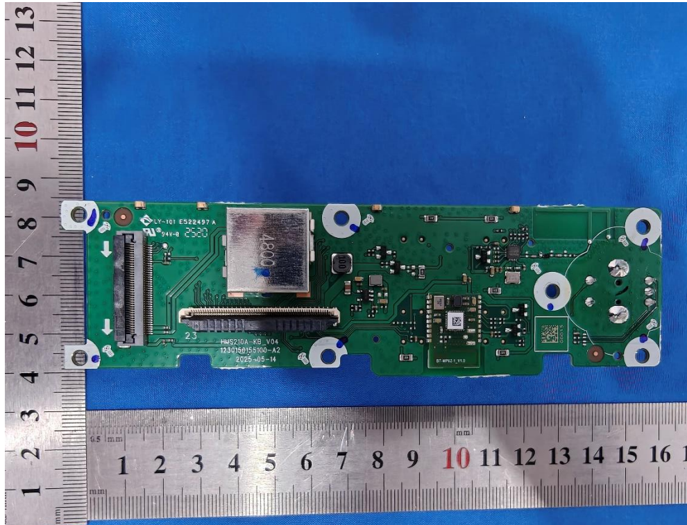
Photo 9: Internal View for PCB C
