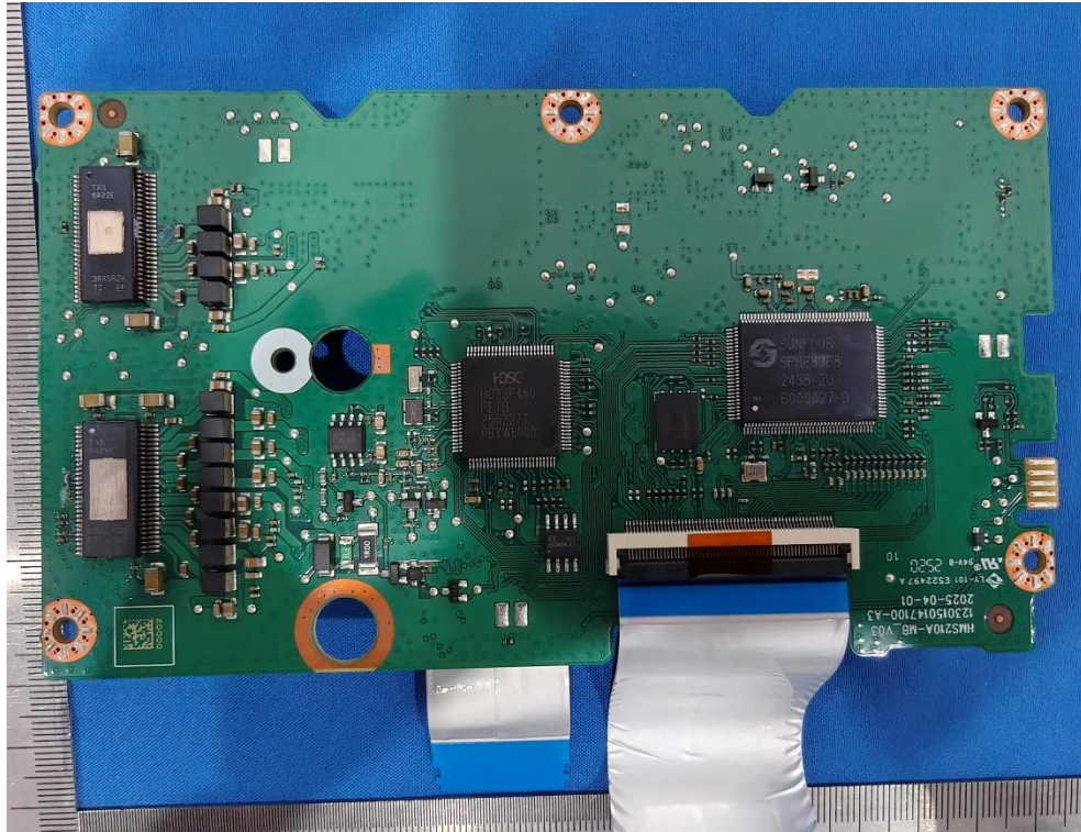
Photo 3: Internal View for PCB A
