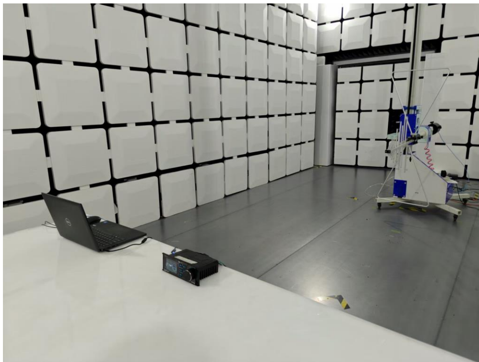
Description: RF Radiated Emission Test Setup for 30MHz ~ 1GHz (Mode1)
