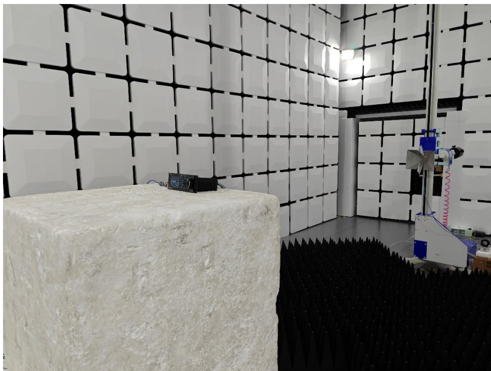
Description: RF Radiated Emission Test Setup for 1GHz ~ 18GHz (Mode1)
