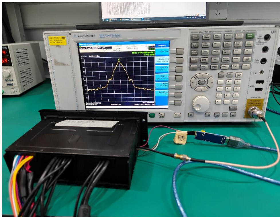
Description: RF Conducted Test Setup Photo
