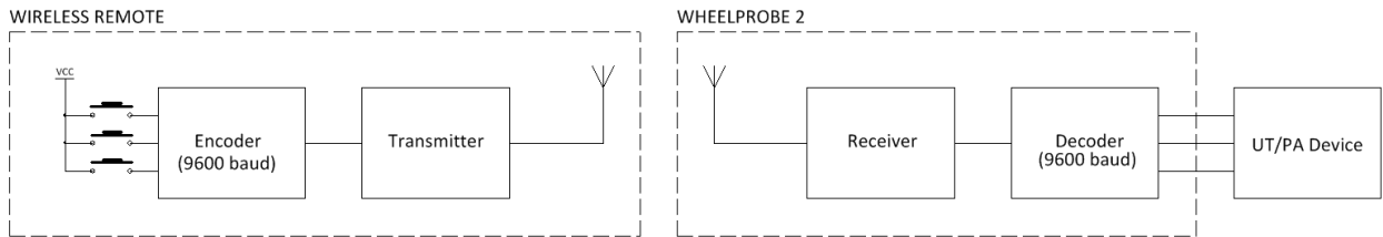
Figure 3.5-1: Setup diagram
