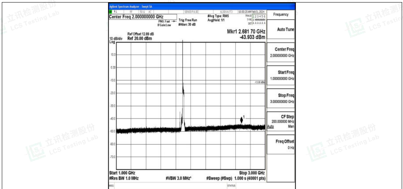
Band2_20MHz_16QAM_19100_1RB#0_1000~3000_1000~3000
