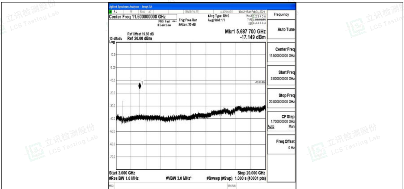
Band2_15MHz_QPSK_19125_1RB#0_3000~20000_3000~20000
