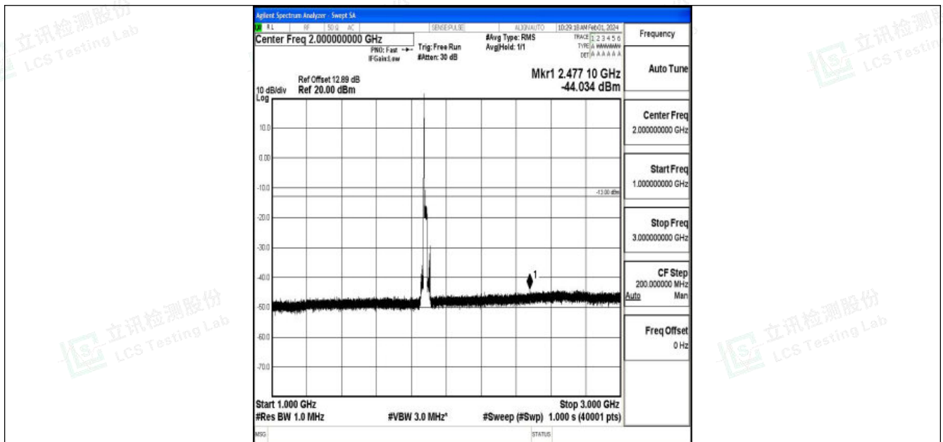
Band2_20MHz_16QAM_18900_1RB#0_1000~3000_1000~3000
