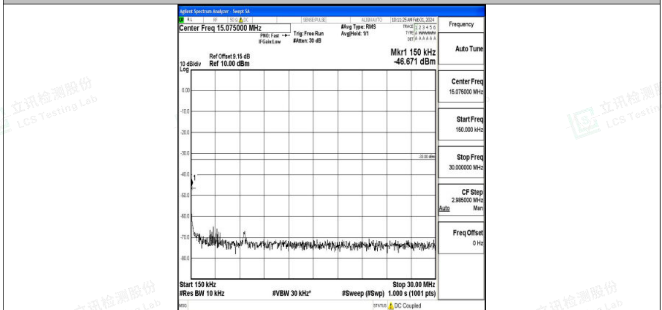
Band2_15MHz_QPSK_18900_1RB#0_0.15~30_0.15~30
