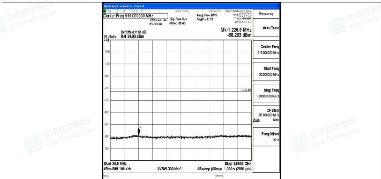
Band2_20MHz_QPSK_18700_1RB#0_30~1000_30~1000
