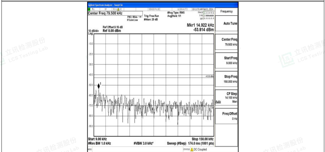
Band2_15MHz_16QAM_18900_1RB#0_0.009~0.15_0.009~0.15
