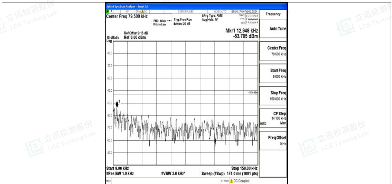
Band2_15MHz_QPSK_18675_1RB#0_0.009~0.15_0.009~0.15
