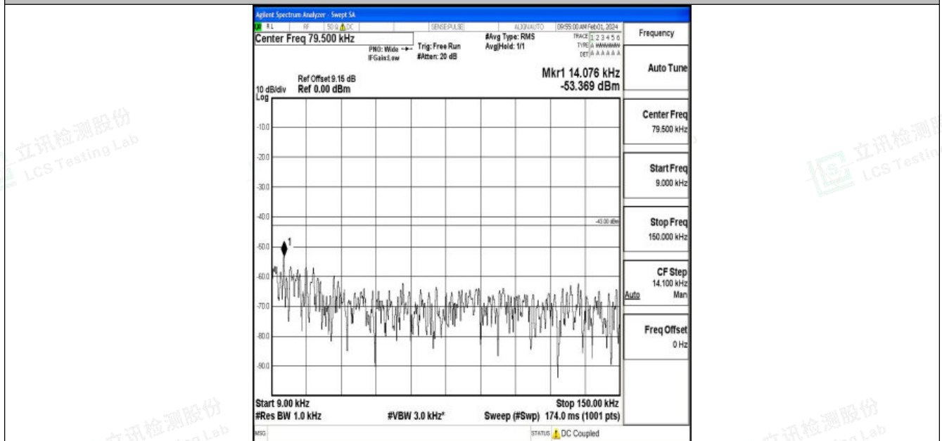
Band2_10MHz_16QAM_19150_1RB#0_0.009~0.15_0.009~0.15
