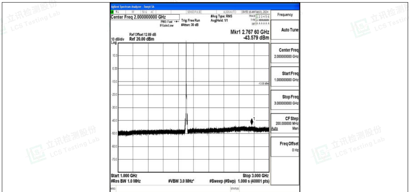
Band2_10MHz_16QAM_19150_1RB#0_1000~3000_1000~3000
