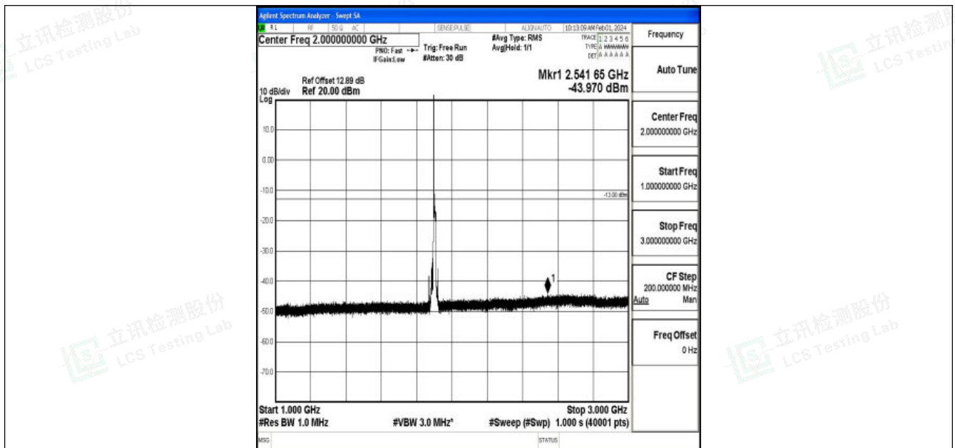
Band2_15MHz_16QAM_19125_1RB#0_1000~3000_1000~3000
