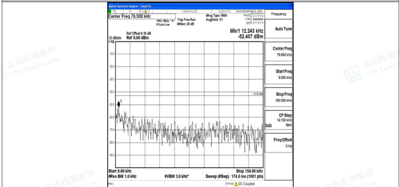
Band2_5MHz_16QAM_18900_1RB#0_0.009~0.15_0.009~0.15
