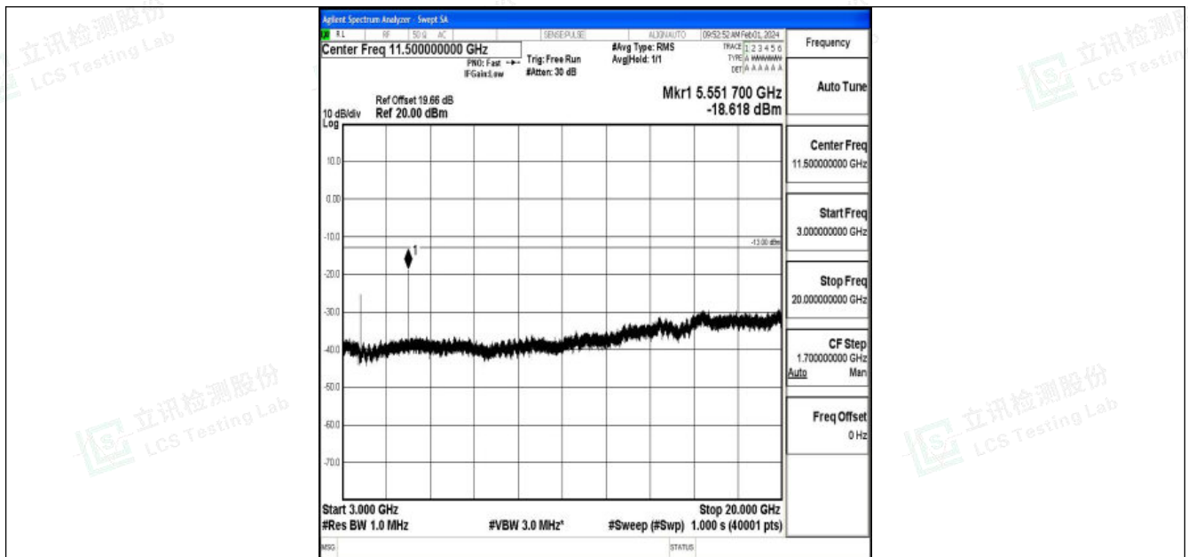
Band2_10MHz_QPSK_18650_1RB#0_3000~20000_3000~20000
