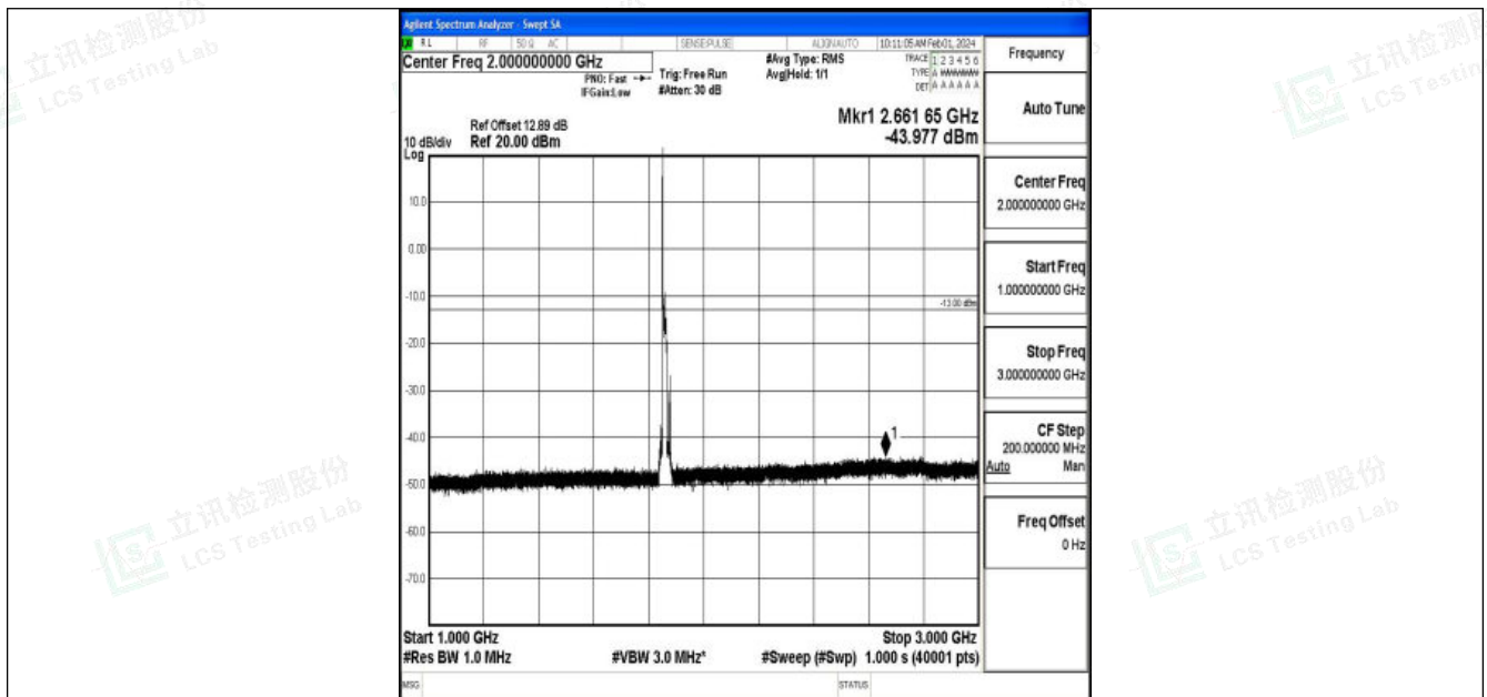
Band2_15MHz_16QAM_18675_1RB#0_1000~3000_1000~3000
