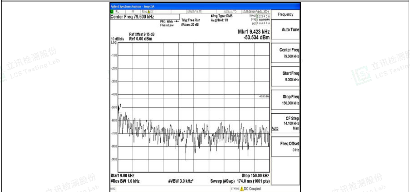
Band2_20MHz_16QAM_18700_1RB#0_0.009~0.15_0.009~0.15
