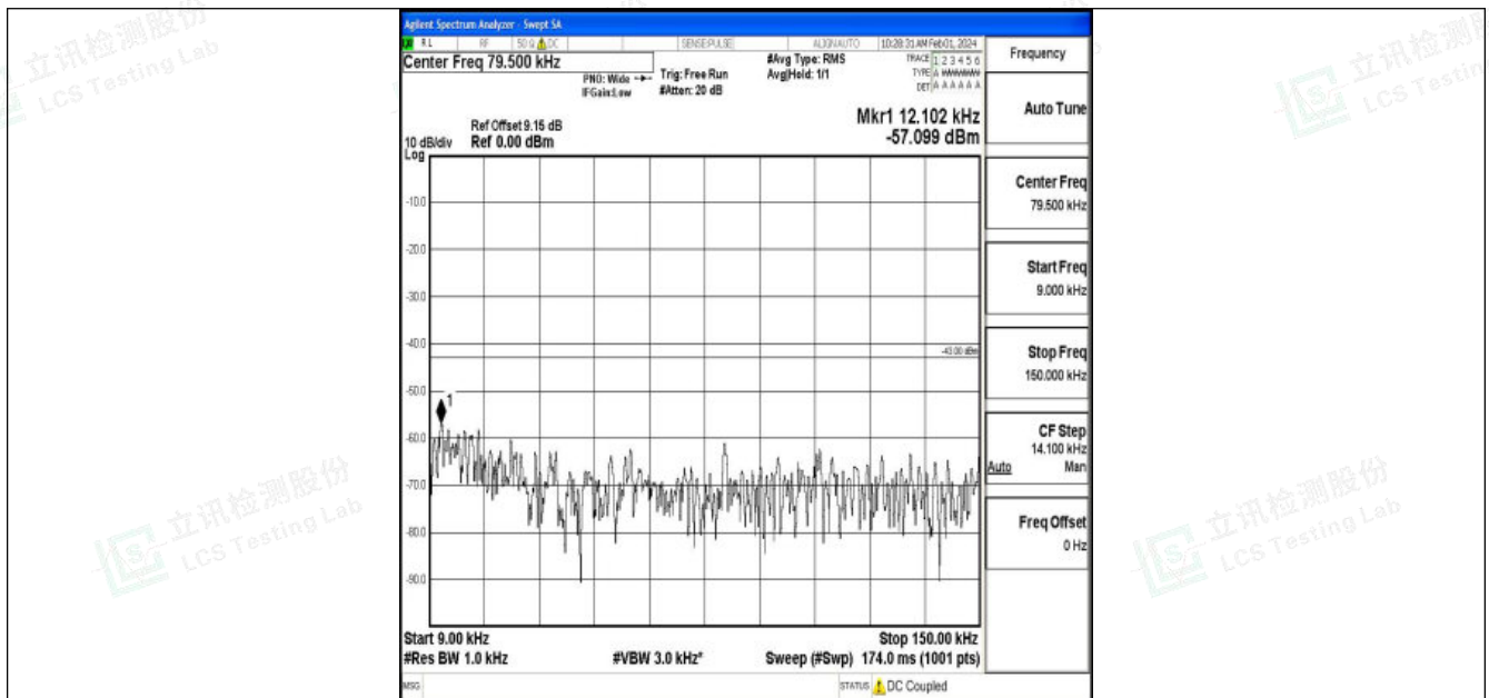
Band2_20MHz_QPSK_18900_1RB#0_0.009~0.15_0.009~0.15
