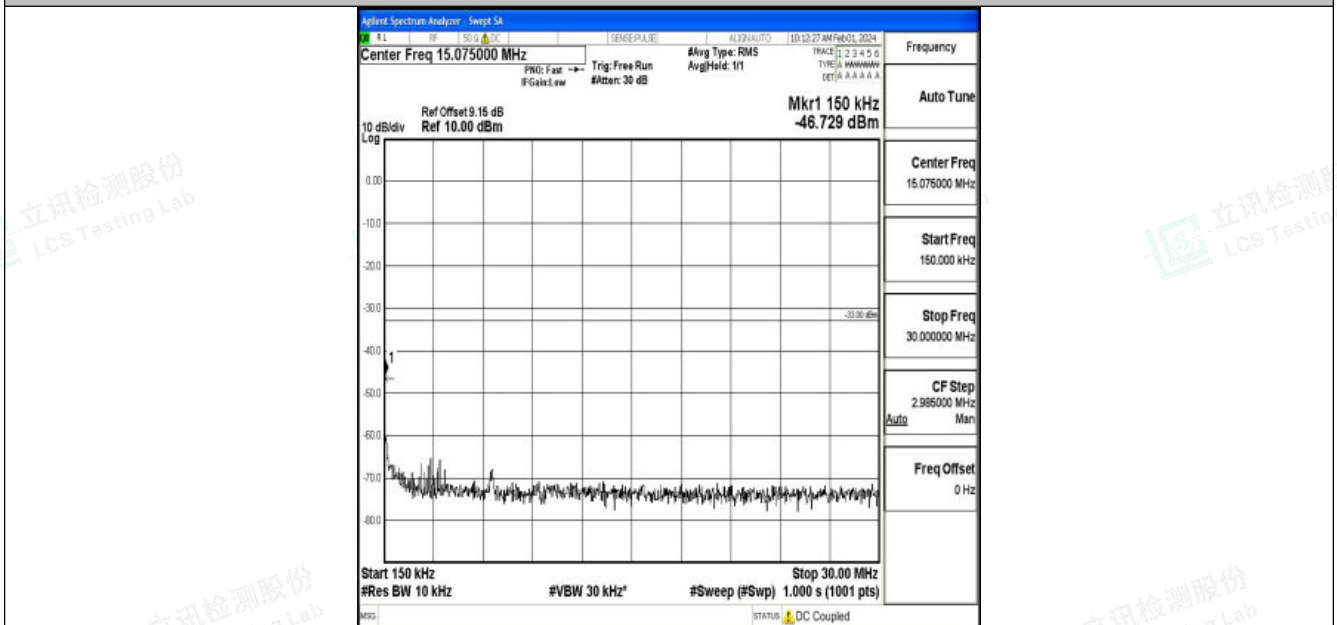
Band2_15MHz_QPSK_19125_1RB#0_0.15~30_0.15~30
