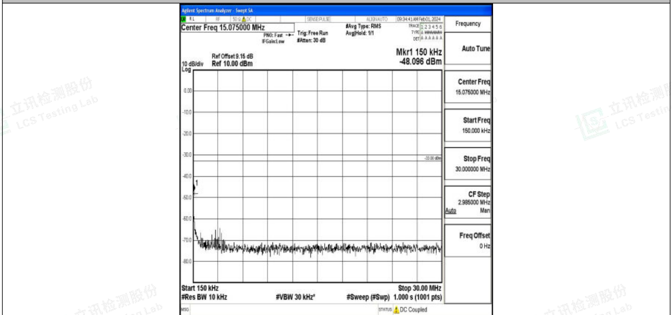
Band2_5MHz_QPSK_19175_1RB#0_0.15~30_0.15~30
