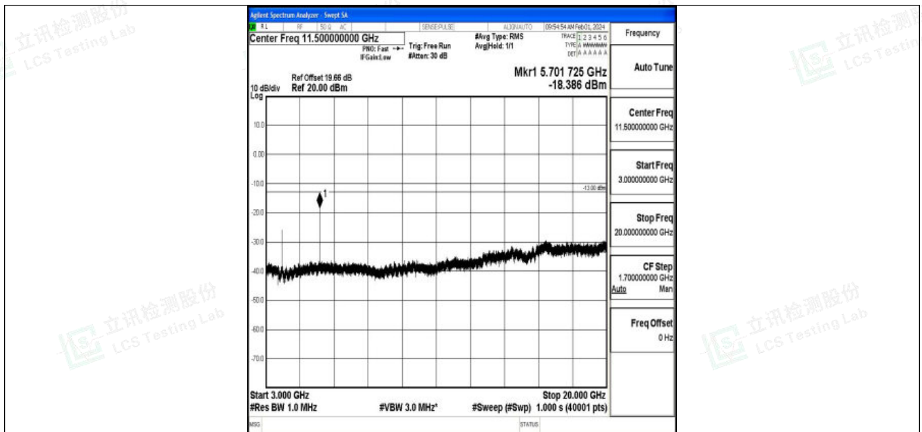
Band2_10MHz_QPSK_19150_1RB#0_3000~20000_3000~20000
