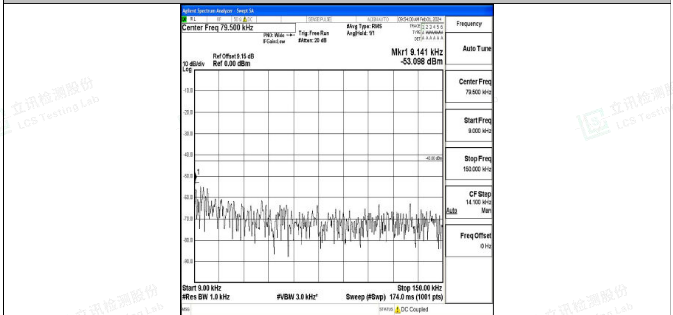
Band2_10MHz_16QAM_18900_1RB#0_0.009~0.15_0.009~0.15
