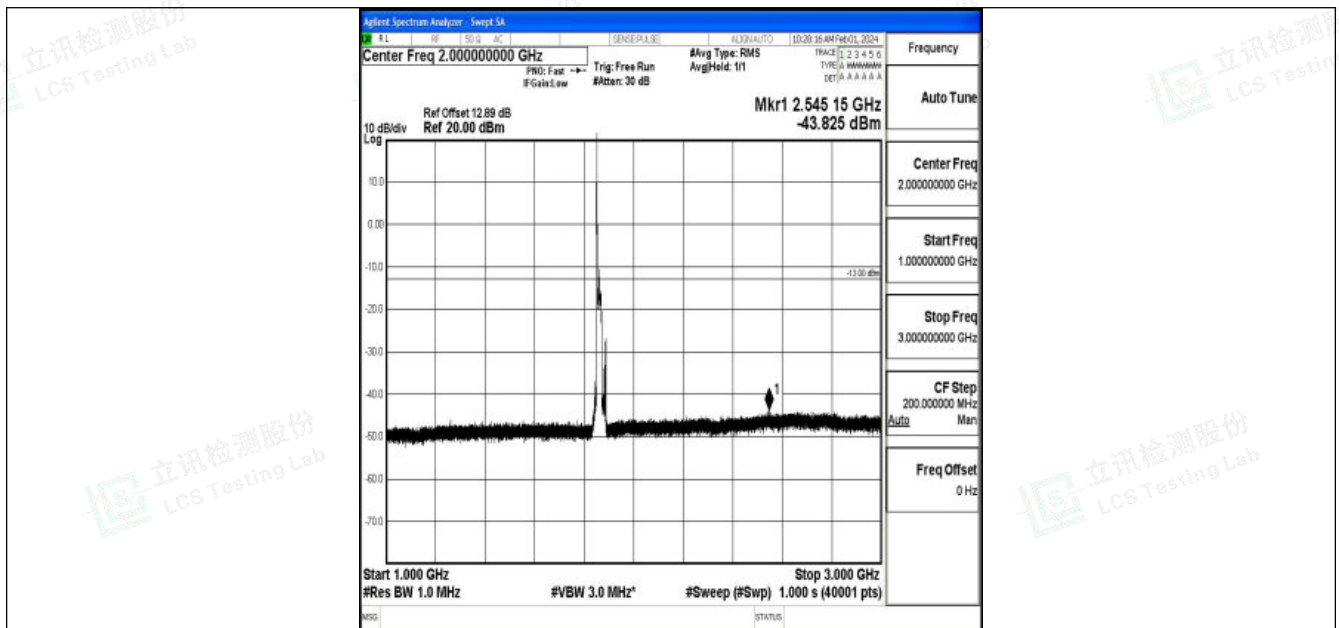
Band2_20MHz_16QAM_18700_1RB#0_1000~3000_1000~3000
