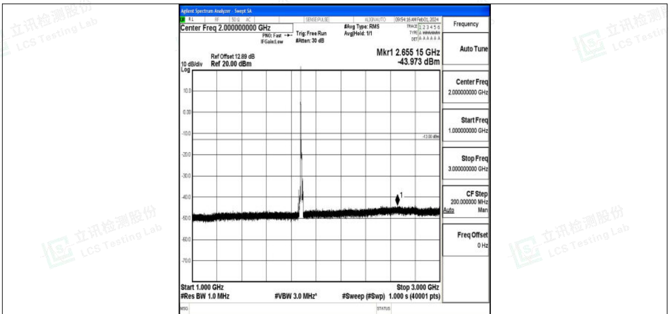
Band2_10MHz_16QAM_18900_1RB#0_1000~3000_1000~3000
