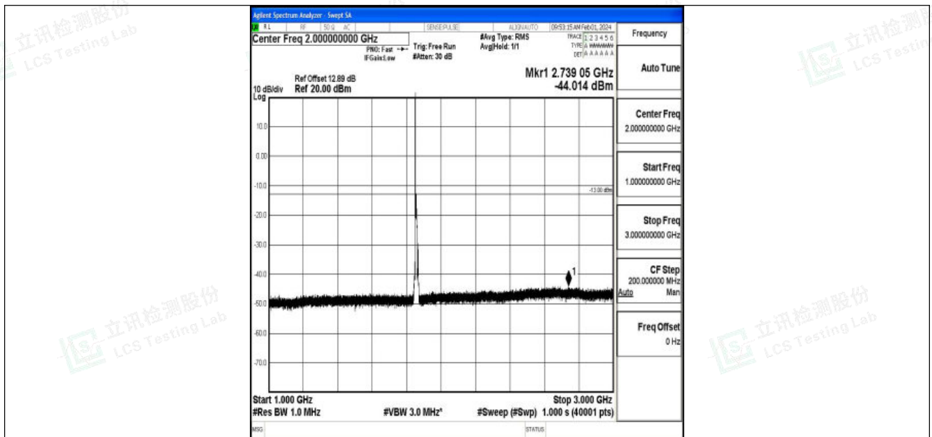
Band2_10MHz_16QAM_18650_1RB#0_1000~3000_1000~3000
