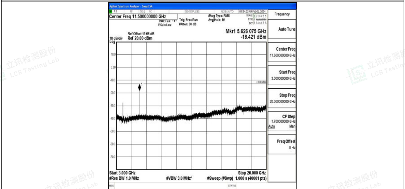
Band2_10MHz_16QAM_18900_1RB#0_3000~20000_3000~20000
