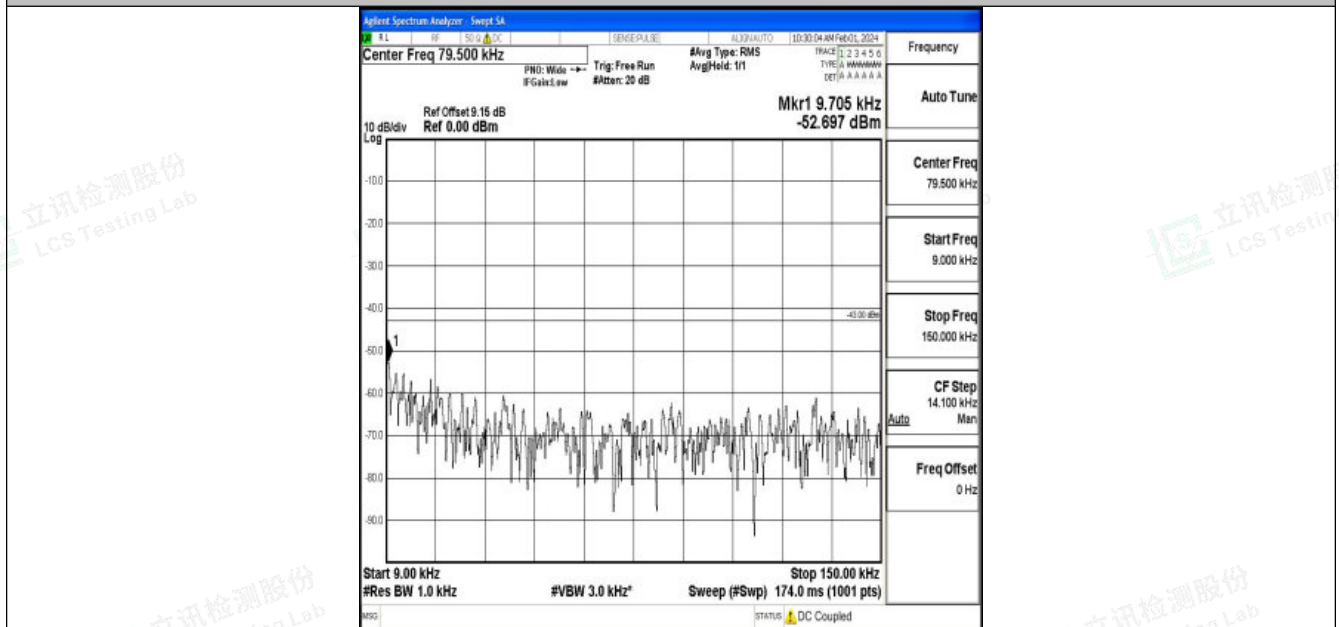
Band2_20MHz_16QAM_19100_1RB#0_0.009~0.15_0.009~0.15
