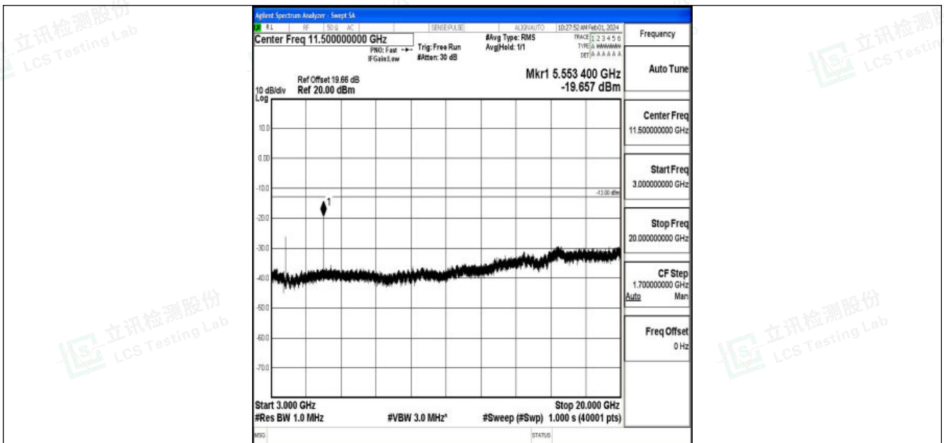
Band2_20MHz_QPSK_18700_1RB#0_3000~20000_3000~20000
