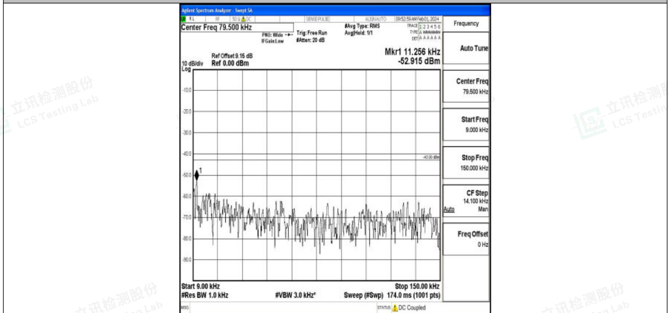
Band2_10MHz_16QAM_18650_1RB#0_0.009~0.15_0.009~0.15
