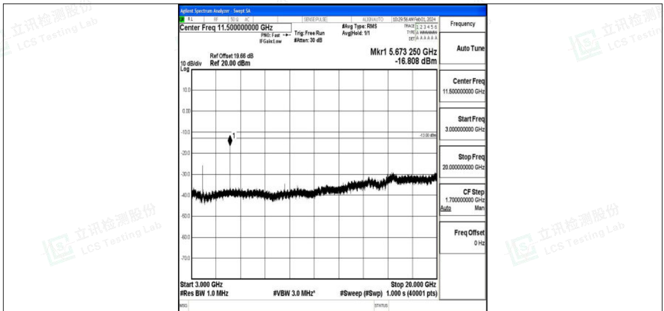
Band2_20MHz_QPSK_19100_1RB#0_3000~20000_3000~20000
