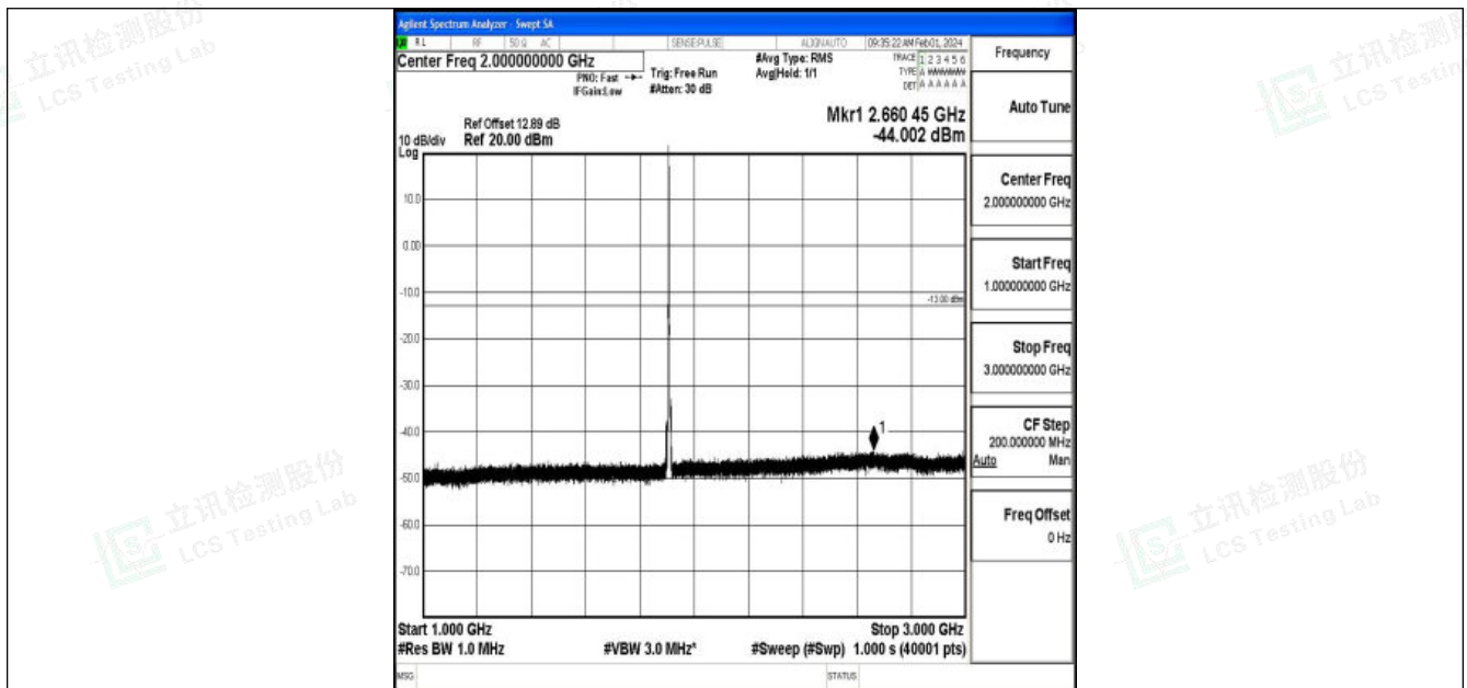
Band2_5MHz_16QAM_19175_1RB#0_1000~3000_1000~3000
