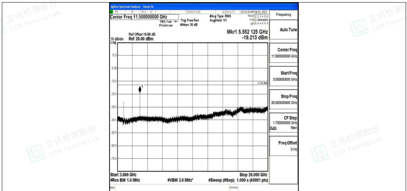
Band2_15MHz_QPSK_18675_1RB#0_3000~20000_3000~20000
