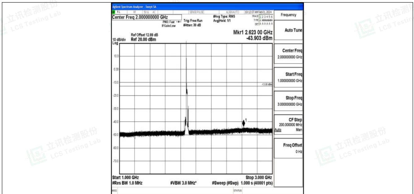
Band2_15MHz_16QAM_18900_1RB#0_1000~3000_1000~3000
