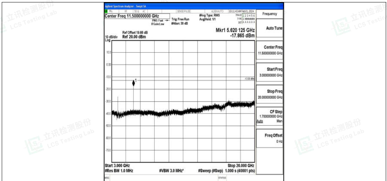
Band2_15MHz_QPSK_18900_1RB#0_3000~20000_3000~20000
