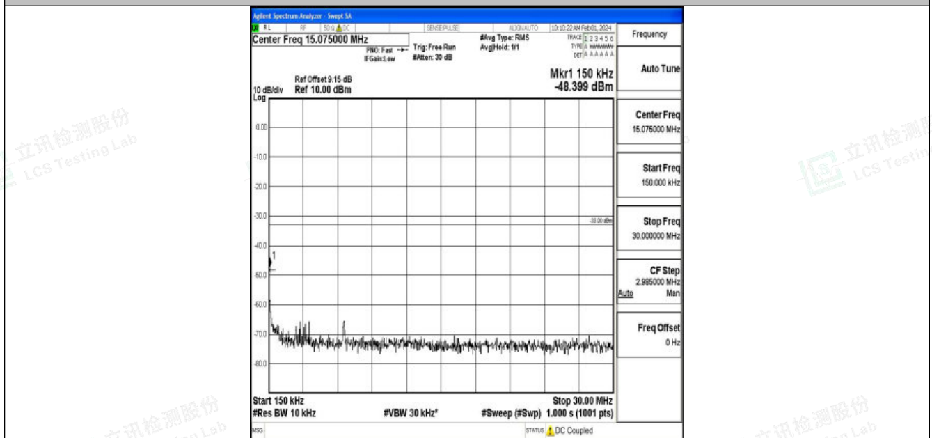
Band2_15MHz_QPSK_18675_1RB#0_0.15~30_0.15~30
