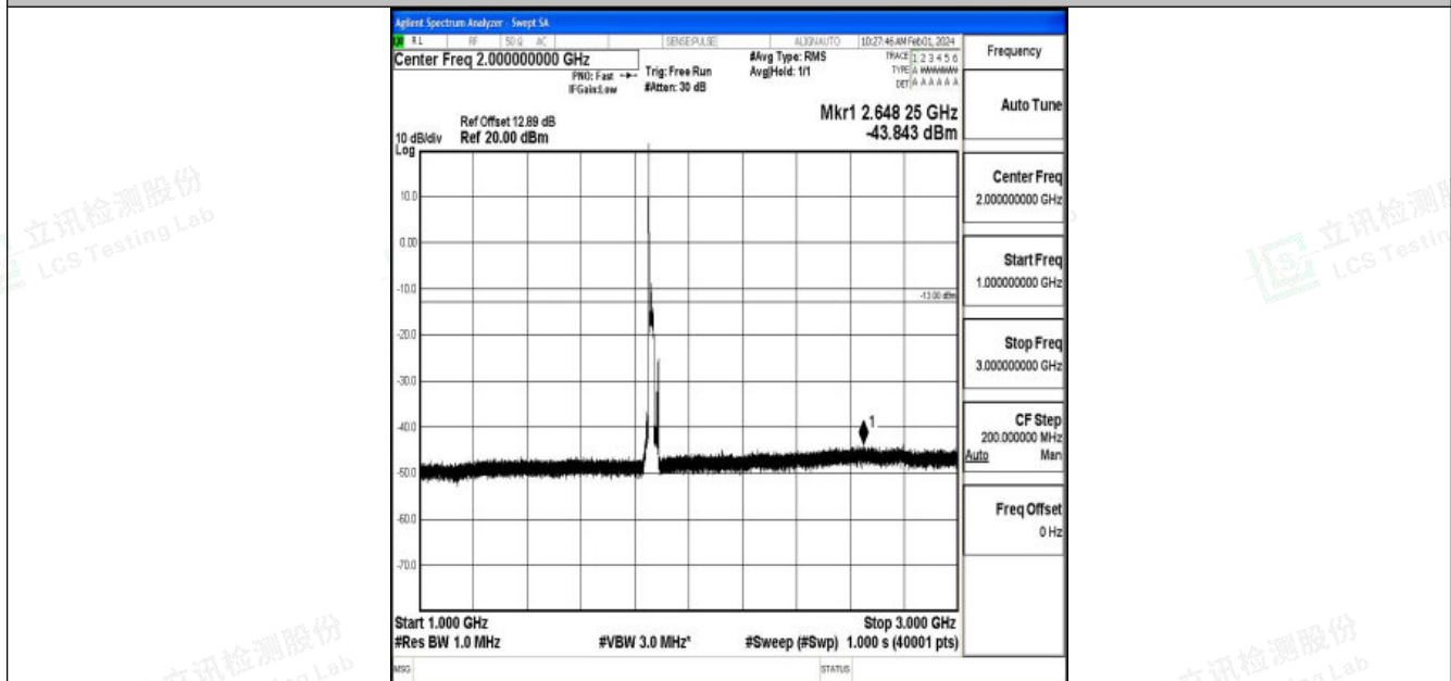
Band2_20MHz_QPSK_18700_1RB#0_1000~3000_1000~3000
