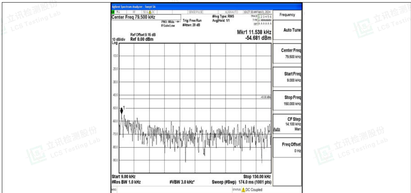
Band2_20MHz_QPSK_18700_1RB#0_0.009~0.15_0.009~0.15
