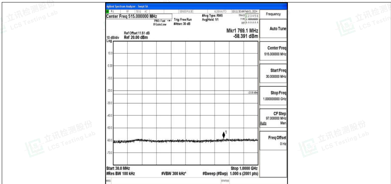
Band2_15MHz_QPSK_18900_1RB#0_30~1000_30~1000
