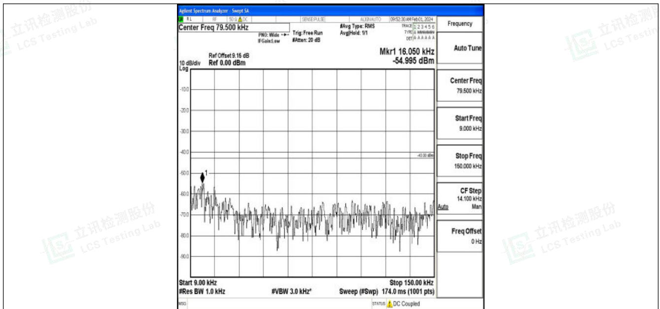
Band2_10MHz_QPSK_18650_1RB#0_0.009~0.15_0.009~0.15
