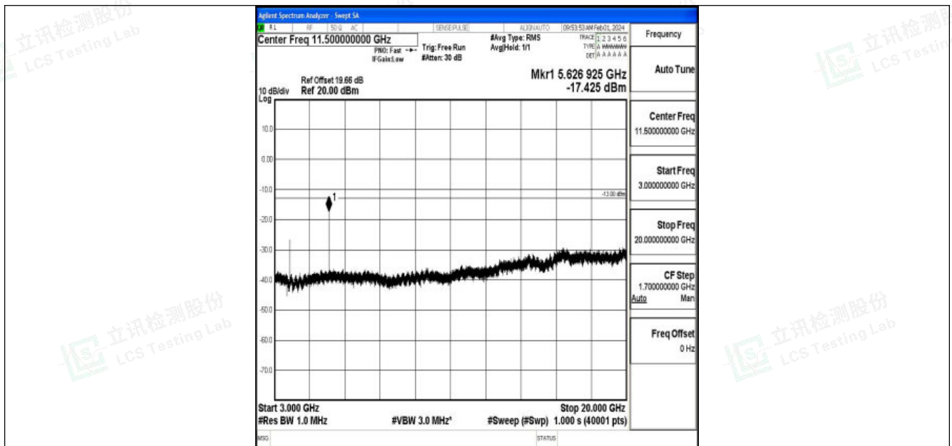
Band2_10MHz_QPSK_18900_1RB#0_3000~20000_3000~20000
