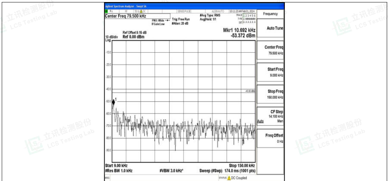
Band2_15MHz_QPSK_18900_1RB#0_0.009~0.15_0.009~0.15
