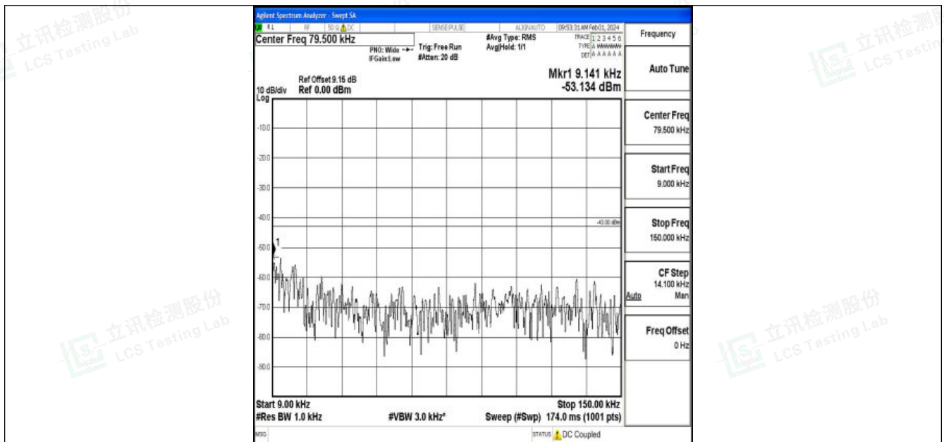
Band2_10MHz_QPSK_18900_1RB#0_0.009~0.15_0.009~0.15
