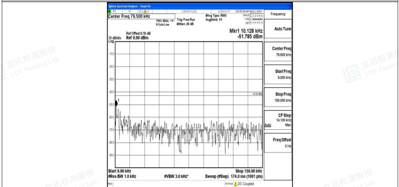
Band2_5MHz_16QAM_19175_1RB#0_0.009~0.15_0.009~0.15
