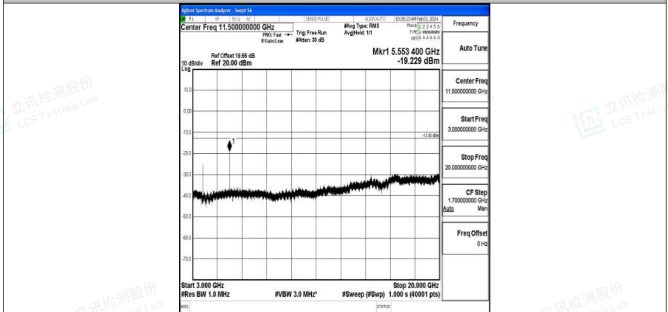
Band2_20MHz_16QAM_18700_1RB#0_3000~20000_3000~20000
