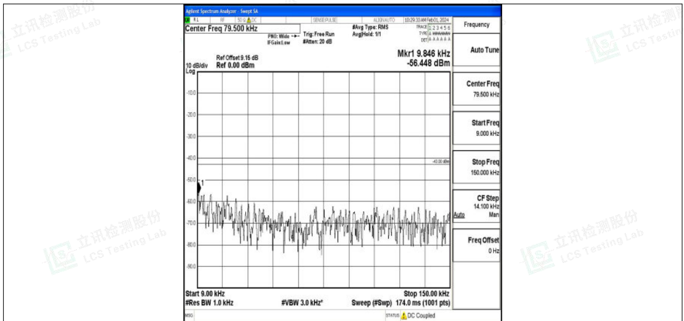
Band2_20MHz_QPSK_19100_1RB#0_0.009~0.15_0.009~0.15
