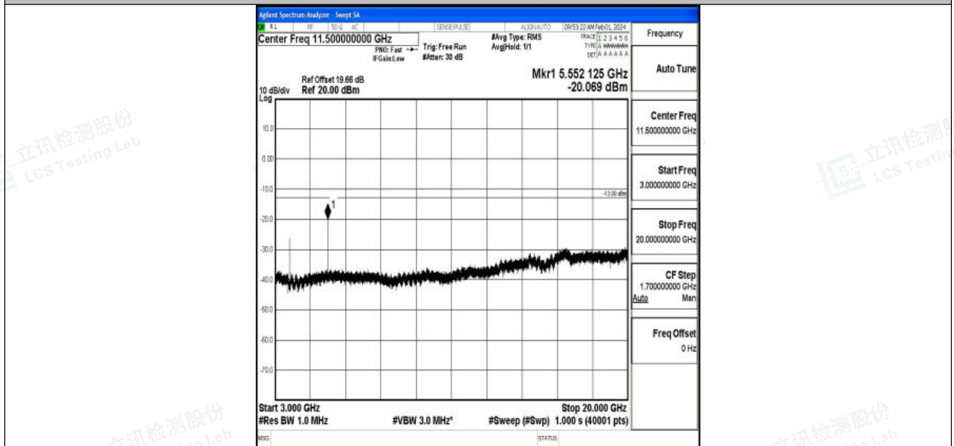
Band2_10MHz_16QAM_18650_1RB#0_3000~20000_3000~20000
