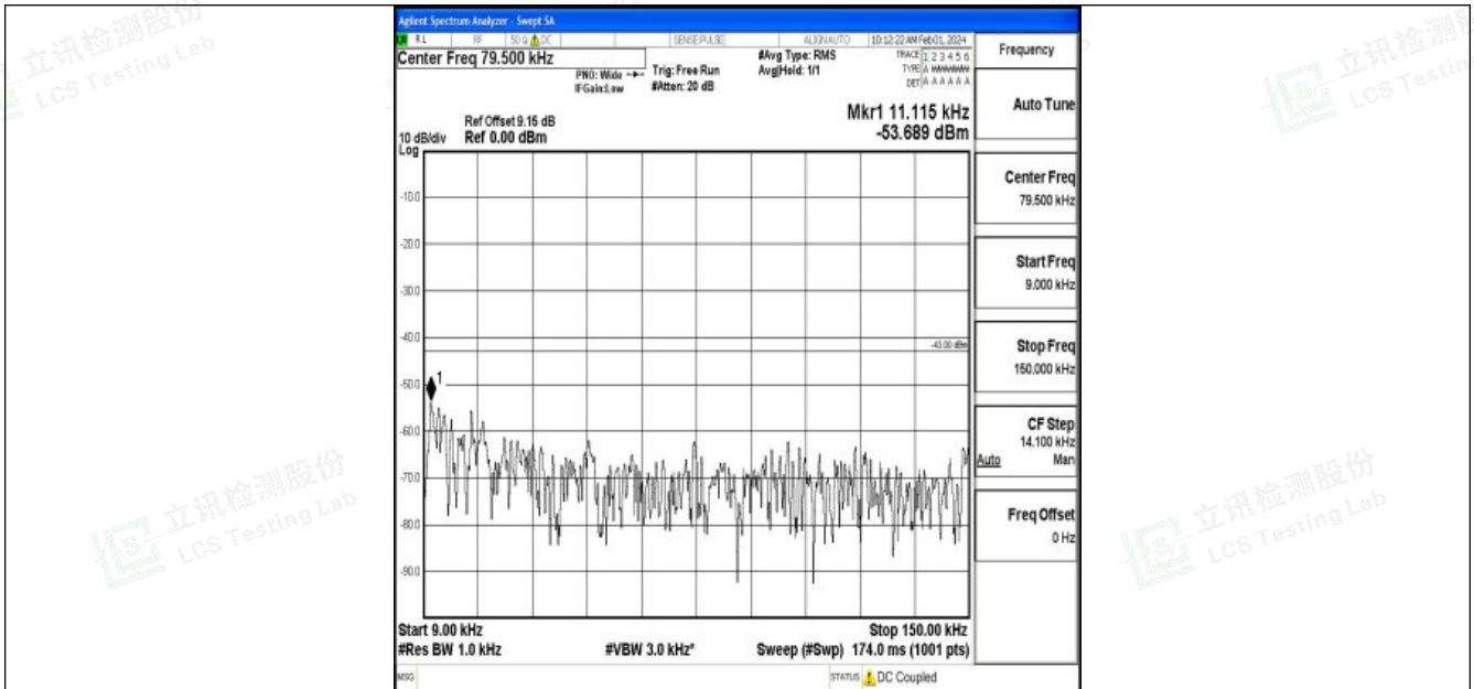
Band2_15MHz_QPSK_19125_1RB#0_0.009~0.15_0.009~0.15
