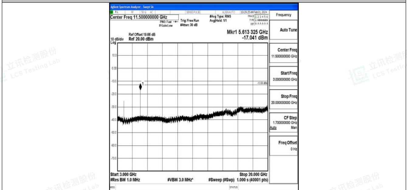
Band2_20MHz_16QAM_18900_1RB#0_3000~20000_3000~20000
