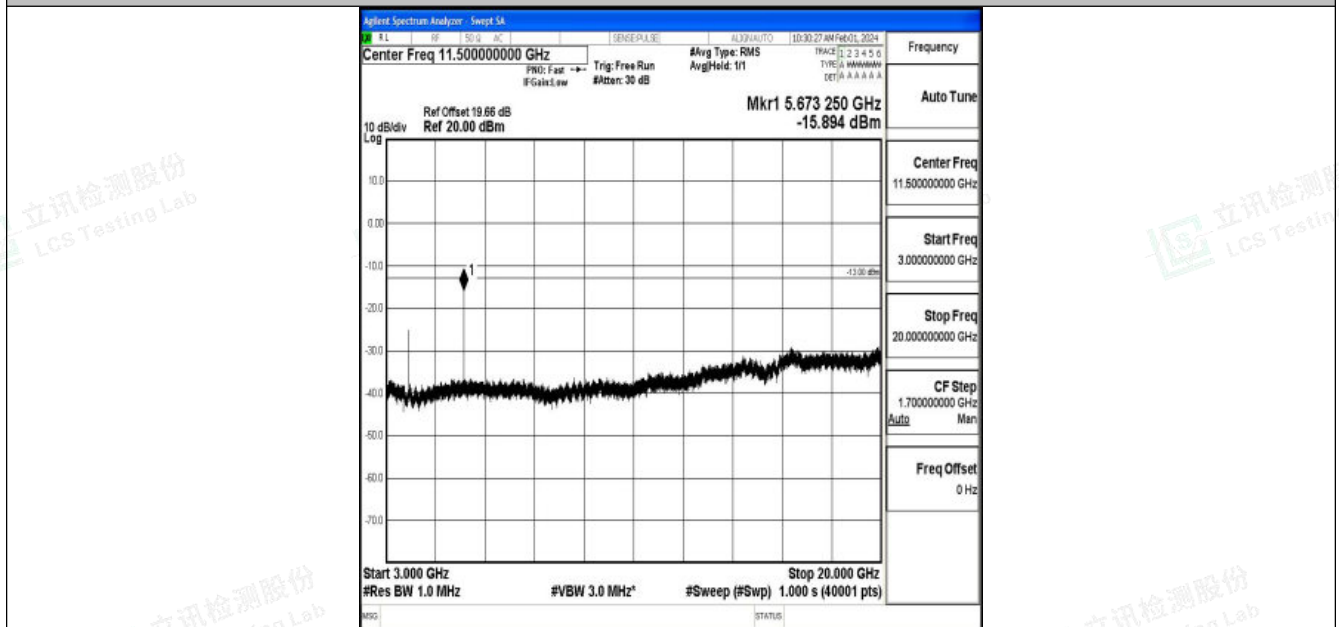
Band2_20MHz_16QAM_19100_1RB#0_3000~20000_3000~20000
