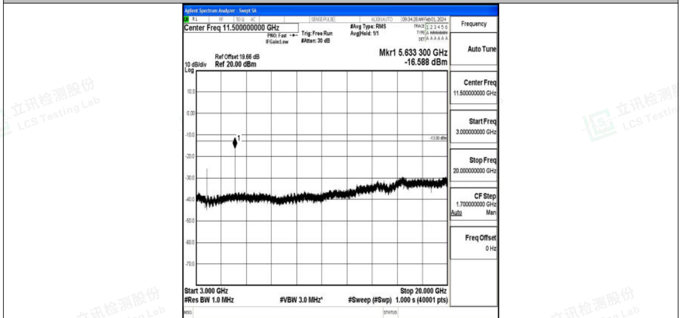
Band2_5MHz_16QAM_18900_1RB#0_3000~20000_3000~20000
