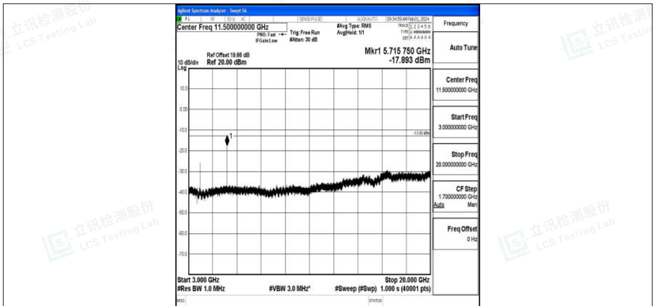
Band2_5MHz_QPSK_19175_1RB#0_3000~20000_3000~20000
