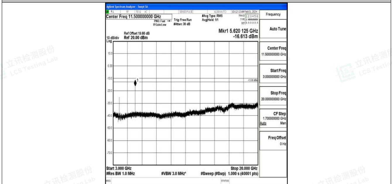
Band2_15MHz_16QAM_18900_1RB#0_3000~20000_3000~20000
