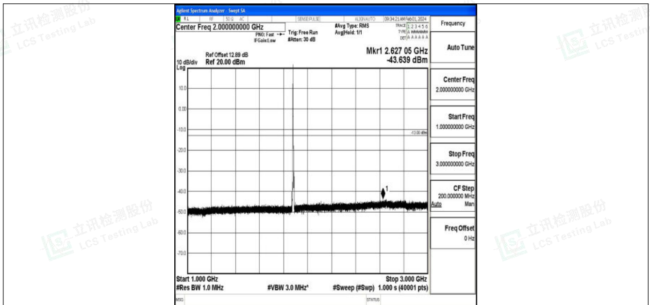
Band2_5MHz_16QAM_18900_1RB#0_1000~3000_1000~3000
