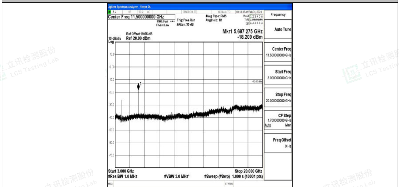
Band2_15MHz_16QAM_19125_1RB#0_3000~20000_3000~20000
