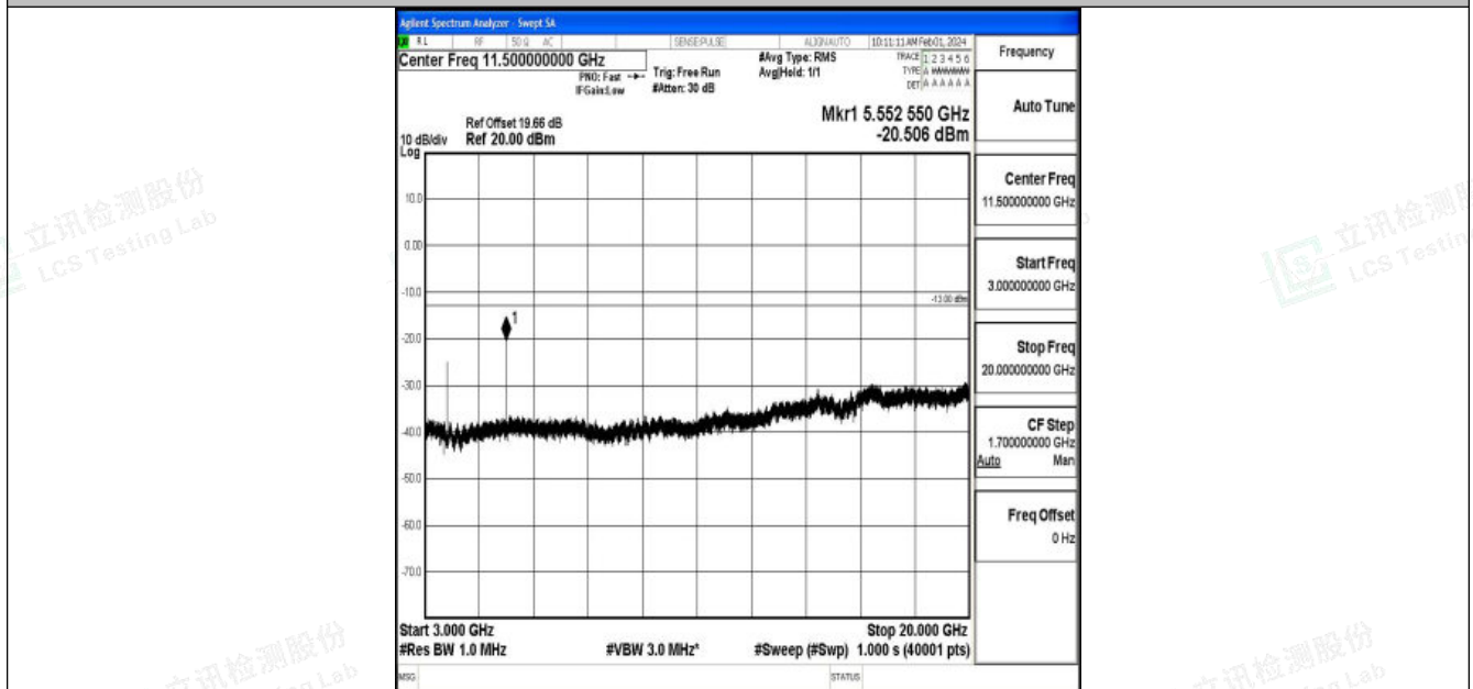
Band2_15MHz_16QAM_18675_1RB#0_3000~20000_3000~20000
