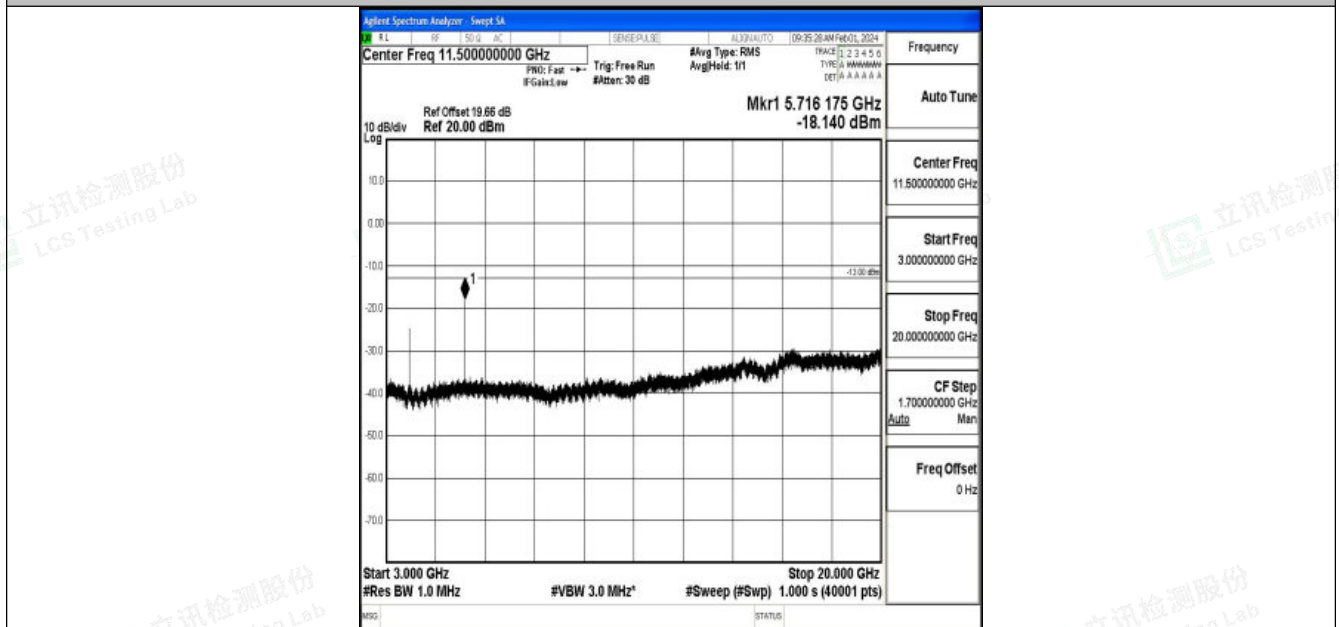
Band2_5MHz_16QAM_19175_1RB#0_3000~20000_3000~20000
