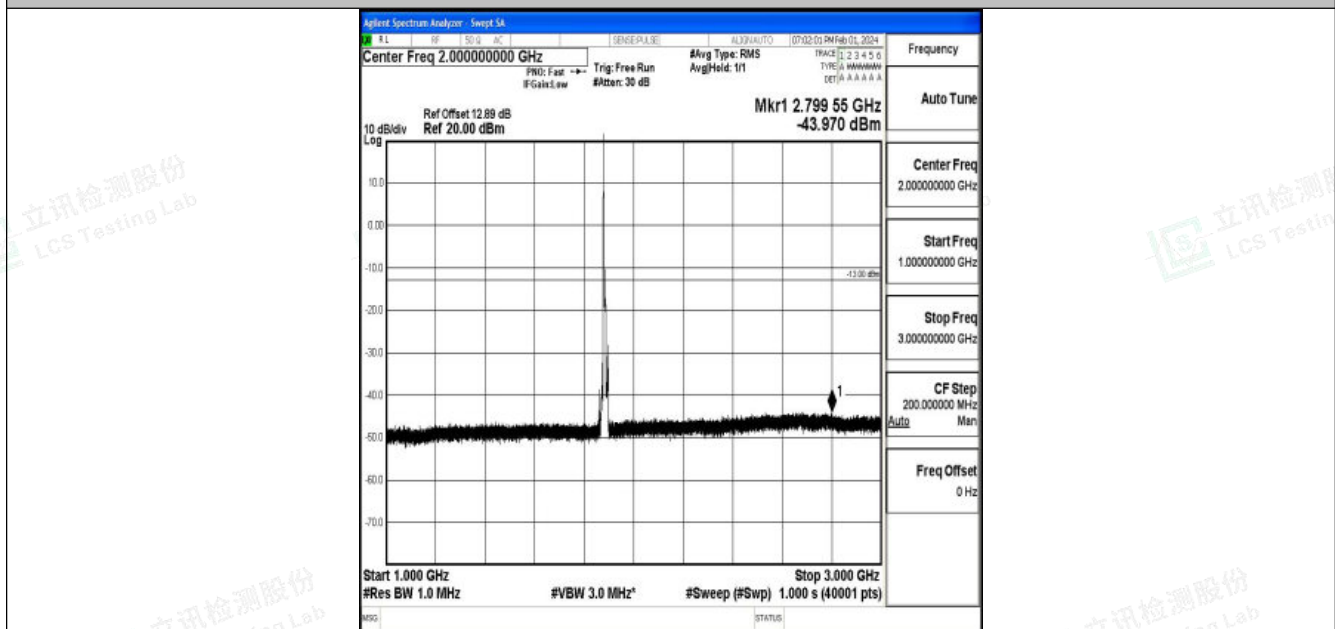
Band25_10MHz_QPSK_26365_1RB#0_1000~3000_1000~3000
