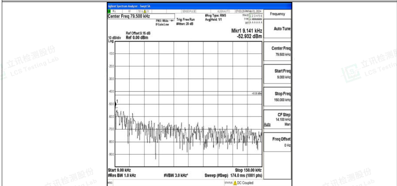
Band25_10MHz_16QAM_26640_1RB#0_0.009~0.15_0.009~0.15
