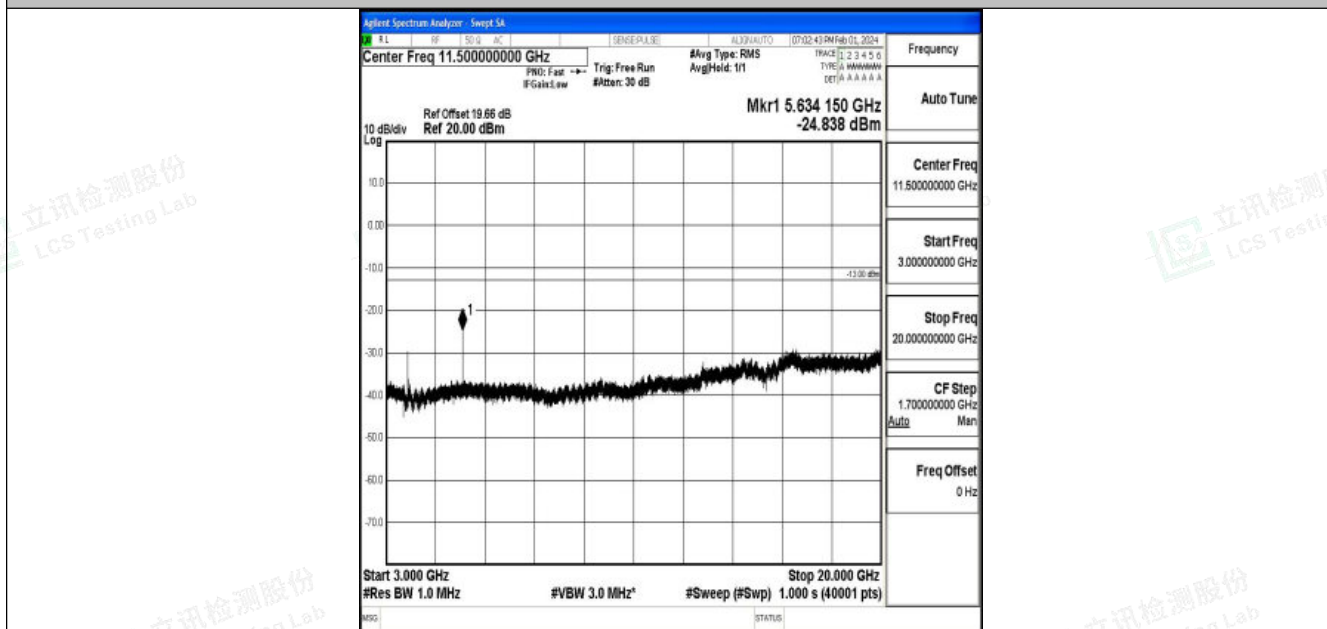
Band25_10MHz_16QAM_26365_1RB#0_3000~20000_3000~20000
