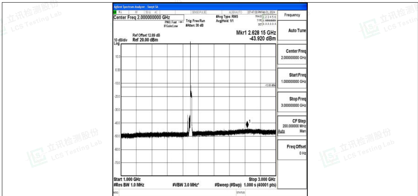
Band25_20MHz_16QAM_26590_1RB#0_1000~3000_1000~3000
