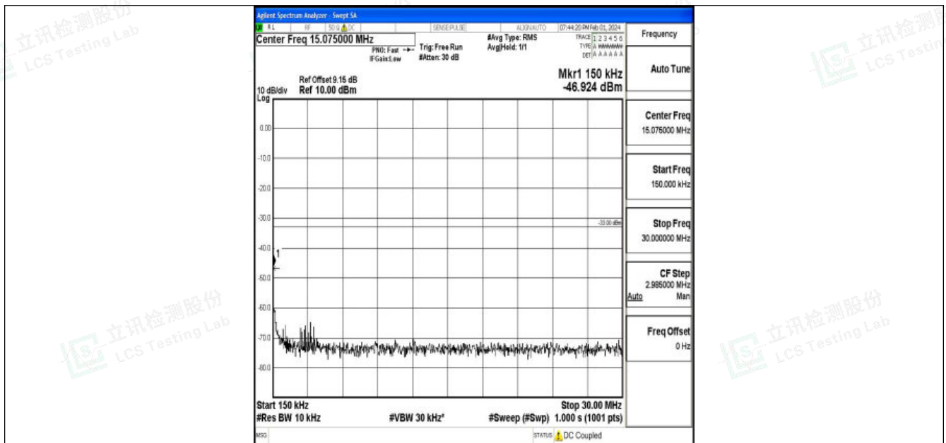
Band25_20MHz_16QAM_26140_1RB#0_0.15~30_0.15~30
