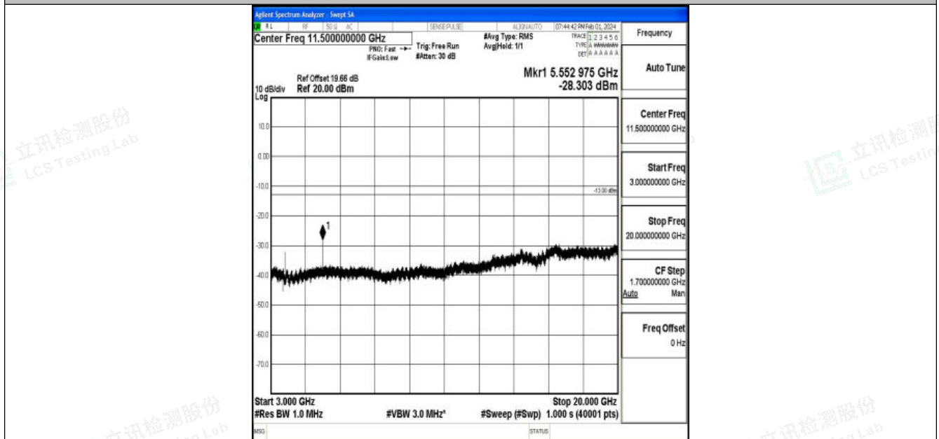
Band25_20MHz_16QAM_26140_1RB#0_3000~20000_3000~20000
