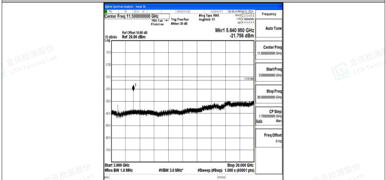
Band25_5MHz_16QAM_26365_1RB#0_3000~20000_3000~20000
