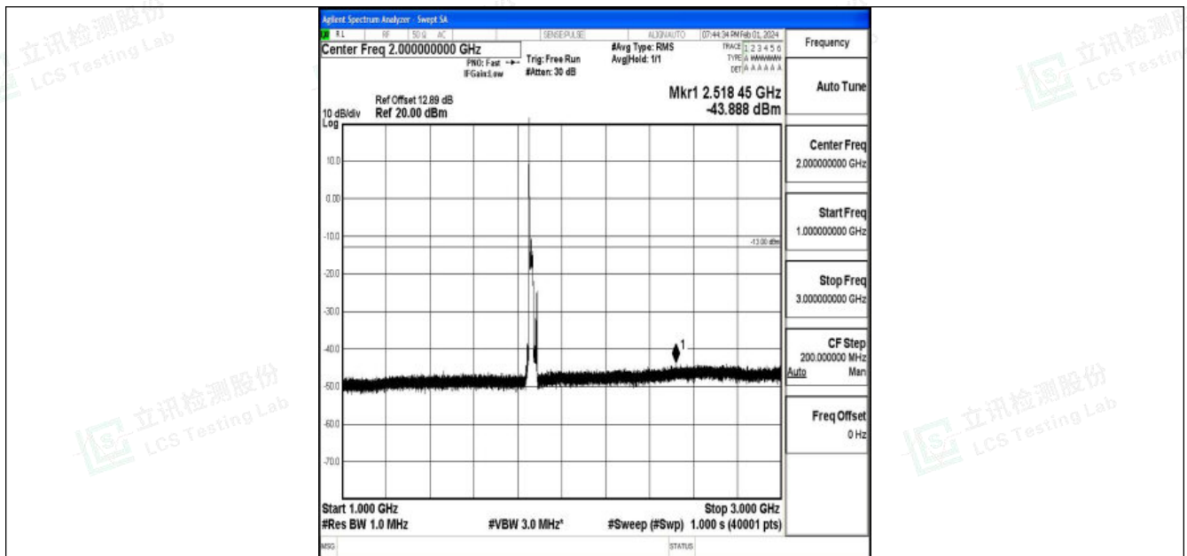
Band25_20MHz_16QAM_26140_1RB#0_1000~3000_1000~3000
