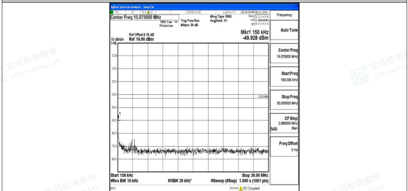
Band25_5MHz_QPSK_26665_1RB#0_0.15~30_0.15~30
