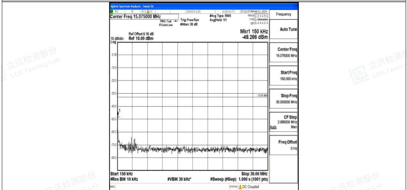
Band25_15MHz_QPSK_26115_1RB#0_0.15~30_0.15~30
