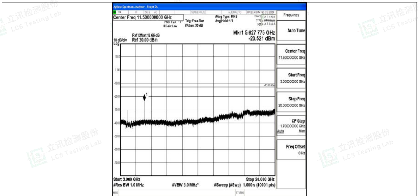
Band25_15MHz_QPSK_26365_1RB#0_3000~20000_3000~20000
