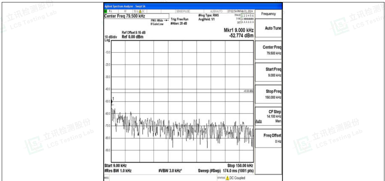
Band25_10MHz_QPSK_26640_1RB#0_0.009~0.15_0.009~0.15
