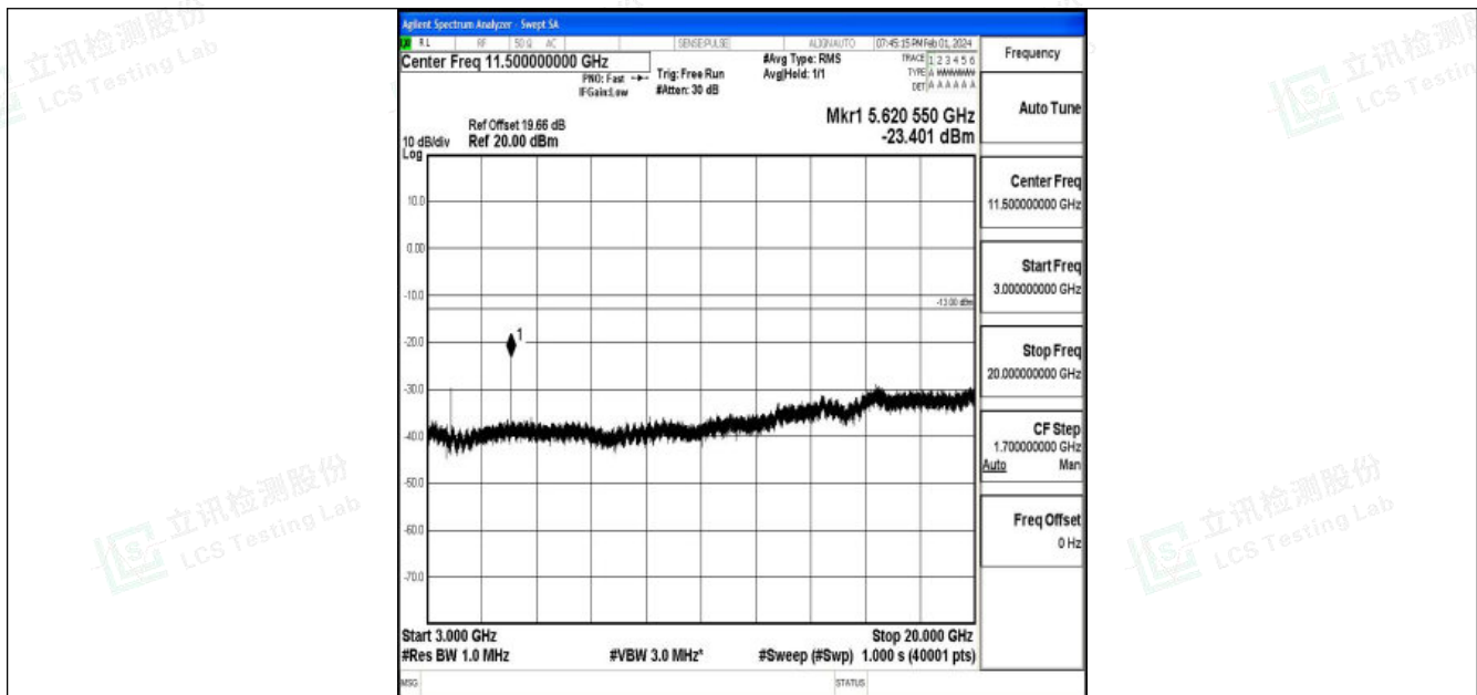
Band25_20MHz_QPSK_26365_1RB#0_3000~20000_3000~20000
