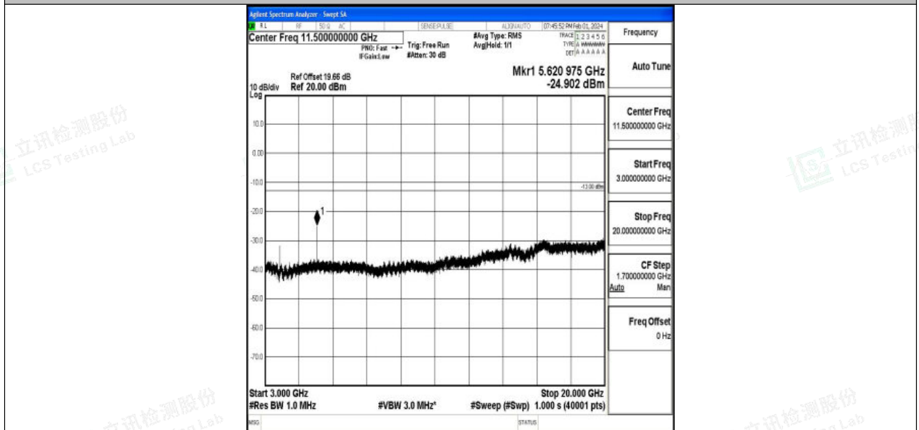
Band25_20MHz_16QAM_26365_1RB#0_3000~20000_3000~20000
