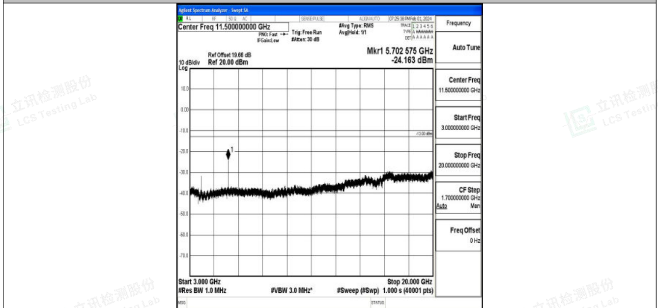
Band25_15MHz_16QAM_26615_1RB#0_3000~20000_3000~20000
