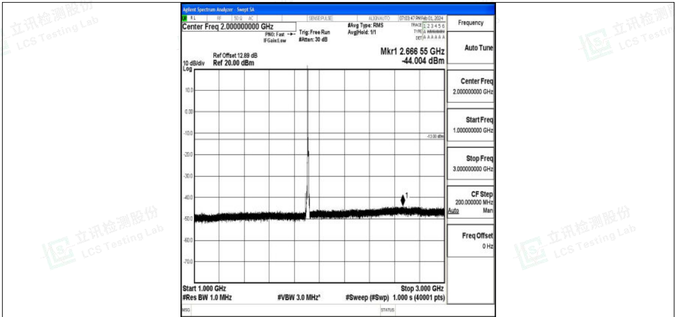
Band25_10MHz_16QAM_26640_1RB#0_1000~3000_1000~3000
