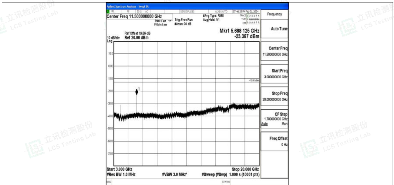
Band25_20MHz_QPSK_26590_1RB#0_3000~20000_3000~20000
