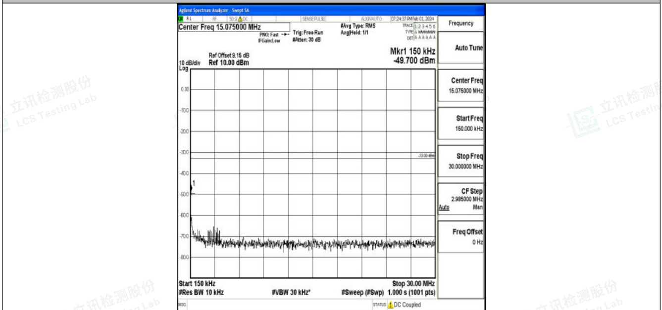
Band25_15MHz_QPSK_26615_1RB#0_0.15~30_0.15~30
