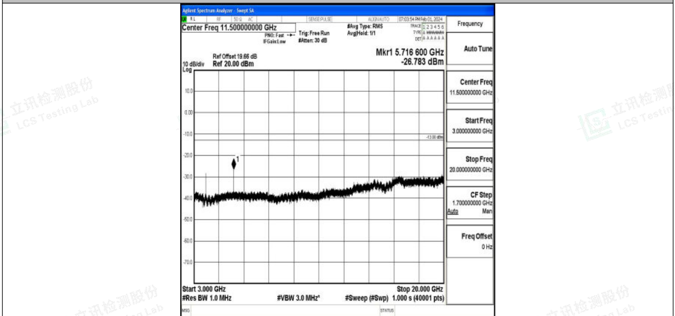
Band25_10MHz_16QAM_26640_1RB#0_3000~20000_3000~20000
