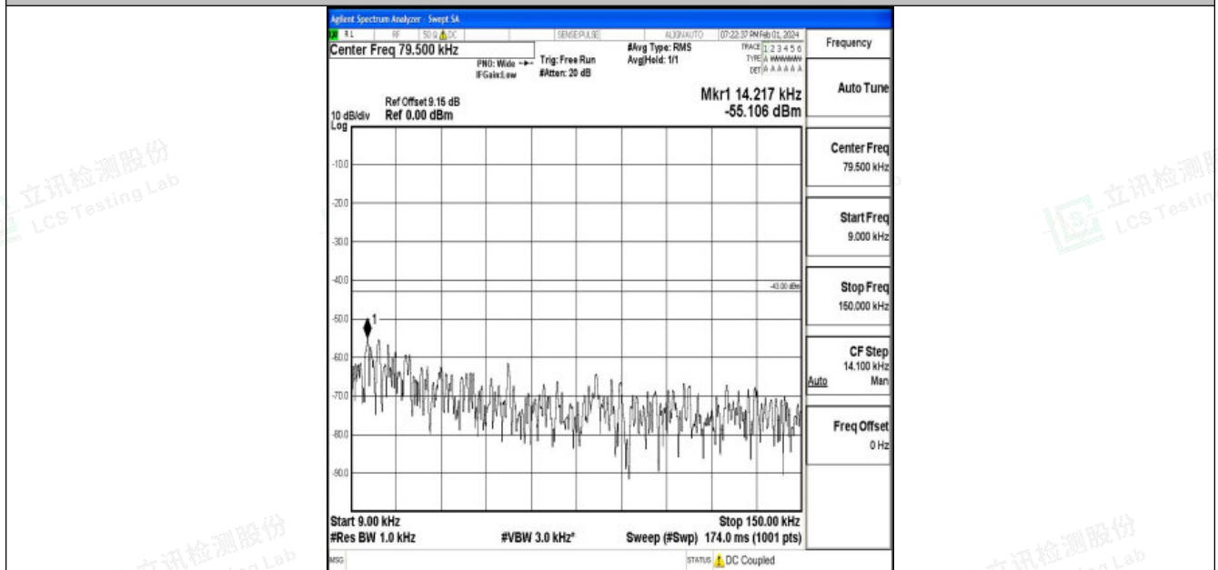
Band25_15MHz_16QAM_26115_1RB#0_0.009~0.15_0.009~0.15
