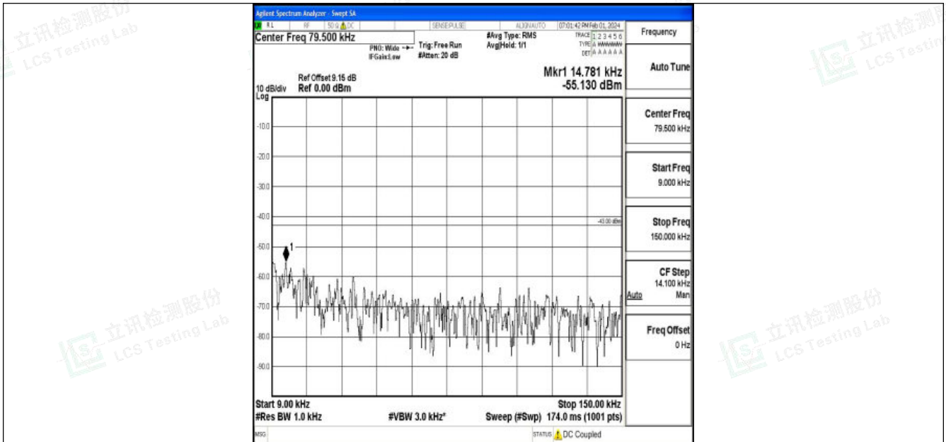
Band25_10MHz_QPSK_26365_1RB#0_0.009~0.15_0.009~0.15
