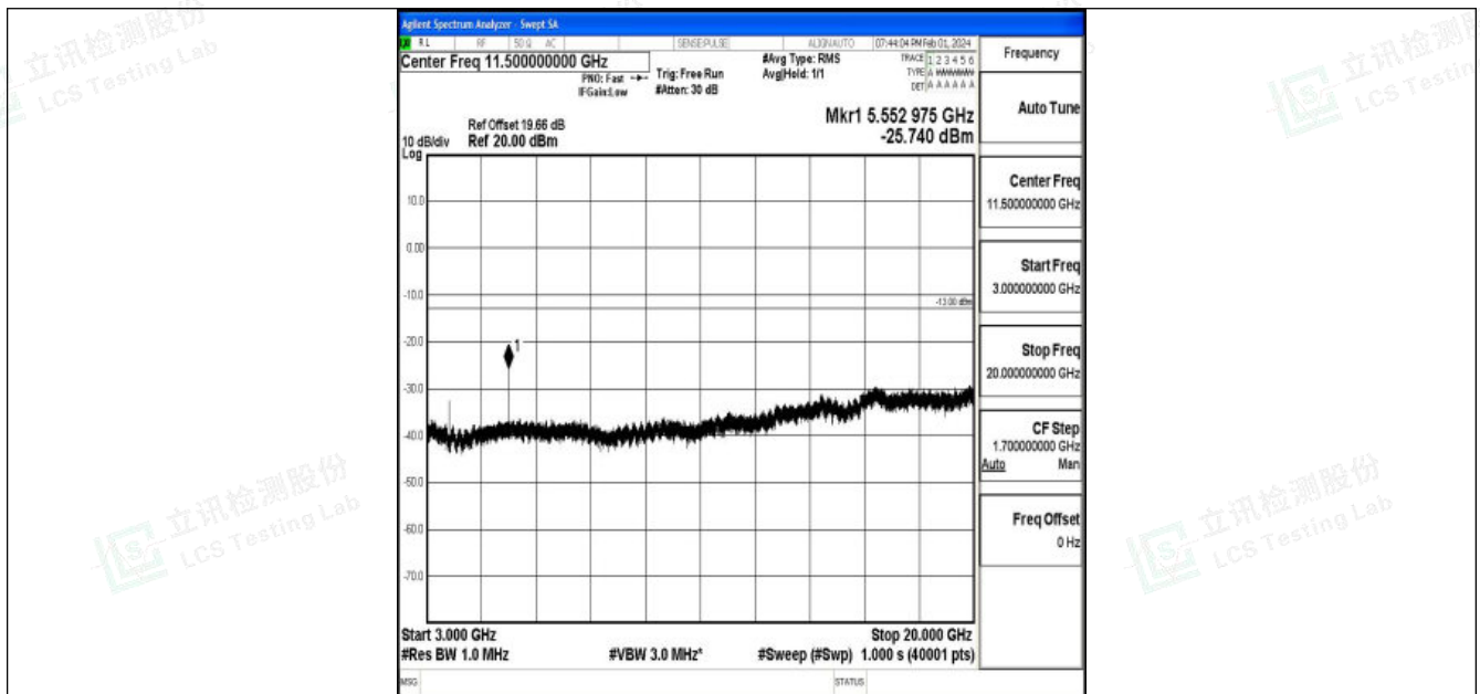
Band25_20MHz_QPSK_26140_1RB#0_3000~20000_3000~20000
