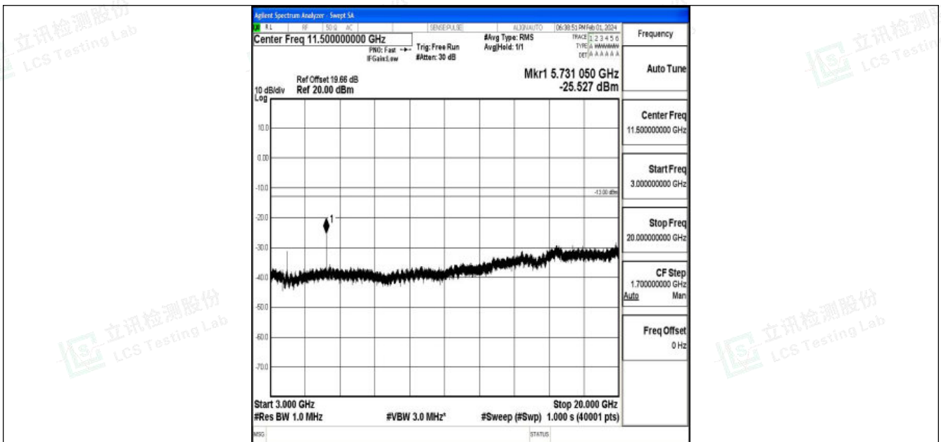
Band25_5MHz_QPSK_26665_1RB#0_3000~20000_3000~20000
