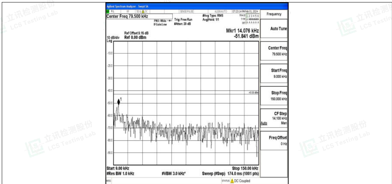
Band25_15MHz_QPSK_26365_1RB#0_0.009~0.15_0.009~0.15
