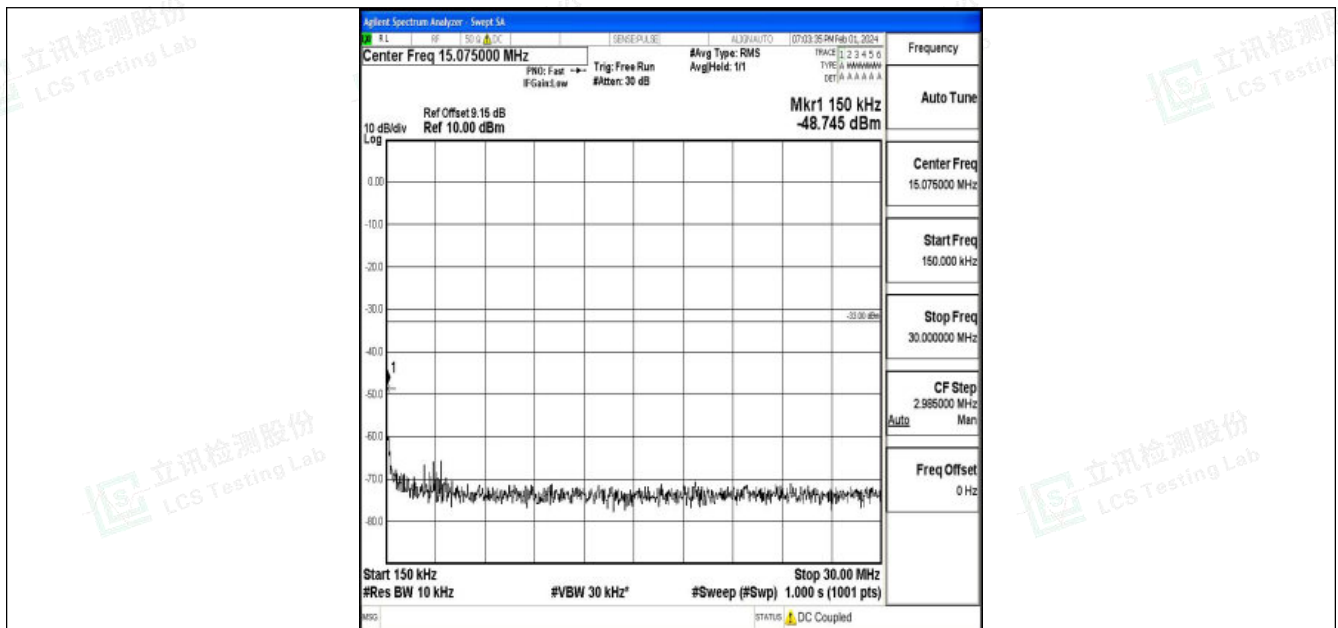
Band25_10MHz_16QAM_26640_1RB#0_0.15~30_0.15~30
