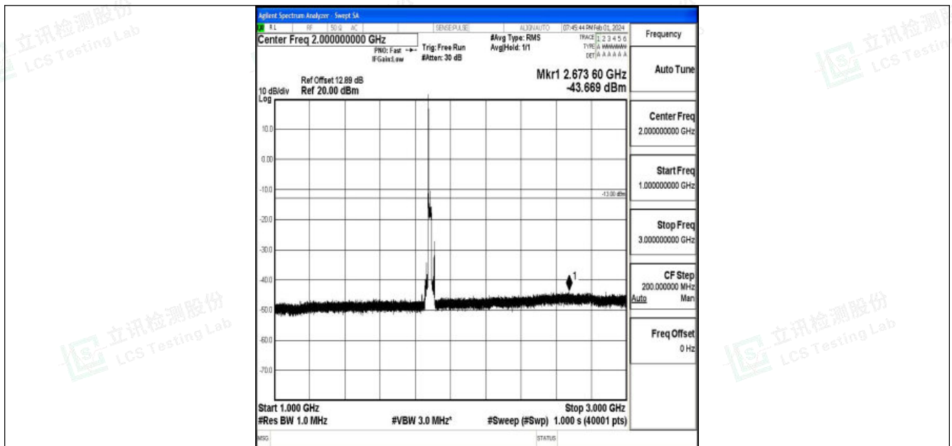
Band25_20MHz_16QAM_26365_1RB#0_1000~3000_1000~3000
