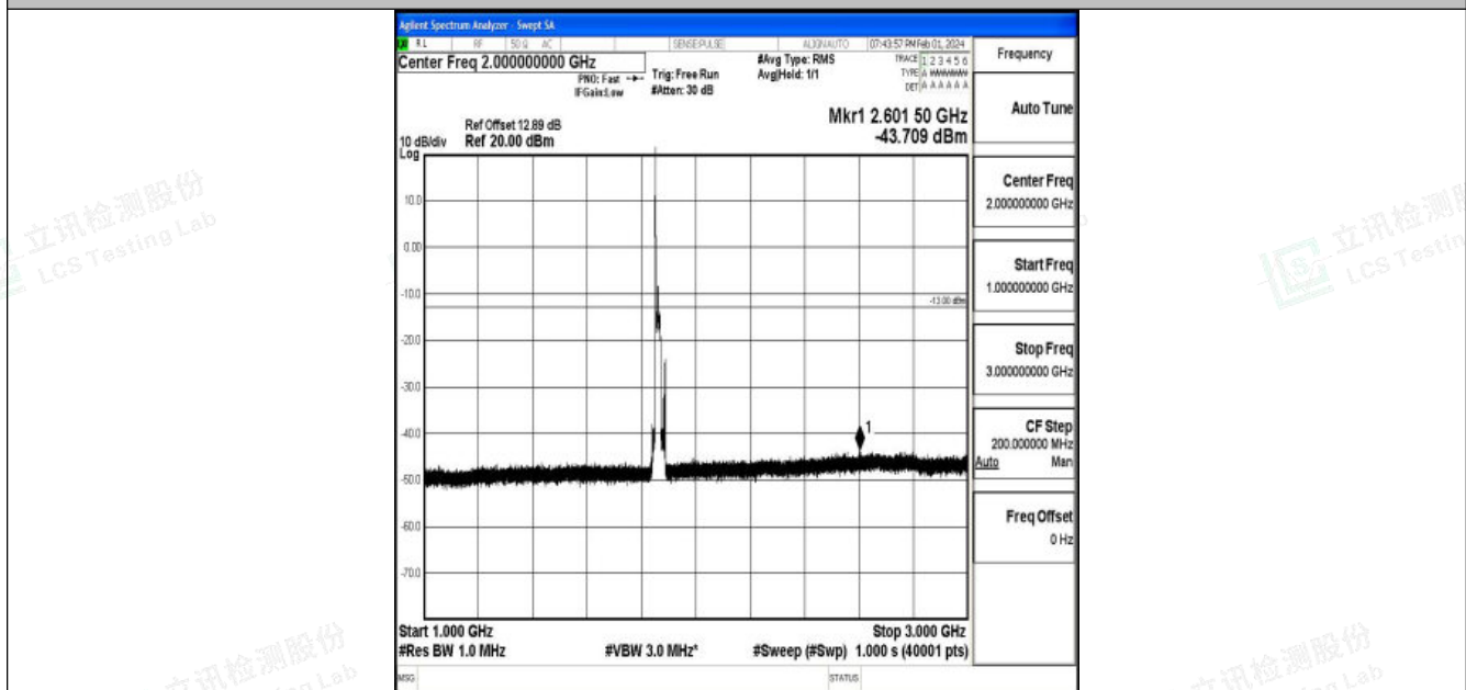
Band25_20MHz_QPSK_26140_1RB#0_1000~3000_1000~3000
