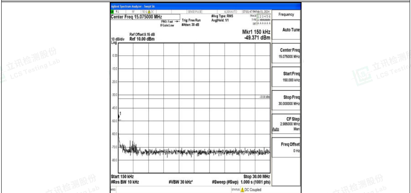
Band25_10MHz_QPSK_26365_1RB#0_0.15~30_0.15~30
