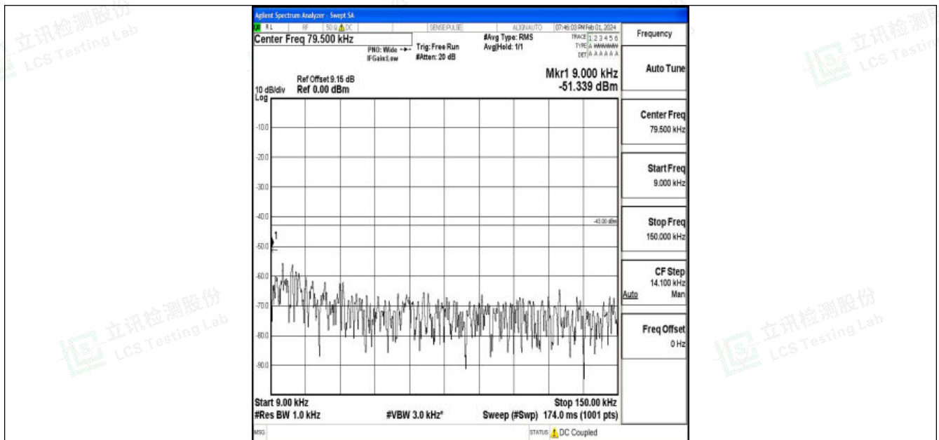
Band25_20MHz_QPSK_26590_1RB#0_0.009~0.15_0.009~0.15
