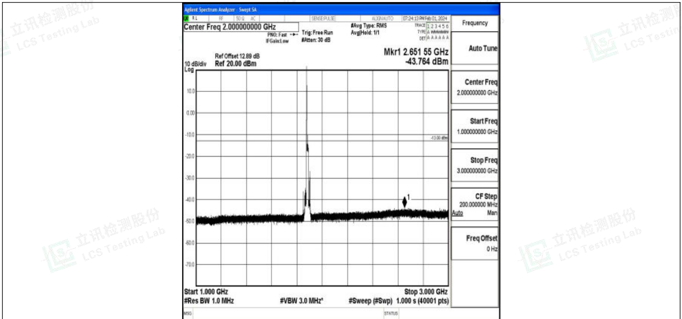
Band25_15MHz_16QAM_26365_1RB#0_1000~3000_1000~3000
