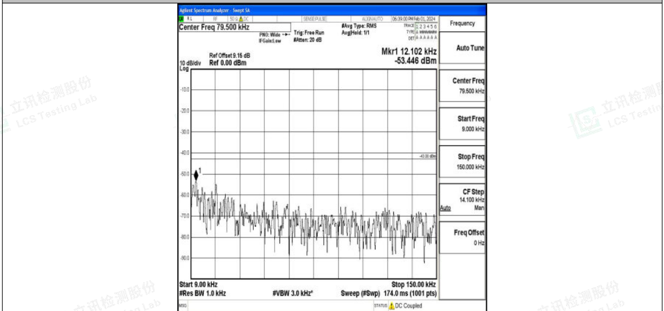
Band25_5MHz_16QAM_26665_1RB#0_0.009~0.15_0.009~0.15
