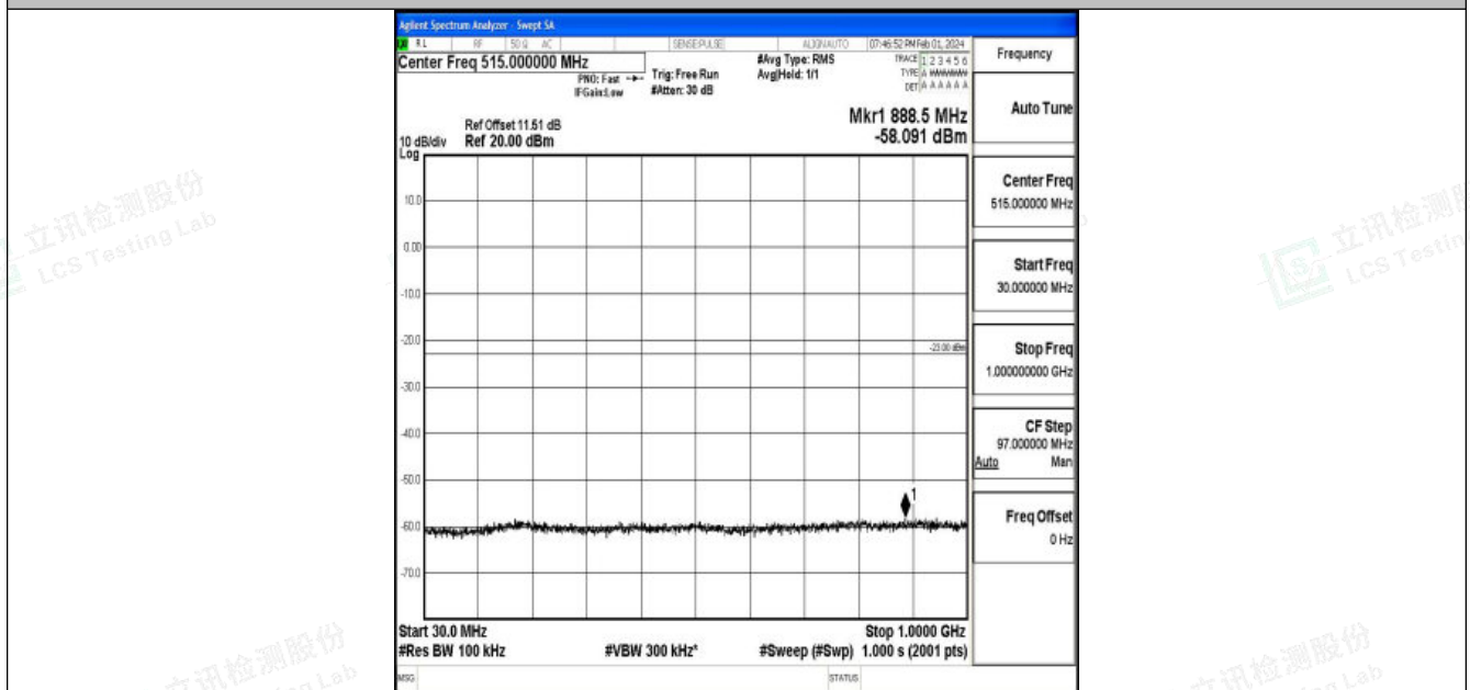
Band25_20MHz_16QAM_26590_1RB#0_30~1000_30~1000
