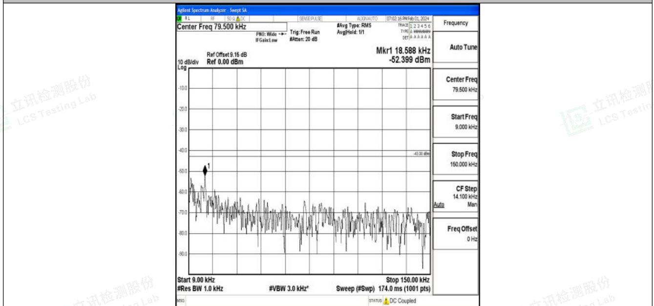
Band25_10MHz_16QAM_26365_1RB#0_0.009~0.15_0.009~0.15
