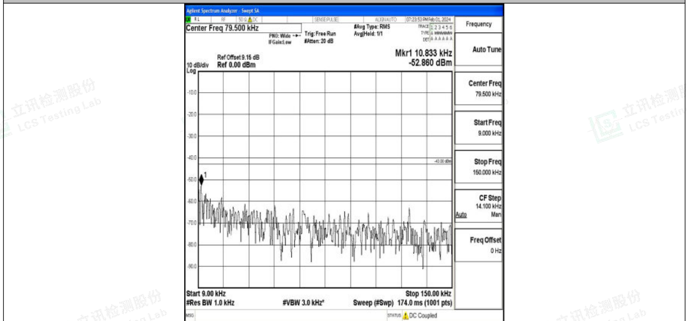
Band25_15MHz_16QAM_26365_1RB#0_0.009~0.15_0.009~0.15
