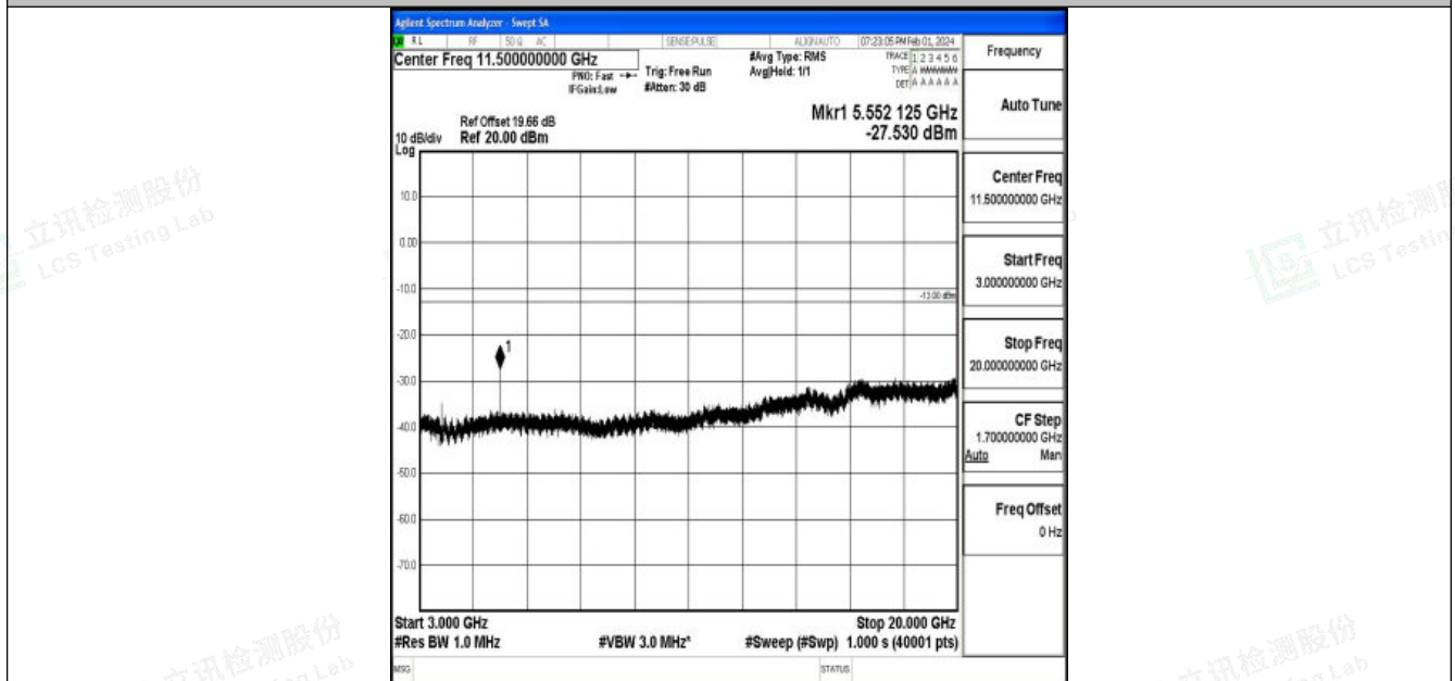
Band25_15MHz_16QAM_26115_1RB#0_3000~20000_3000~20000
