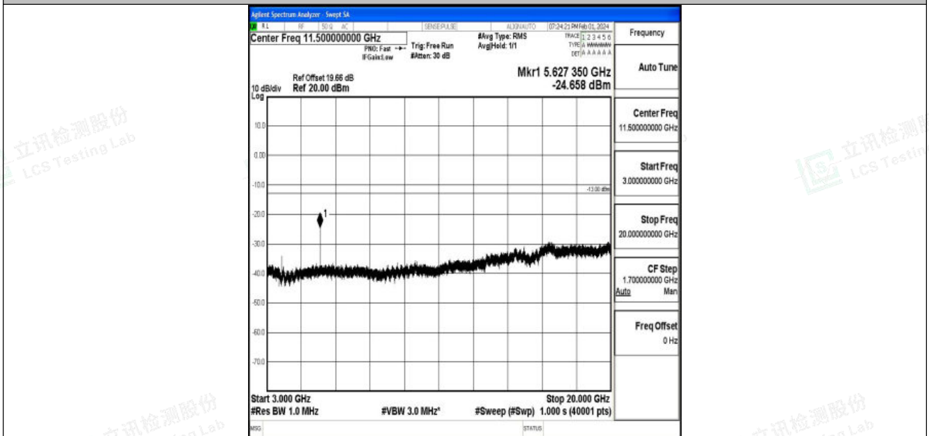
Band25_15MHz_16QAM_26365_1RB#0_3000~20000_3000~20000
