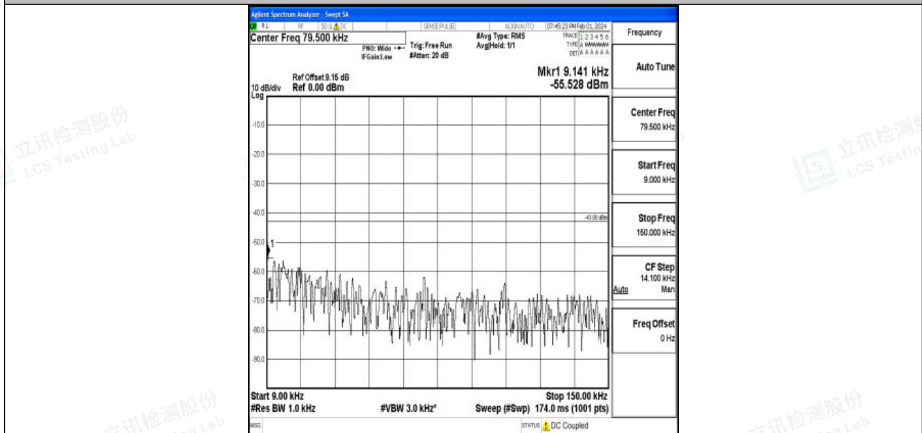
Band25_20MHz_16QAM_26365_1RB#0_0.009~0.15_0.009~0.15
