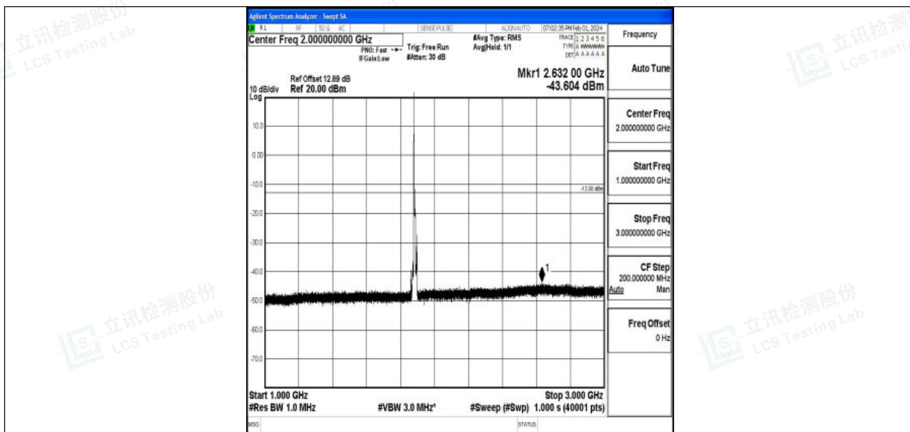
Band25_10MHz_16QAM_26365_1RB#0_1000~3000_1000~3000
