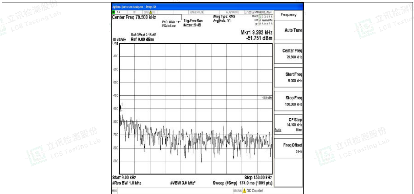
Band25_15MHz_QPSK_26115_1RB#0_0.009~0.15_0.009~0.15
