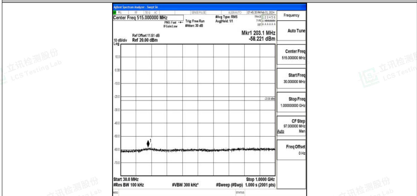
Band25_20MHz_16QAM_26365_1RB#0_30~1000_30~1000
