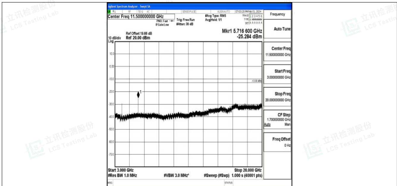
Band25_10MHz_QPSK_26640_1RB#0_3000~20000_3000~20000
