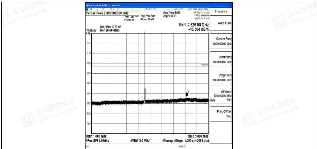
Band25_5MHz_16QAM_26665_1RB#0_1000~3000_1000~3000
