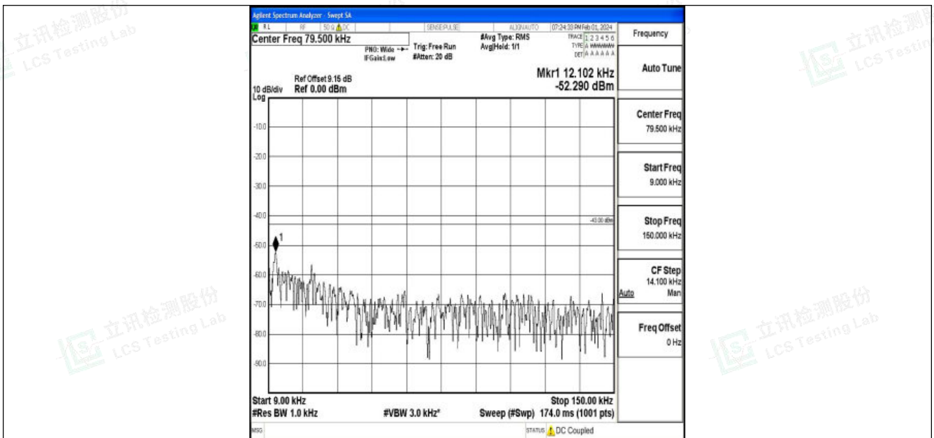
Band25_15MHz_QPSK_26615_1RB#0_0.009~0.15_0.009~0.15
