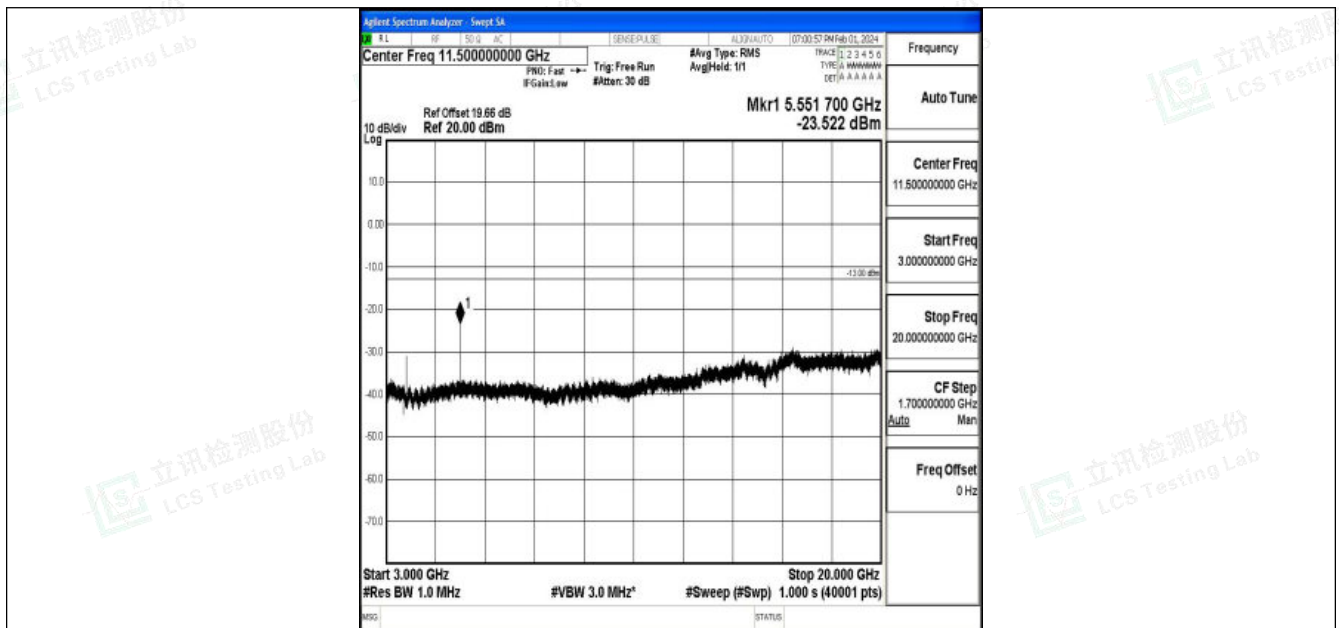
Band25_10MHz_QPSK_26090_1RB#0_3000~20000_3000~20000
