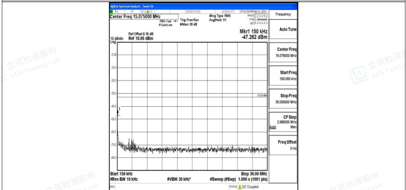
Band25_10MHz_QPSK_26640_1RB#0_0.15~30_0.15~30
