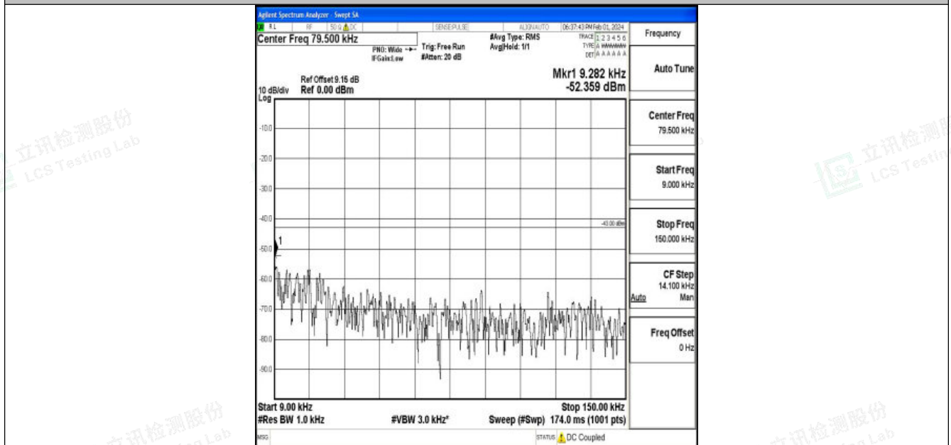
Band25_5MHz_16QAM_26365_1RB#0_0.009~0.15_0.009~0.15
