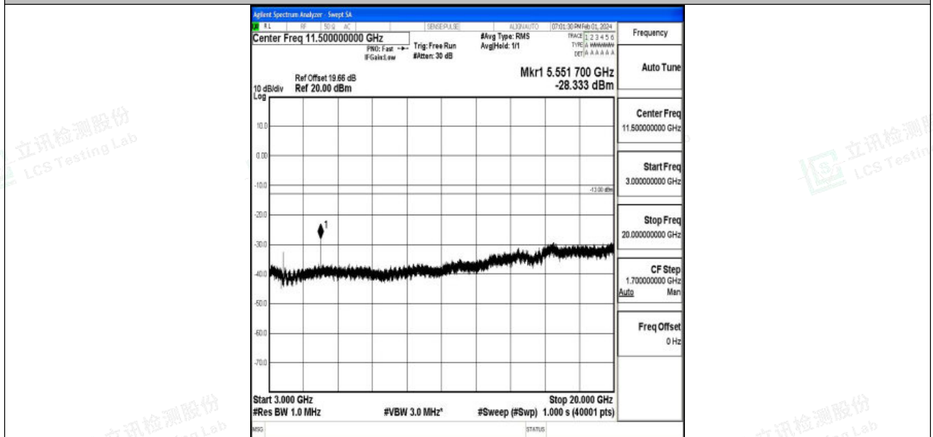
Band25_10MHz_16QAM_26090_1RB#0_3000~20000_3000~20000
