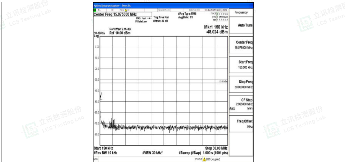
Band25_20MHz_16QAM_26365_1RB#0_0.15~30_0.15~30
