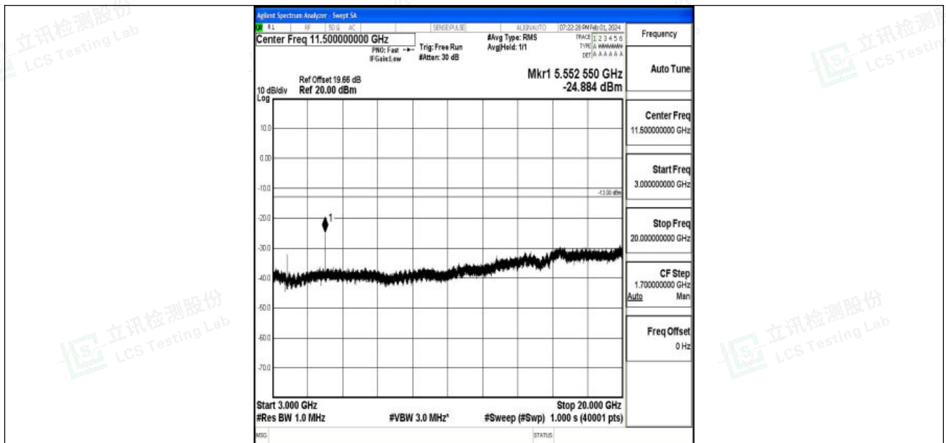
Band25_15MHz_QPSK_26115_1RB#0_3000~20000_3000~20000
