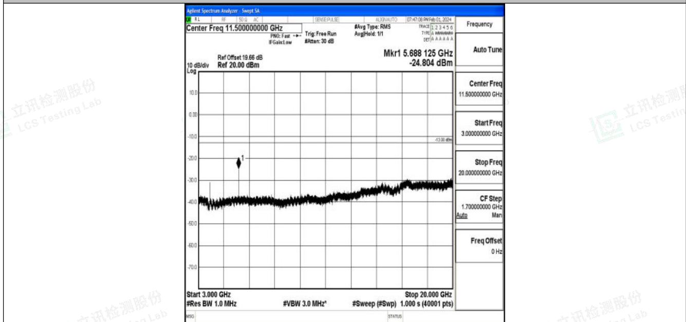
Band25_20MHz_16QAM_26590_1RB#0_3000~20000_3000~20000
