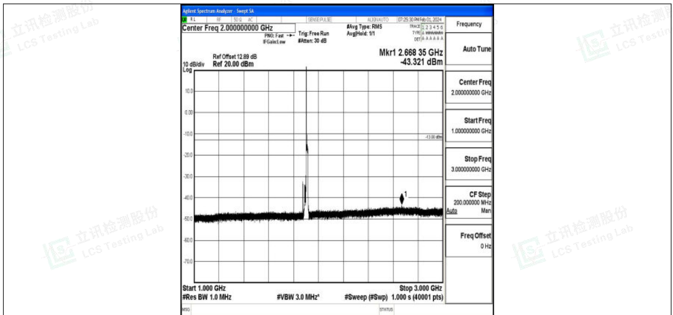
Band25_15MHz_16QAM_26615_1RB#0_1000~3000_1000~3000
