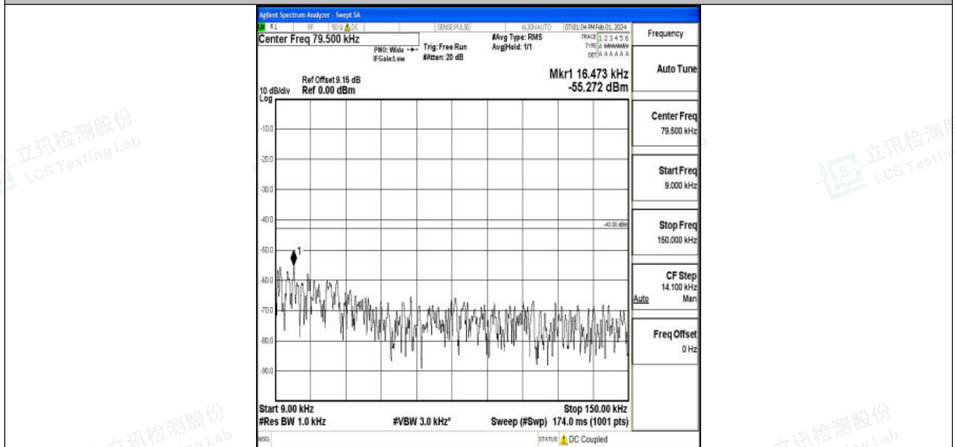
Band25_10MHz_16QAM_26090_1RB#0_0.009~0.15_0.009~0.15
