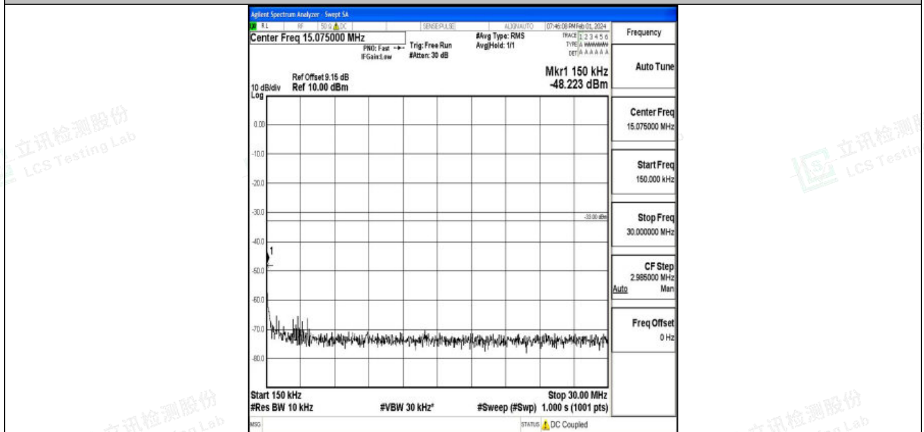
Band25_20MHz_QPSK_26590_1RB#0_0.15~30_0.15~30
