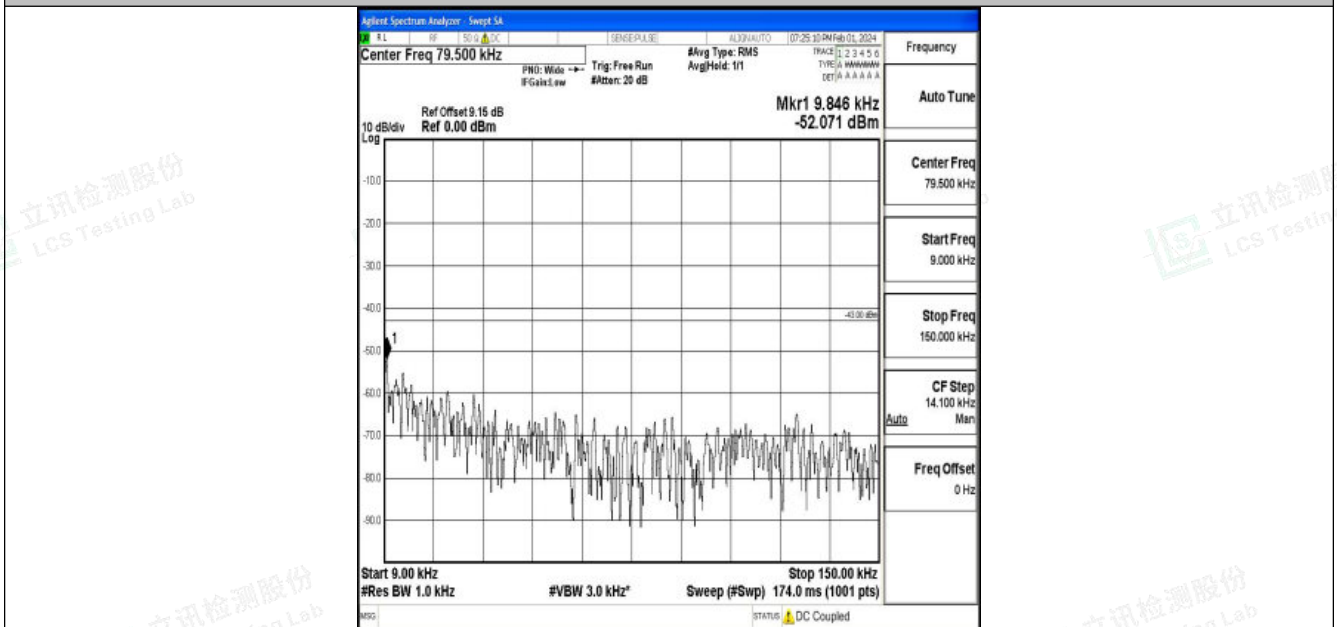
Band25_15MHz_16QAM_26615_1RB#0_0.009~0.15_0.009~0.15
