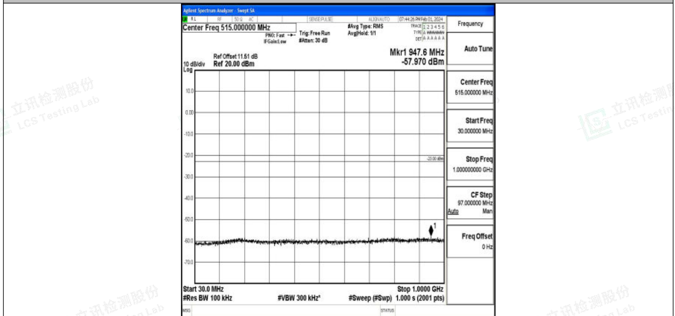
Band25_20MHz_16QAM_26140_1RB#0_30~1000_30~1000
