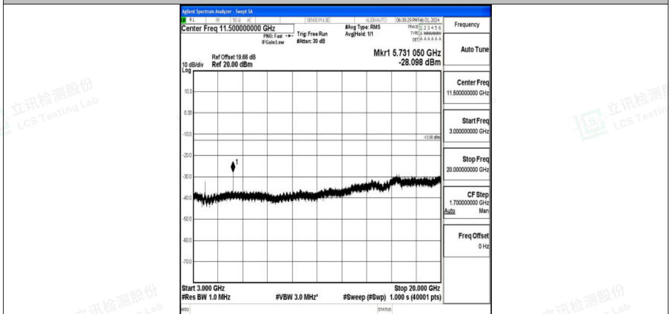
Band25_5MHz_16QAM_26665_1RB#0_3000~20000_3000~20000
