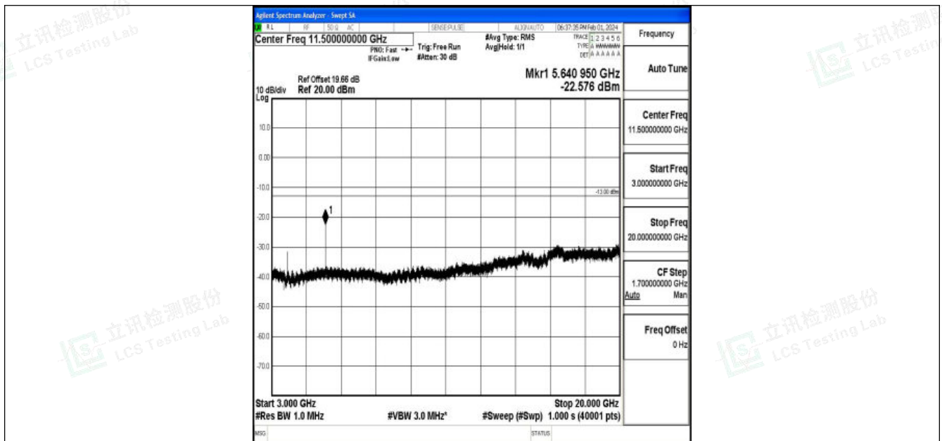
Band25_5MHz_QPSK_26365_1RB#0_3000~20000_3000~20000
