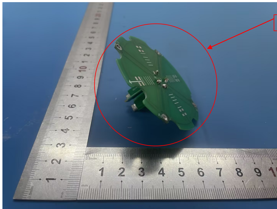
GNSS Antenna
