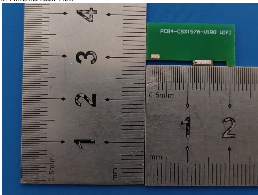
Wi-Fi&BT&BLE Antenna back view
