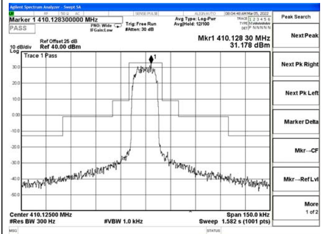
Channel 101 / 410.125 MHz
