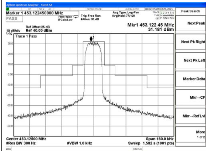
Channel 27 / 453.125 MHz
