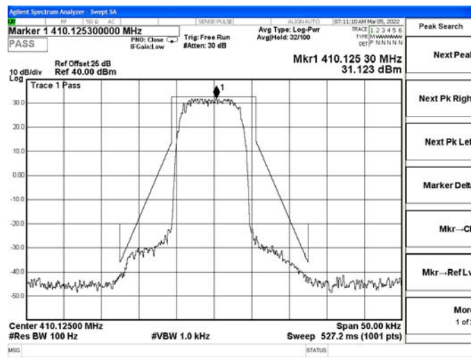
Channel 101 / 410.125 MHz
