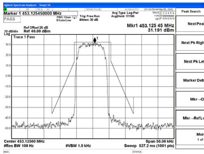
Channel 27 / 453.125 MHz
