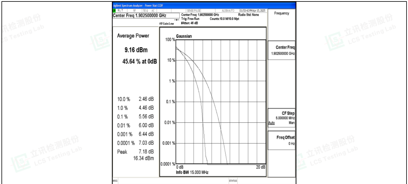
Band2-15MHz-QPSK-19125-75RB#0-PASS
