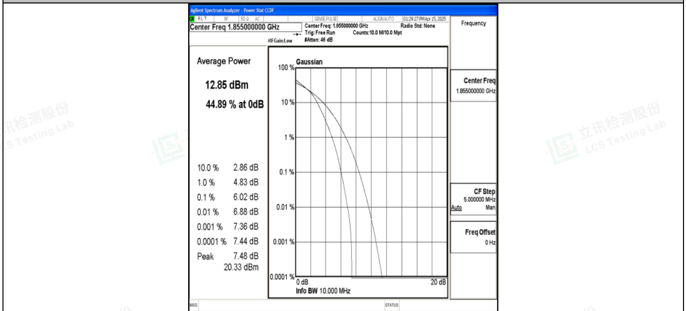
Band2-10MHz-16QAM-18650-50RB#0-PASS
