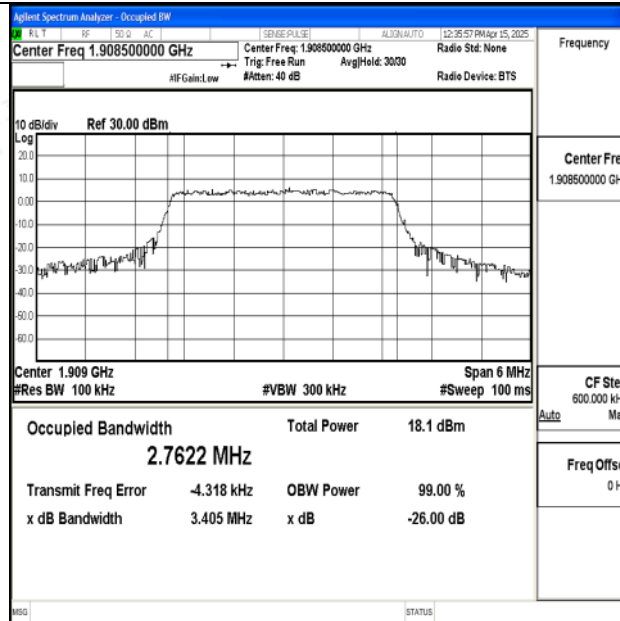
Band2-3MHz-QPSK-19185-15RB#0-PASS
