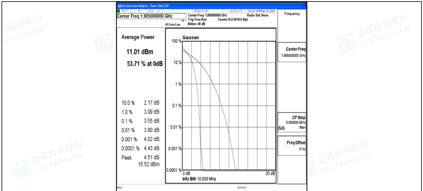
Band2-10MHz-QPSK-19150-1RB#0-PASS
