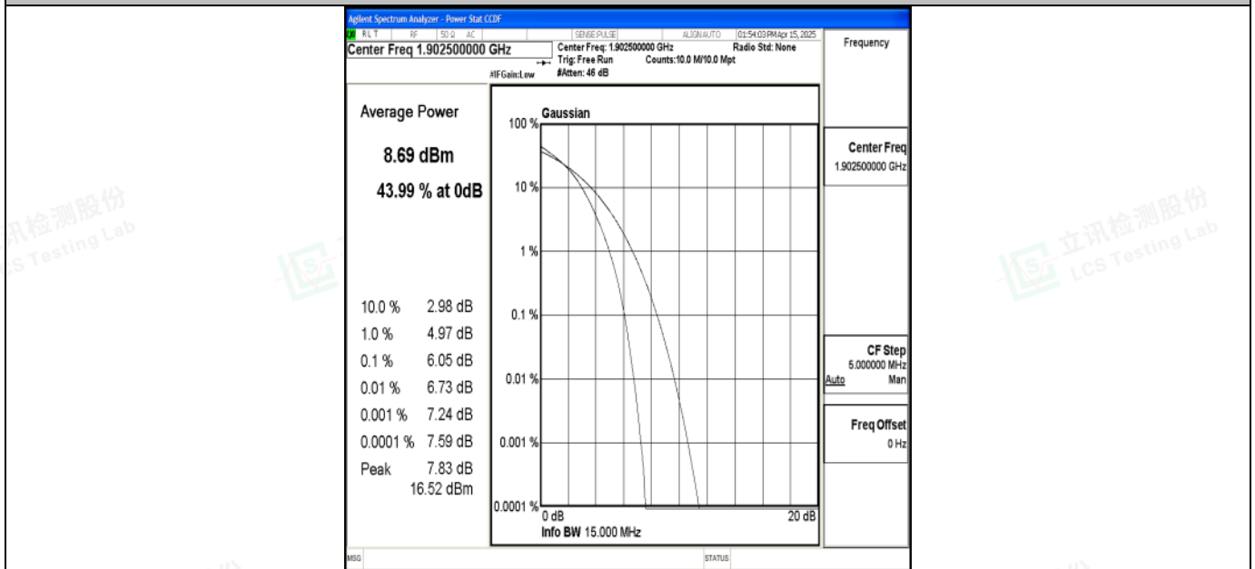
Band2-15MHz-16QAM-19125-75RB#0-PASS
