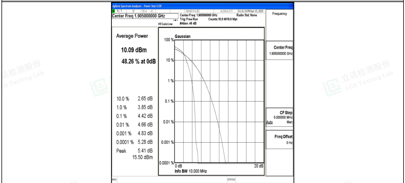
Band2-10MHz-16QAM-19150-1RB#0-PASS
