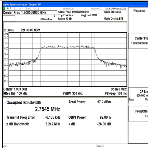
Band2-3MHz-16QAM-19185-15RB#0-PASS
