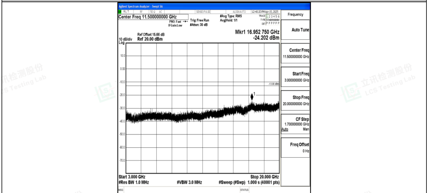
Band2_3MHz_16QAM_19185_1RB#0_3000~20000_3000~20000
