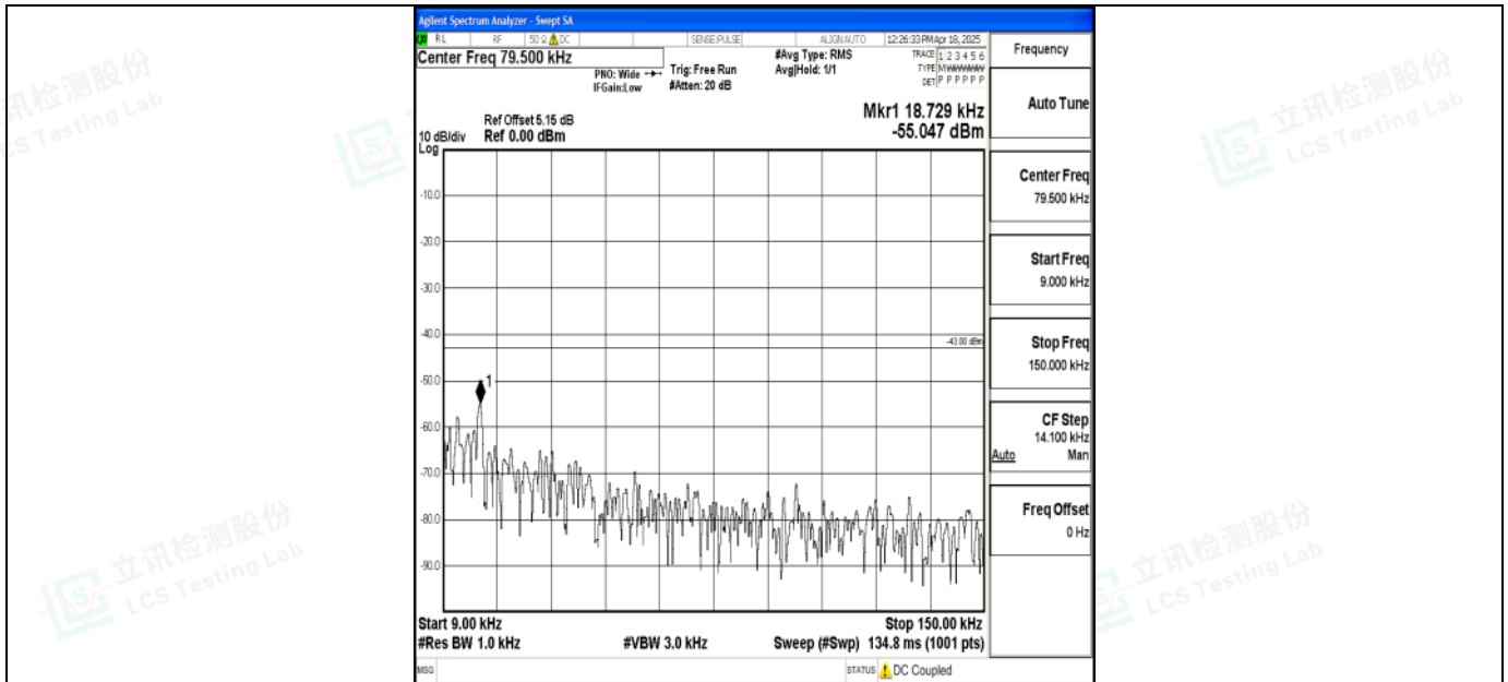
Band2_5MHz_QPSK_18625_1RB#0_0.009~0.15_0.009~0.15
