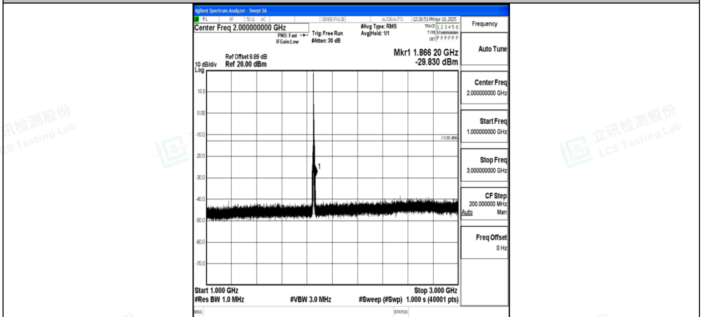
Band2_5MHz_QPSK_18625_1RB#0_1000~3000_1000~3000
