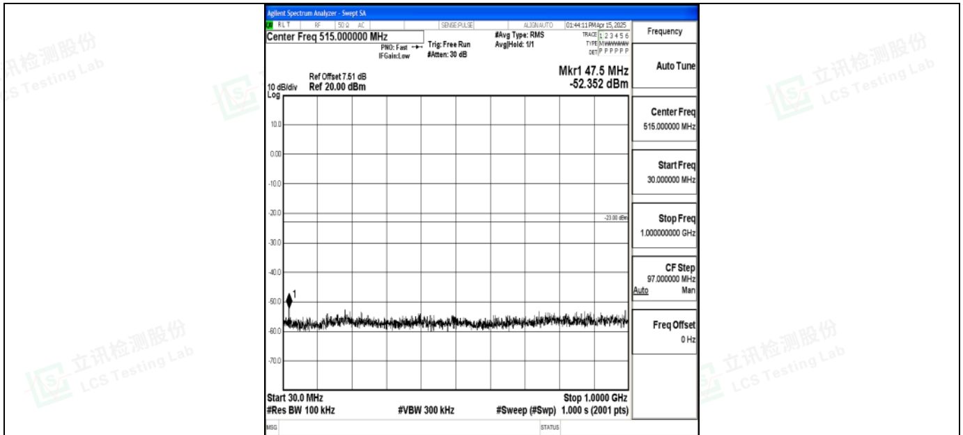
Band2_15MHz_QPSK_18900_1RB#0_30~1000_30~1000
