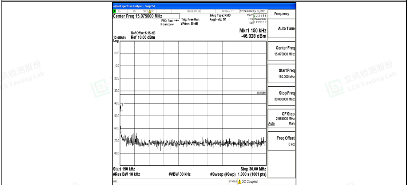
Band2_5MHz_16QAM_19175_1RB#0_0.15~30_0.15~30
