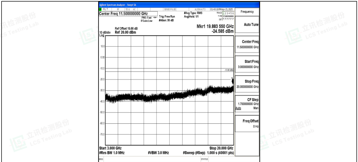
Band2_15MHz_QPSK_18675_1RB#0_3000~20000_3000~20000
