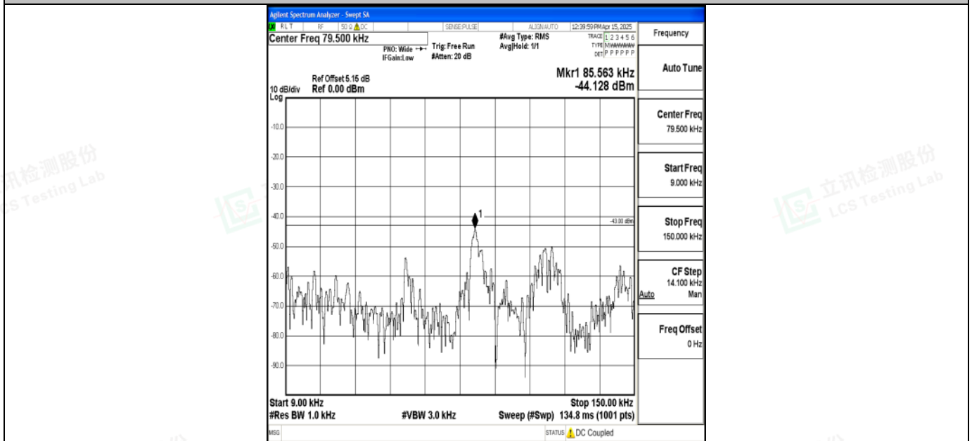
Band2_3MHz_16QAM_19185_1RB#0_0.009~0.15_0.009~0.15
