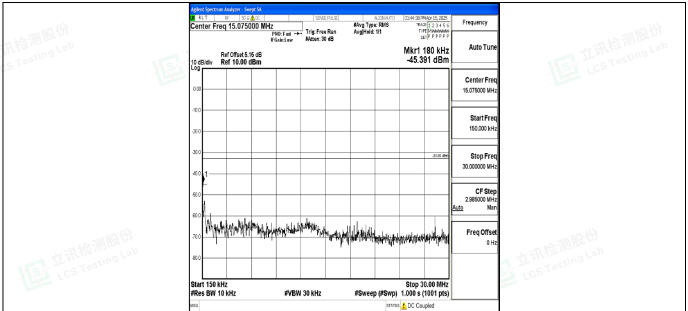
Band2_15MHz_16QAM_18900_1RB#0_0.15~30_0.15~30
