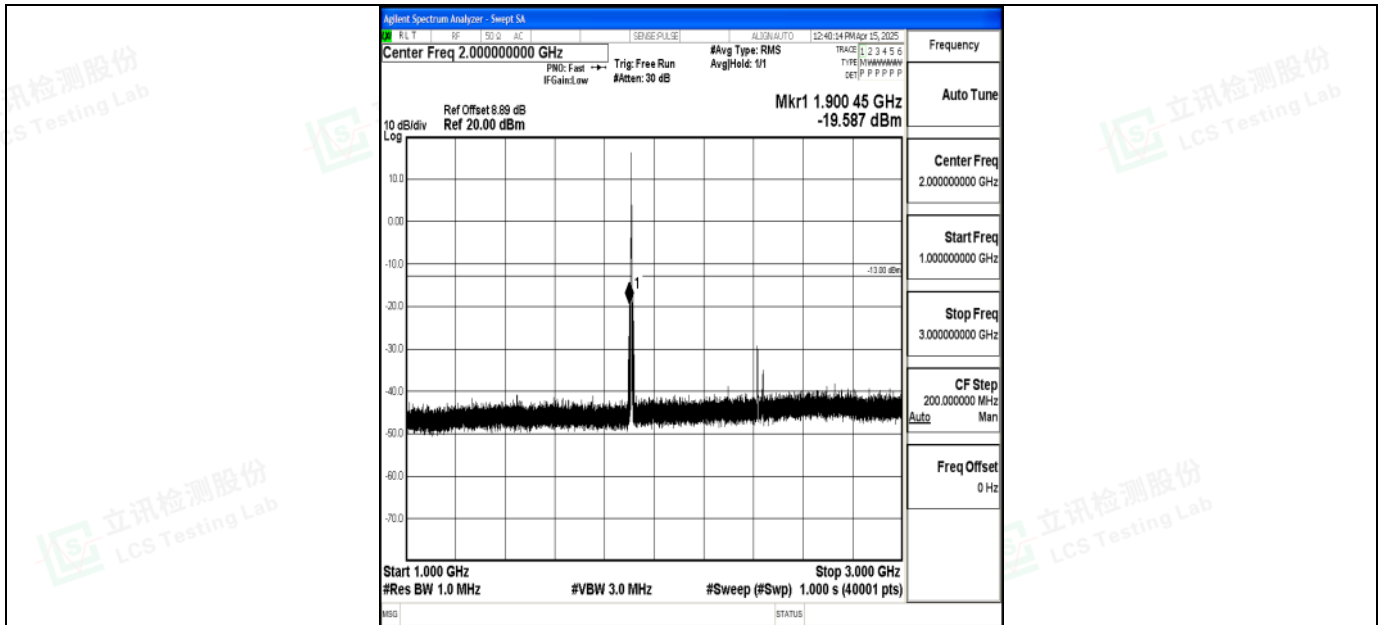
Band2_3MHz_16QAM_19185_1RB#0_1000~3000_1000~3000
