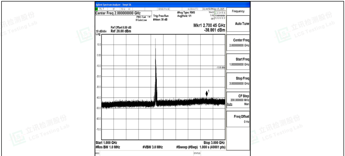
Band2_15MHz_16QAM_18900_1RB#0_1000~3000_1000~3000
