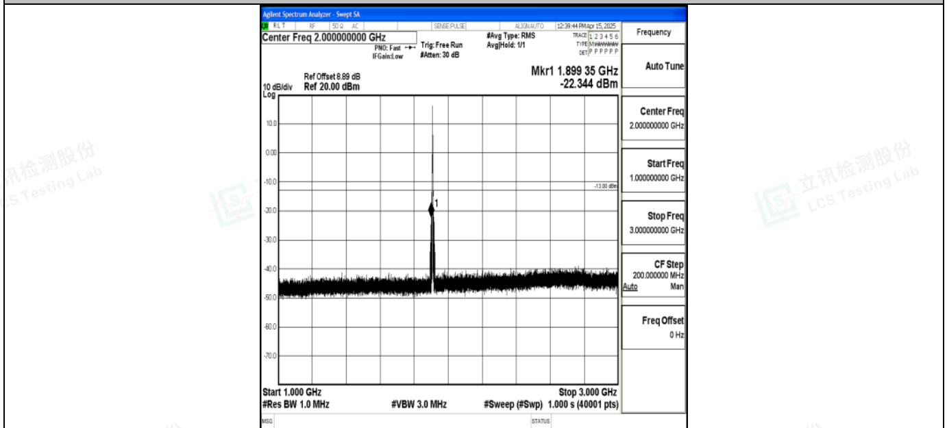
Band2_3MHz_QPSK_19185_1RB#0_1000~3000_1000~3000
