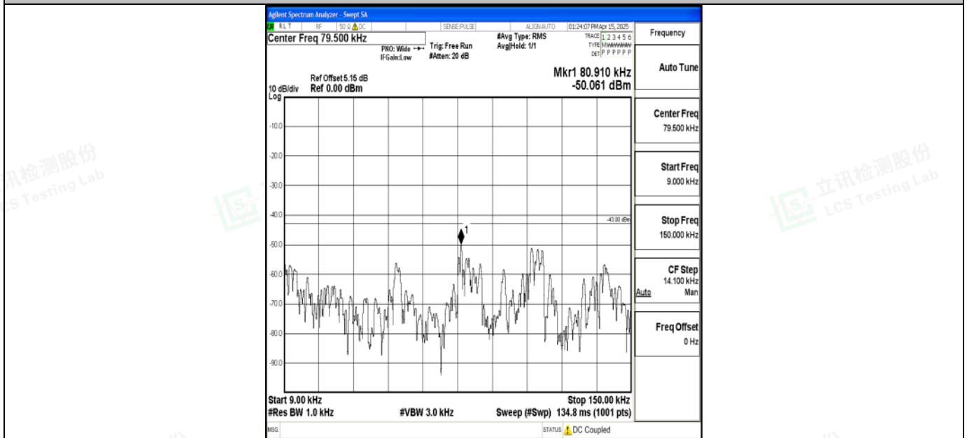
Band2_10MHz_16QAM_19150_1RB#0_0.009~0.15_0.009~0.15
