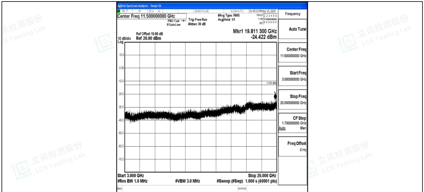
Band2_15MHz_QPSK_19125_1RB#0_3000~20000_3000~20000
