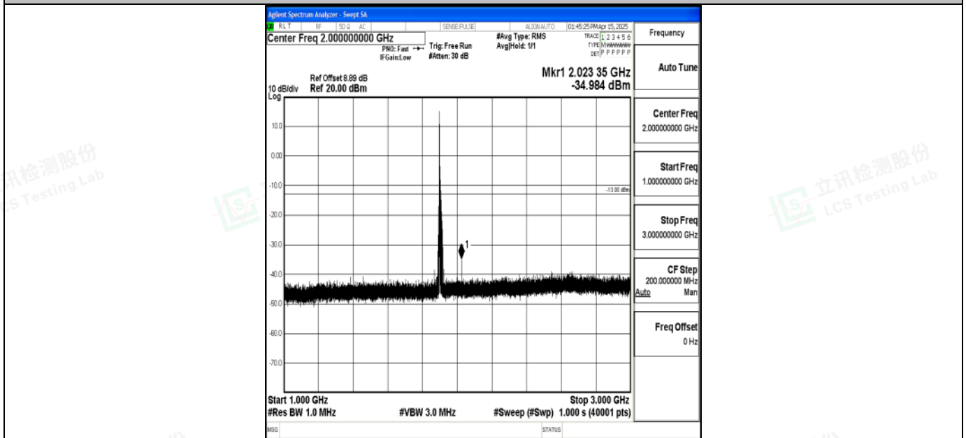
Band2_15MHz_QPSK_19125_1RB#0_1000~3000_1000~3000
