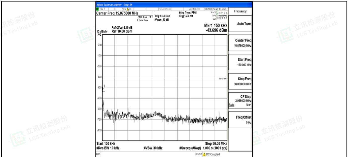
Band2_10MHz_16QAM_18900_1RB#0_0.15~30_0.15~30
