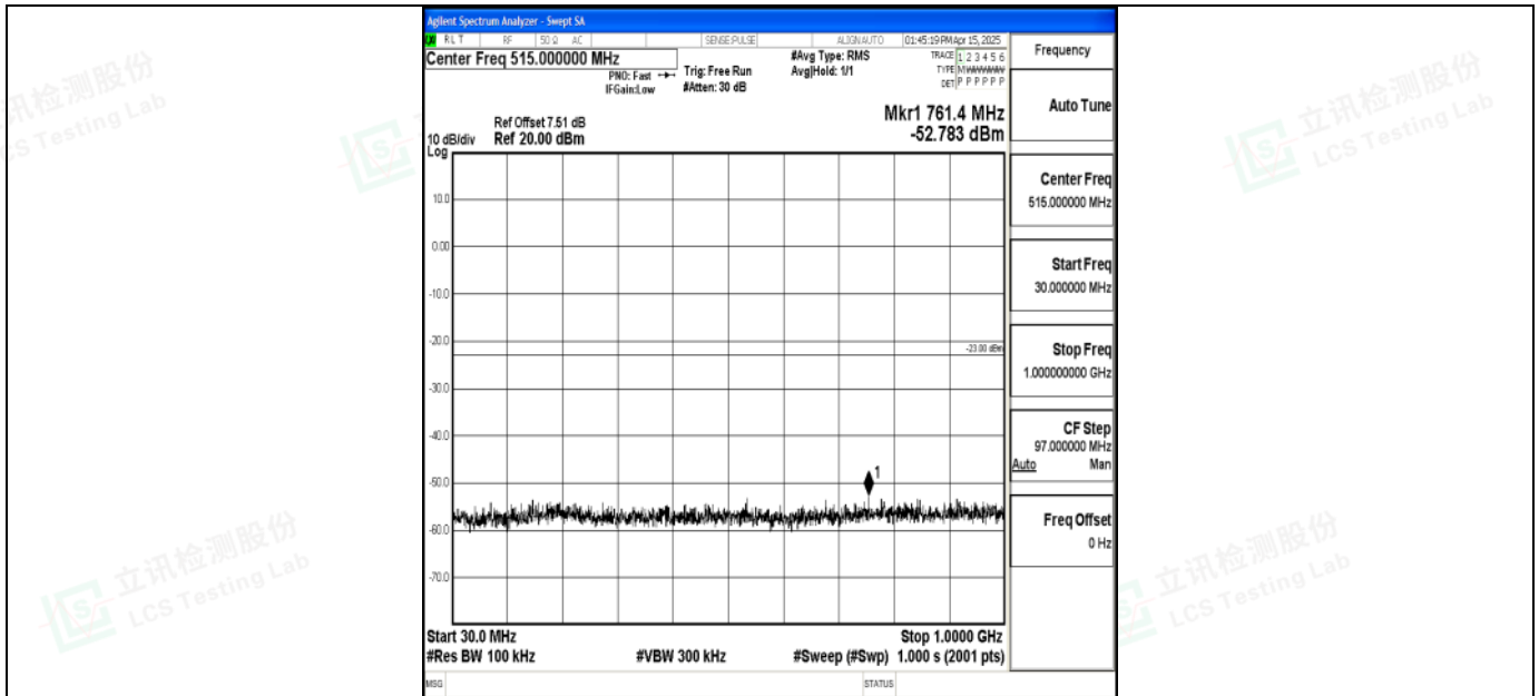
Band2_15MHz_QPSK_19125_1RB#0_30~1000_30~1000
