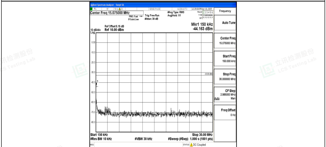
Band2_5MHz_QPSK_19175_1RB#0_0.15~30_0.15~30
