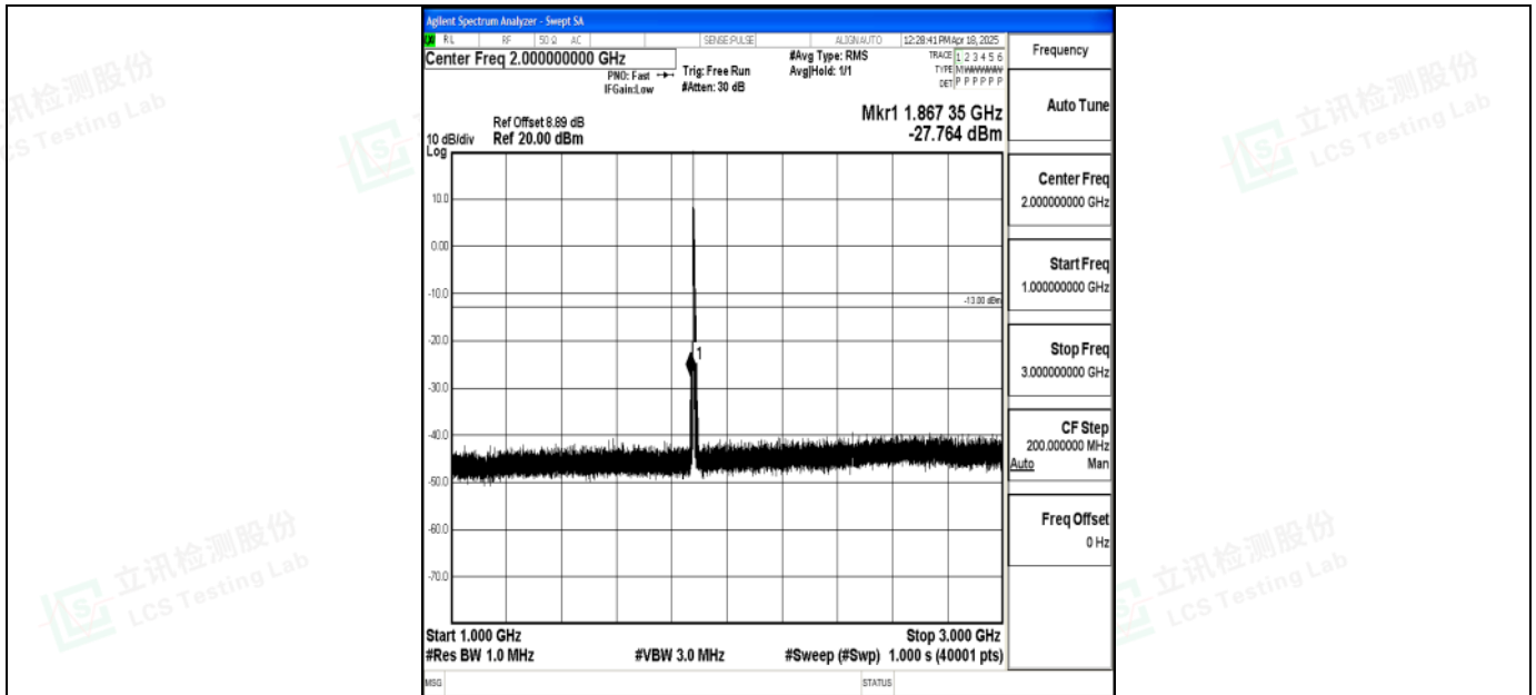
Band2_5MHz_16QAM_18900_1RB#0_1000~3000_1000~3000
