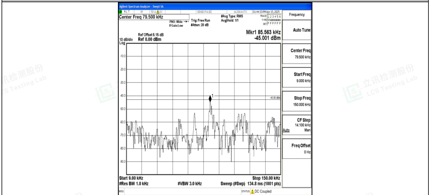
Band2_15MHz_16QAM_18900_1RB#0_0.009~0.15_0.009~0.15
