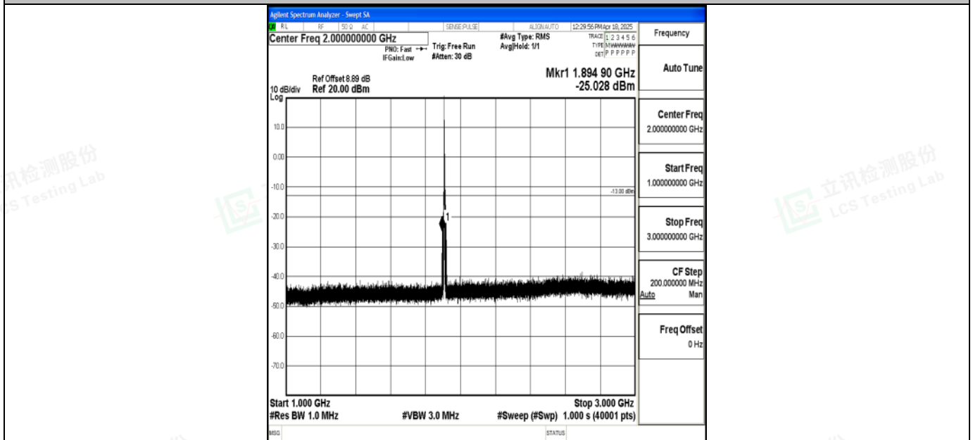
Band2_5MHz_16QAM_19175_1RB#0_1000~3000_1000~3000
