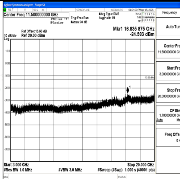
Band2_10MHz_16QAM_19150_1RB#0_3000~20000_3000~20000
