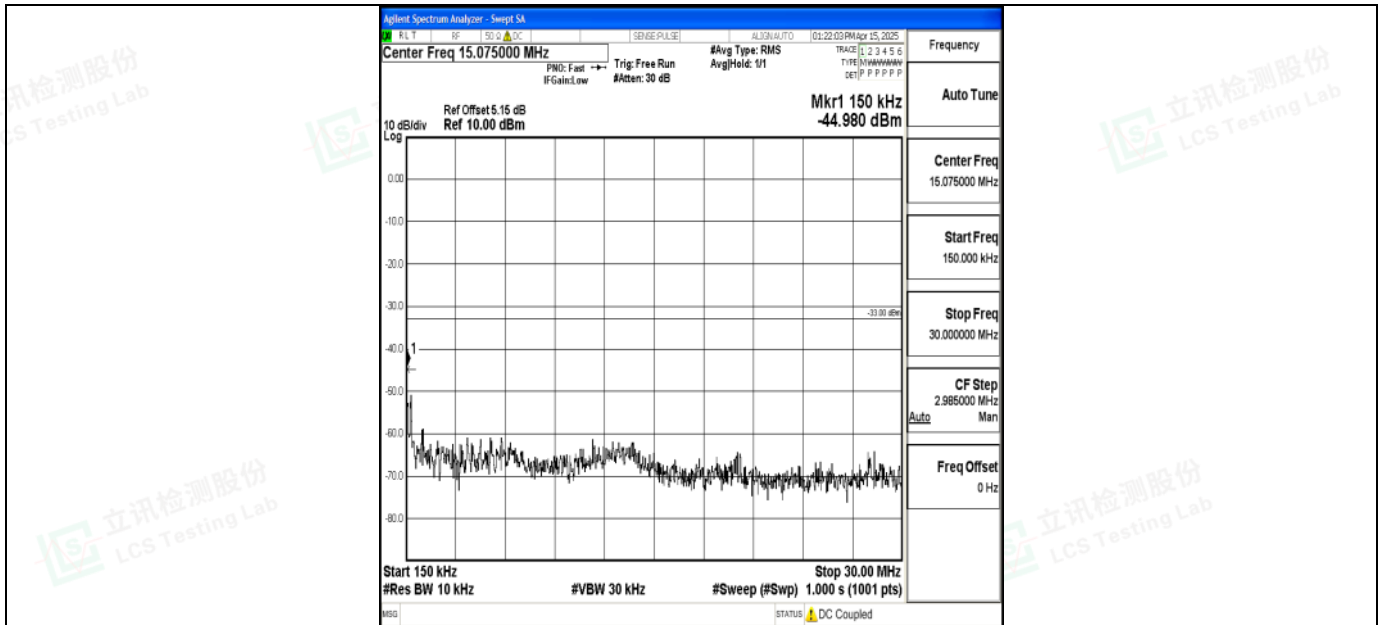
Band2_10MHz_16QAM_18650_1RB#0_0.15~30_0.15~30
