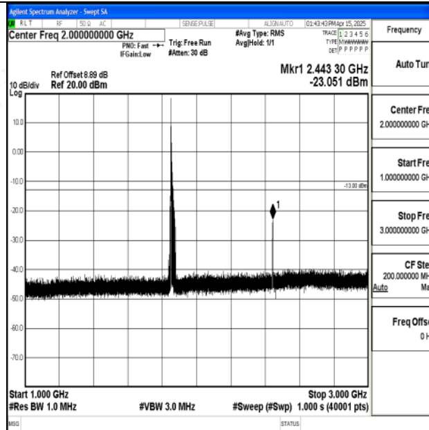
Band2_15MHz_16QAM_18675_1RB#0_1000~3000_1000~3000
