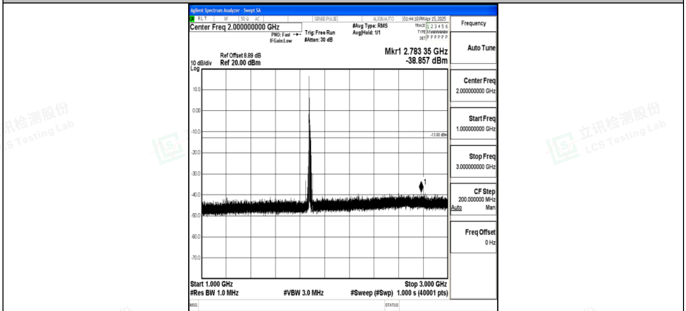
Band2_15MHz_QPSK_18900_1RB#0_1000~3000_1000~3000
