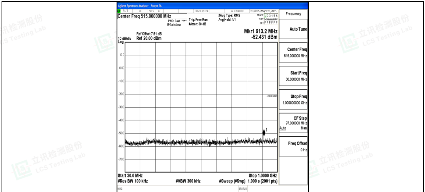
Band2_15MHz_QPSK_18675_1RB#0_30~1000_30~1000
