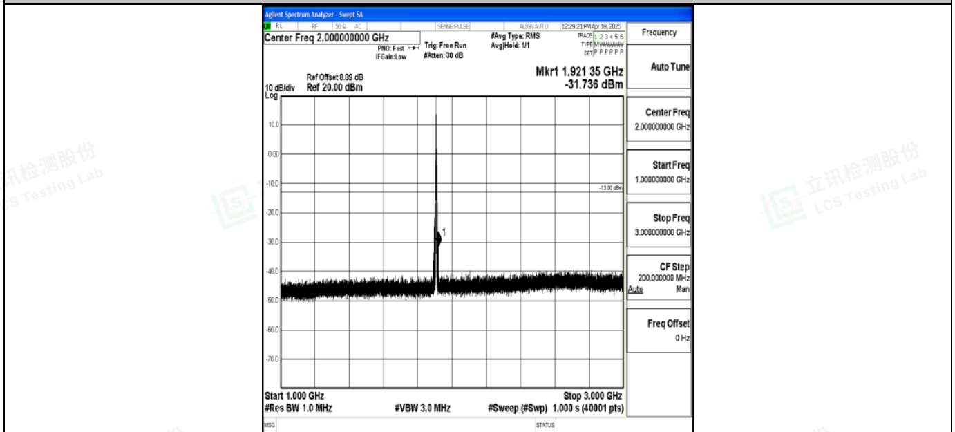
Band2_5MHz_QPSK_19175_1RB#0_1000~3000_1000~3000
