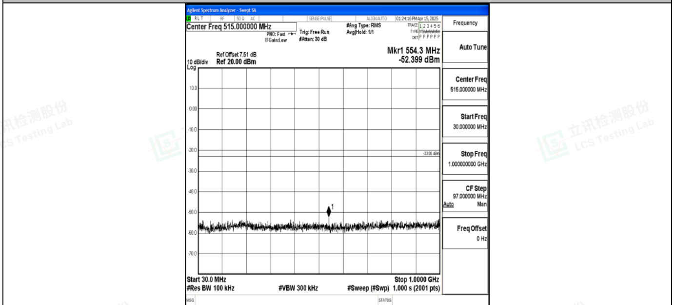
Band2_10MHz_16QAM_19150_1RB#0_30~1000_30~1000
