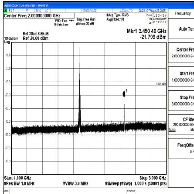
Band2_10MHz_16QAM_18900_1RB#0_1000~3000_1000~3000
