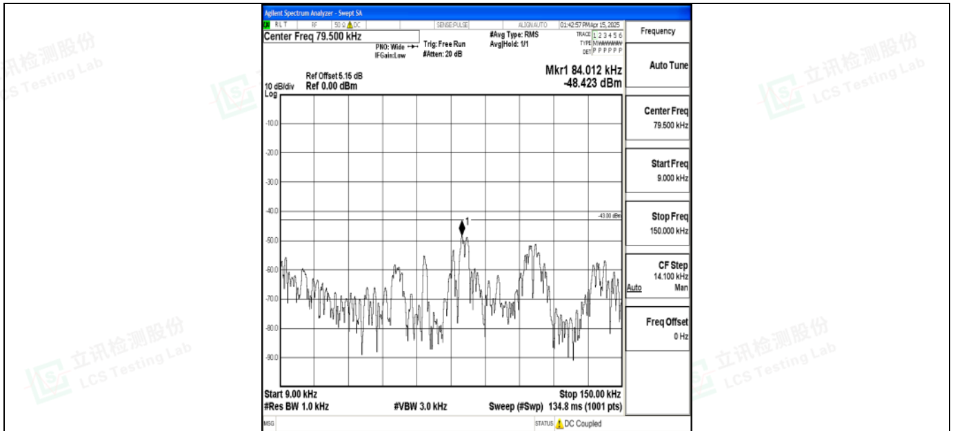
Band2_15MHz_QPSK_18675_1RB#0_0.009~0.15_0.009~0.15
