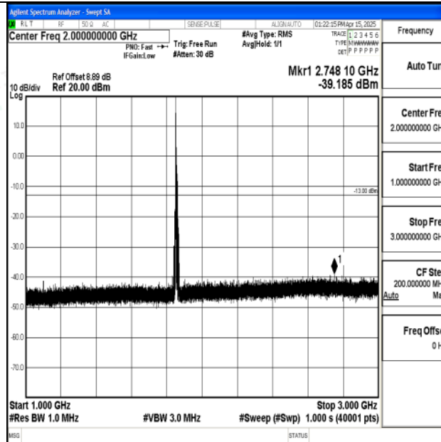
Band2_10MHz_16QAM_18650_1RB#0_1000~3000_1000~3000
