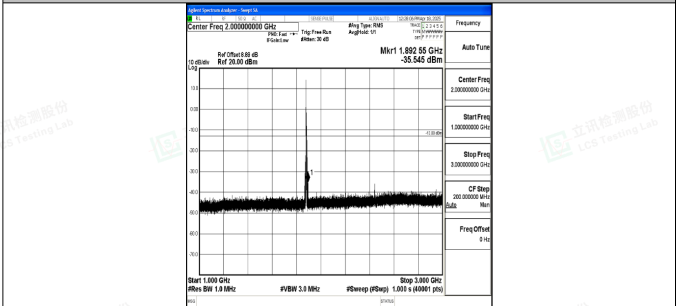
Band2_5MHz_QPSK_18900_1RB#0_1000~3000_1000~3000
