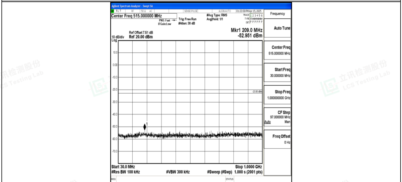
Band2_10MHz_16QAM_18650_1RB#0_30~1000_30~1000
