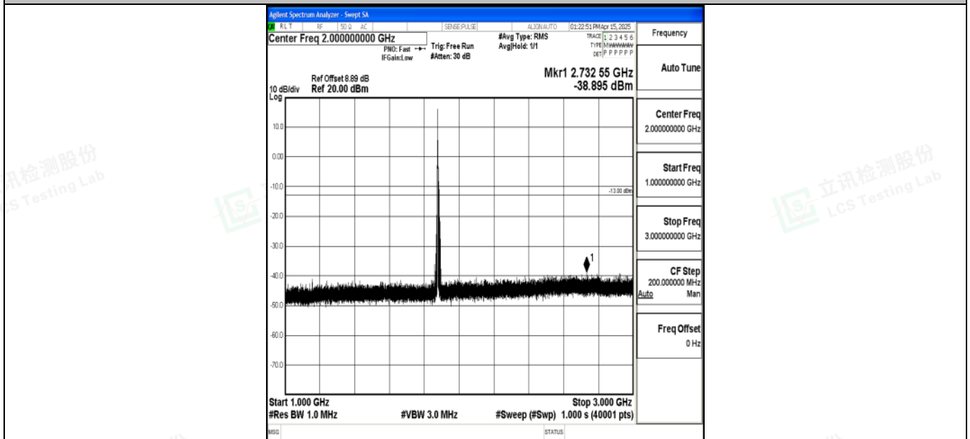
Band2_10MHz_QPSK_18900_1RB#0_1000~3000_1000~3000
