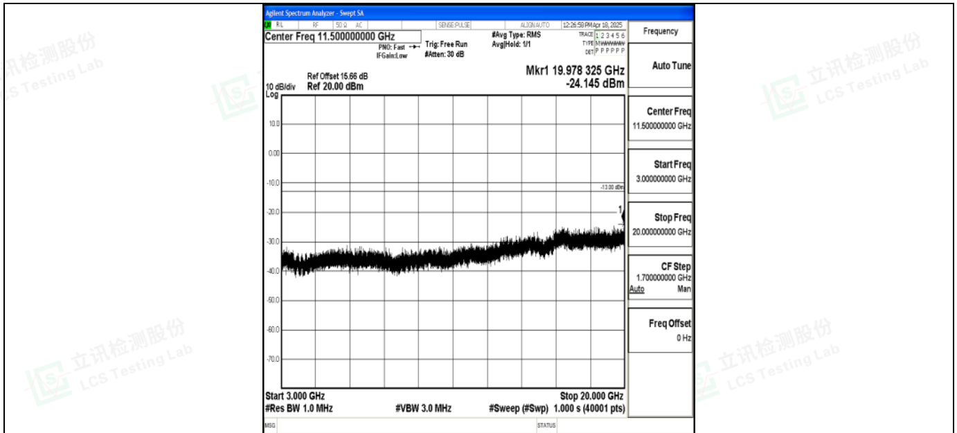
Band2_5MHz_QPSK_18625_1RB#0_3000~20000_3000~20000
