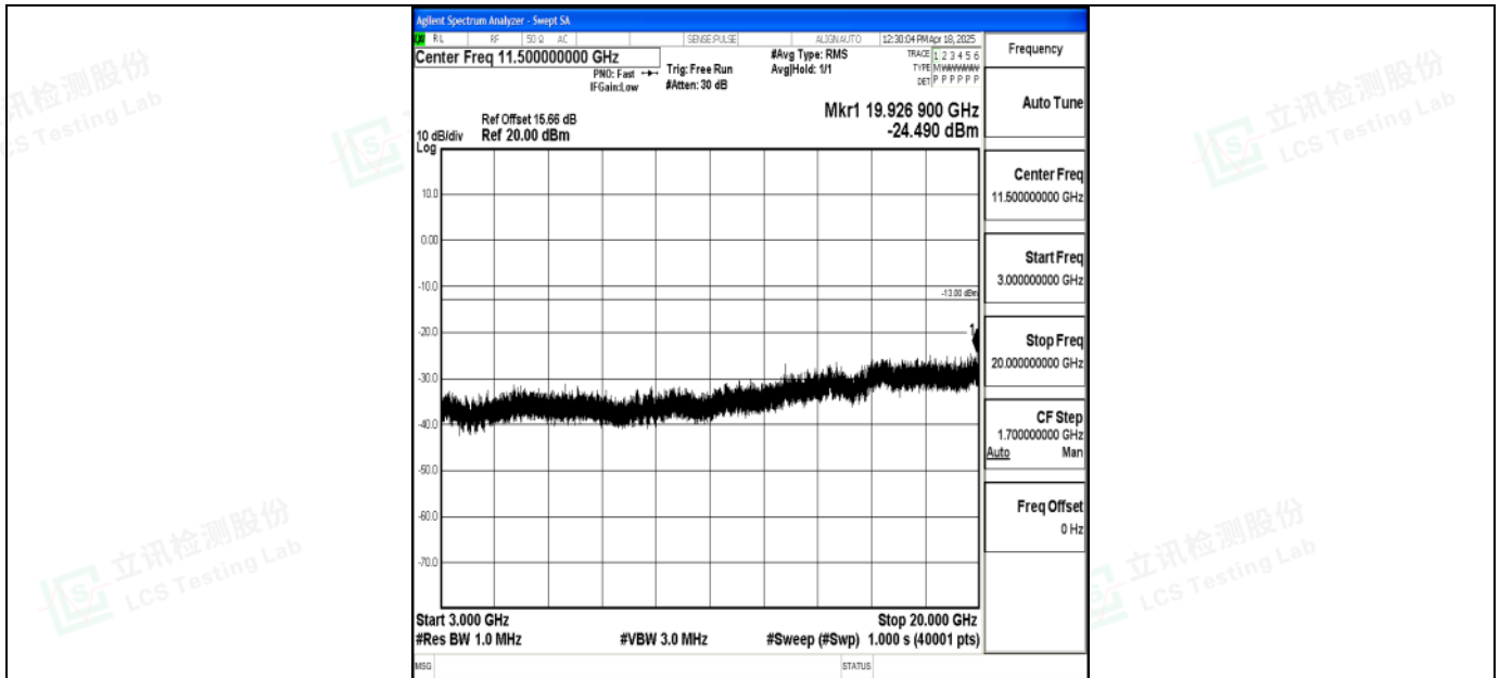
Band2_5MHz_16QAM_19175_1RB#0_3000~20000_3000~20000
