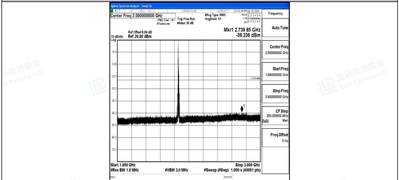
Band2_10MHz_QPSK_18650_1RB#0_1000~3000_1000~3000
