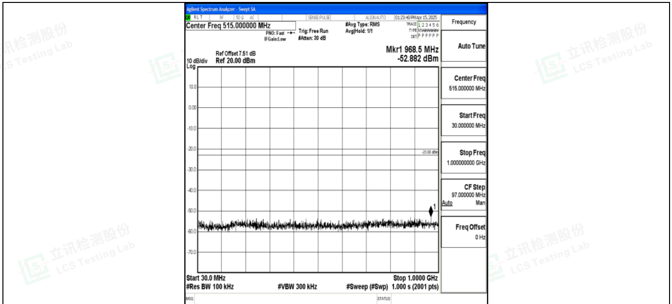
Band2_10MHz_QPSK_19150_1RB#0_30~1000_30~1000
