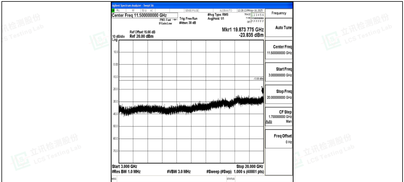
Band2_5MHz_QPSK_18900_1RB#0_3000~20000_3000~20000
