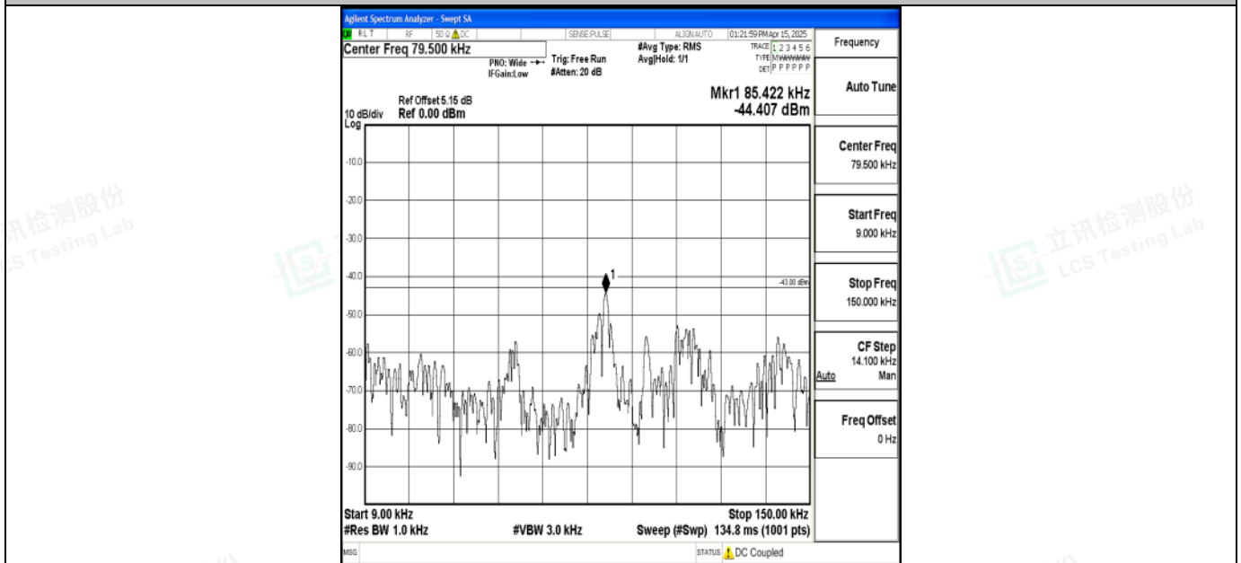
Band2_10MHz_16QAM_18650_1RB#0_0.009~0.15_0.009~0.15
