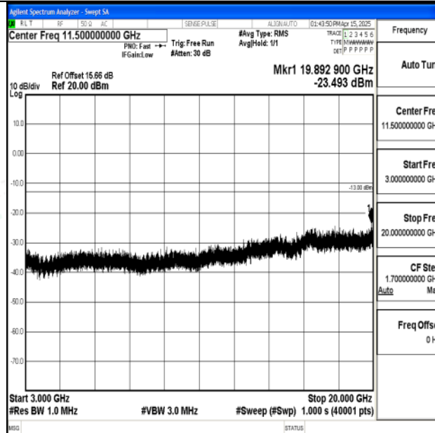
Band2_15MHz_16QAM_18675_1RB#0_3000~20000_3000~20000
