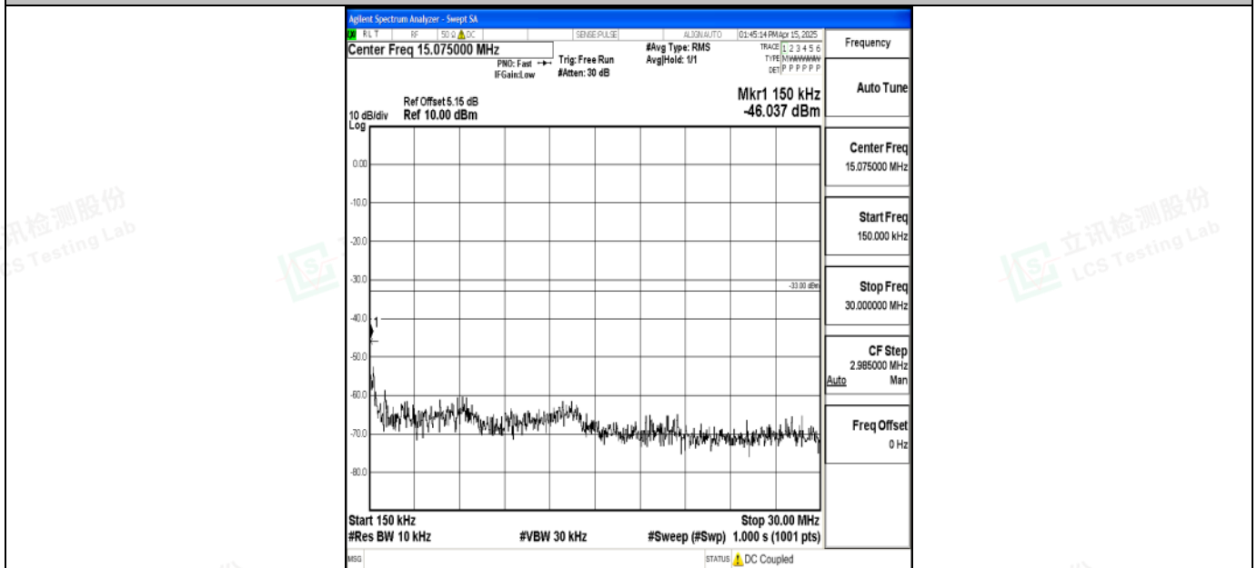
Band2_15MHz_QPSK_19125_1RB#0_0.15~30_0.15~30
