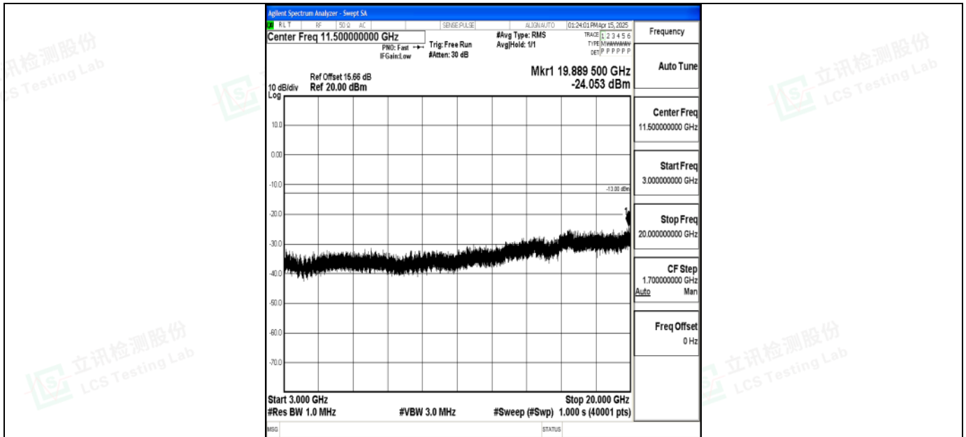
Band2_10MHz_QPSK_19150_1RB#0_3000~20000_3000~20000
