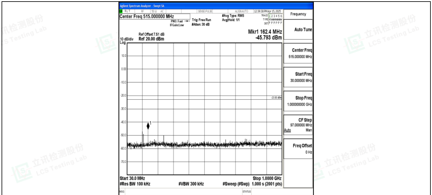
Band2_3MHz_QPSK_19185_1RB#0_30~1000_30~1000
