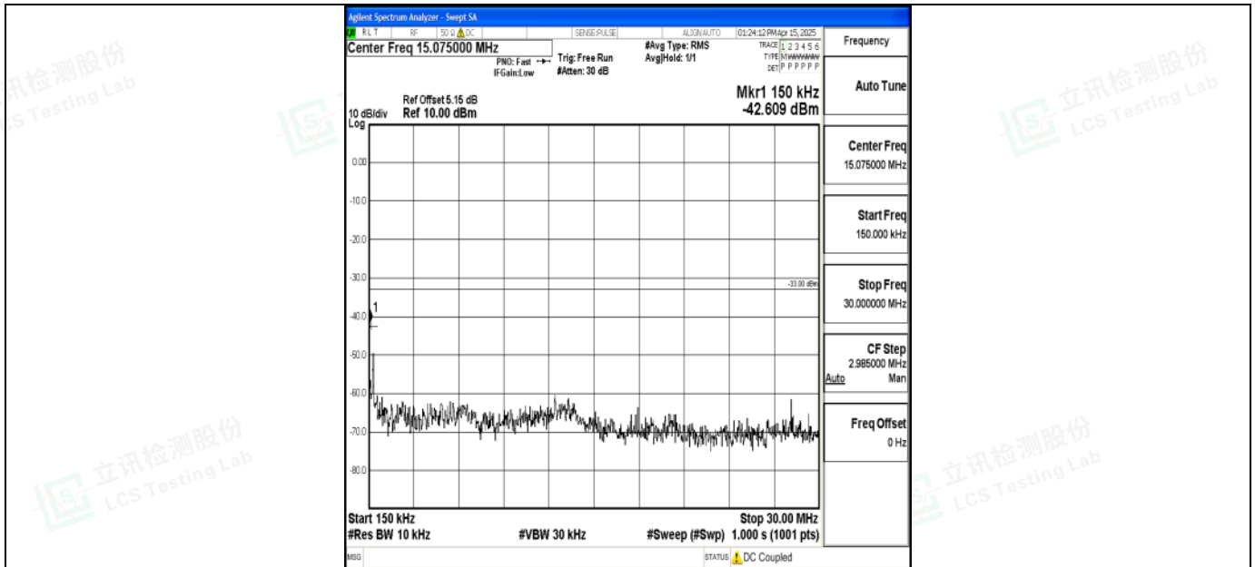
Band2_10MHz_16QAM_19150_1RB#0_0.15~30_0.15~30
