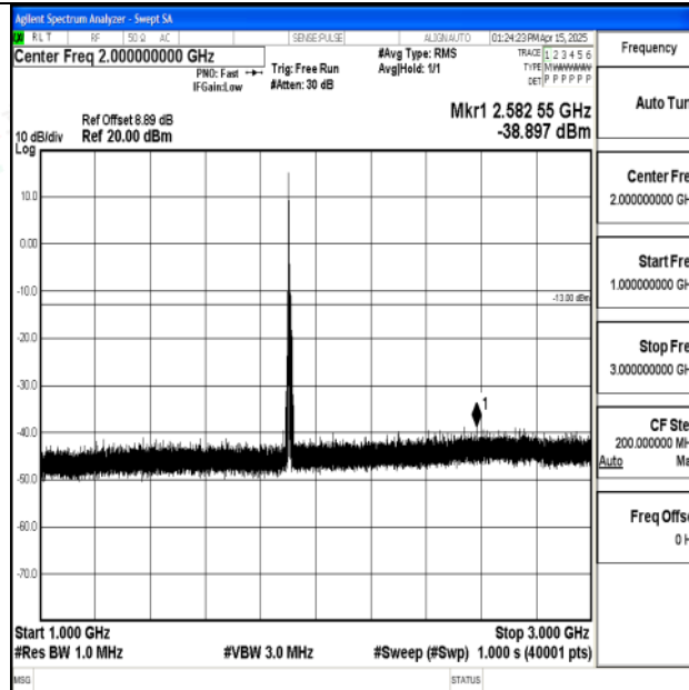
Band2_10MHz_16QAM_19150_1RB#0_1000~3000_1000~3000
