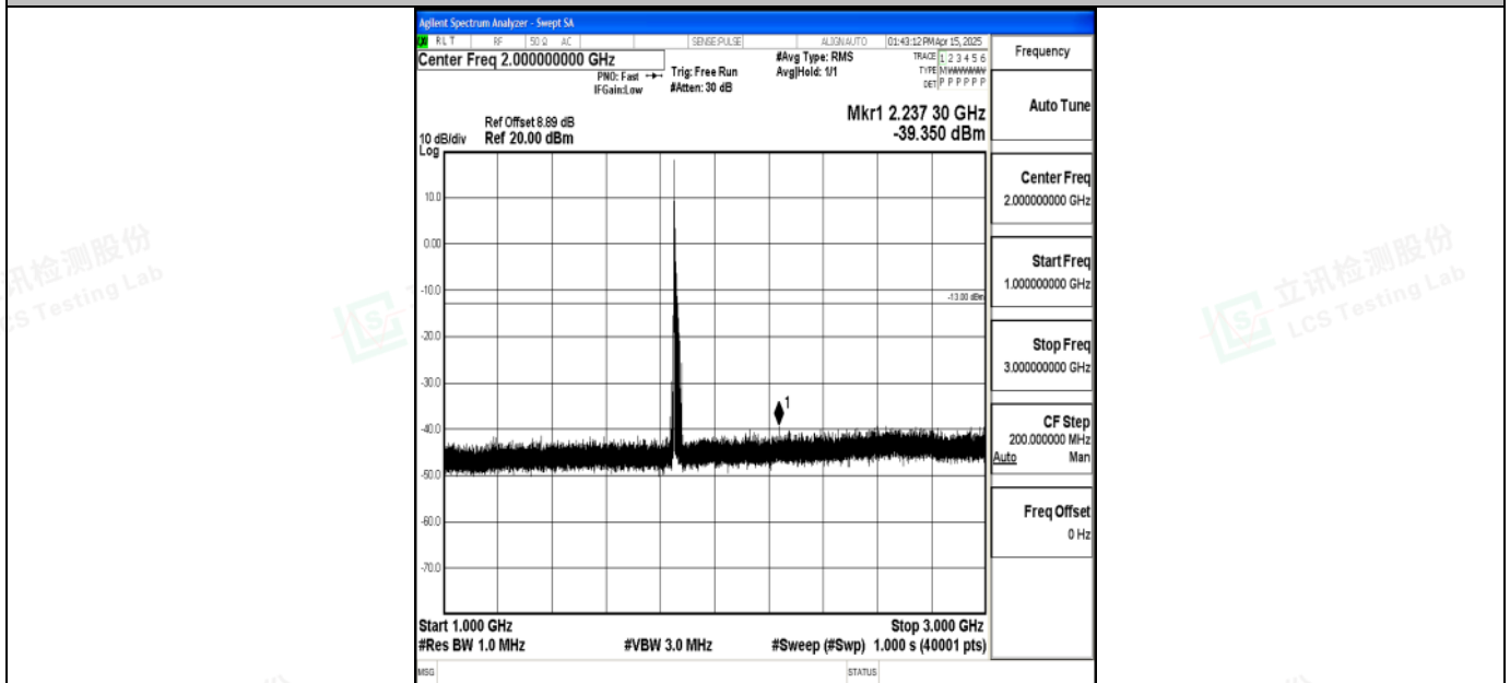
Band2_15MHz_QPSK_18675_1RB#0_1000~3000_1000~3000
