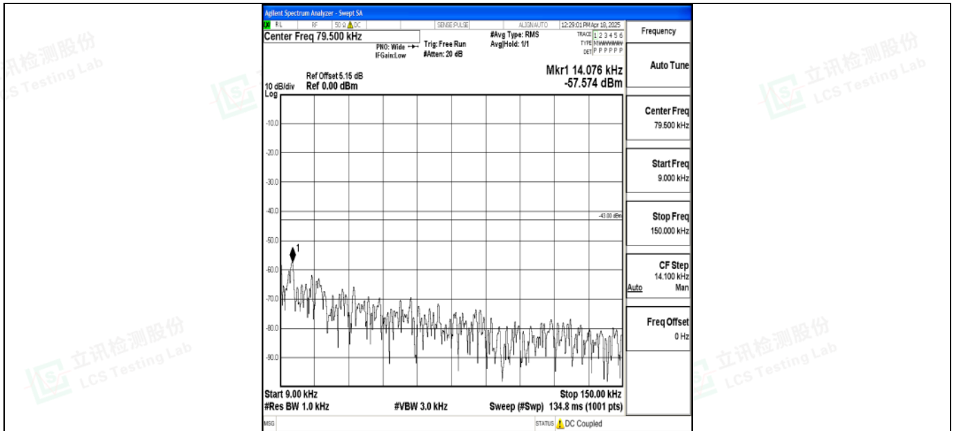
Band2_5MHz_QPSK_19175_1RB#0_0.009~0.15_0.009~0.15
