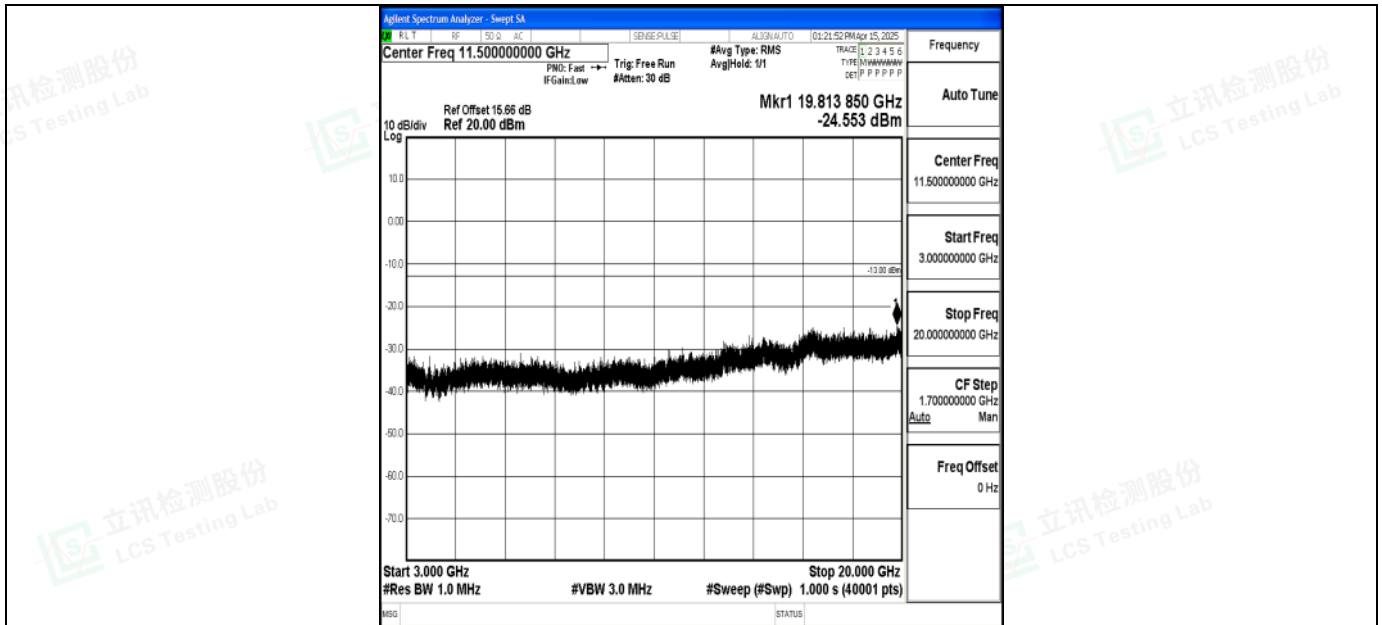
Band2_10MHz_QPSK_18650_1RB#0_3000~20000_3000~20000
