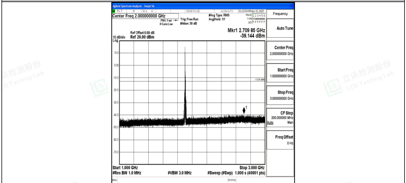
Band2_10MHz_QPSK_19150_1RB#0_1000~3000_1000~3000
