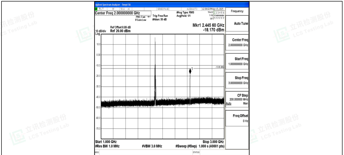
Band2_3MHz_16QAM_18900_1RB#0_1000~3000_1000~3000
