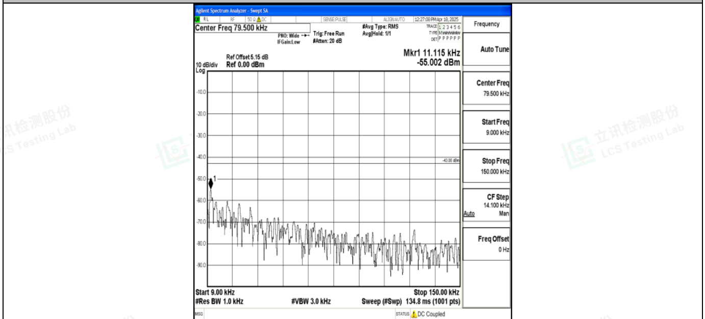
Band2_5MHz_16QAM_18625_1RB#0_0.009~0.15_0.009~0.15
