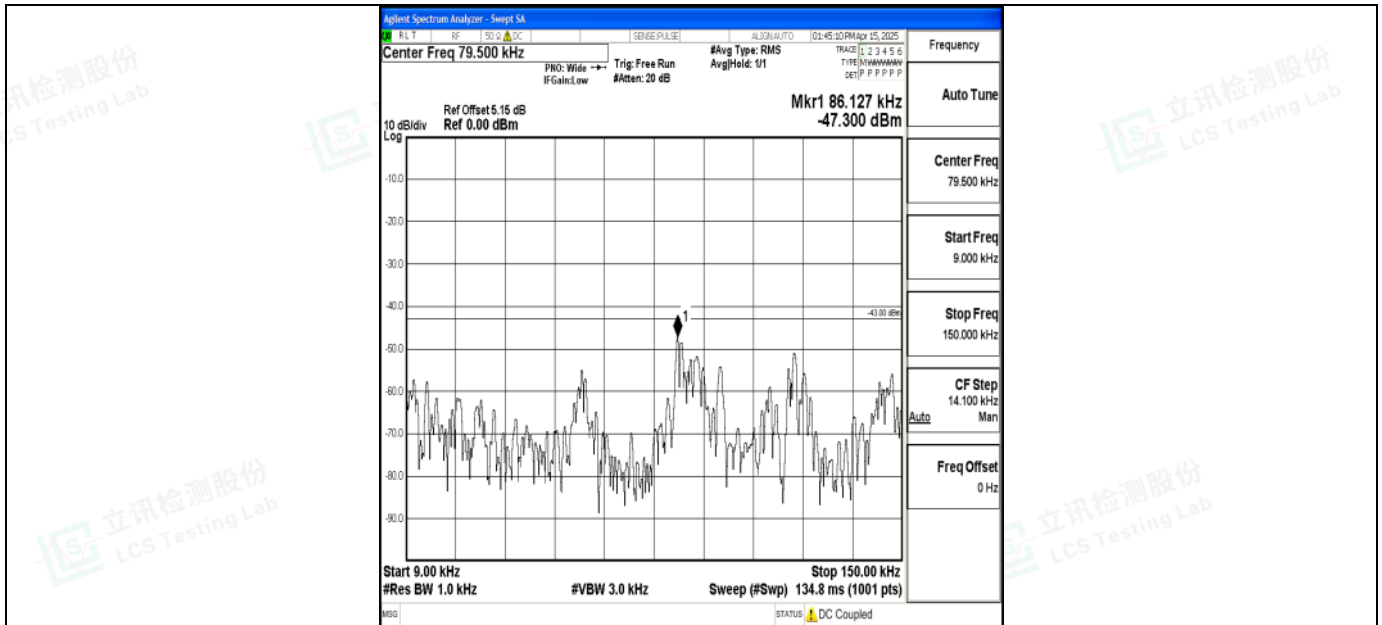
Band2_15MHz_QPSK_19125_1RB#0_0.009~0.15_0.009~0.15
