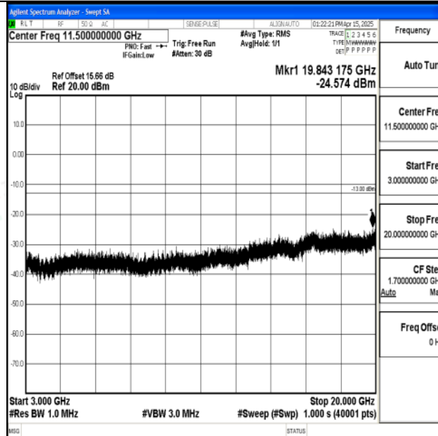
Band2_10MHz_16QAM_18650_1RB#0_3000~20000_3000~20000
