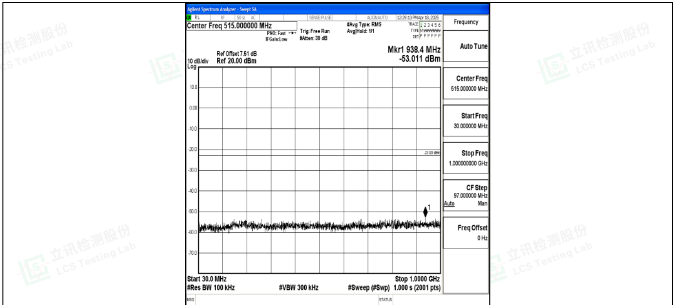
Band2_5MHz_QPSK_19175_1RB#0_30~1000_30~1000
