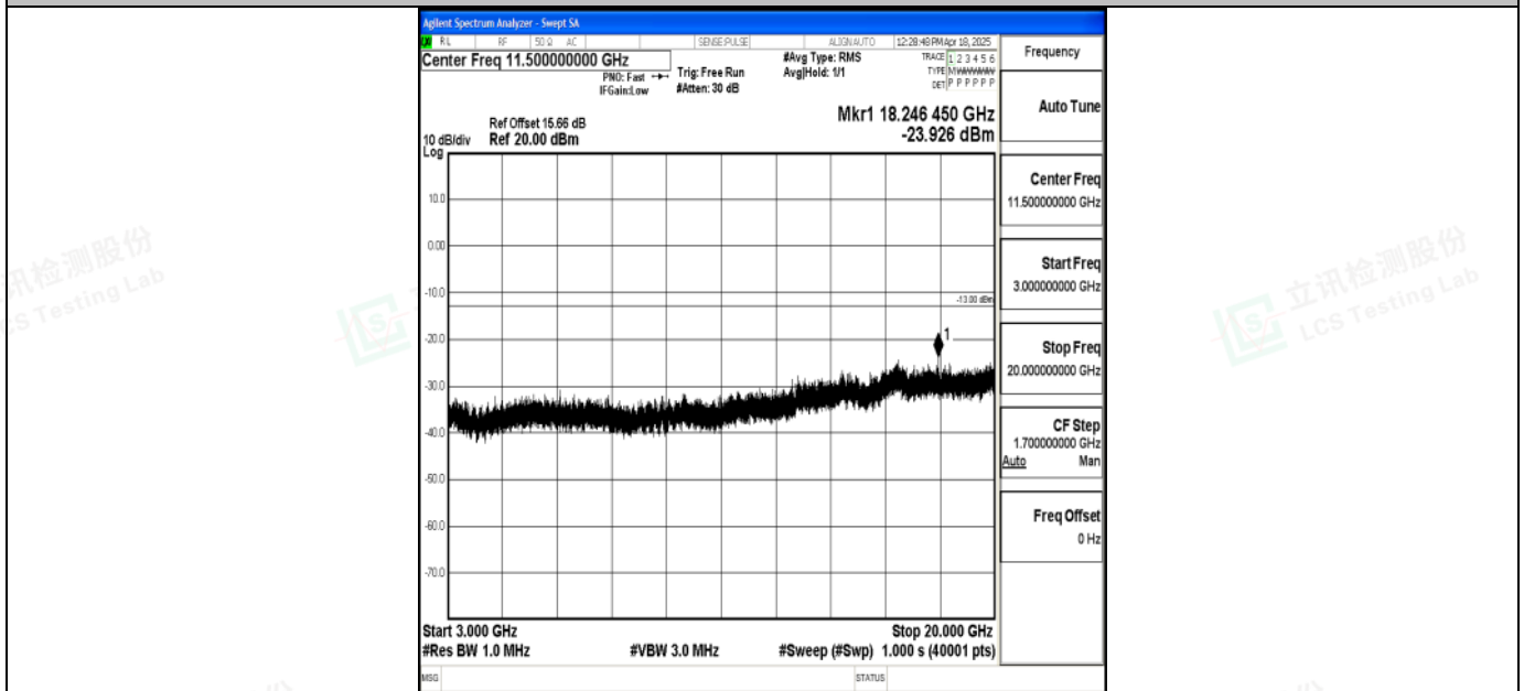
Band2_5MHz_16QAM_18900_1RB#0_3000~20000_3000~20000
