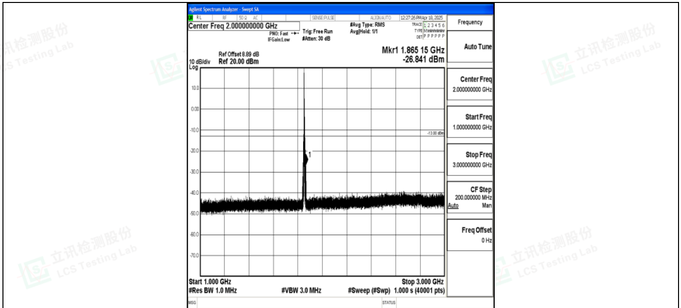
Band2_5MHz_16QAM_18625_1RB#0_1000~3000_1000~3000
