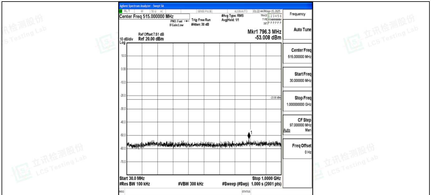
Band2_10MHz_QPSK_18900_1RB#0_30~1000_30~1000
