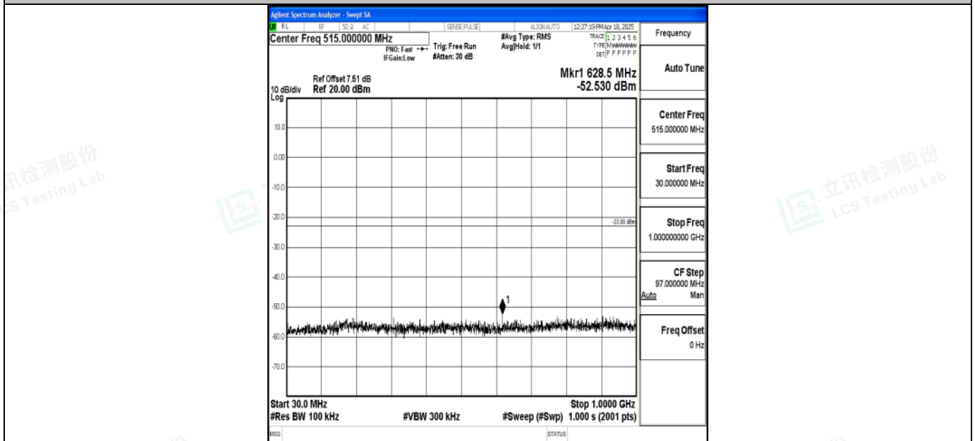
Band2_5MHz_16QAM_18625_1RB#0_30~1000_30~1000
