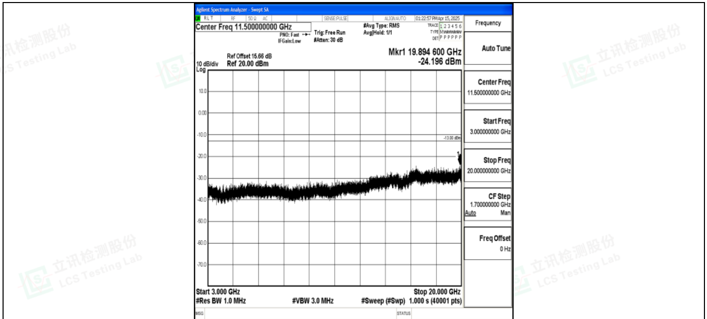
Band2_10MHz_QPSK_18900_1RB#0_3000~20000_3000~20000
