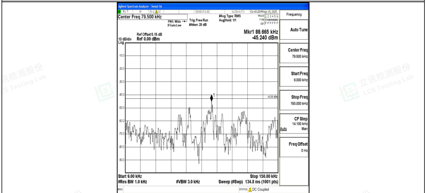
Band2_15MHz_16QAM_18675_1RB#0_0.009~0.15_0.009~0.15
