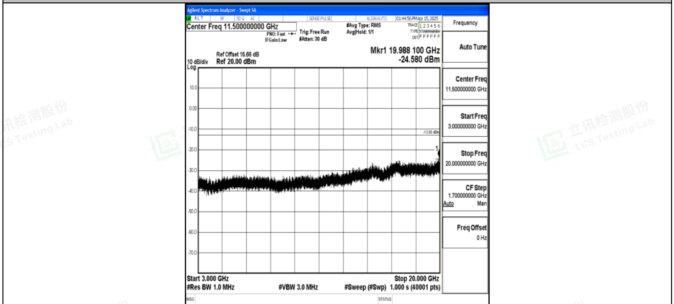
Band2_15MHz_16QAM_18900_1RB#0_3000~20000_3000~20000
