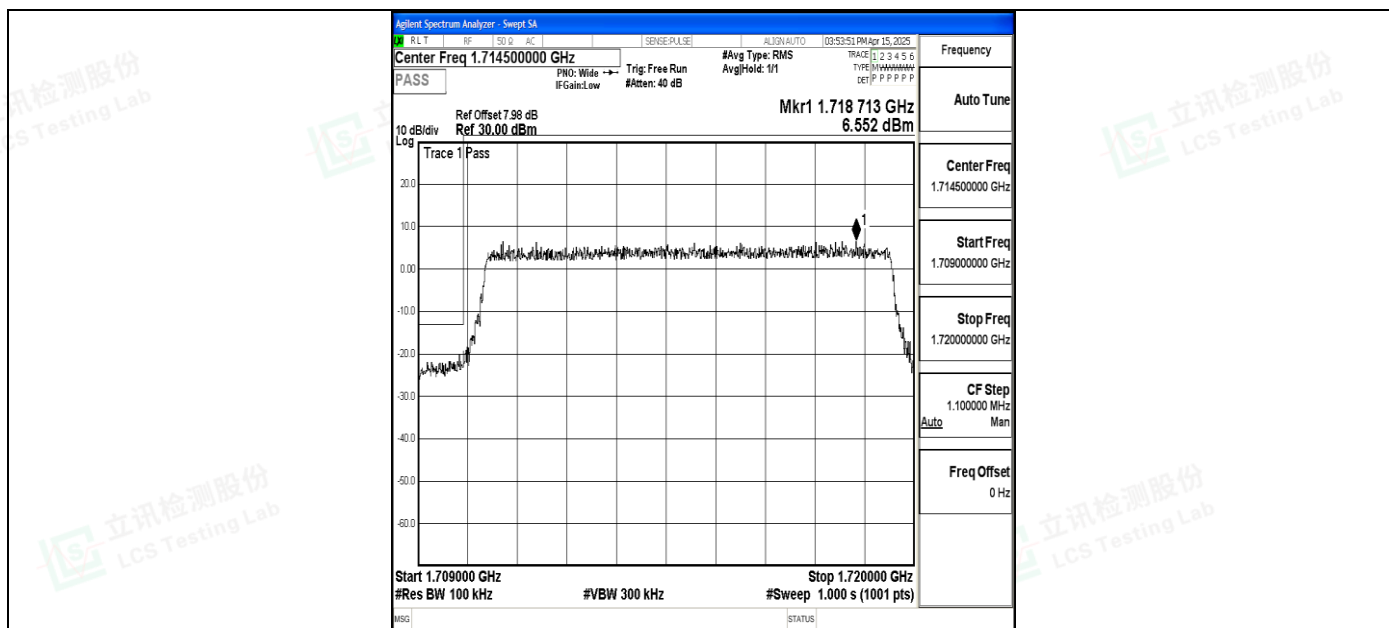
Band4_10MHz_QPSK_20000_50RB#0
