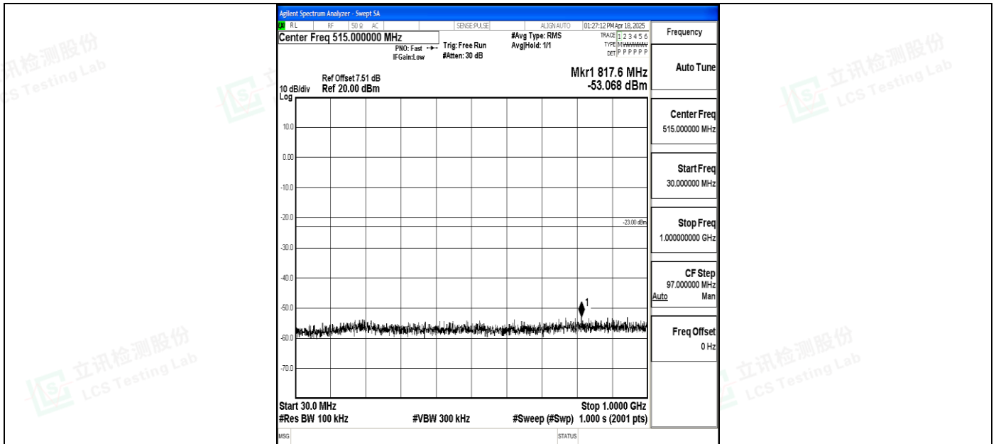
Band4_3MHz_QPSK_20385_1RB#0_30~1000_30~1000
