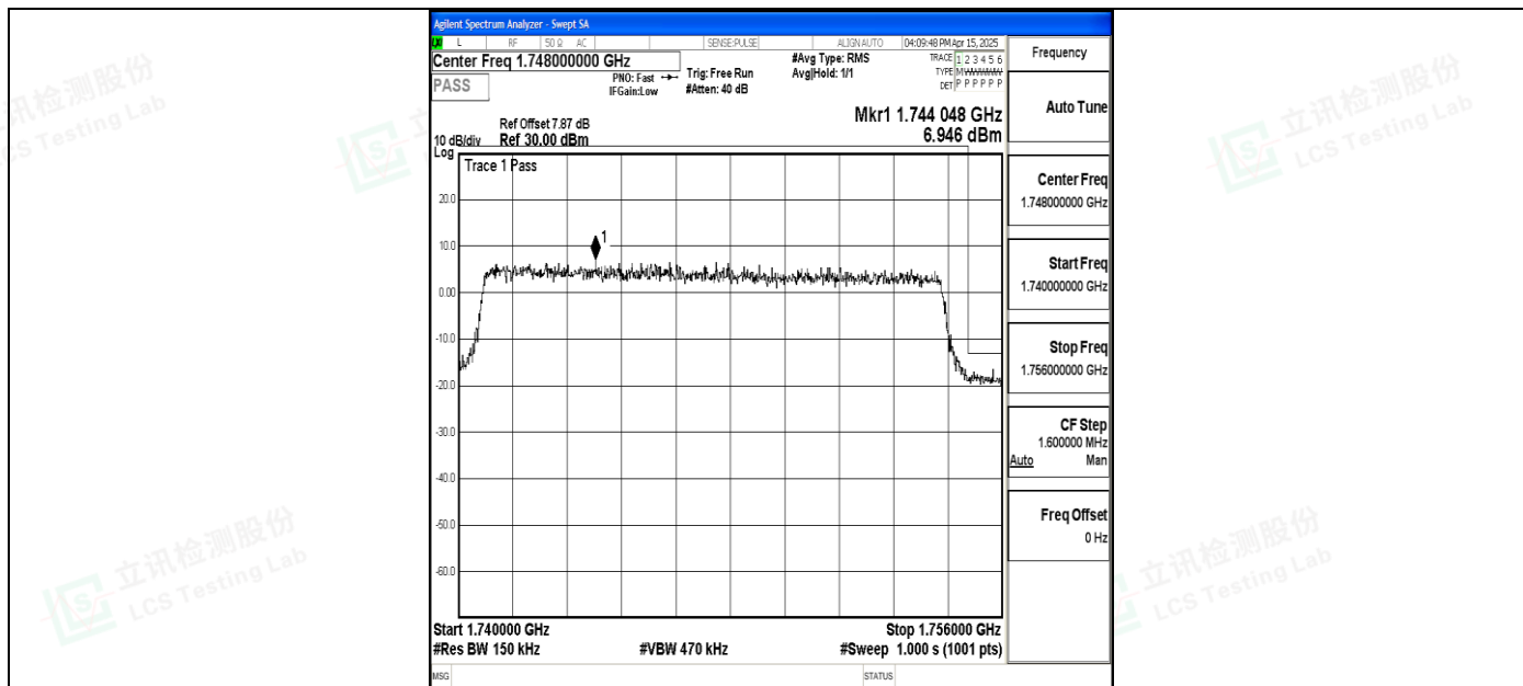
Band4_15MHz_QPSK_20325_75RB#0
