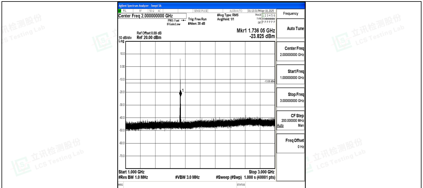
Band4_1.4MHz_16QAM_20175_1RB#0_1000~3000_1000~3000
