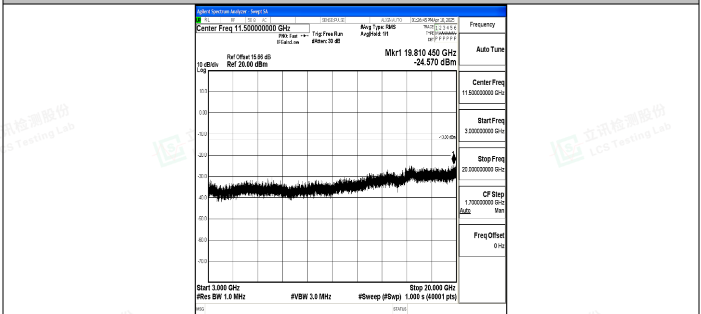
Band4_3MHz_16QAM_20175_1RB#0_3000~20000_3000~20000
