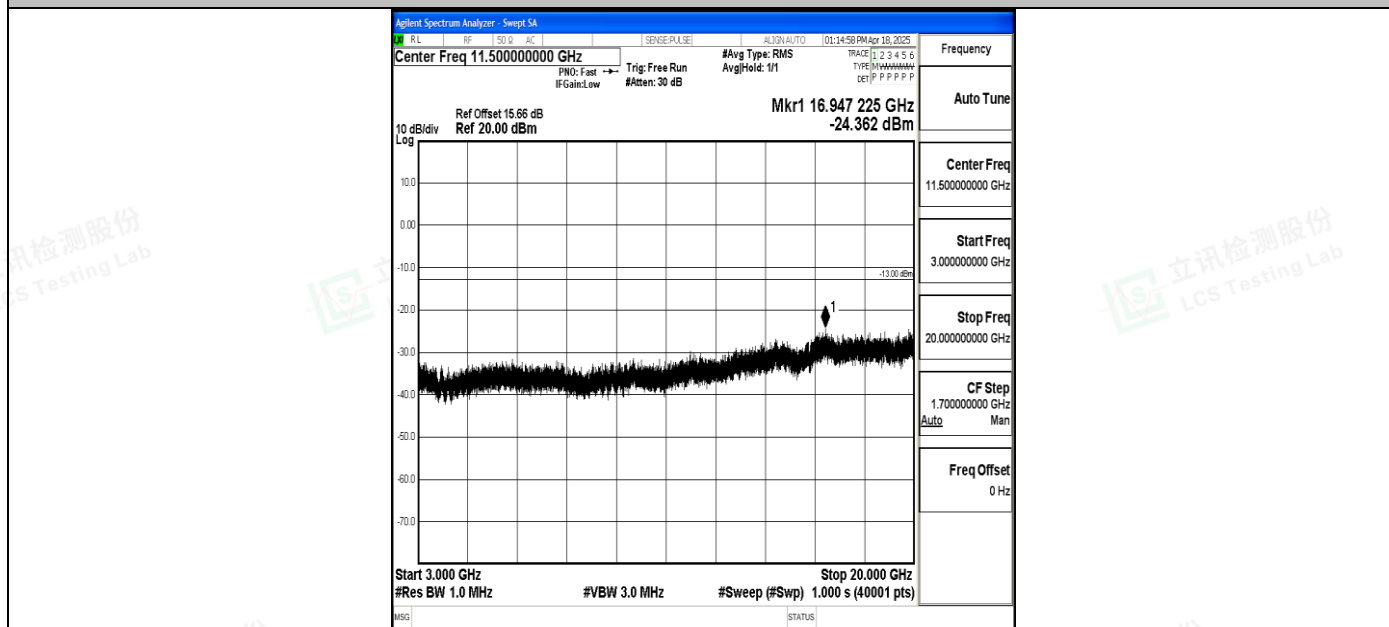
Band4_1.4MHz_16QAM_20393_1RB#0_3000~20000_3000~20000
