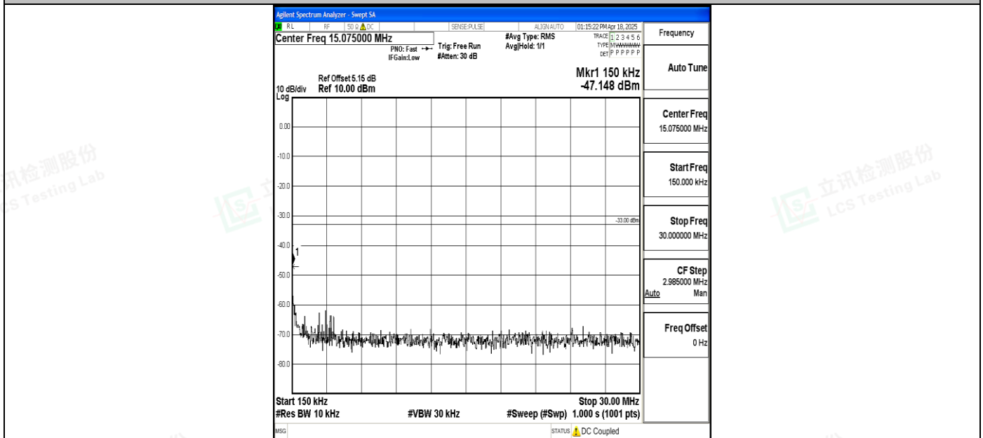
Band4_3MHz_QPSK_19965_1RB#0_0.15~30_0.15~30
