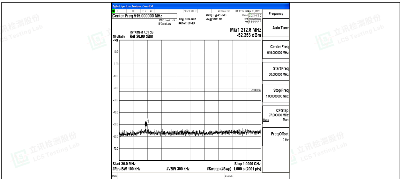
Band4_3MHz_QPSK_19965_1RB#0_30~1000_30~1000
