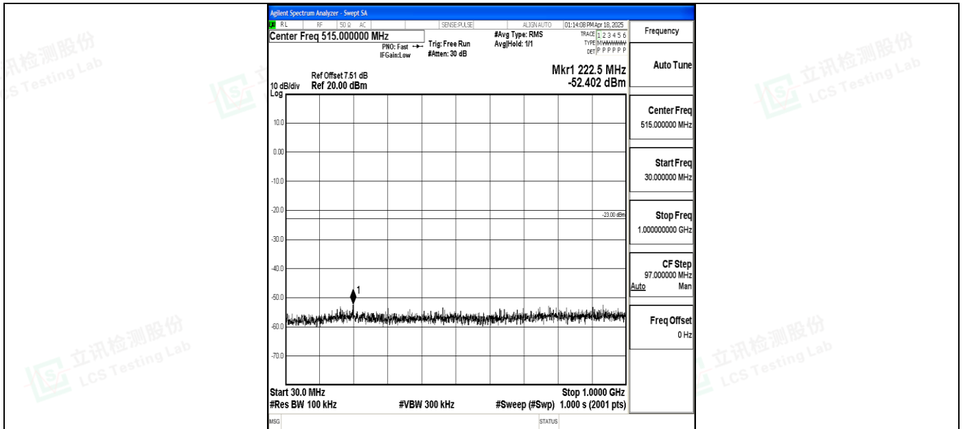
Band4_1.4MHz_QPSK_20393_1RB#0_30~1000_30~1000
