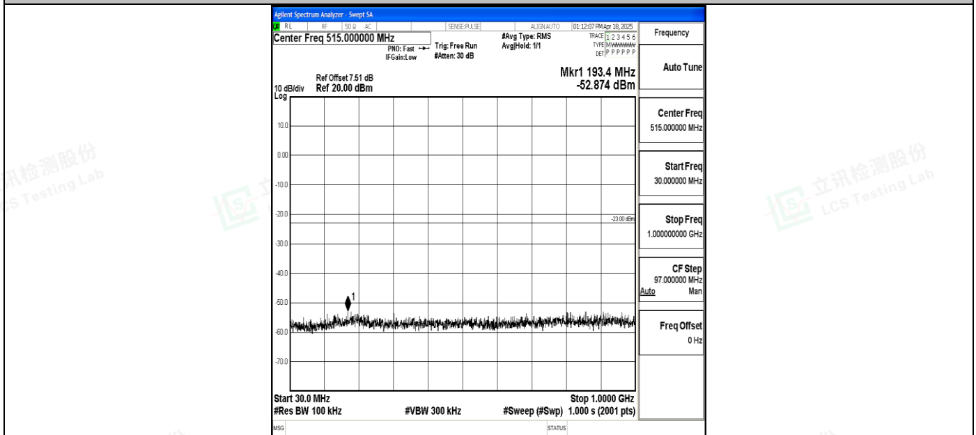
Band4_1.4MHz_16QAM_19957_1RB#0_30~1000_30~1000
