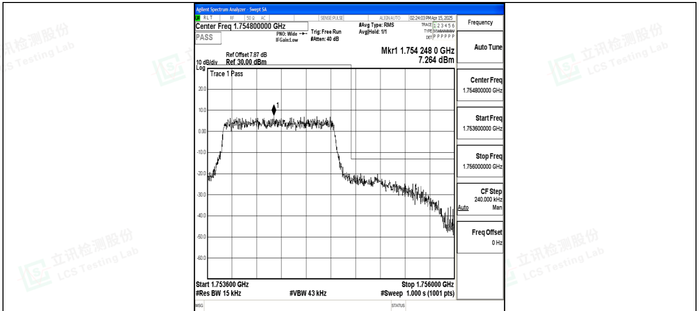
Band4_1.4MHz_QPSK_20393_6RB#0
