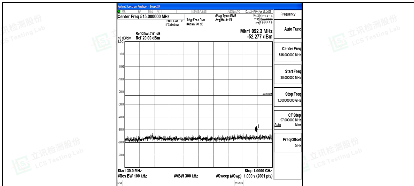
Band4_1.4MHz_QPSK_20175_1RB#0_30~1000_30~1000
