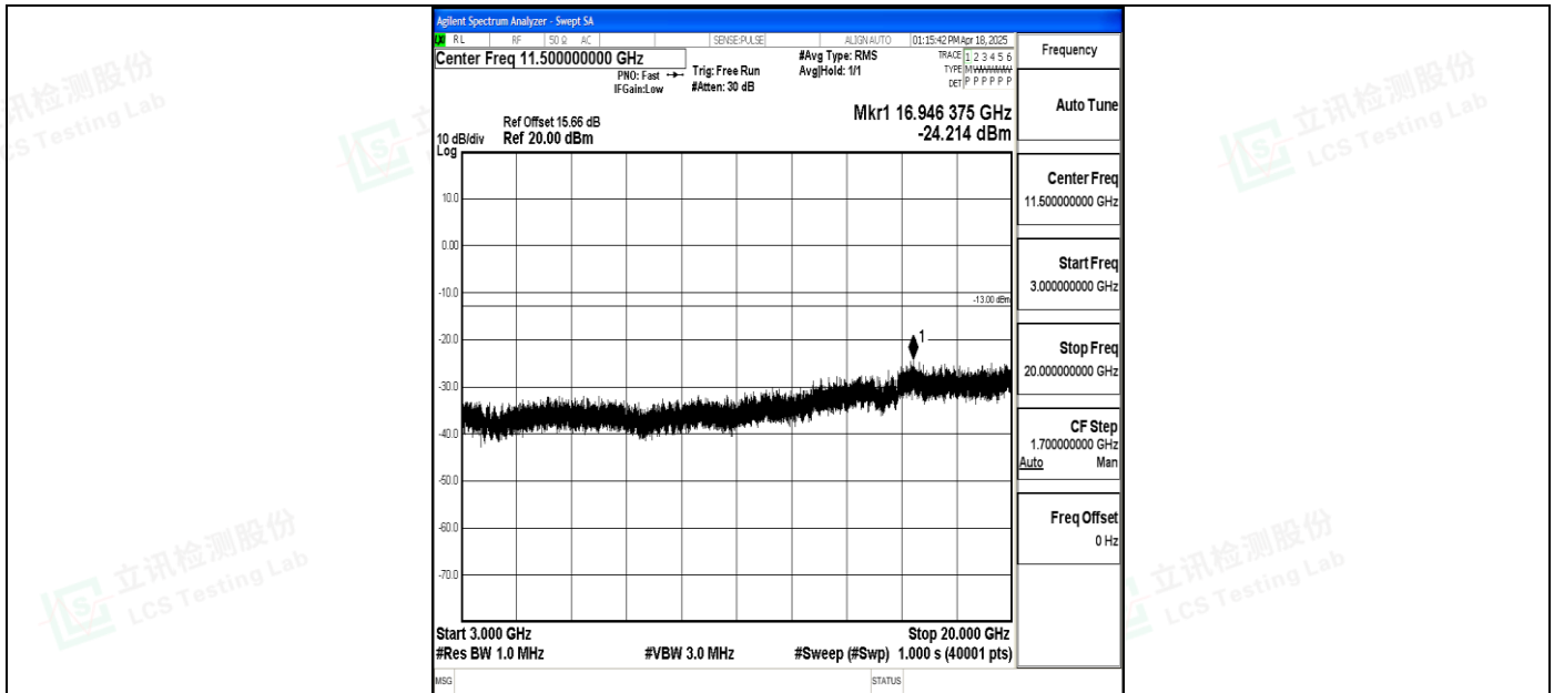
Band4_3MHz_QPSK_19965_1RB#0_3000~20000_3000~20000
