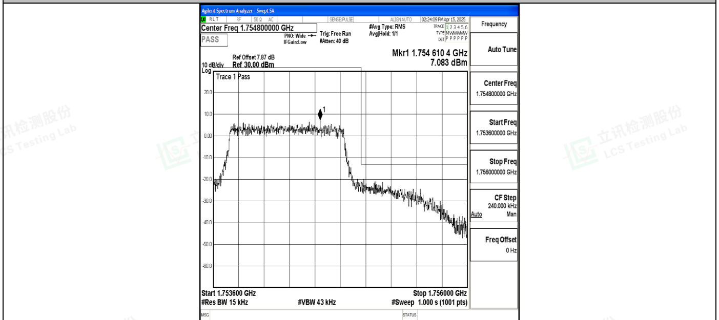
Band4_1.4MHz_16QAM_20393_6RB#0
