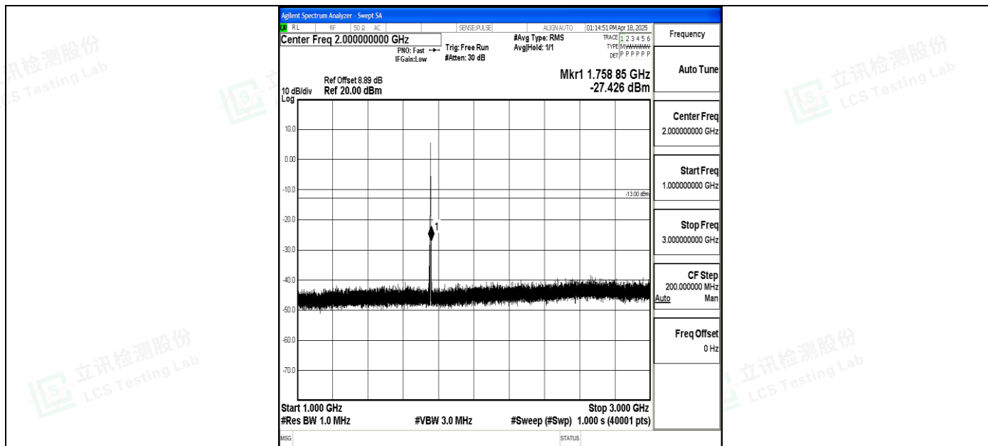
Band4_1.4MHz_16QAM_20393_1RB#0_1000~3000_1000~3000
