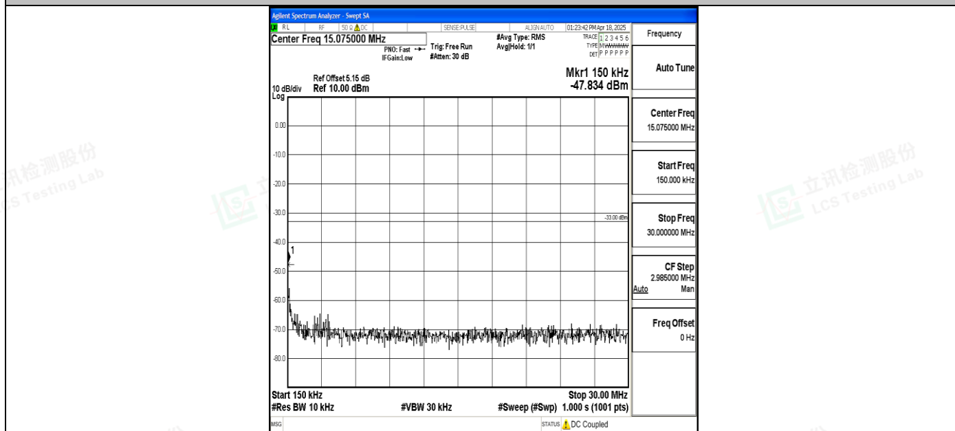
Band4_3MHz_QPSK_20175_1RB#0_0.15~30_0.15~30
