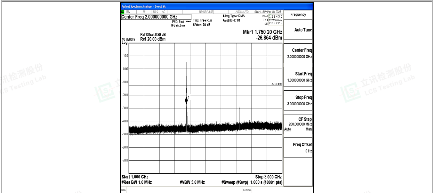
Band4_1.4MHz_QPSK_20393_1RB#0_1000~3000_1000~3000
