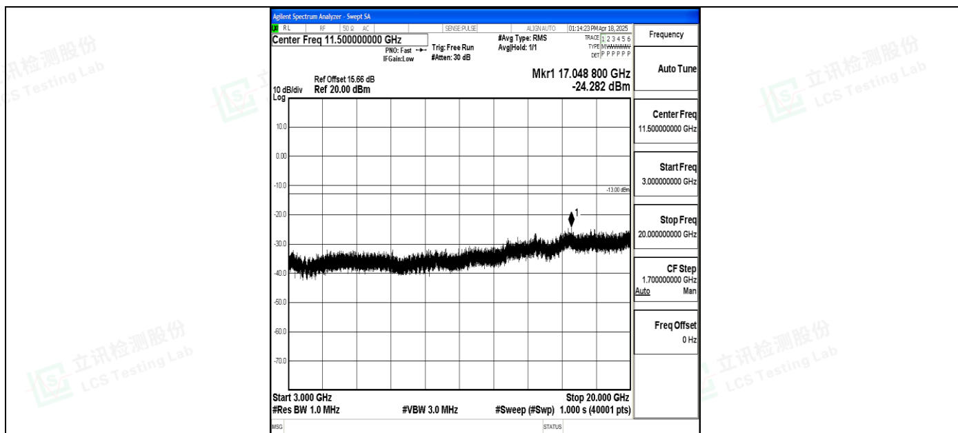
Band4_1.4MHz_QPSK_20393_1RB#0_3000~20000_3000~20000
