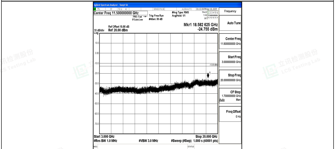
Band4_1.4MHz_16QAM_20175_1RB#0_3000~20000_3000~20000
