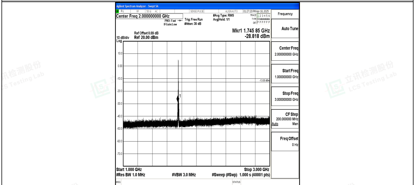
Band4_3MHz_QPSK_20385_1RB#0_1000~3000_1000~3000
