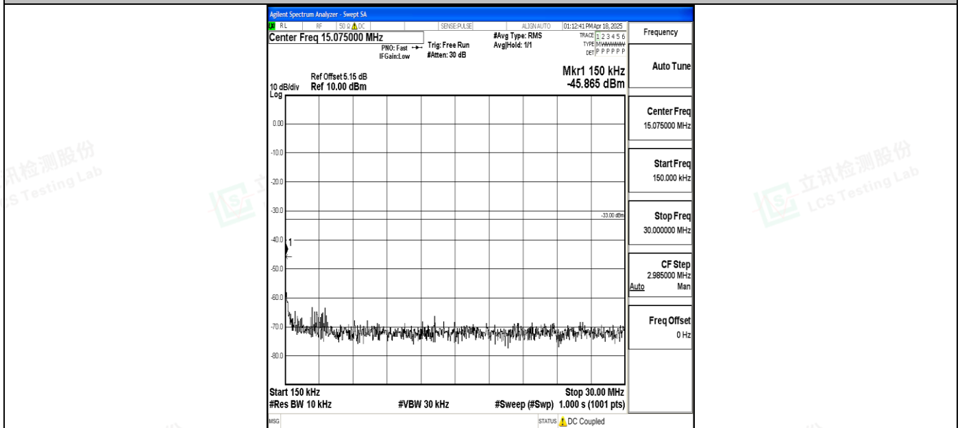
Band4_1.4MHz_QPSK_20175_1RB#0_0.15~30_0.15~30
