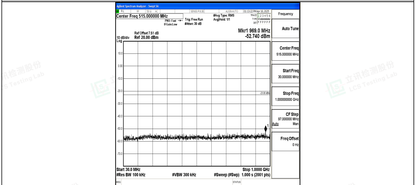
Band4_1.4MHz_16QAM_20175_1RB#0_30~1000_30~1000
