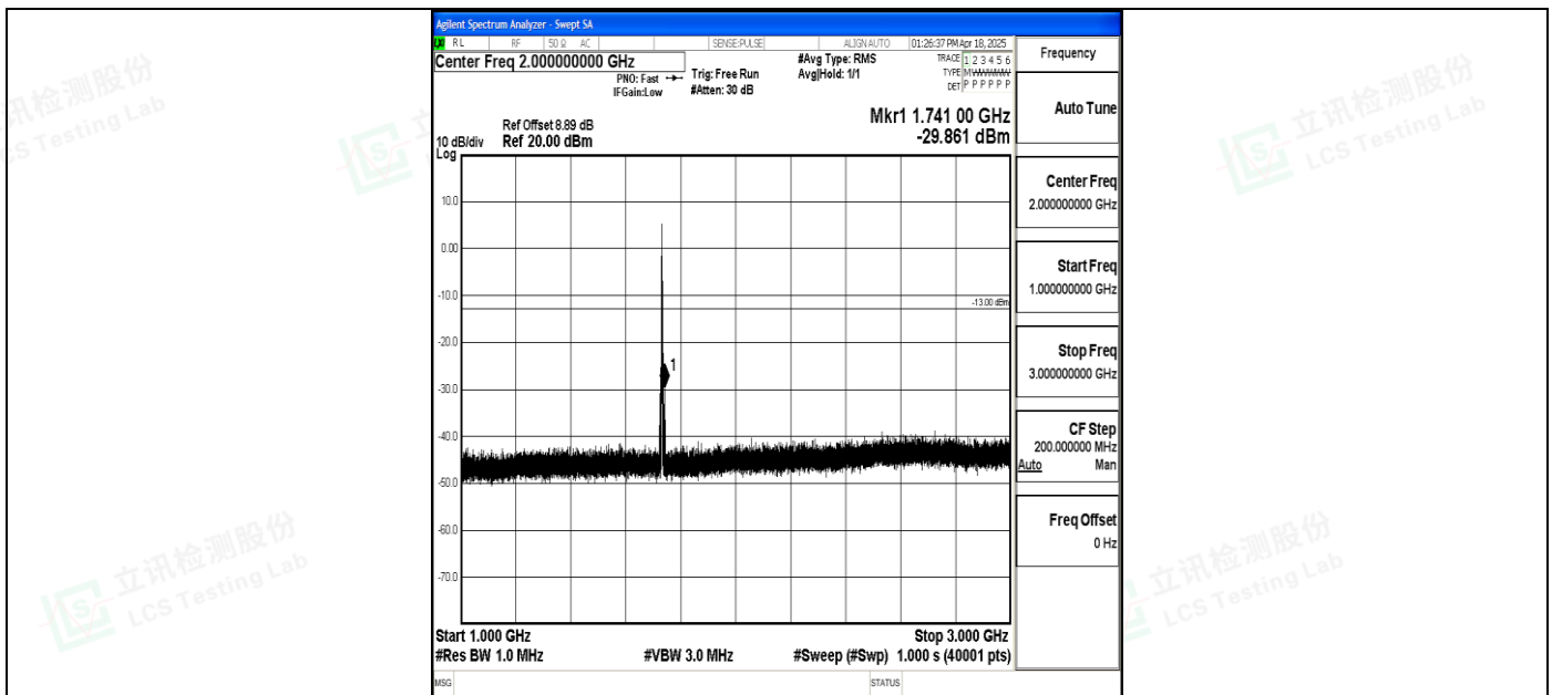
Band4_3MHz_16QAM_20175_1RB#0_1000~3000_1000~3000
