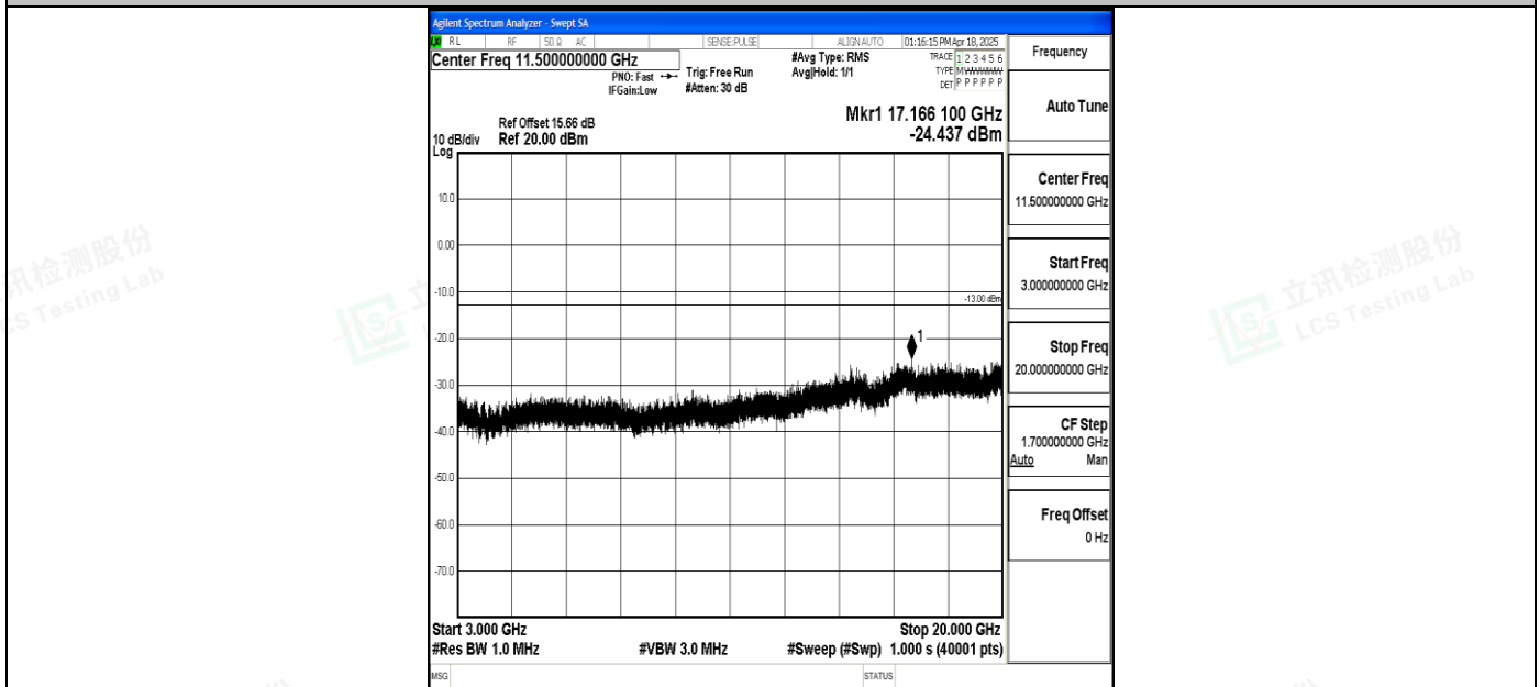
Band4_3MHz_16QAM_19965_1RB#0_3000~20000_3000~20000
