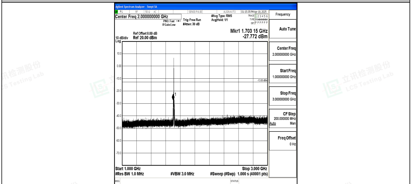
Band4_3MHz_QPSK_19965_1RB#0_1000~3000_1000~3000
