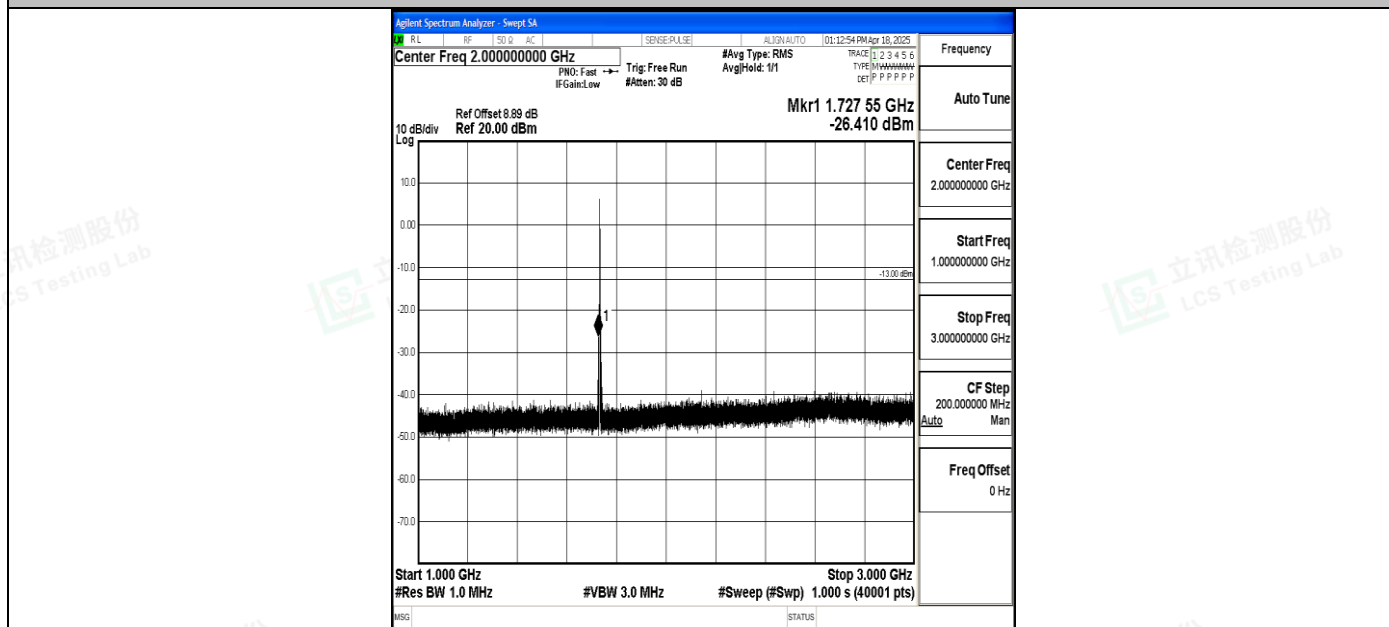
Band4_1.4MHz_QPSK_20175_1RB#0_1000~3000_1000~3000
