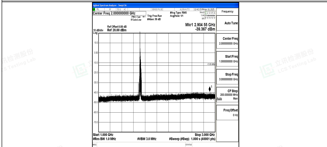
Band4_15MHz_QPSK_20025_1RB#0_1000~3000_1000~3000
