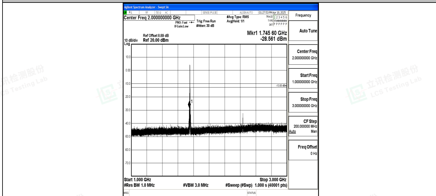
Band4_3MHz_16QAM_20385_1RB#0_1000~3000_1000~3000
