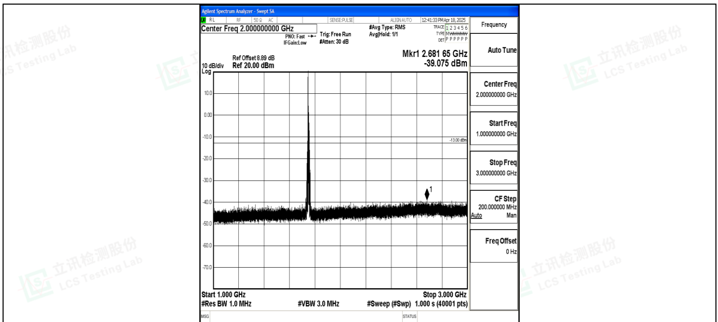
Band4_10MHz_16QAM_20350_1RB#0_1000~3000_1000~3000
