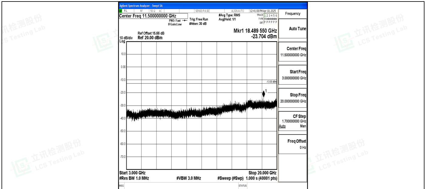
Band4_10MHz_QPSK_20350_1RB#0_3000~20000_3000~20000
