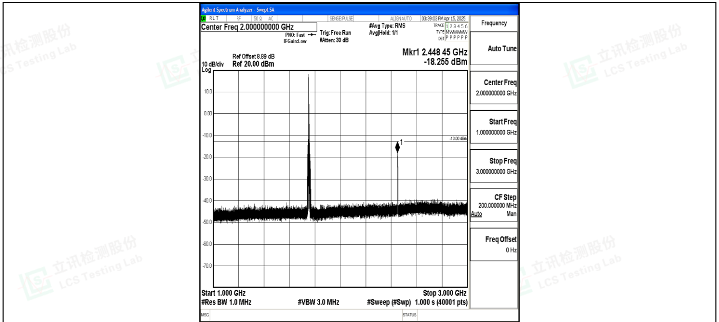
Band4_5MHz_16QAM_20375_1RB#0_1000~3000_1000~3000
