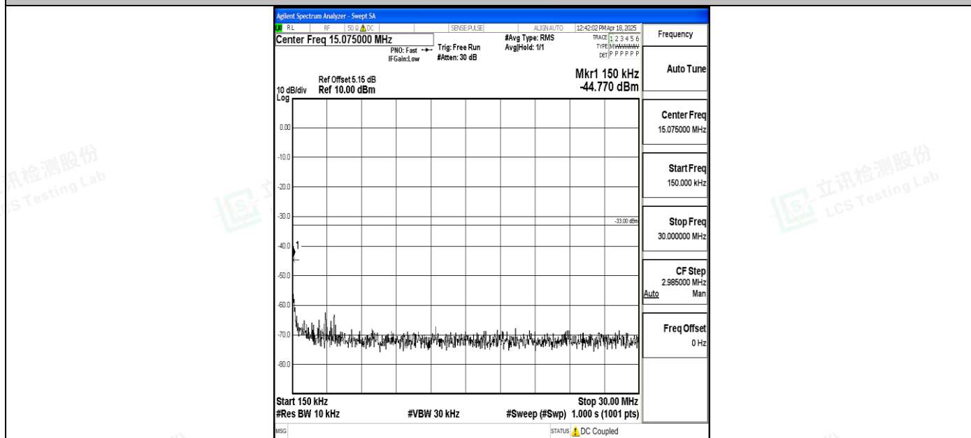
Band4_15MHz_QPSK_20025_1RB#0_0.15~30_0.15~30
