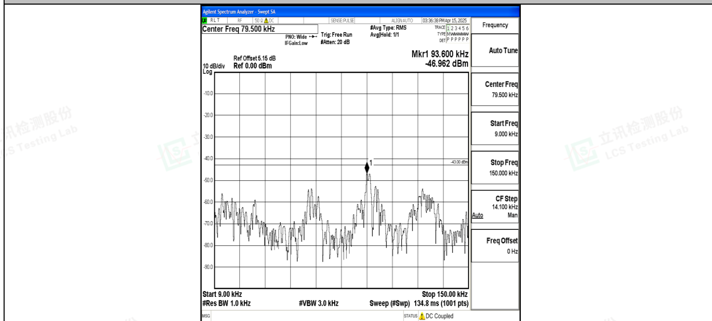
Band4_5MHz_16QAM_19975_1RB#0_0.009~0.15_0.009~0.15
