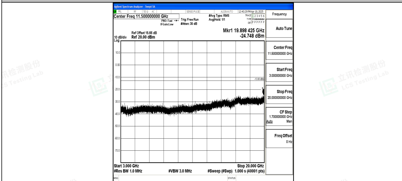
Band4_10MHz_16QAM_20175_1RB#0_3000~20000_3000~20000
