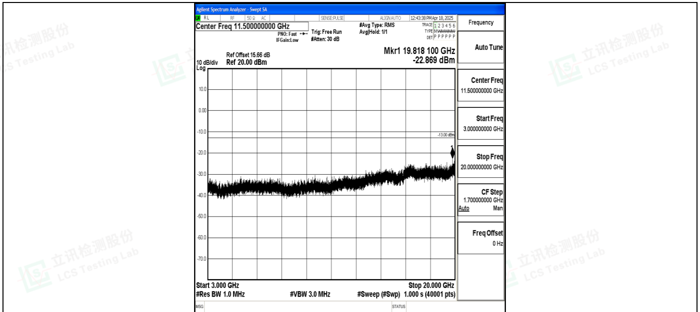
Band4_15MHz_QPSK_20175_1RB#0_3000~20000_3000~20000
