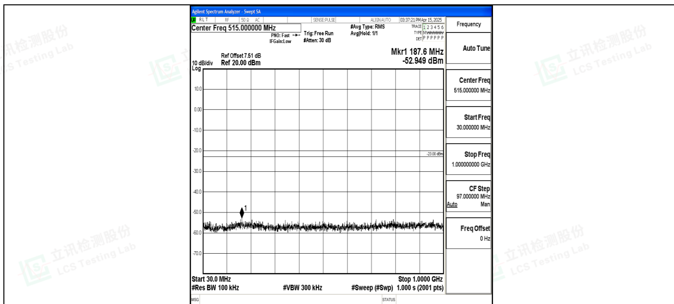
Band4_5MHz_QPSK_20175_1RB#0_30~1000_30~1000
