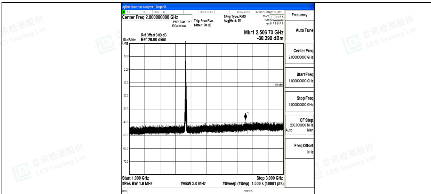
Band4_10MHz_16QAM_20175_1RB#0_1000~3000_1000~3000
