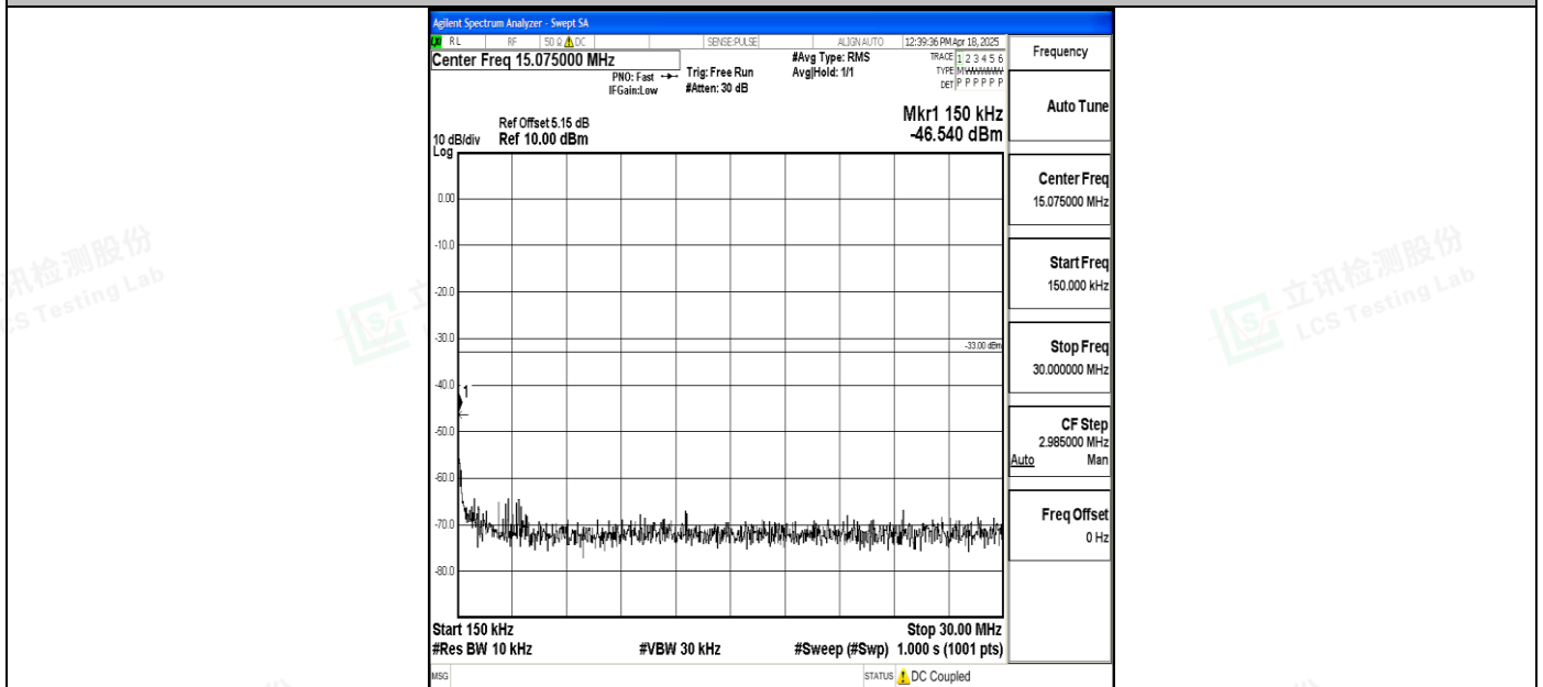
Band4_10MHz_QPSK_20175_1RB#0_0.15~30_0.15~30
