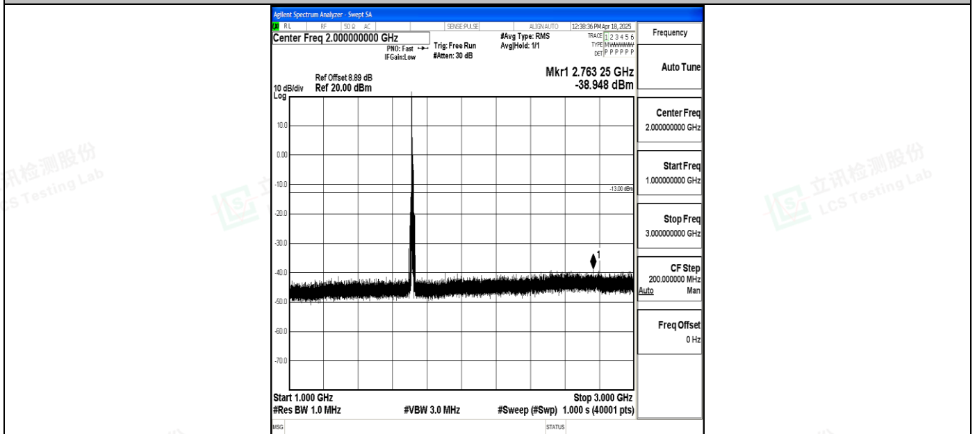
Band4_10MHz_QPSK_20000_1RB#0_1000~3000_1000~3000
