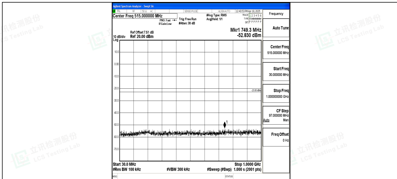
Band4_10MHz_QPSK_20350_1RB#0_30~1000_30~1000
