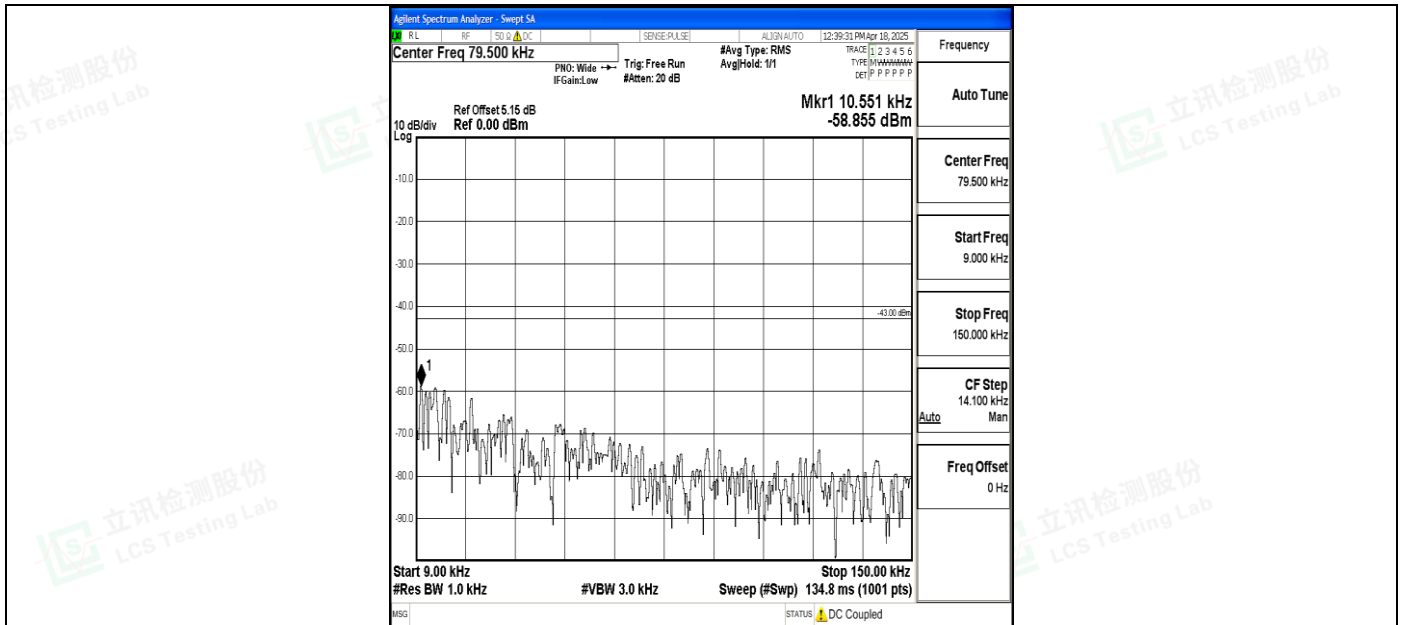
Band4_10MHz_QPSK_20175_1RB#0_0.009~0.15_0.009~0.15
