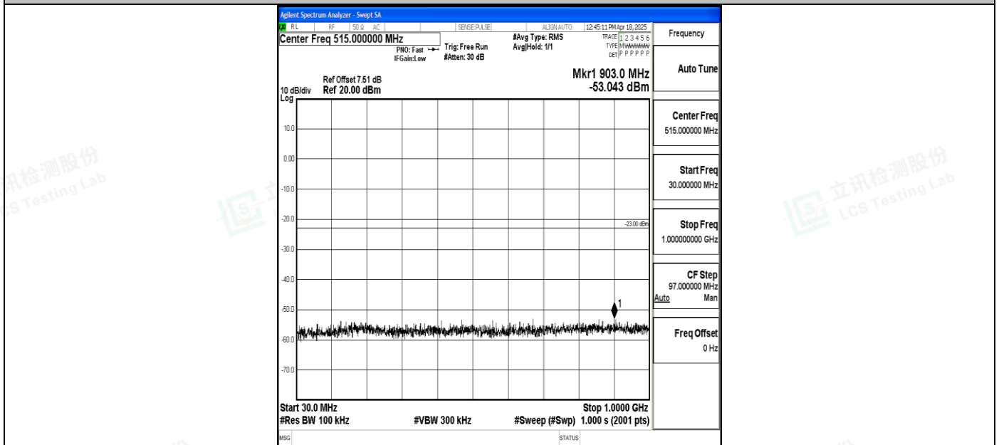
Band4_15MHz_16QAM_20325_1RB#0_30~1000_30~1000
