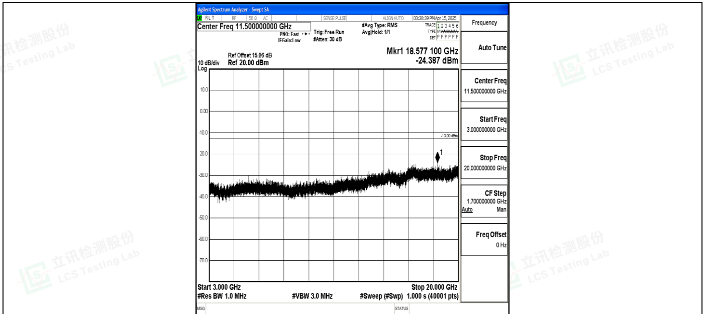
Band4_5MHz_QPSK_20375_1RB#0_3000~20000_3000~20000
