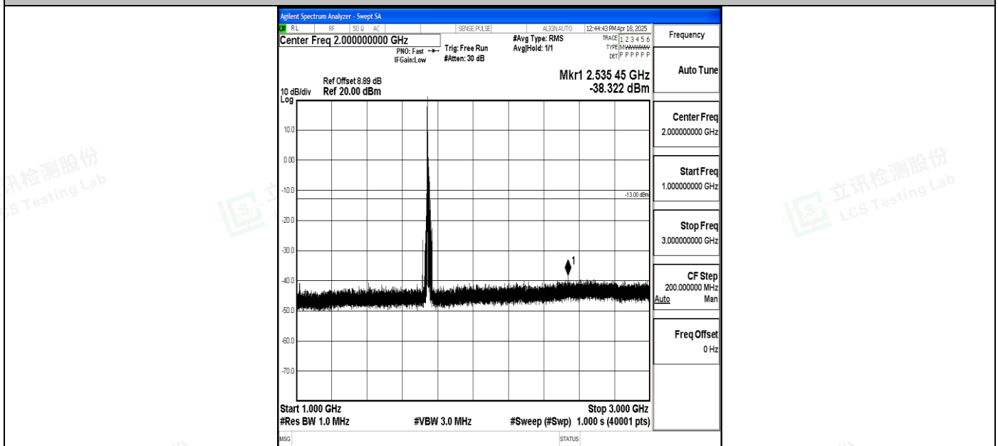
Band4_15MHz_QPSK_20325_1RB#0_1000~3000_1000~3000
