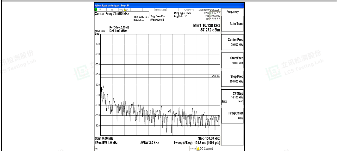
Band4_10MHz_16QAM_20000_1RB#0_0.009~0.15_0.009~0.15
