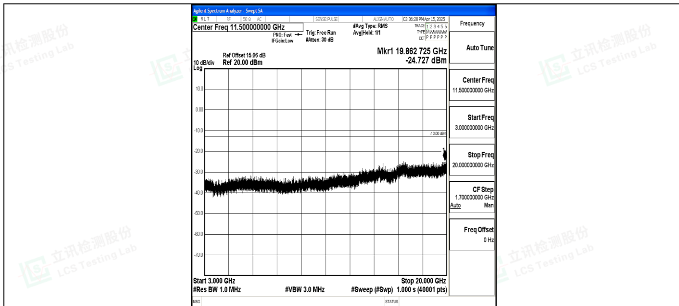
Band4_5MHz_QPSK_19975_1RB#0_3000~20000_3000~20000
