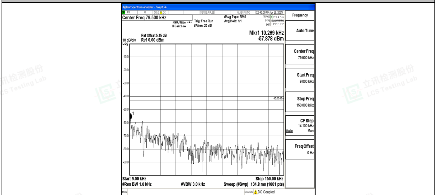
Band4_15MHz_16QAM_20325_1RB#0_0.009~0.15_0.009~0.15
