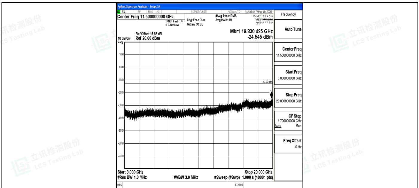
Band4_10MHz_QPSK_20000_1RB#0_3000~20000_3000~20000
