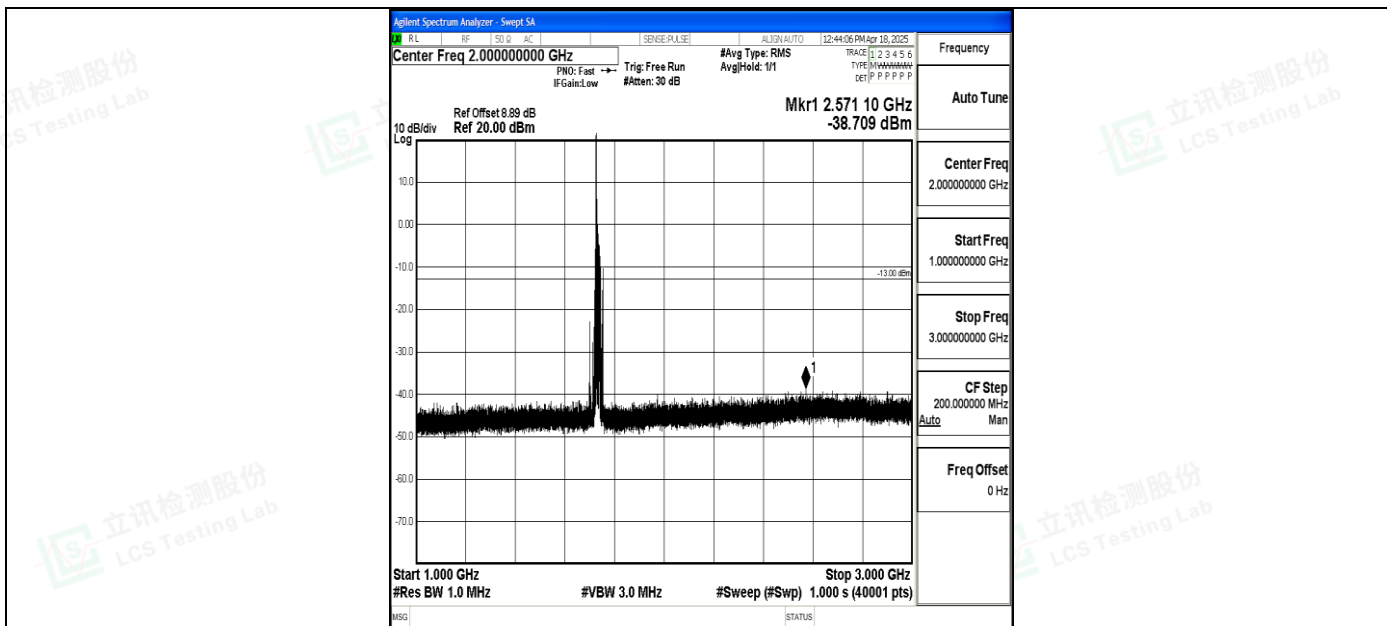
Band4_15MHz_16QAM_20175_1RB#0_1000~3000_1000~3000
