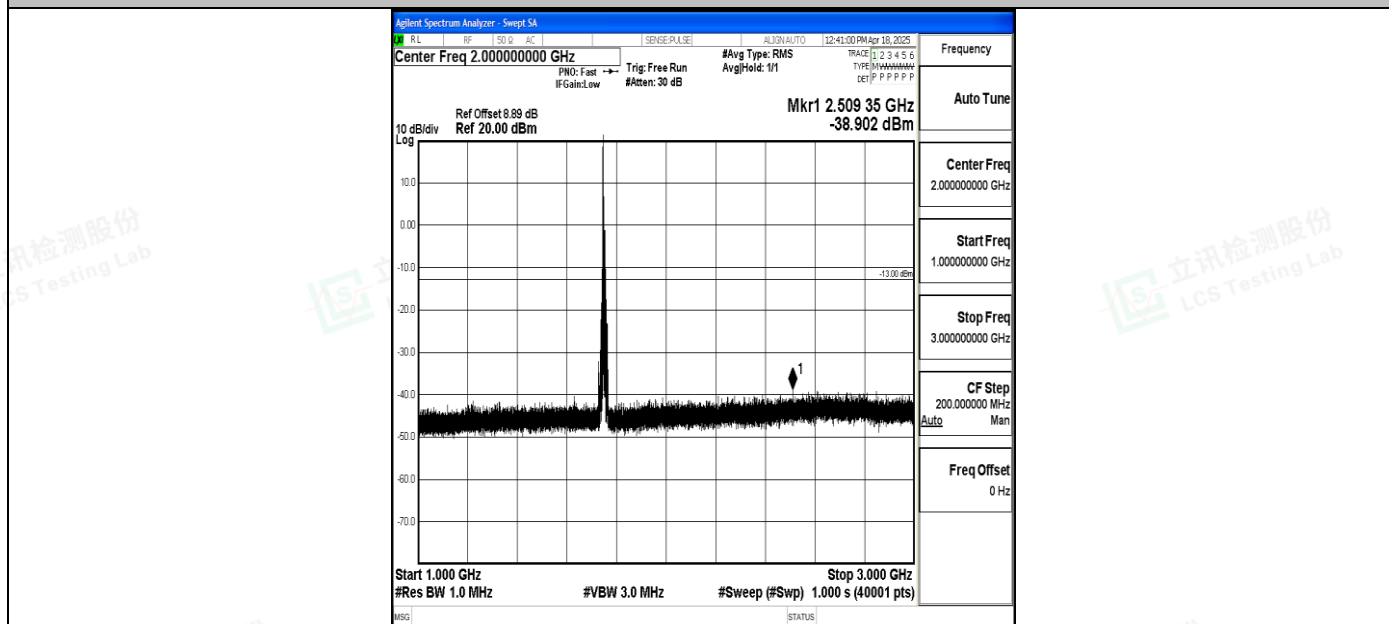
Band4_10MHz_QPSK_20350_1RB#0_1000~3000_1000~3000
