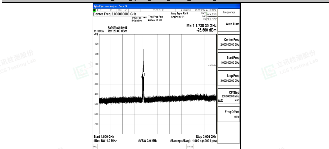
Band4_5MHz_QPSK_20375_1RB#0_1000~3000_1000~3000
