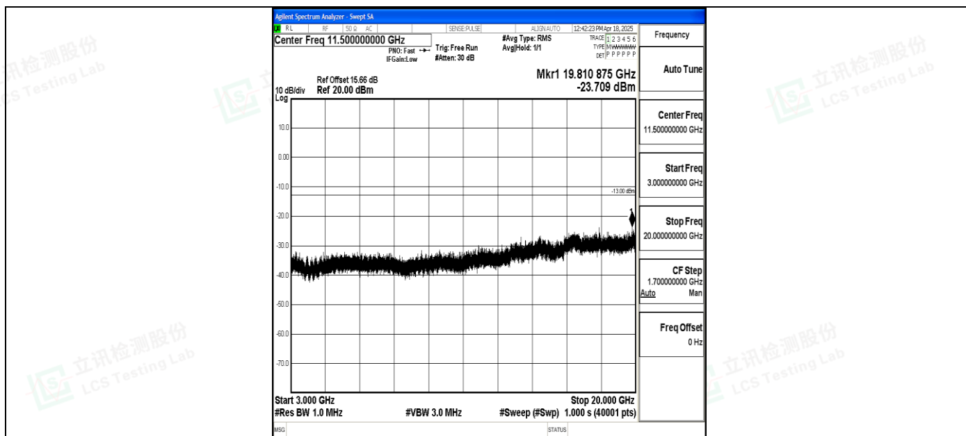
Band4_15MHz_QPSK_20025_1RB#0_3000~20000_3000~20000
