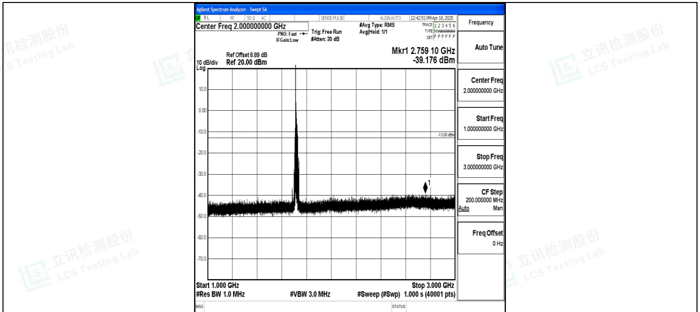
Band4_15MHz_16QAM_20025_1RB#0_1000~3000_1000~3000
