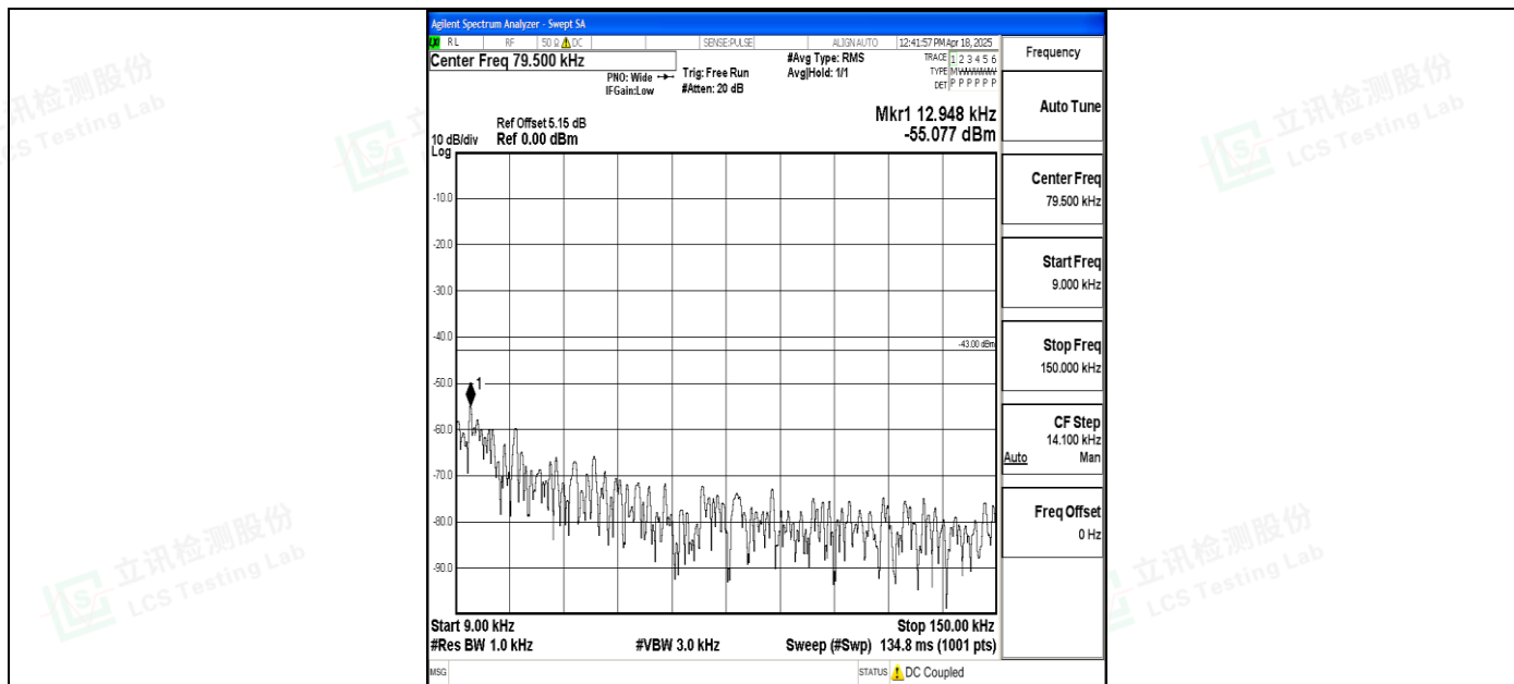
Band4_15MHz_QPSK_20025_1RB#0_0.009~0.15_0.009~0.15
