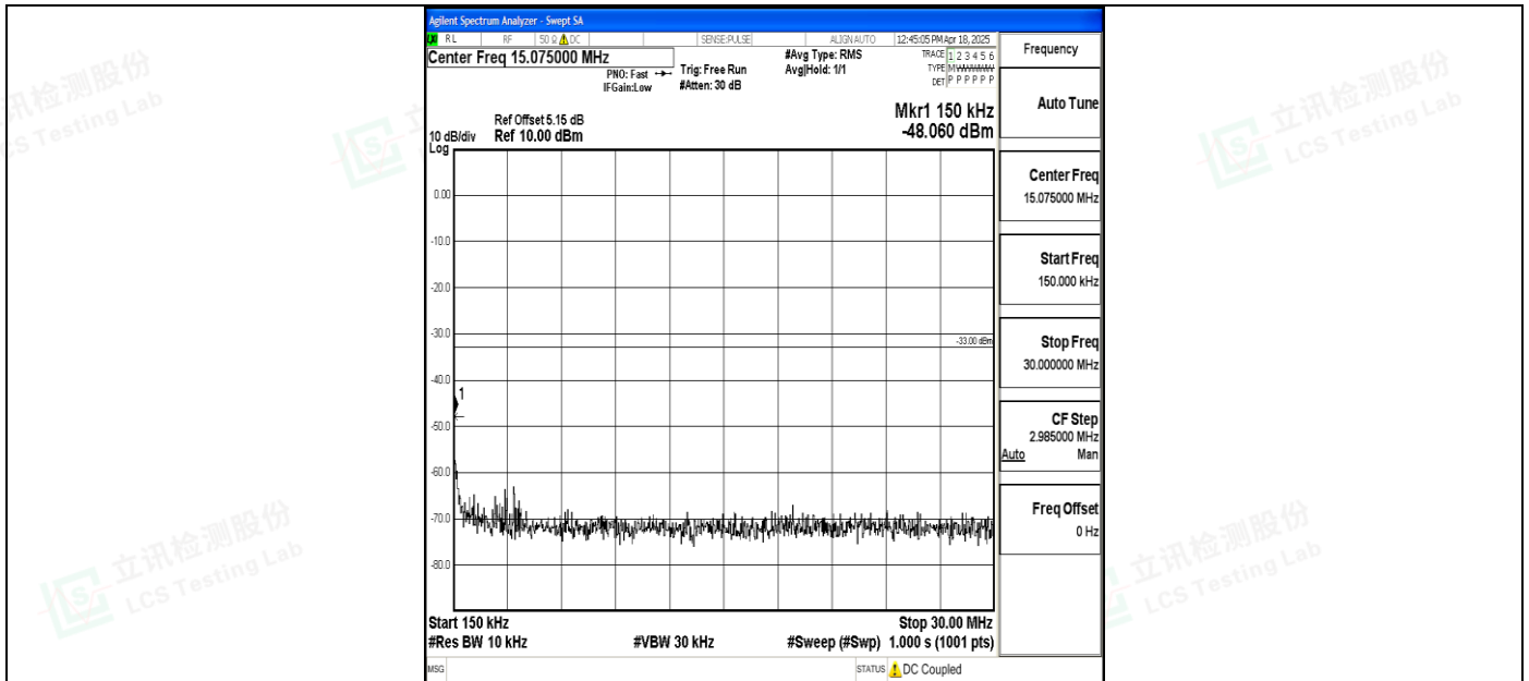
Band4_15MHz_16QAM_20325_1RB#0_0.15~30_0.15~30
