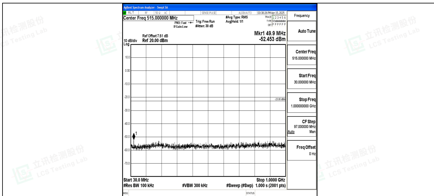
Band4_5MHz_QPSK_20375_1RB#0_30~1000_30~1000
