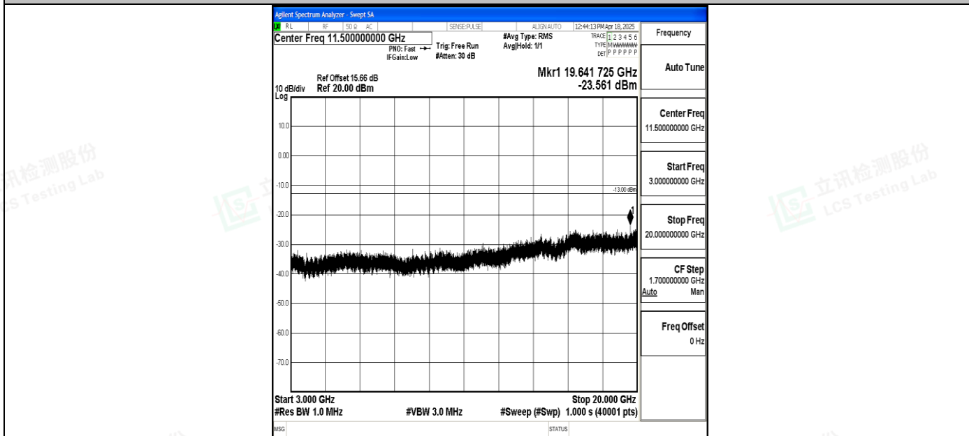
Band4_15MHz_16QAM_20175_1RB#0_3000~20000_3000~20000
