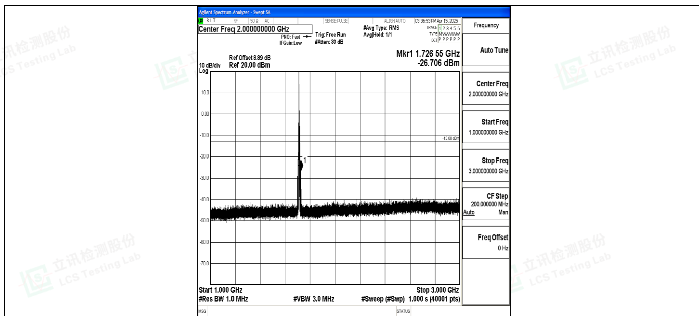
Band4_5MHz_16QAM_19975_1RB#0_1000~3000_1000~3000
