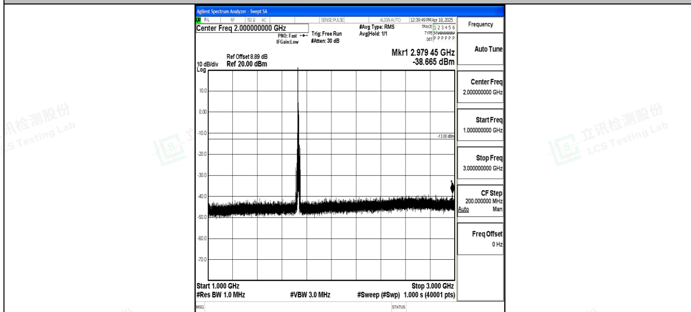
Band4_10MHz_QPSK_20175_1RB#0_1000~3000_1000~3000
