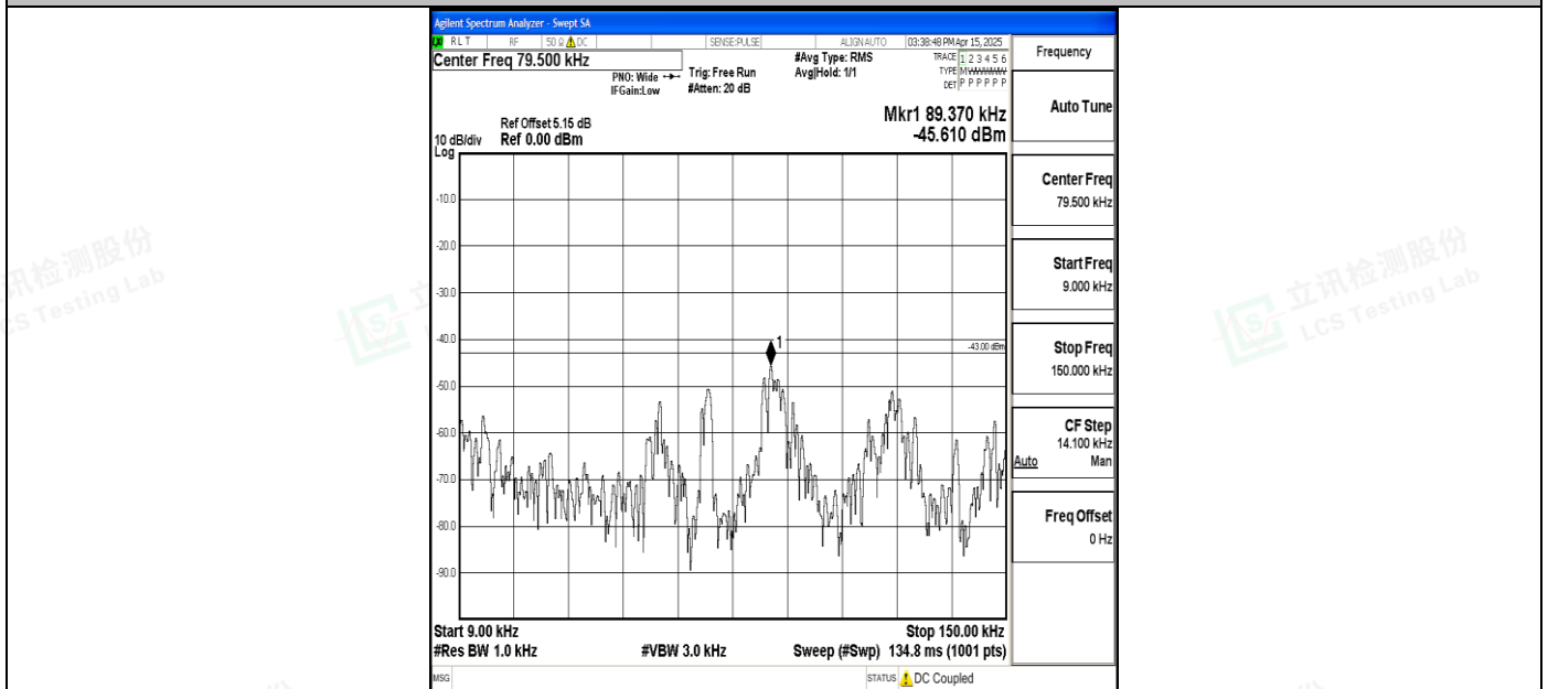
Band4_5MHz_16QAM_20375_1RB#0_0.009~0.15_0.009~0.15
