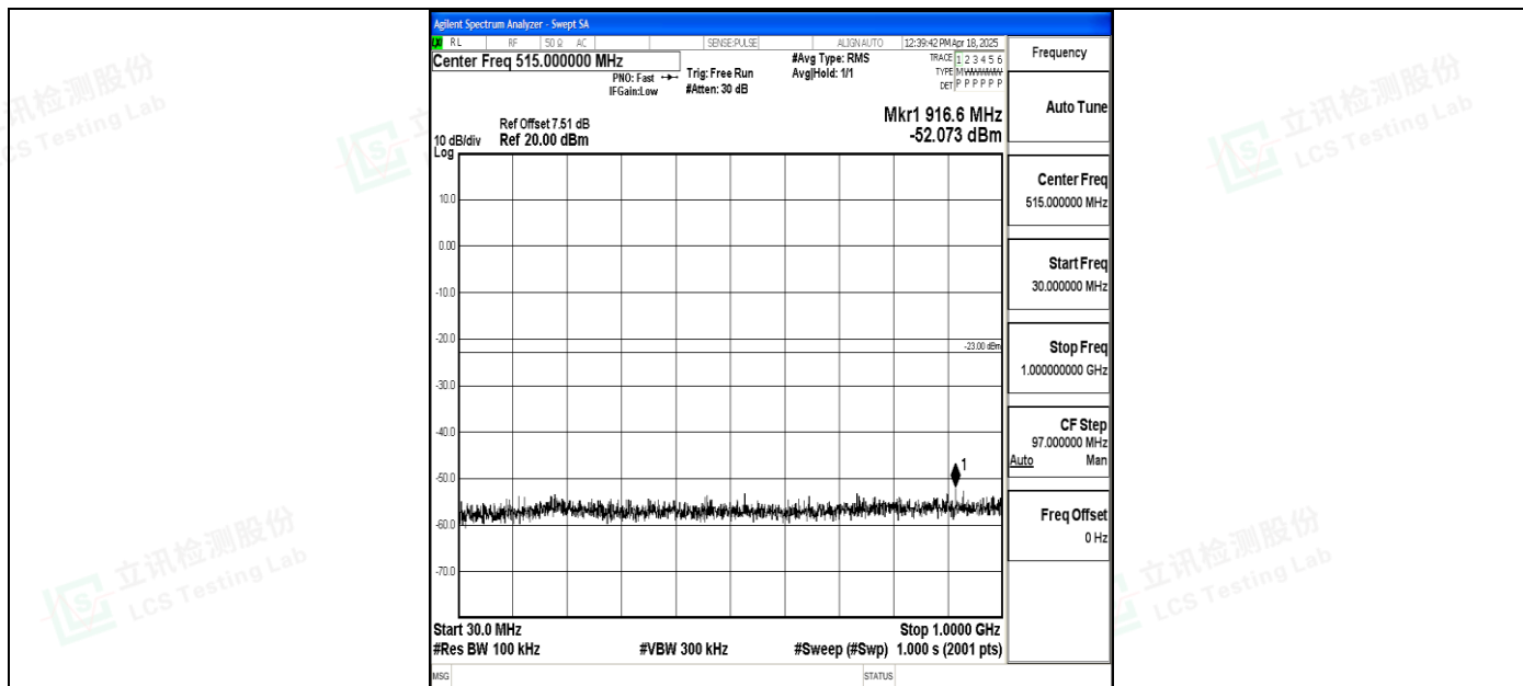
Band4_10MHz_QPSK_20175_1RB#0_30~1000_30~1000
