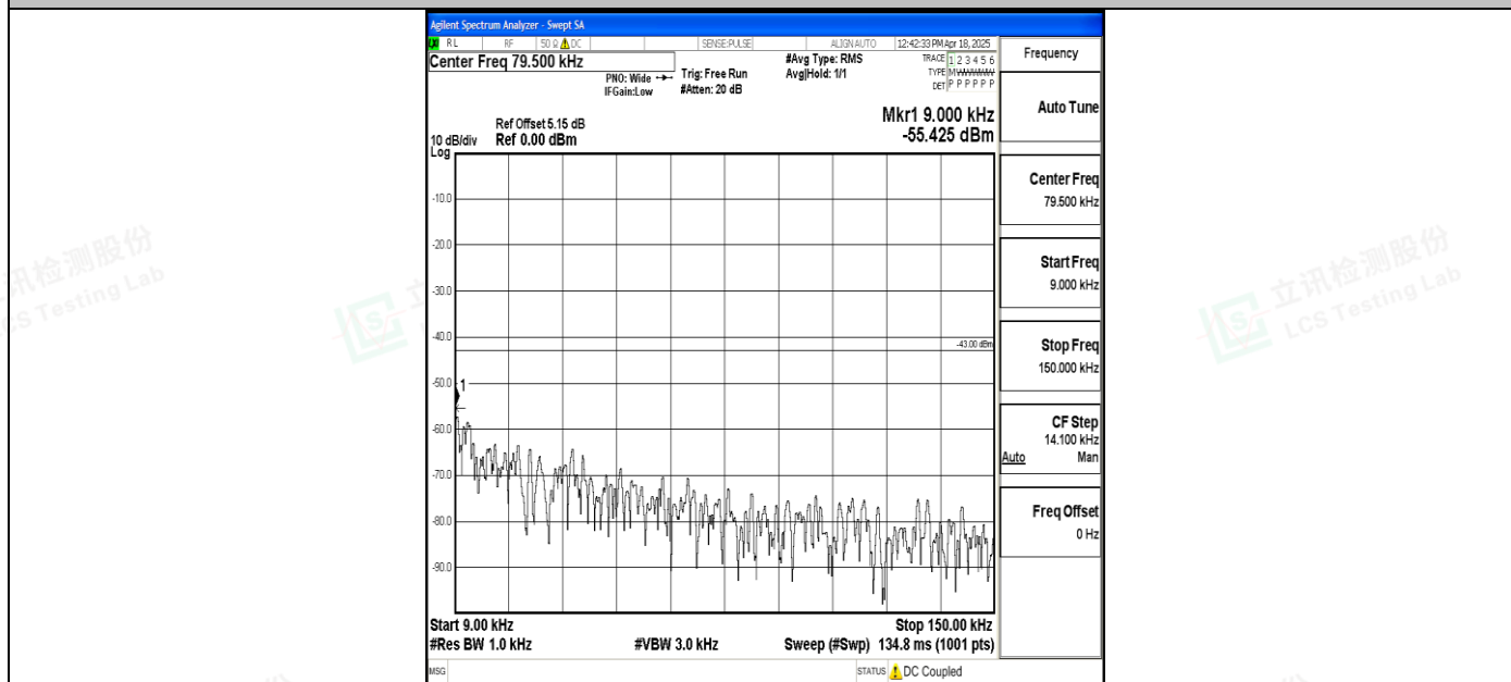
Band4_15MHz_16QAM_20025_1RB#0_0.009~0.15_0.009~0.15
