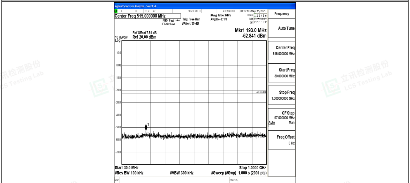
Band4_20MHz_16QAM_20050_1RB#0_30~1000_30~1000
