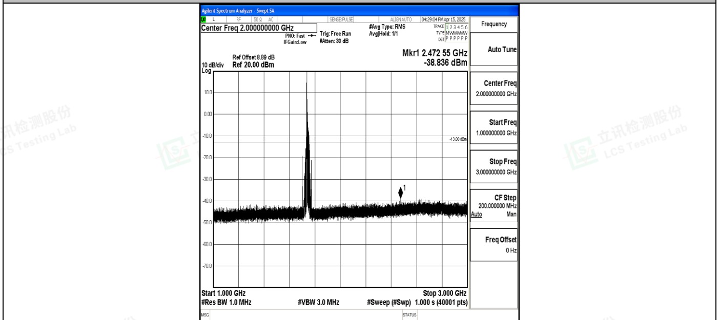
Band4_20MHz_QPSK_20300_1RB#0_1000~3000_1000~3000
