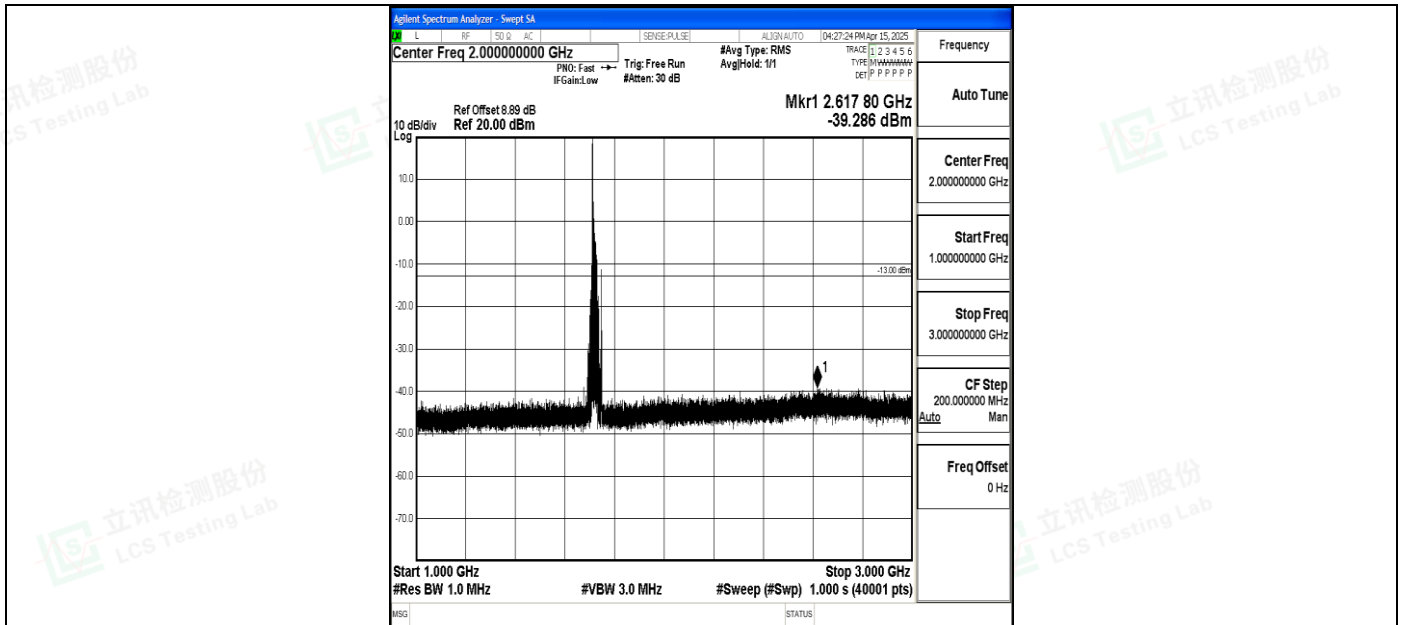
Band4_20MHz_16QAM_20050_1RB#0_1000~3000_1000~3000
