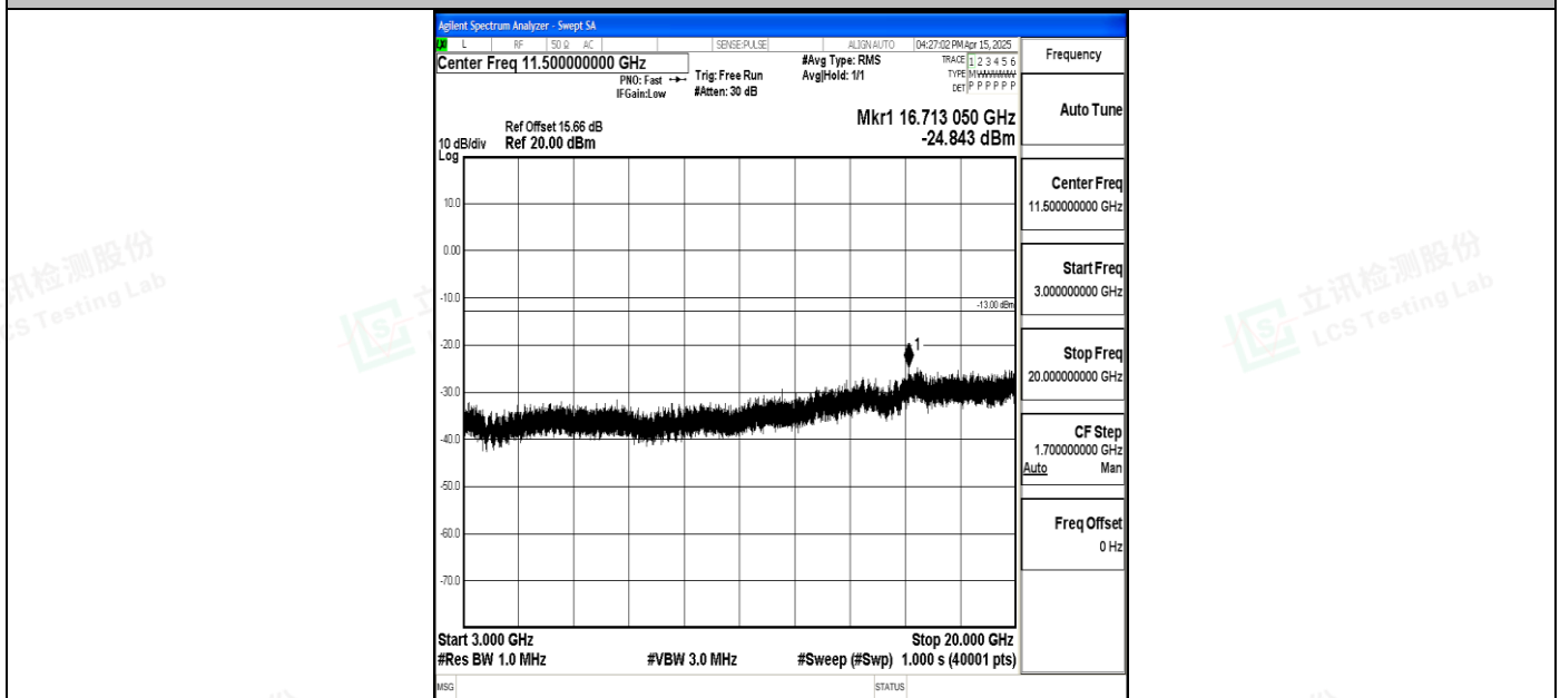
Band4_20MHz_QPSK_20050_1RB#0_3000~20000_3000~20000
