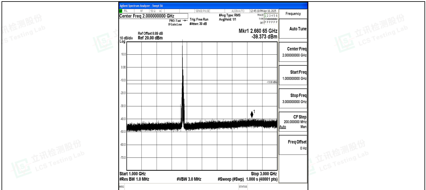
Band4_15MHz_16QAM_20325_1RB#0_1000~3000_1000~3000
