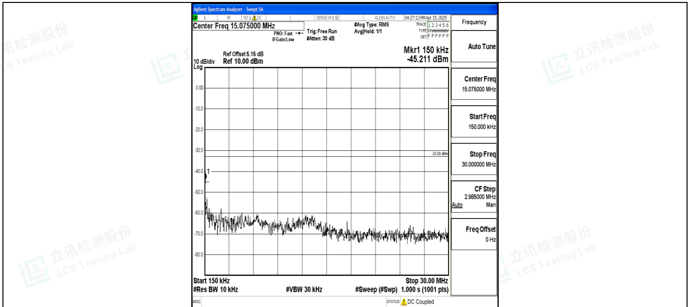
Band4_20MHz_16QAM_20050_1RB#0_0.15~30_0.15~30
