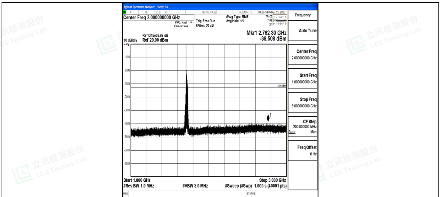
Band4_20MHz_QPSK_20050_1RB#0_1000~3000_1000~3000
