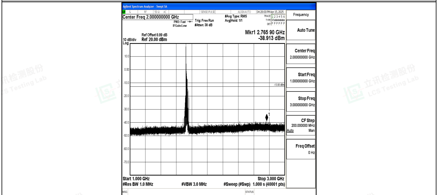
Band4_20MHz_QPSK_20175_1RB#0_1000~3000_1000~3000
