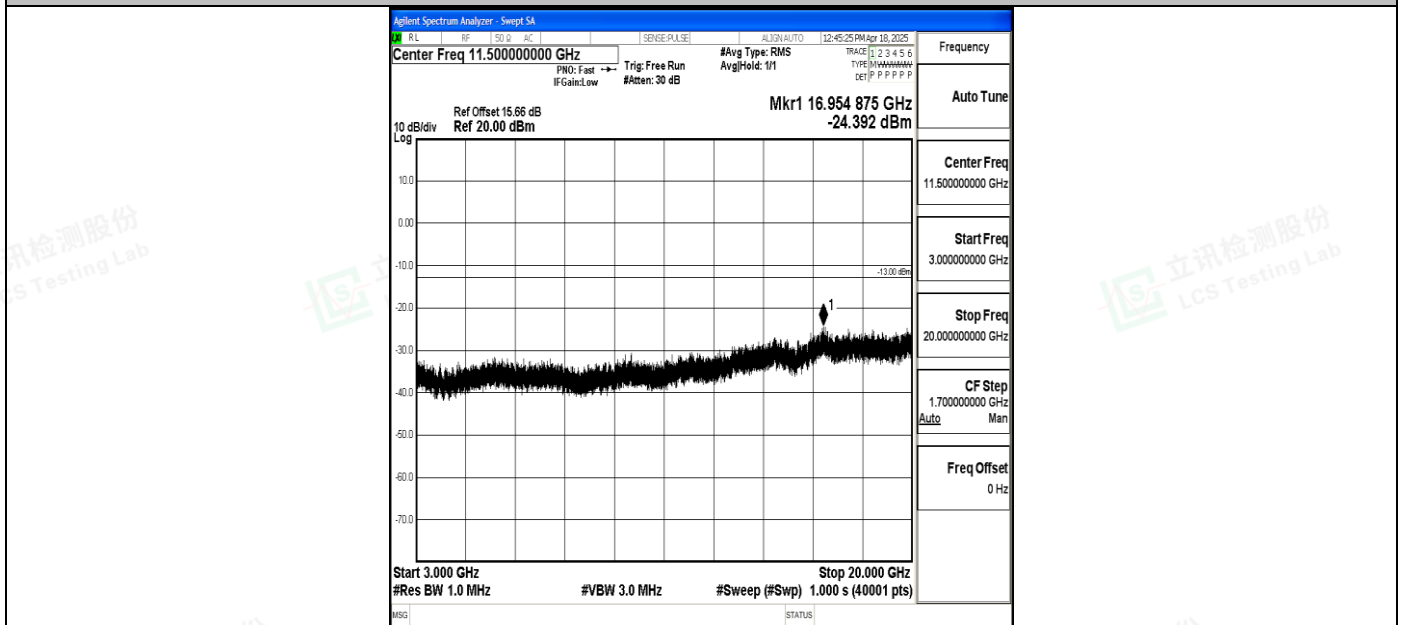
Band4_15MHz_16QAM_20325_1RB#0_3000~20000_3000~20000
