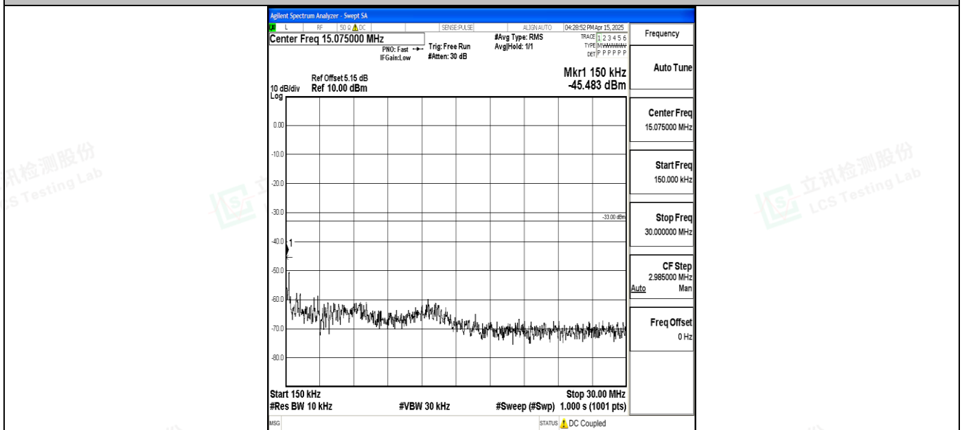
Band4_20MHz_QPSK_20300_1RB#0_0.15~30_0.15~30
