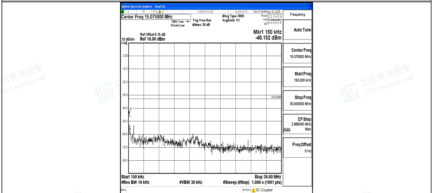
Band4_20MHz_QPSK_20175_1RB#0_0.15~30_0.15~30
