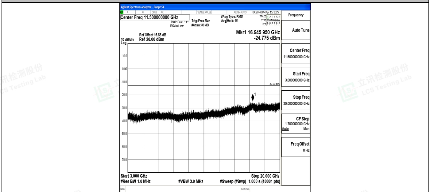
Band4_20MHz_16QAM_20300_1RB#0_3000~20000_3000~20000
