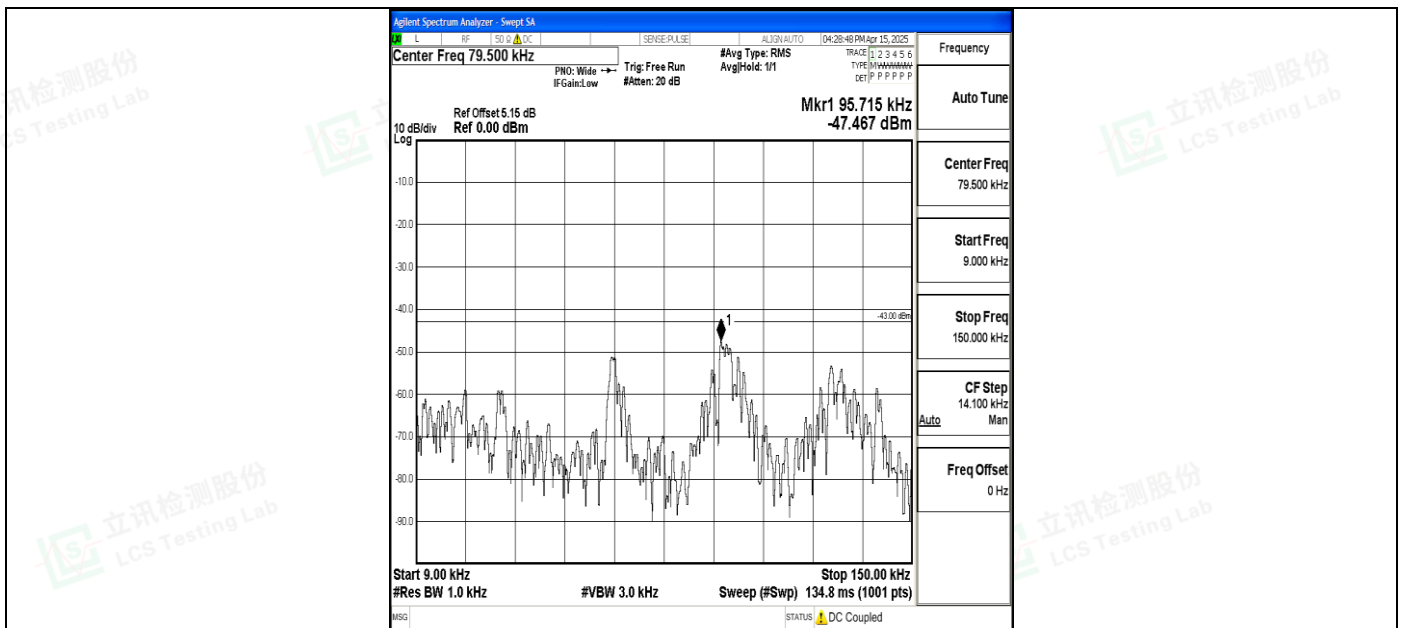
Band4_20MHz_QPSK_20300_1RB#0_0.009~0.15_0.009~0.15
