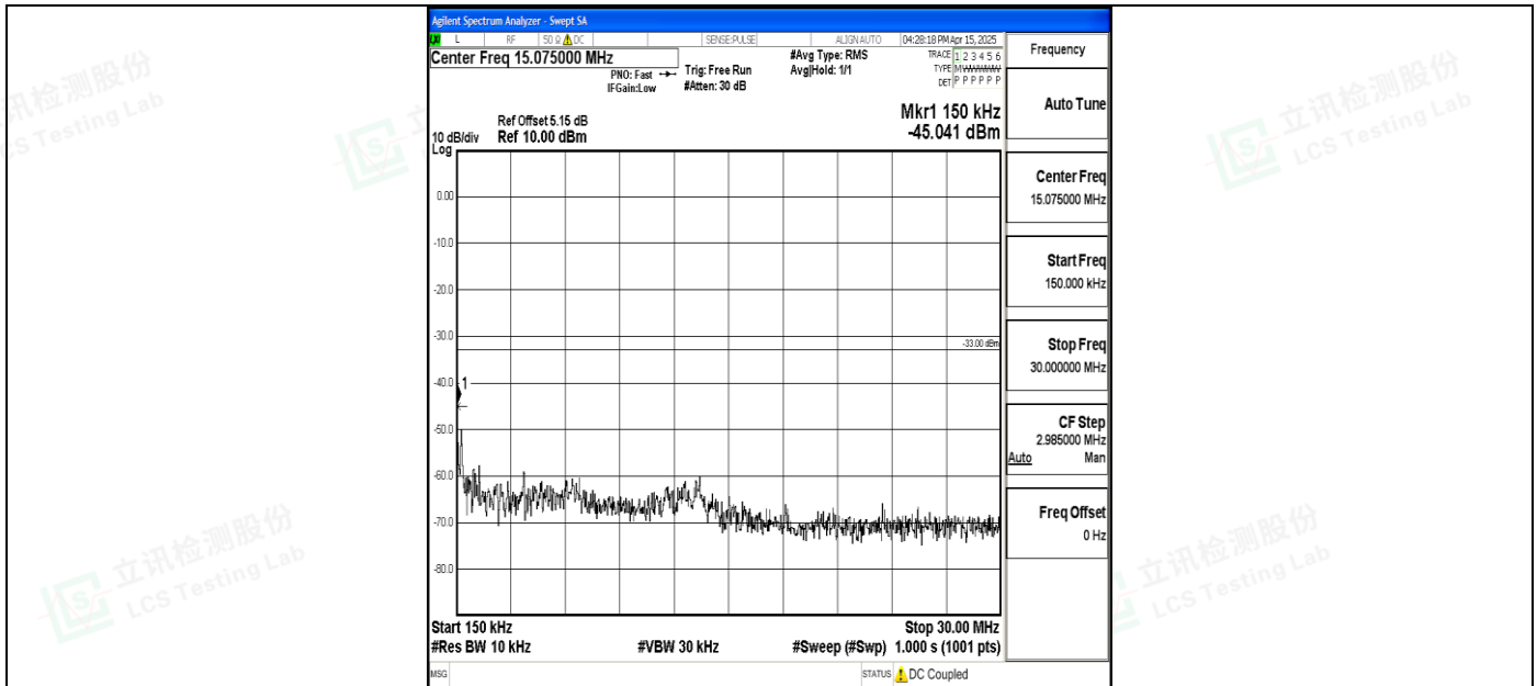
Band4_20MHz_16QAM_20175_1RB#0_0.15~30_0.15~30
