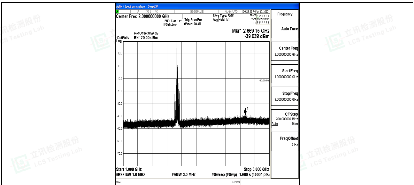
Band4_20MHz_16QAM_20300_1RB#0_1000~3000_1000~3000
