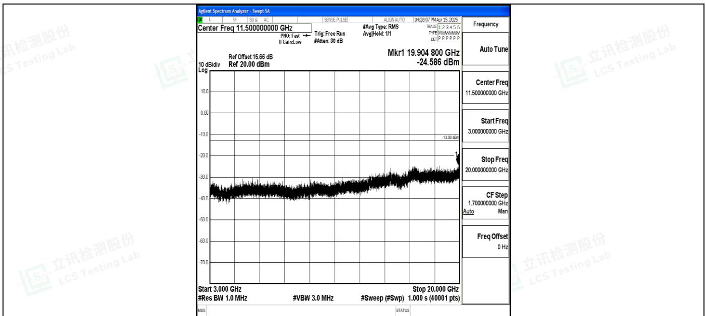
Band4_20MHz_QPSK_20175_1RB#0_3000~20000_3000~20000
