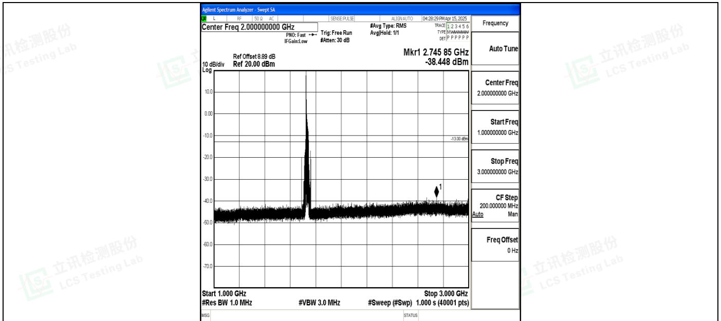
Band4_20MHz_16QAM_20175_1RB#0_1000~3000_1000~3000
