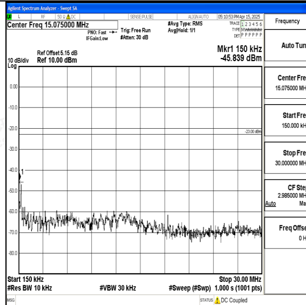
Band5_3MHz_QPSK_20525_1RB#0_0.15~30_0.15~30
