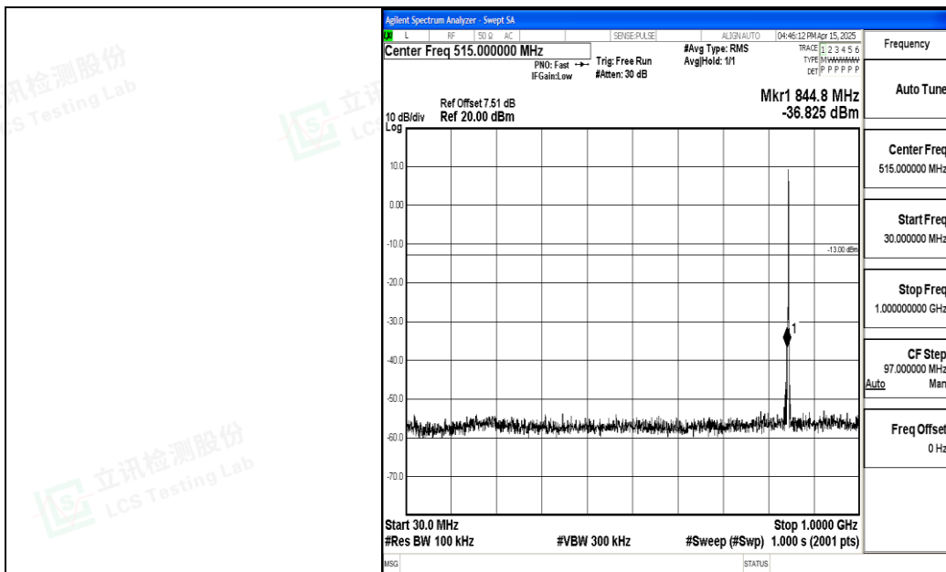
Band5_1.4MHz_QPSK_20643_1RB#0_30~1000_30~1000
