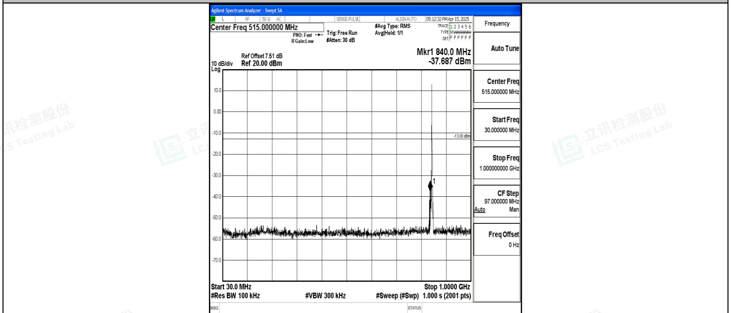
Band5_3MHz_16QAM_20635_1RB#0_30~1000_30~1000
