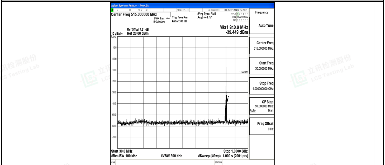
Band5_1.4MHz_16QAM_20525_1RB#0_30~1000_30~1000
