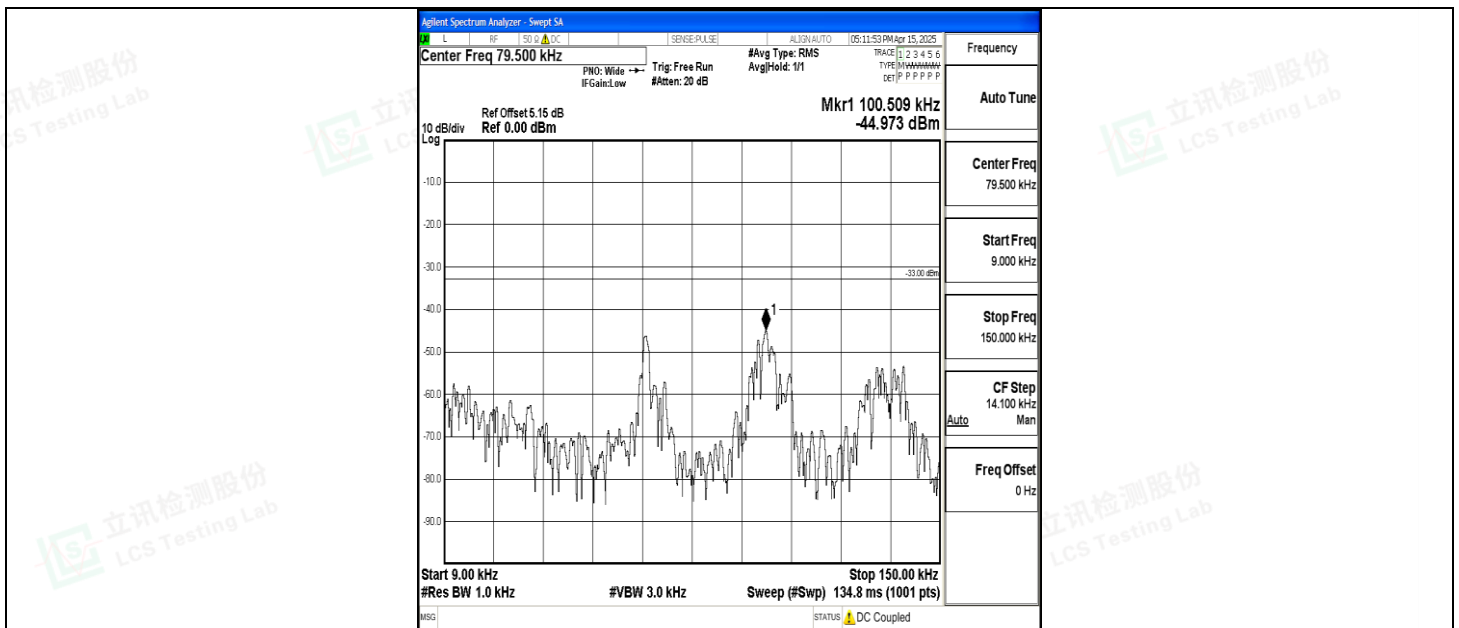
Band5_3MHz_QPSK_20635_1RB#0_0.009~0.15_0.009~0.15
