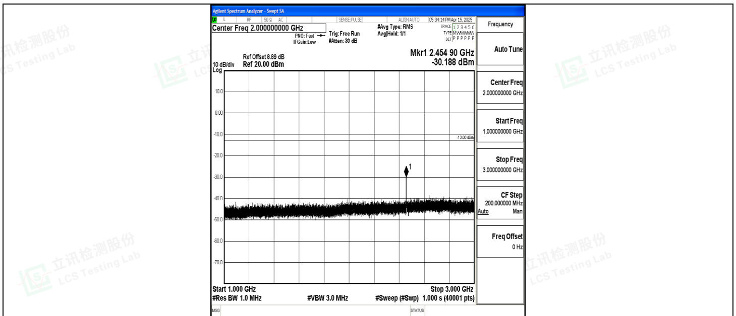
Band5_5MHz_16QAM_20625_1RB#0_1000~3000_1000~3000
