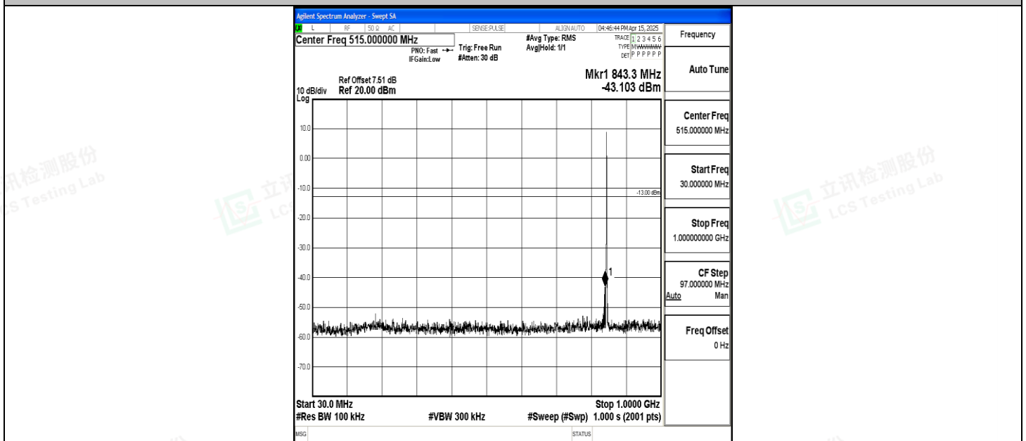
Band5_1.4MHz_16QAM_20643_1RB#0_30~1000_30~1000
