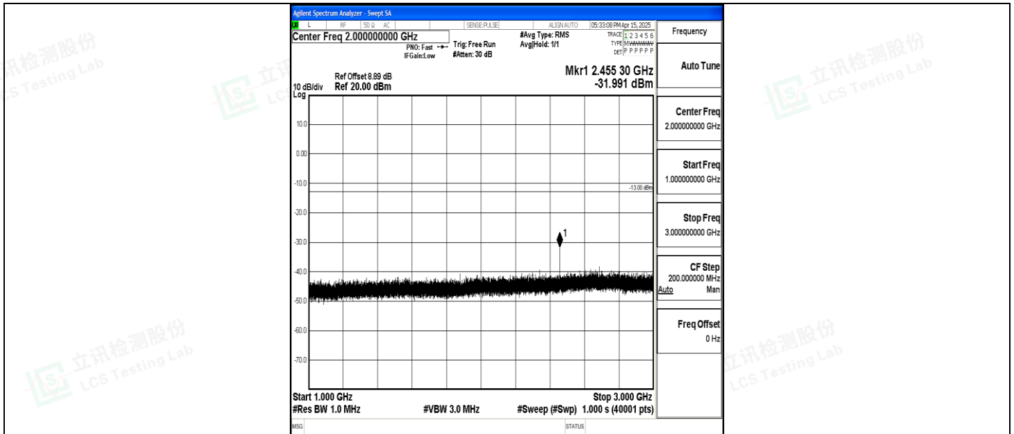
Band5_5MHz_16QAM_20525_1RB#0_1000~3000_1000~3000
