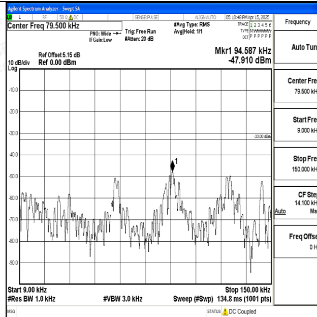
Band5_3MHz_QPSK_20525_1RB#0_0.009~0.15_0.009~0.15
