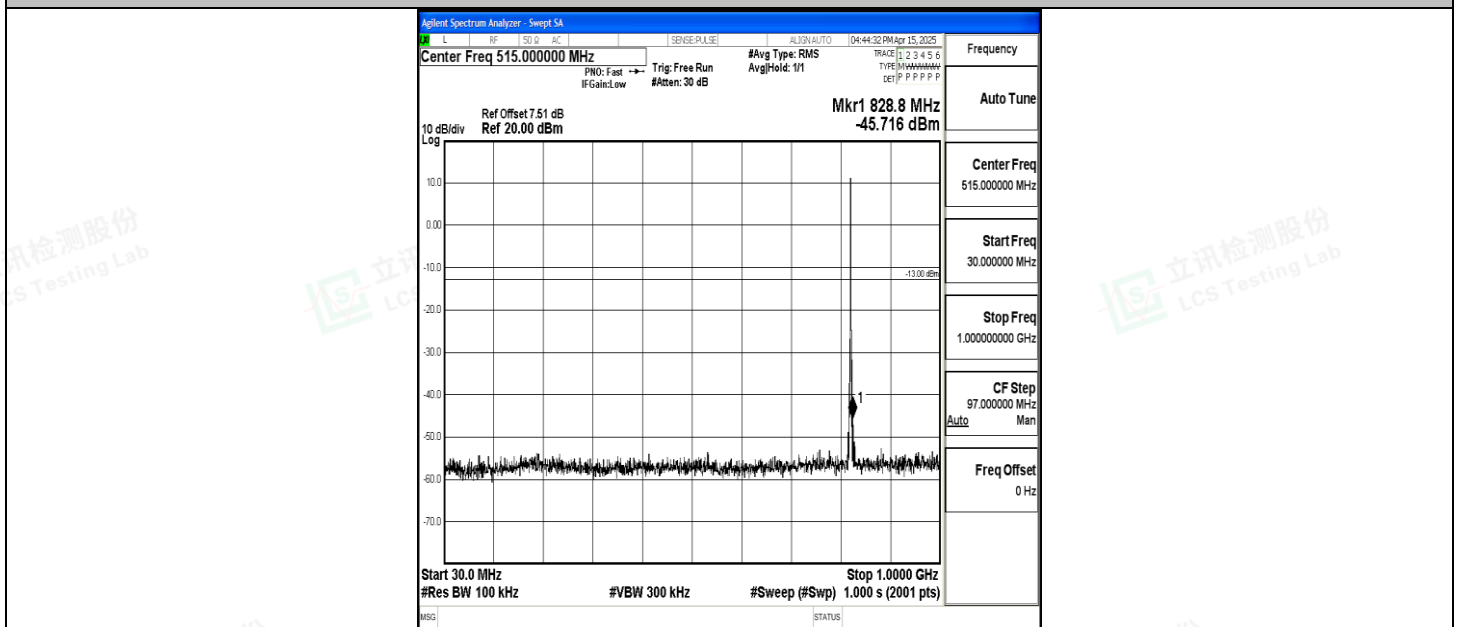
Band5_1.4MHz_16QAM_20407_1RB#0_30~1000_30~1000
