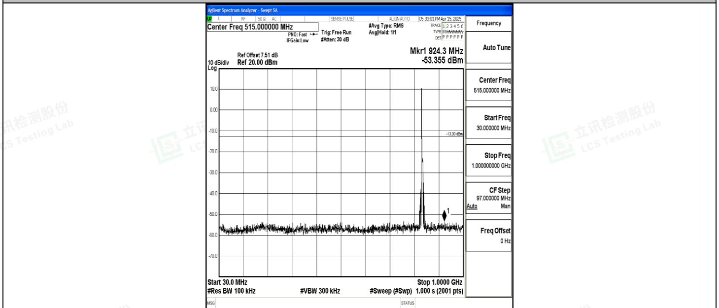
Band5_5MHz_16QAM_20525_1RB#0_30~1000_30~1000
