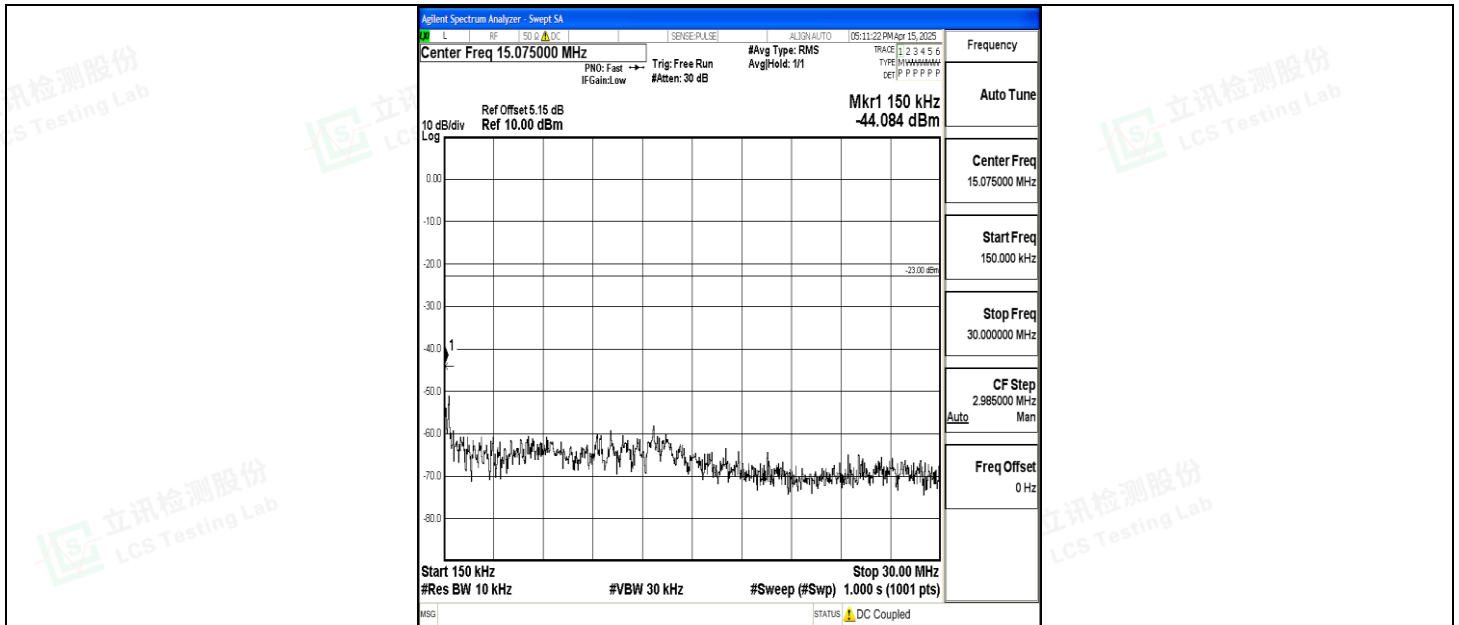
Band5_3MHz_16QAM_20525_1RB#0_0.15~30_0.15~30
