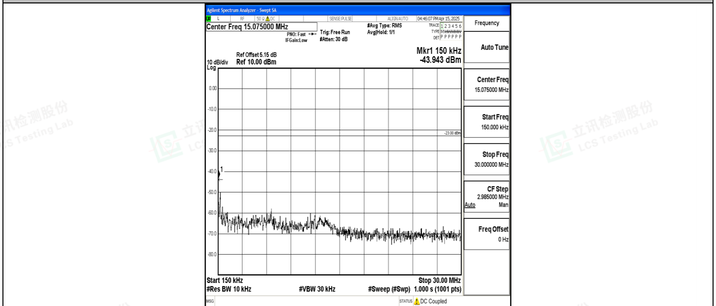
Band5_1.4MHz_QPSK_20643_1RB#0_0.15~30_0.15~30
