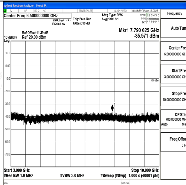
Band5_1.4MHz_16QAM_20643_1RB#0_3000~10000_3000~10000
