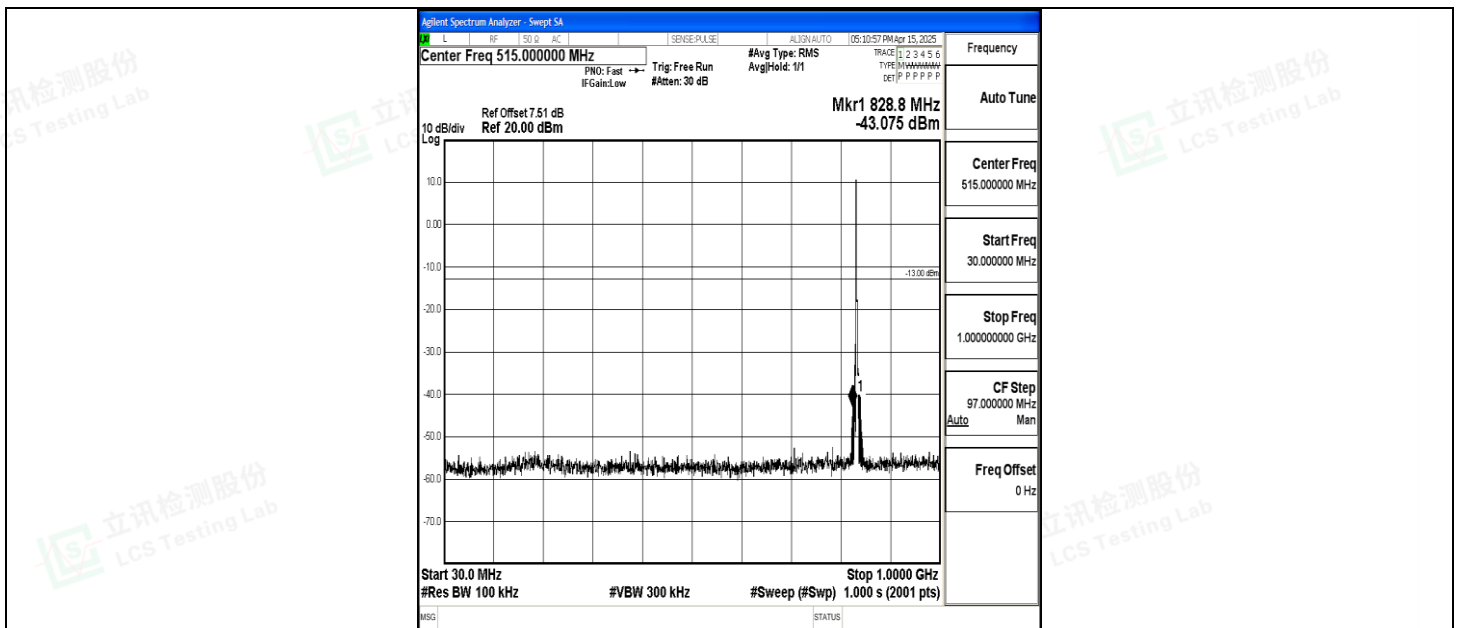
Band5_3MHz_QPSK_20525_1RB#0_30~1000_30~1000
