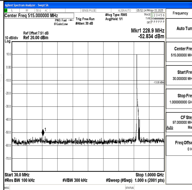
Band5_10MHz_16QAM_20450_1RB#0_30~1000_30~1000
