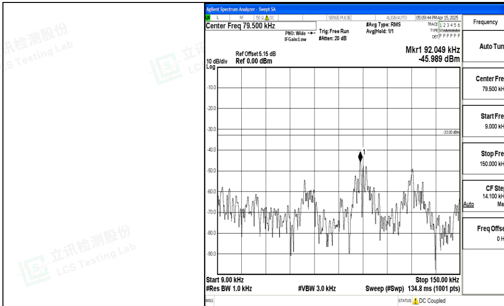
Band5_3MHz_QPSK_20415_1RB#0_0.009~0.15_0.009~0.15
