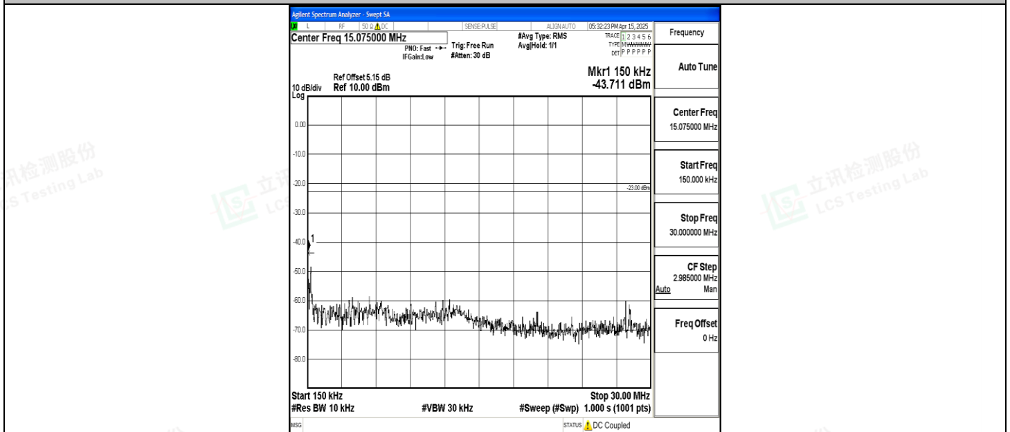
Band5_5MHz_QPSK_20525_1RB#0_0.15~30_0.15~30
