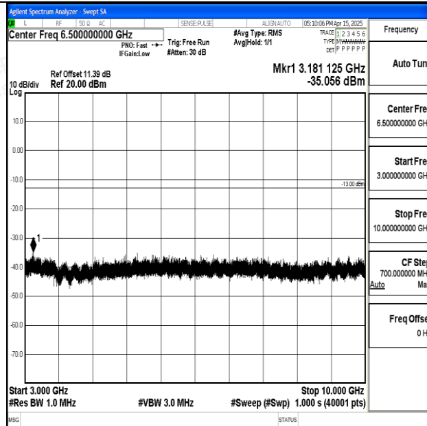
Band5_3MHz_QPSK_20415_1RB#0_3000~10000_3000~10000
