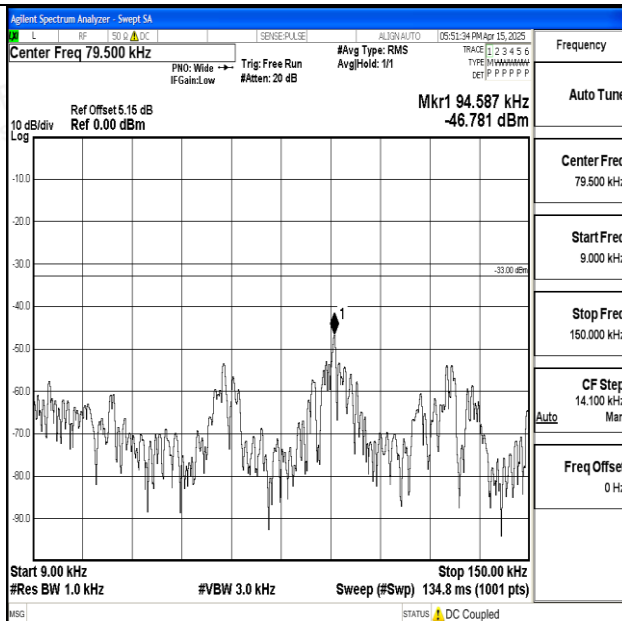
Band5_10MHz_QPSK_20450_1RB#0_0.009~0.15_0.009~0.15
