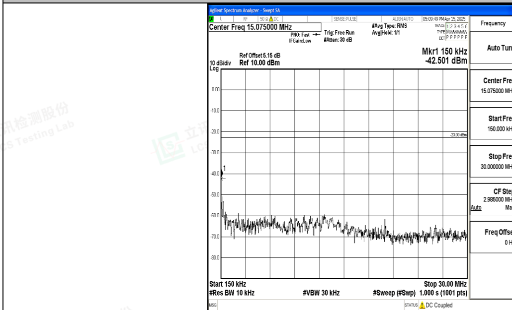
Band5_3MHz_QPSK_20415_1RB#0_0.15~30_0.15~30
