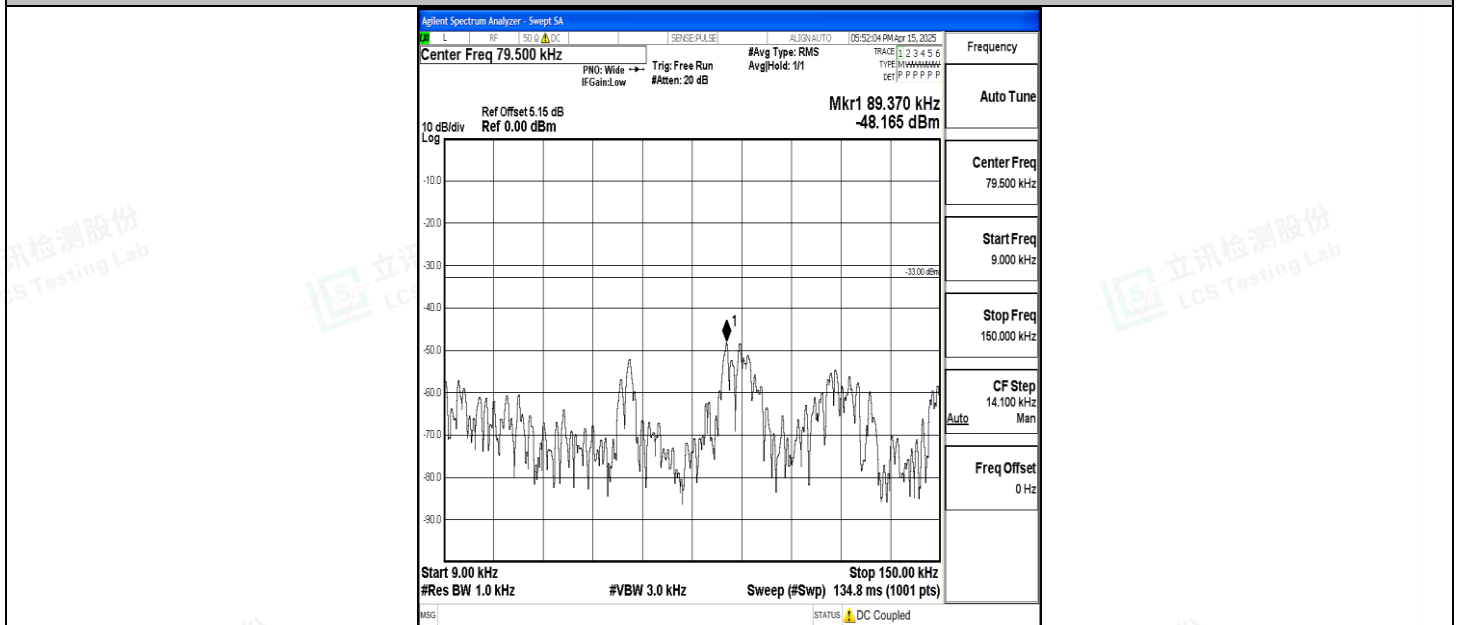
Band5_10MHz_16QAM_20450_1RB#0_0.009~0.15_0.009~0.15
