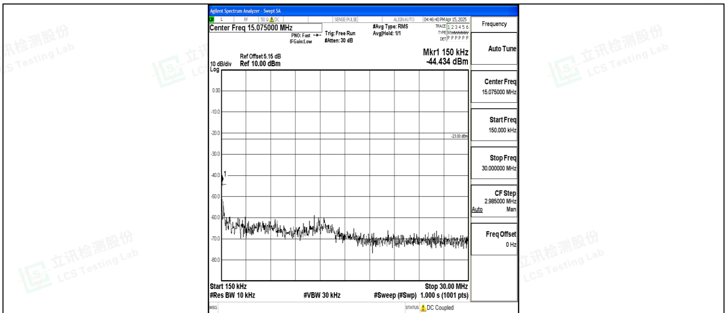
Band5_1.4MHz_16QAM_20643_1RB#0_0.15~30_0.15~30
