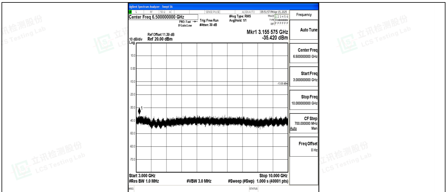
Band5_10MHz_QPSK_20450_1RB#0_3000~10000_3000~10000
