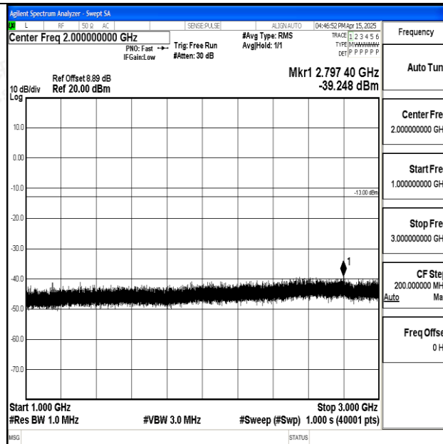
Band5_1.4MHz_16QAM_20643_1RB#0_1000~3000_1000~3000
