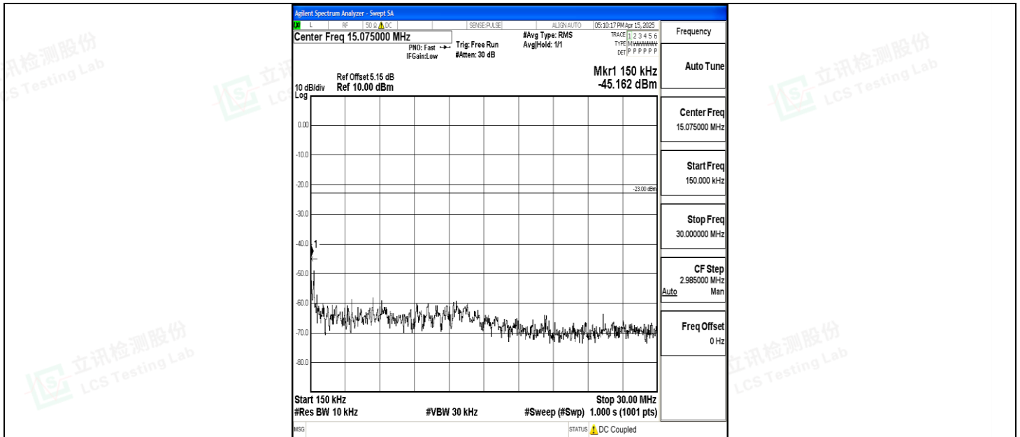
Band5_3MHz_16QAM_20415_1RB#0_0.15~30_0.15~30
