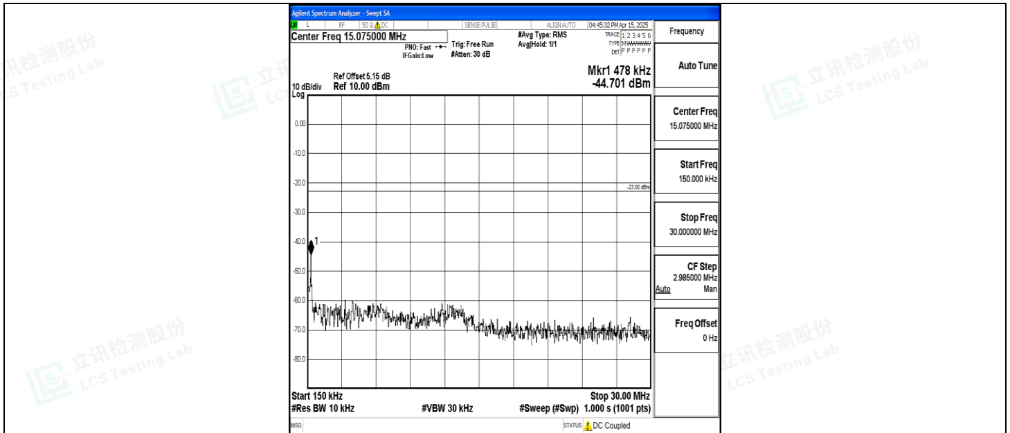
Band5_1.4MHz_16QAM_20525_1RB#0_0.15~30_0.15~30
