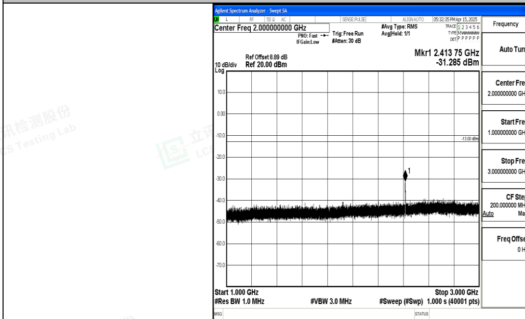
Band5_5MHz_QPSK_20525_1RB#0_1000~3000_1000~3000
