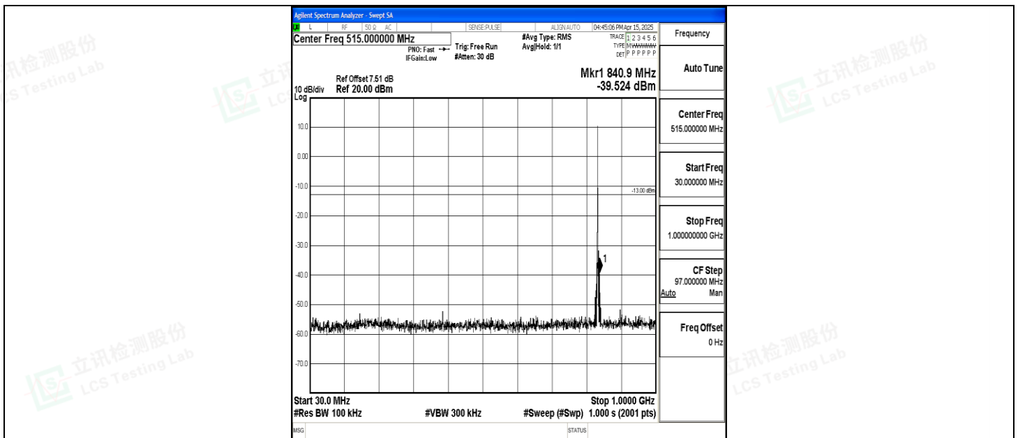
Band5_1.4MHz_QPSK_20525_1RB#0_30~1000_30~1000
