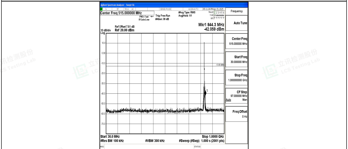
Band5_3MHz_16QAM_20525_1RB#0_30~1000_30~1000
