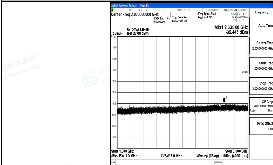
Band5_1.4MHz_QPSK_20643_1RB#0_1000~3000_1000~3000
