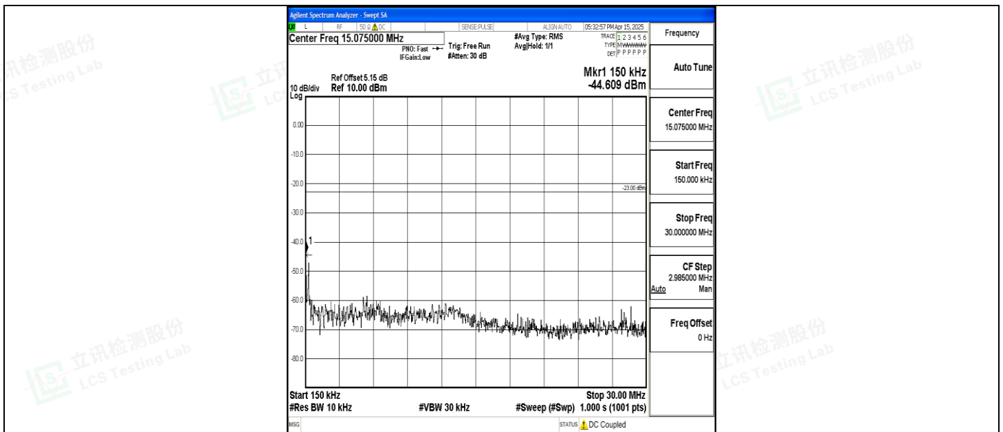
Band5_5MHz_16QAM_20525_1RB#0_0.15~30_0.15~30
