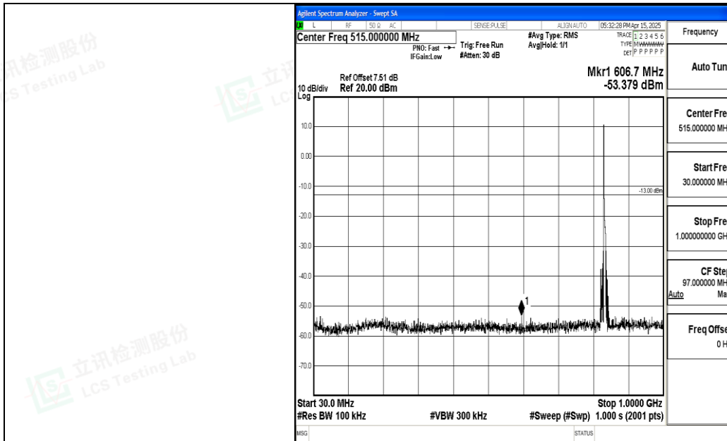
Band5_5MHz_QPSK_20525_1RB#0_30~1000_30~1000
