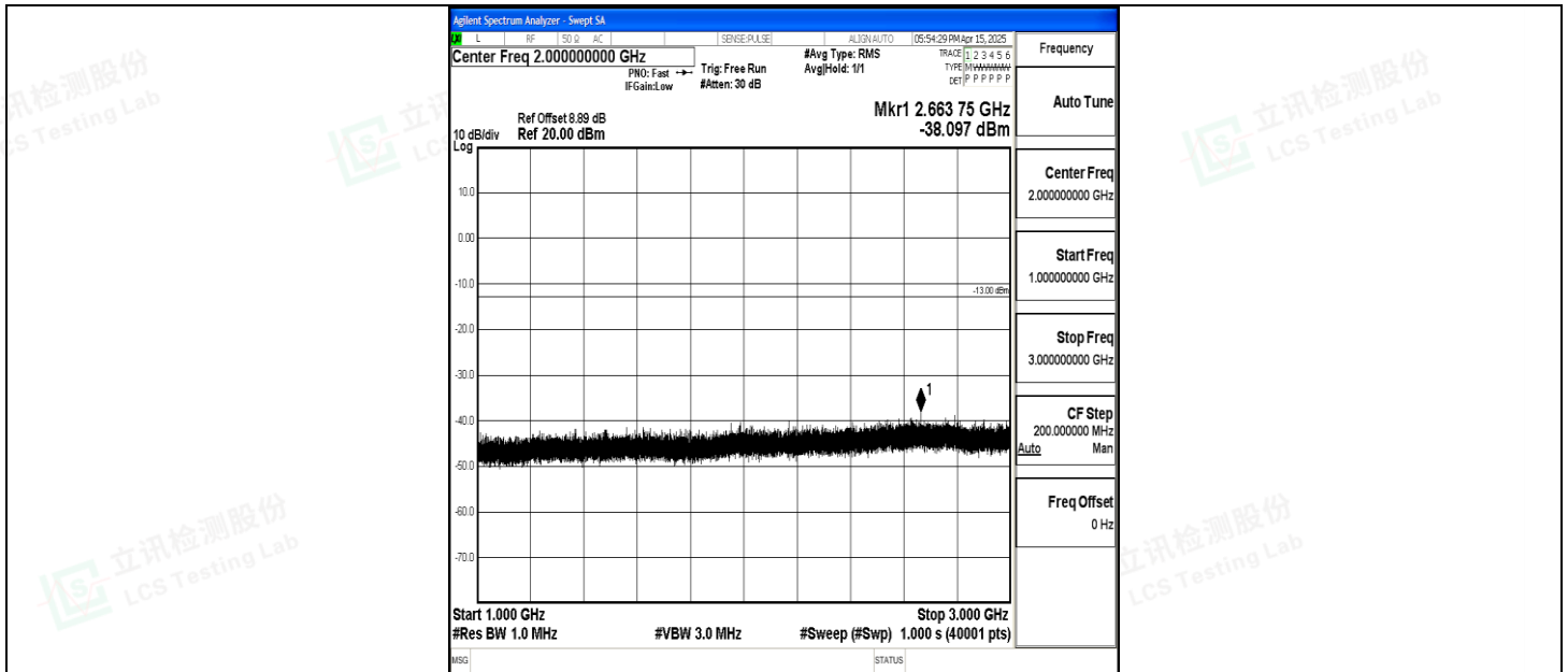
Band5_10MHz_16QAM_20600_1RB#0_1000~3000_1000~3000
