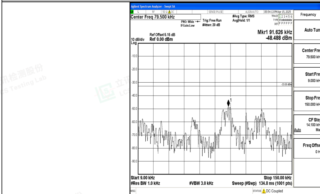
Band5_10MHz_16QAM_20600_1RB#0_0.009~0.15_0.009~0.15
