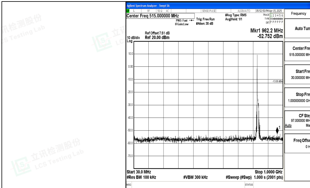
Band5_10MHz_QPSK_20525_1RB#0_30~1000_30~1000
