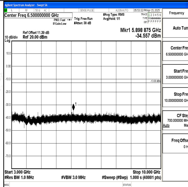
Band5_10MHz_16QAM_20525_1RB#0_3000~10000_3000~10000
