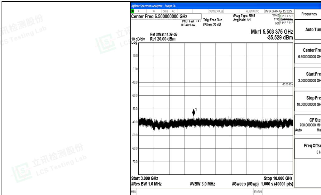
Band5_10MHz_QPSK_20600_1RB#0_3000~10000_3000~10000
