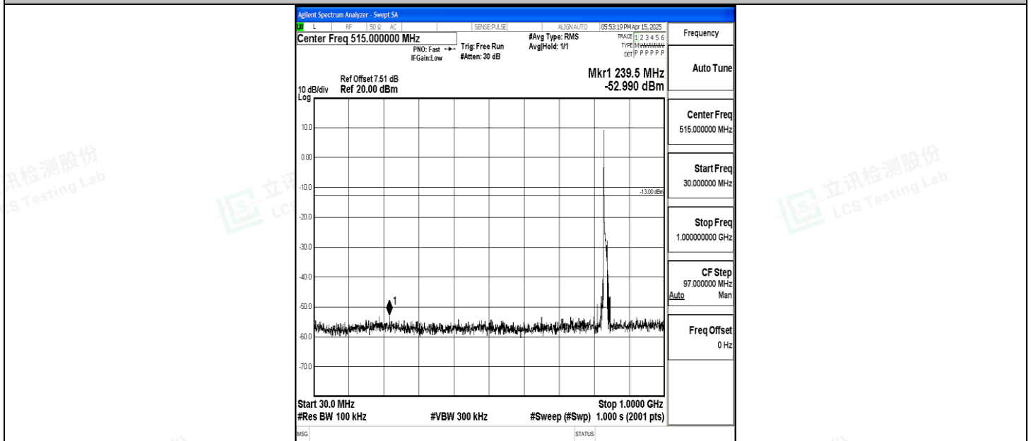
Band5_10MHz_16QAM_20525_1RB#0_30~1000_30~1000
