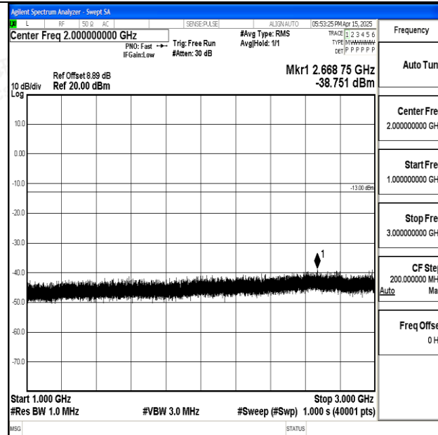
Band5_10MHz_16QAM_20525_1RB#0_1000~3000_1000~3000
