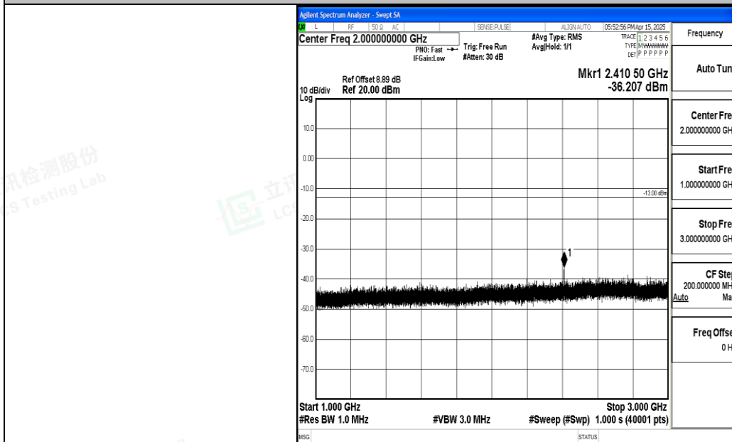
Band5_10MHz_QPSK_20525_1RB#0_1000~3000_1000~3000
