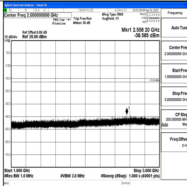
Band12_1.4MHz_16QAM_23095_1RB#0_1000~3000_1000~3000
