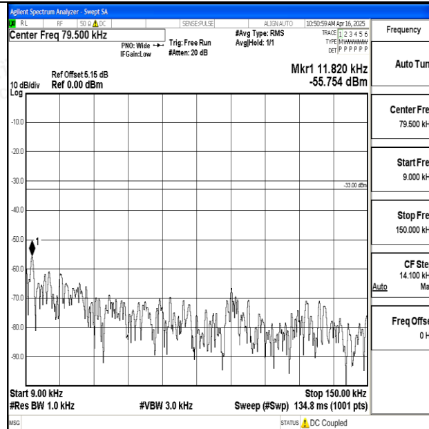
Band12_1.4MHz_QPSK_23095_1RB#0_0.009~0.15_0.009~0.15
