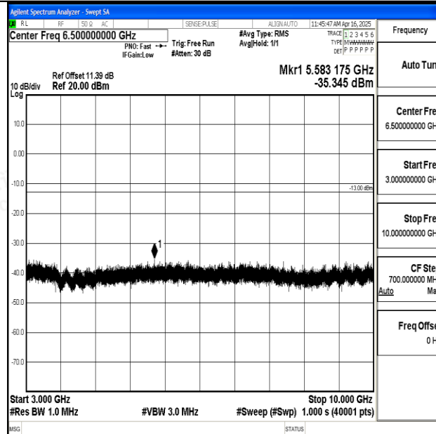
Band12_5MHz_16QAM_23035_1RB#0_3000~10000_3000~10000
