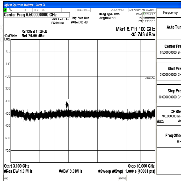
Band12_10MHz_QPSK_23060_1RB#0_3000~10000_3000~10000
