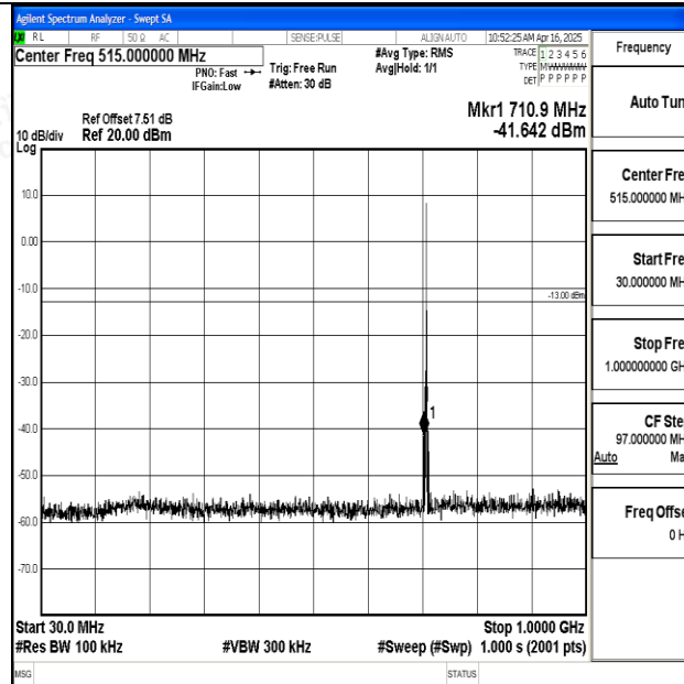
Band12_1.4MHz_QPSK_23173_1RB#0_30~1000_30~1000
