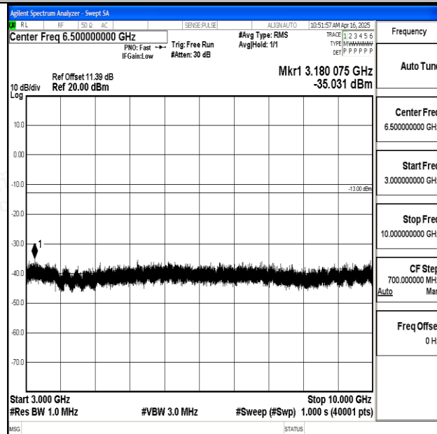
Band12_1.4MHz_16QAM_23095_1RB#0_3000~10000_3000~10000
