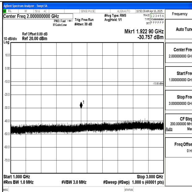
Band12_1.4MHz_16QAM_23017_1RB#0_1000~3000_1000~3000
