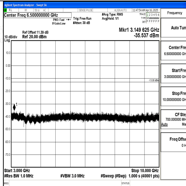
Band12_5MHz_QPSK_23155_1RB#0_3000~10000_3000~10000
