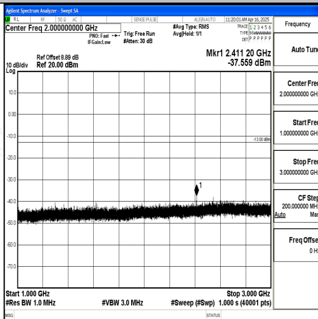
Band12_3MHz_QPSK_23165_1RB#0_1000~3000_1000~3000
