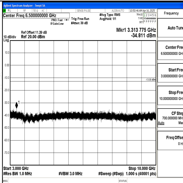
Band12_1.4MHz_16QAM_23017_1RB#0_3000~10000_3000~10000
