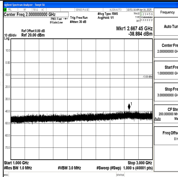
Band12_1.4MHz_QPSK_23095_1RB#0_1000~3000_1000~3000
