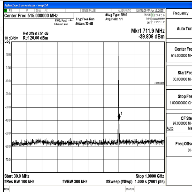
Band12_1.4MHz_QPSK_23095_1RB#0_30~1000_30~1000
