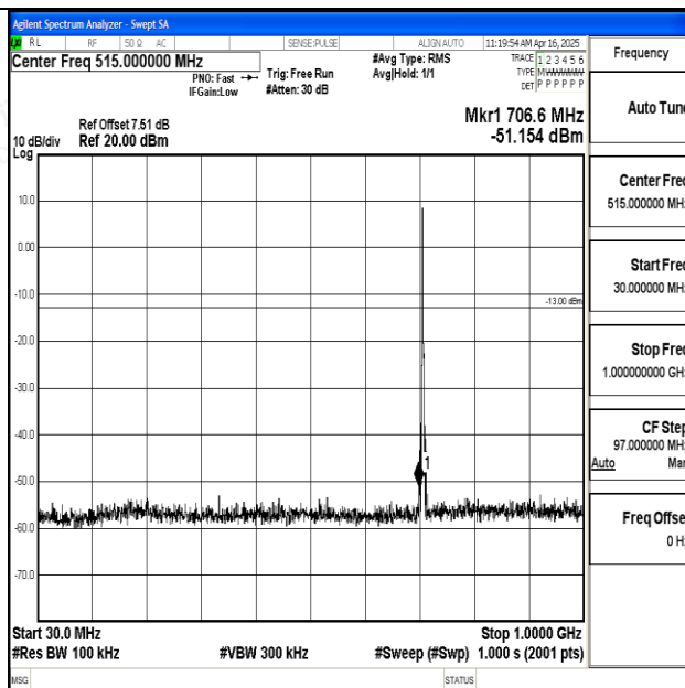
Band12_3MHz_QPSK_23165_1RB#0_30~1000_30~1000
