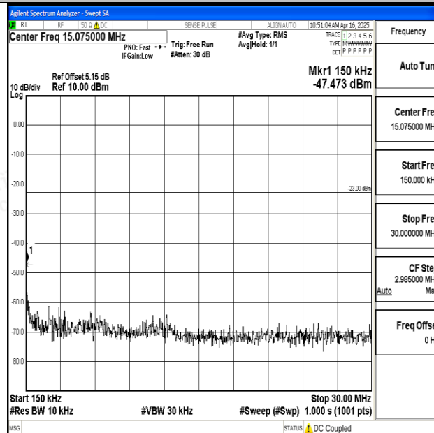
Band12_1.4MHz_QPSK_23095_1RB#0_0.15~30_0.15~30
