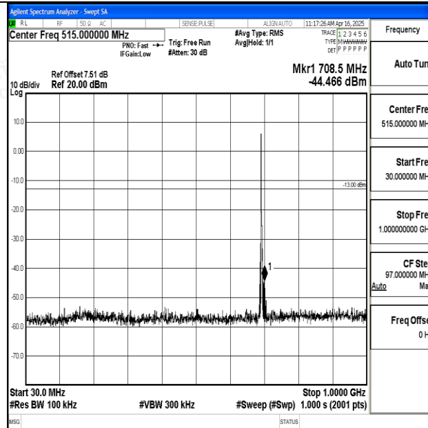
Band12_3MHz_QPSK_23025_1RB#0_30~1000_30~1000
