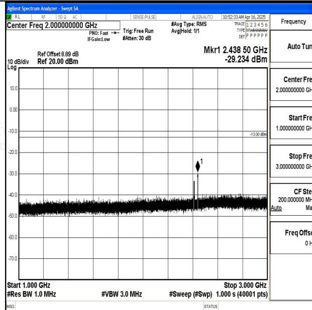
Band12_1.4MHz_QPSK_23173_1RB#0_1000~3000_1000~3000
