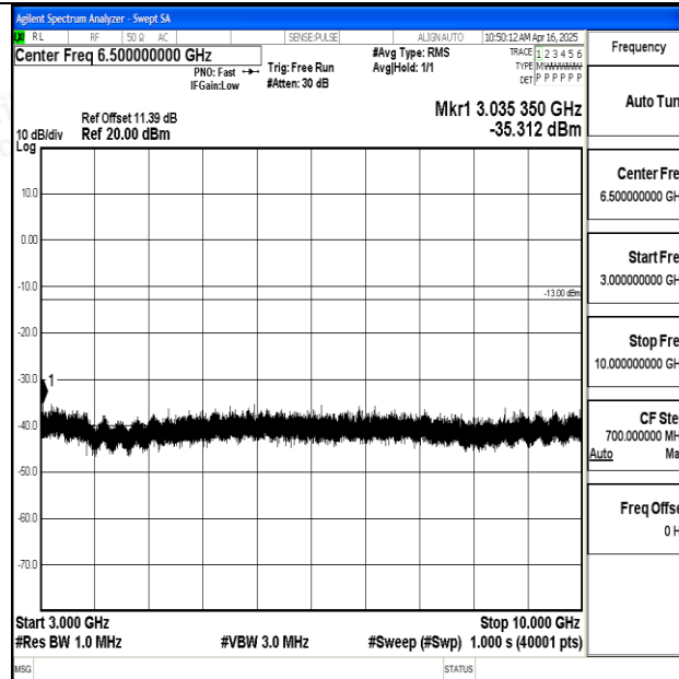
Band12_1.4MHz_QPSK_23017_1RB#0_3000~10000_3000~10000
