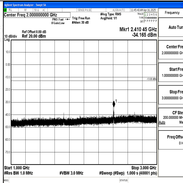
Band12_5MHz_16QAM_23035_1RB#0_1000~3000_1000~3000
