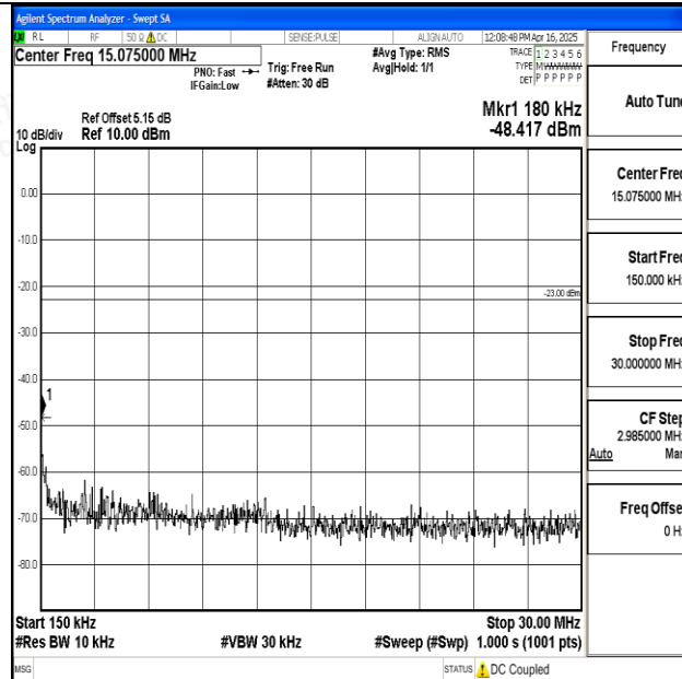
Band12_10MHz_16QAM_23095_1RB#0_0.15~30_0.15~30
