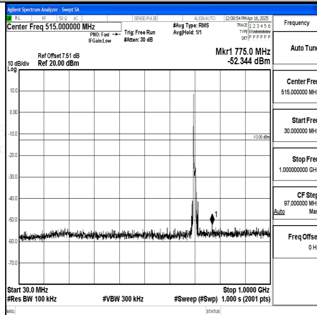
Band12_10MHz_16QAM_23095_1RB#0_30~1000_30~1000
