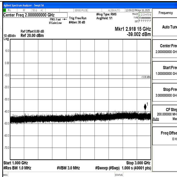
Band12_10MHz_16QAM_23095_1RB#0_1000~3000_1000~3000
