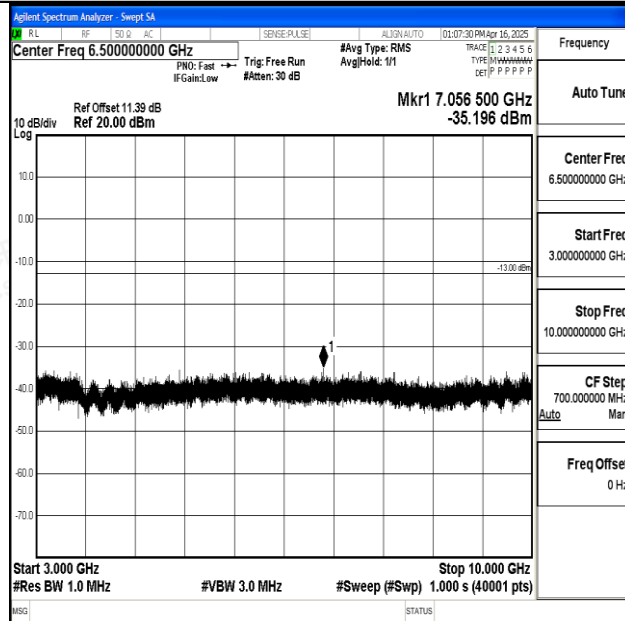
Band17_10MHz_QPSK_23790_1RB#0_3000~10000_3000~10000
