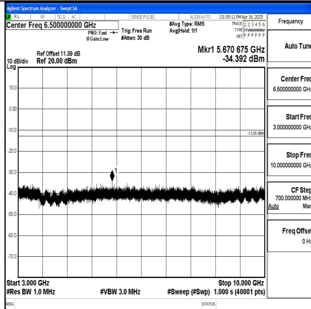
Band17_10MHz_16QAM_23800_1RB#0_3000~10000_3000~10000
