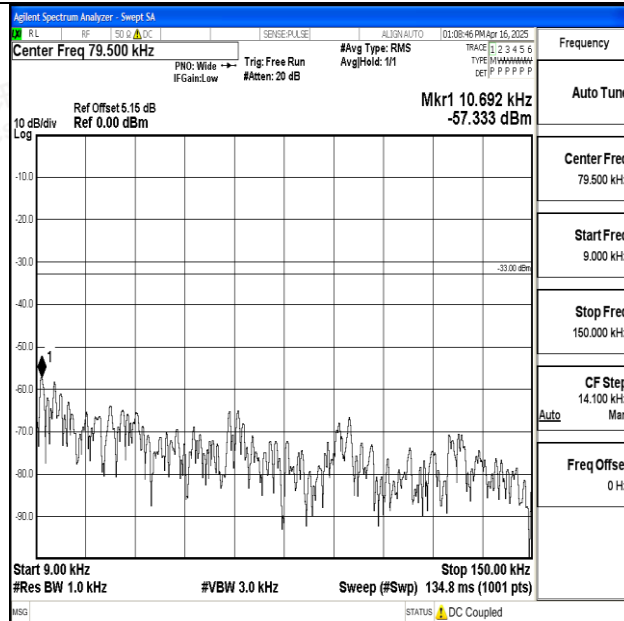
Band17_10MHz_16QAM_23800_1RB#0_0.009~0.15_0.009~0.15
