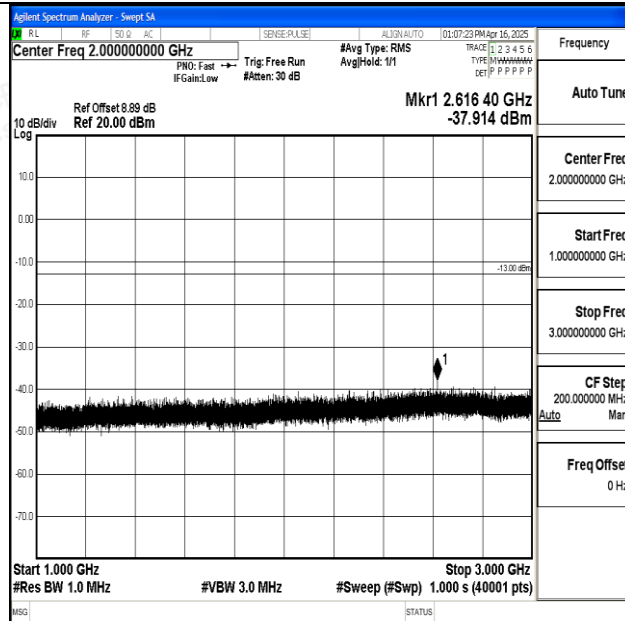
Band17_10MHz_QPSK_23790_1RB#0_1000~3000_1000~3000
