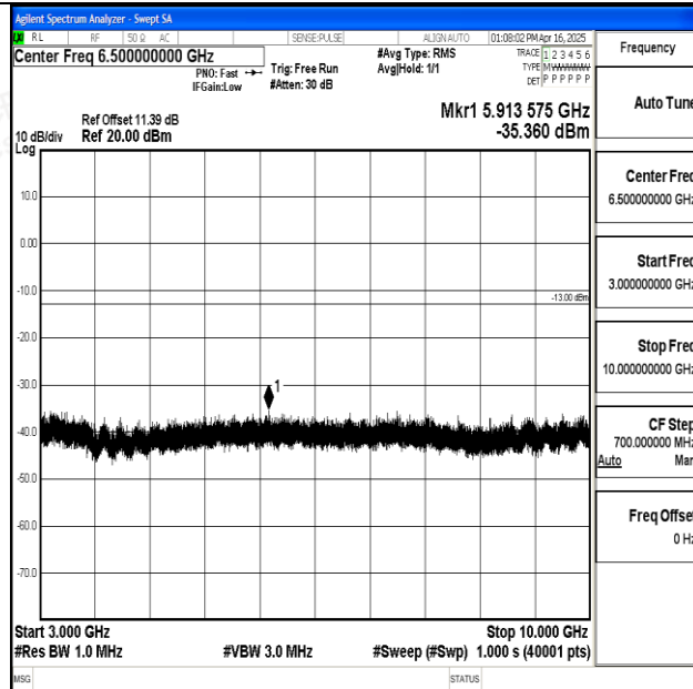
Band17_10MHz_16QAM_23790_1RB#0_3000~10000_3000~10000
