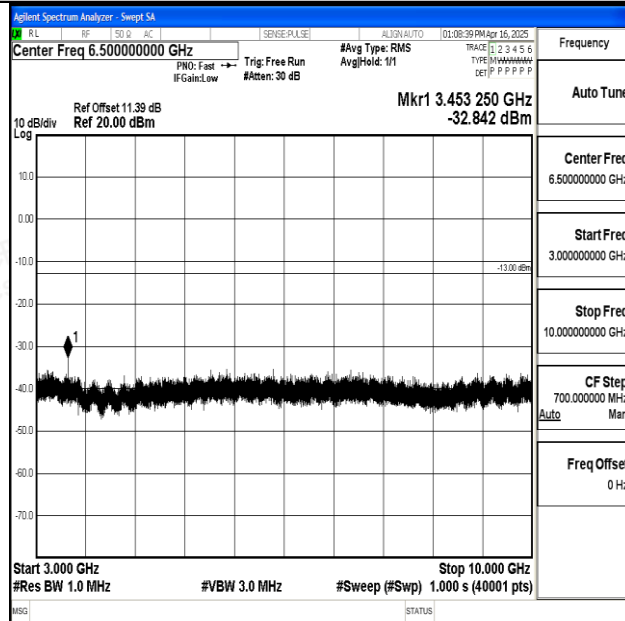
Band17_10MHz_QPSK_23800_1RB#0_3000~10000_3000~10000
