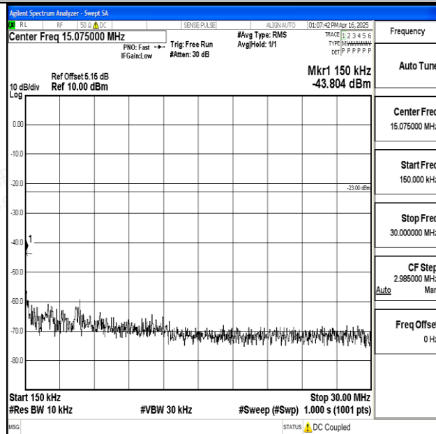
Band17_10MHz_16QAM_23790_1RB#0_0.15~30_0.15~30
