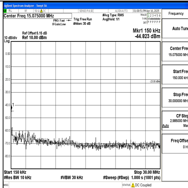
Band17_10MHz_16QAM_23800_1RB#0_0.15~30_0.15~30
