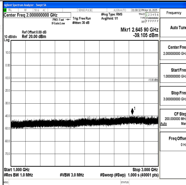
Band17_10MHz_QPSK_23800_1RB#0_1000~3000_1000~3000
