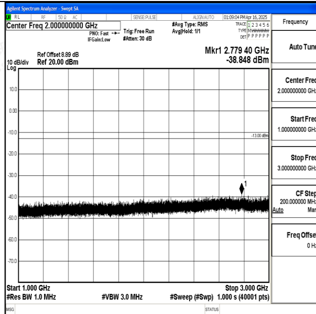
Band17_10MHz_16QAM_23800_1RB#0_1000~3000_1000~3000
