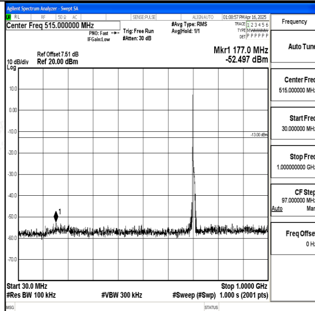
Band17_10MHz_16QAM_23800_1RB#0_30~1000_30~1000
