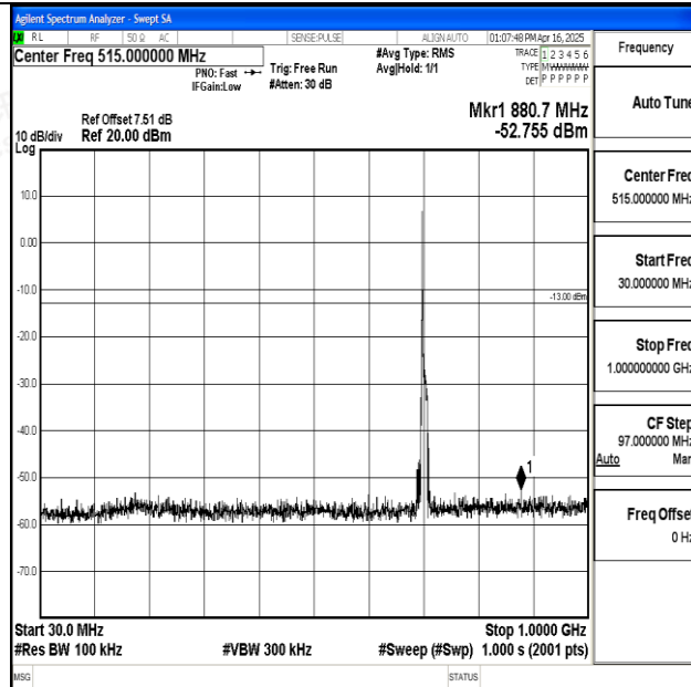
Band17_10MHz_16QAM_23790_1RB#0_30~1000_30~1000
