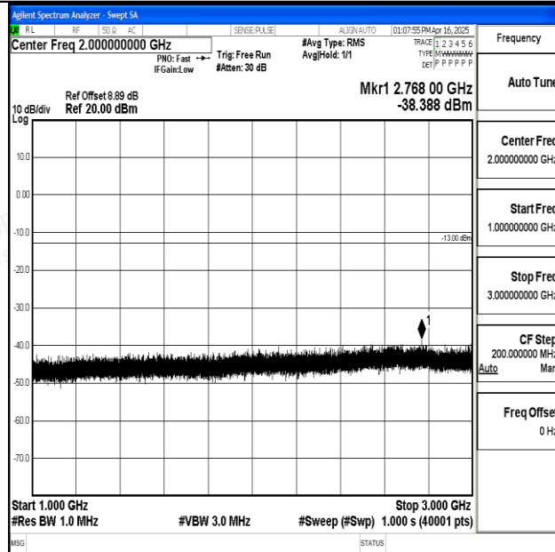
Band17_10MHz_16QAM_23790_1RB#0_1000~3000_1000~3000
