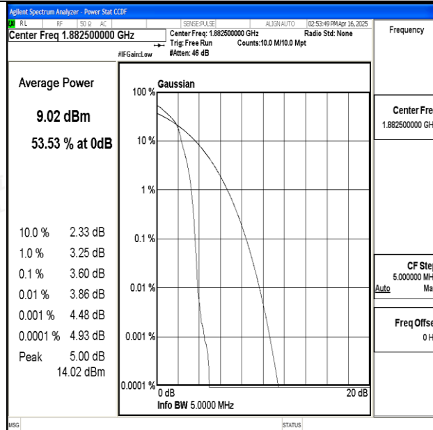
Band25-5MHz-16QAM-26365-1RB#0-PASS
