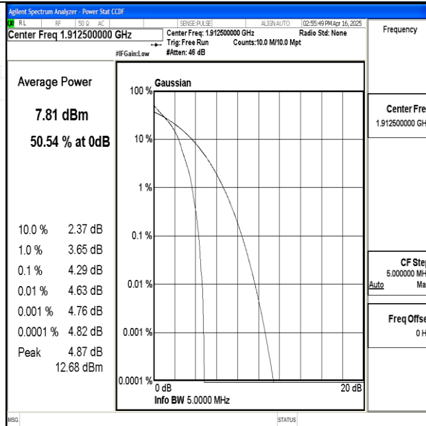
Band25-5MHz-QPSK-26665-1RB#0-PASS
