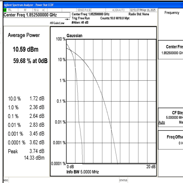
Band25-5MHz-QPSK-26065-1RB#0-PASS
