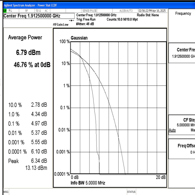
Band25-5MHz-16QAM-26665-1RB#0-PASS
