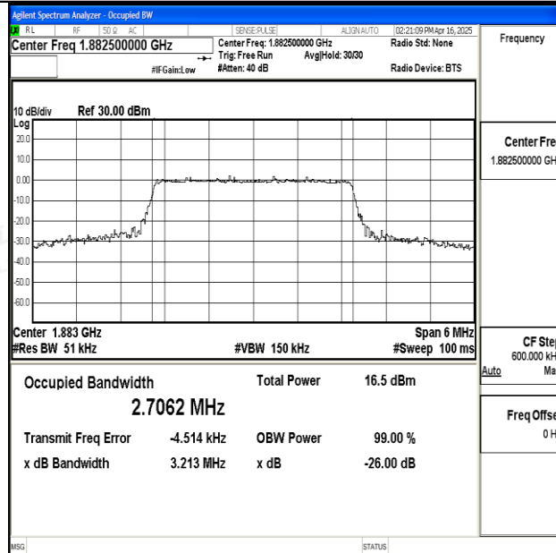
Band25-3MHz-16QAM-26365-15RB#0-PASS
