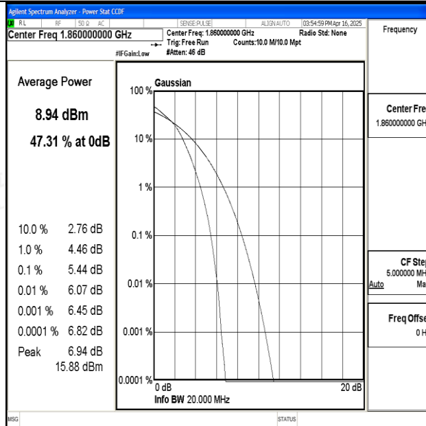
Band25-20MHz-16QAM-26140-100RB#0-PASS
