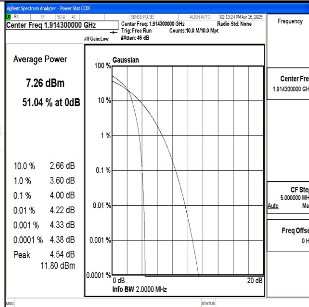
Band25-1.4MHz-16QAM-26683-1RB#0-PASS
