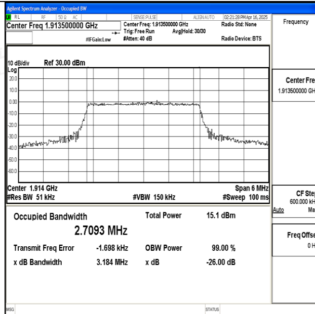
Band25-3MHz-QPSK-26675-15RB#0-PASS
