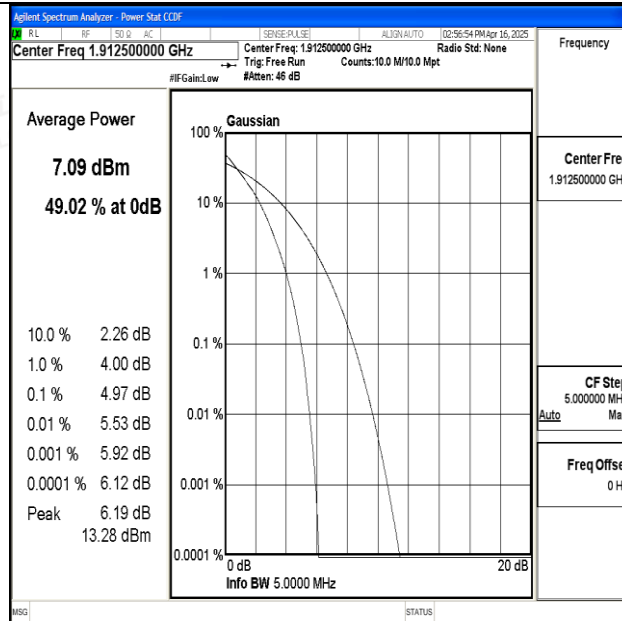
Band25-5MHz-QPSK-26665-25RB#0-PASS
