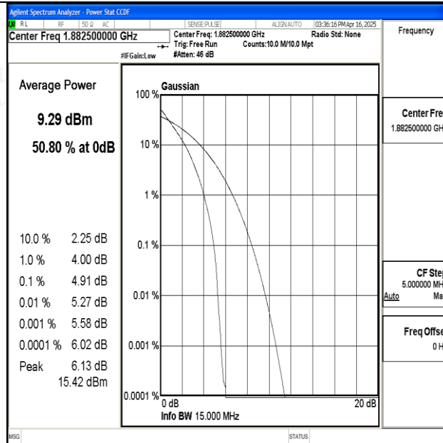
Band25-15MHz-QPSK-26365-75RB#0-PASS
