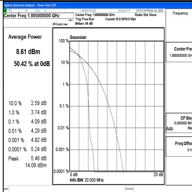
Band25-20MHz-16QAM-26590-1RB#0-PASS
