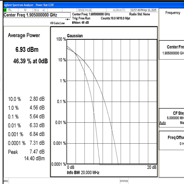
Band25-20MHz-16QAM-26590-100RB#0-PASS
