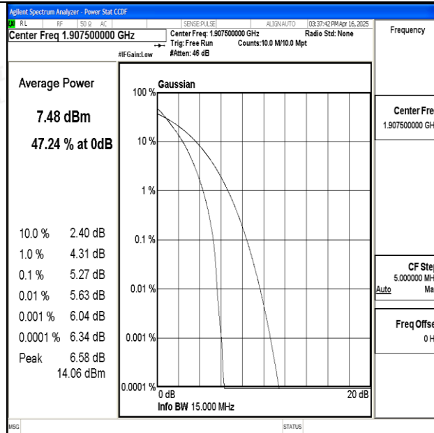
Band25-15MHz-QPSK-26615-75RB#0-PASS
