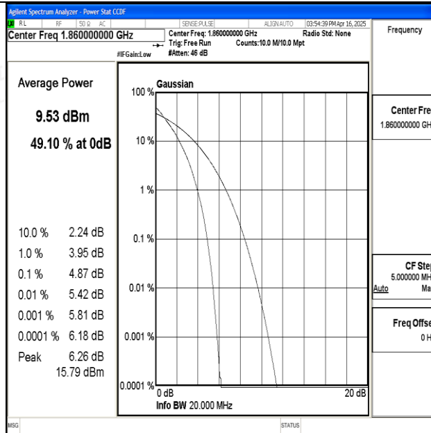
Band25-20MHz-QPSK-26140-100RB#0-PASS
