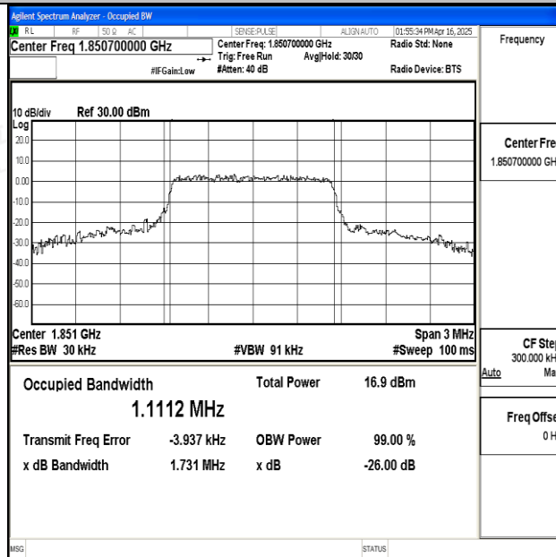
Band25-1.4MHz-16QAM-26047-6RB#0-PASS
