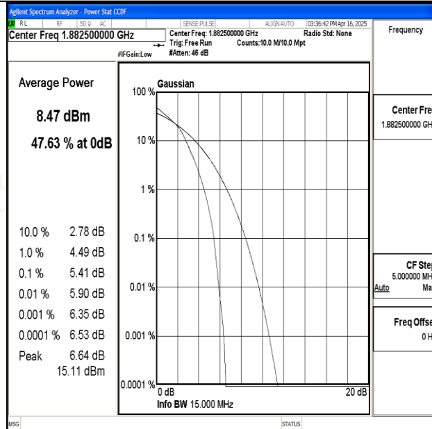
Band25-15MHz-16QAM-26365-75RB#0-PASS
