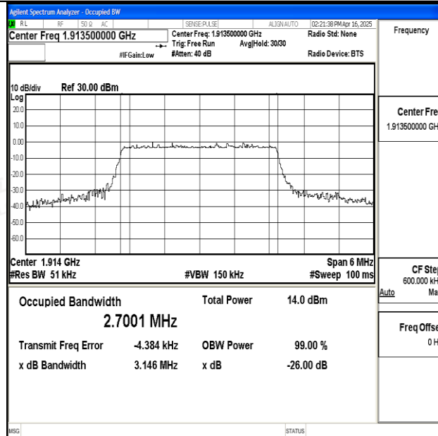
Band25-3MHz-16QAM-26675-15RB#0-PASS
