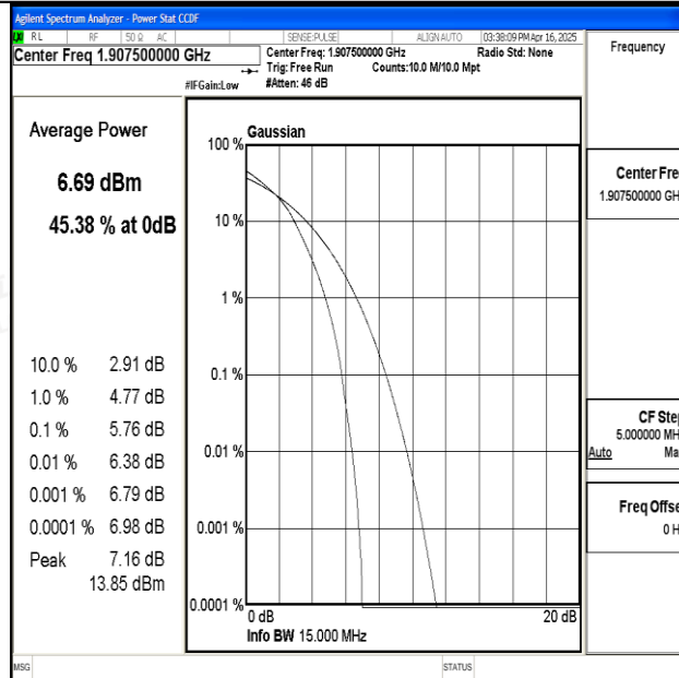
Band25-15MHz-16QAM-26615-75RB#0-PASS
