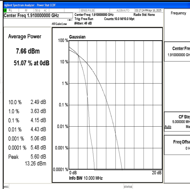
Band25-10MHz-16QAM-26640-1RB#0-PASS
