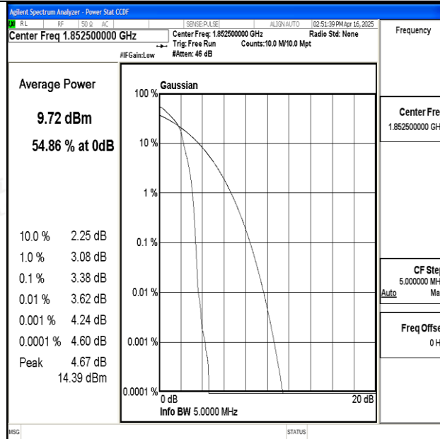
Band25-5MHz-16QAM-26065-1RB#0-PASS
