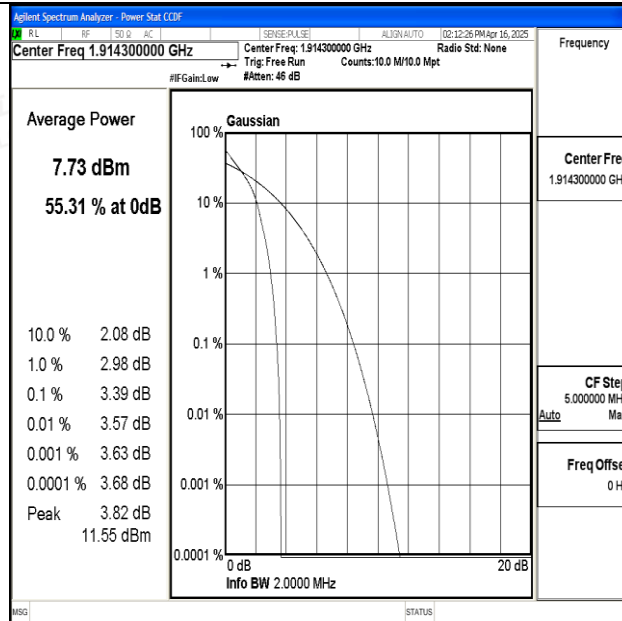
Band25-1.4MHz-QPSK-26683-1RB#0-PASS
