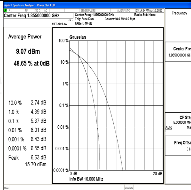
Band25-10MHz-16QAM-26090-50RB#0-PASS
