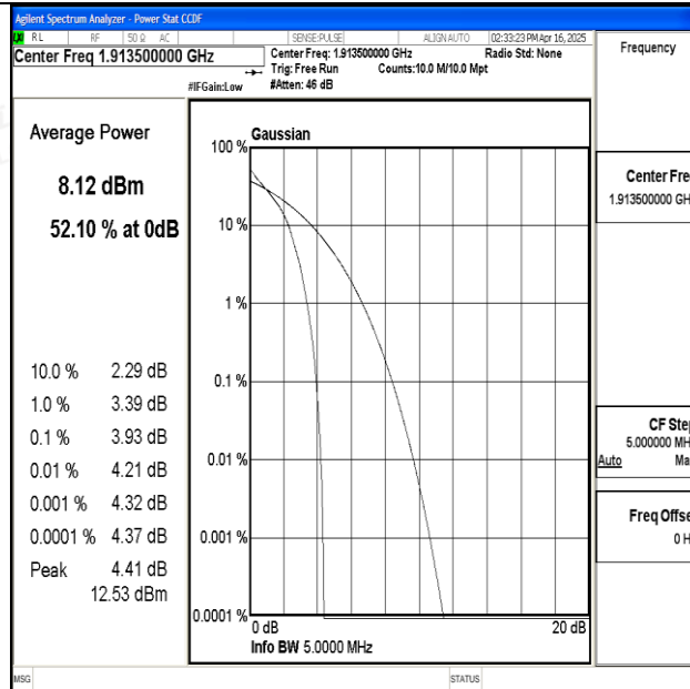
Band25-3MHz-QPSK-26675-1RB#0-PASS
