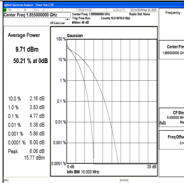
Band25-10MHz-QPSK-26090-50RB#0-PASS
