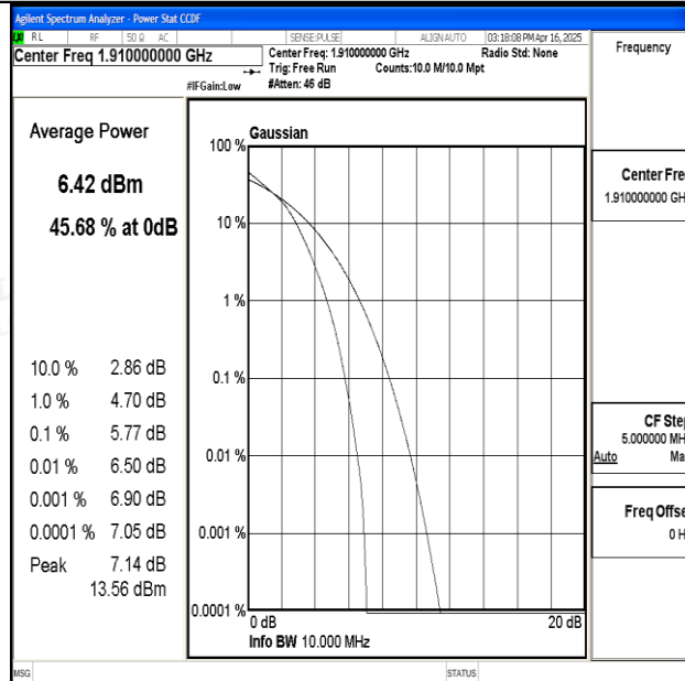
Band25-10MHz-16QAM-26640-50RB#0-PASS
