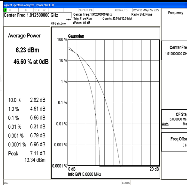
Band25-5MHz-16QAM-26665-25RB#0-PASS
