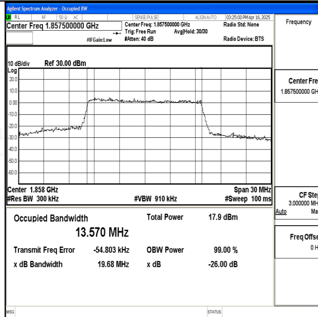
Band25-15MHz-16QAM-26115-75RB#0-PASS
