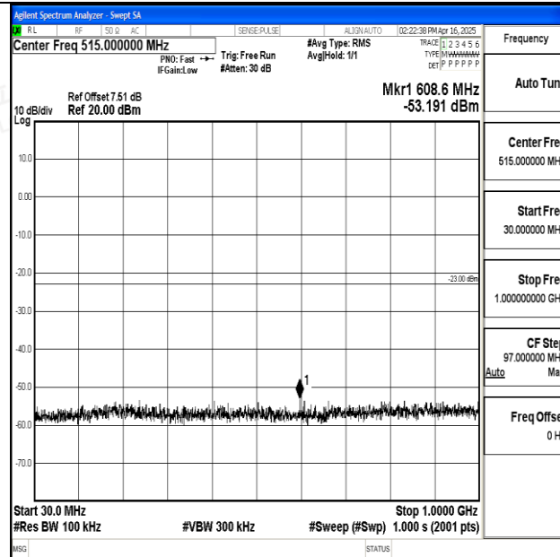
Band25_3MHz_QPSK_26055_1RB#0_30~1000_30~1000
