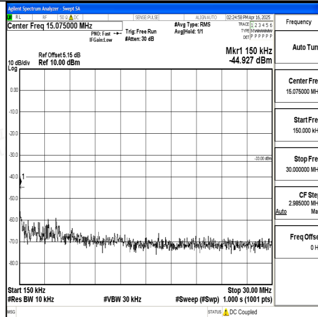
Band25_3MHz_QPSK_26675_1RB#0_0.15~30_0.15~30
