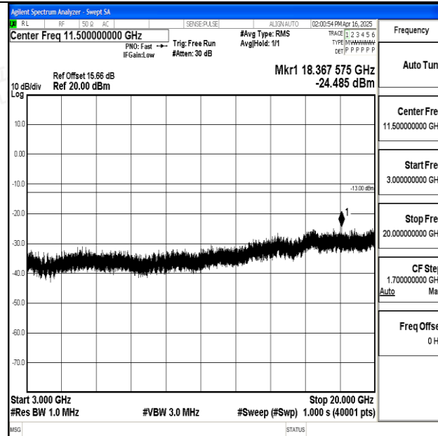
Band25_1.4MHz_QPSK_26683_1RB#0_3000~20000_3000~20000
