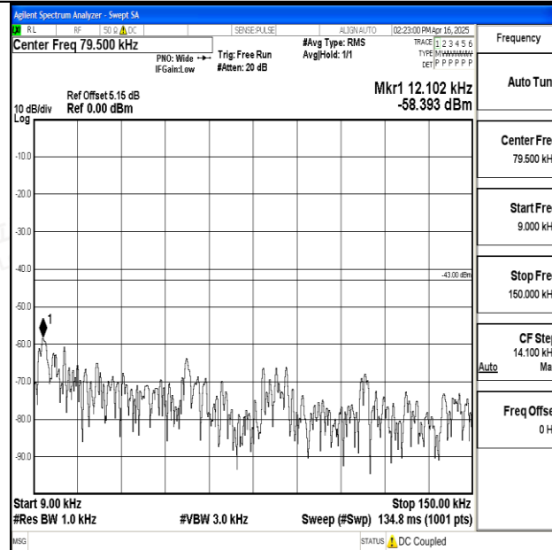
Band25_3MHz_16QAM_26055_1RB#0_0.009~0.15_0.009~0.15
