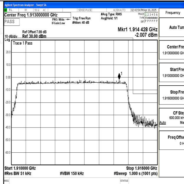
Band25_5MHz_QPSK_26665_25RB#0
