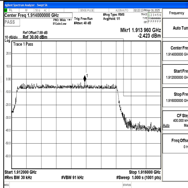
Band25_3MHz_16QAM_26675_15RB#0
