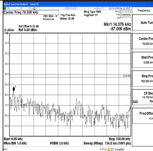
Band25_1.4MHz_16QAM_26683_1RB#0_0.009~0.15_0.009~0.15
