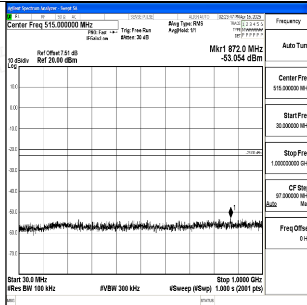
Band25_3MHz_QPSK_26365_1RB#0_30~1000_30~1000
