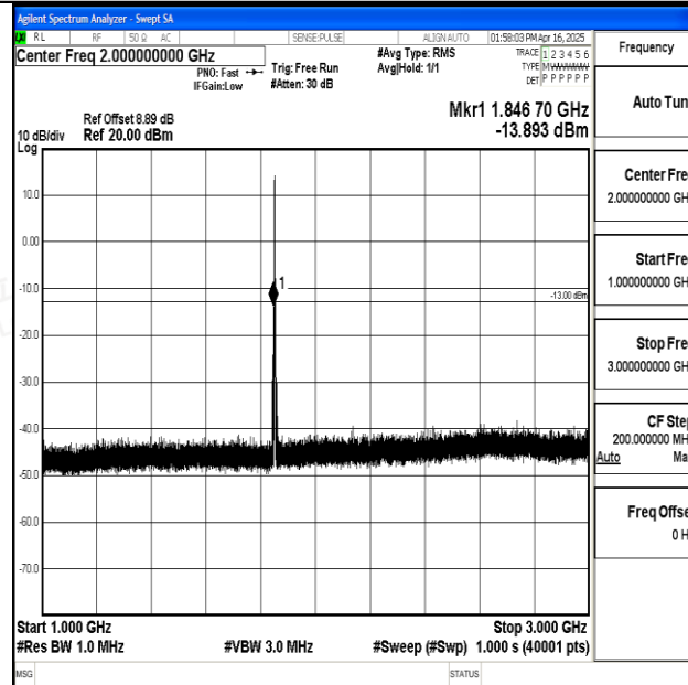
Band25_1.4MHz_QPSK_26047_1RB#0_1000~3000_1000~3000
