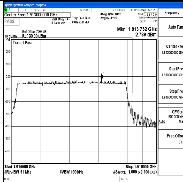
Band25_5MHz_16QAM_26665_25RB#0
