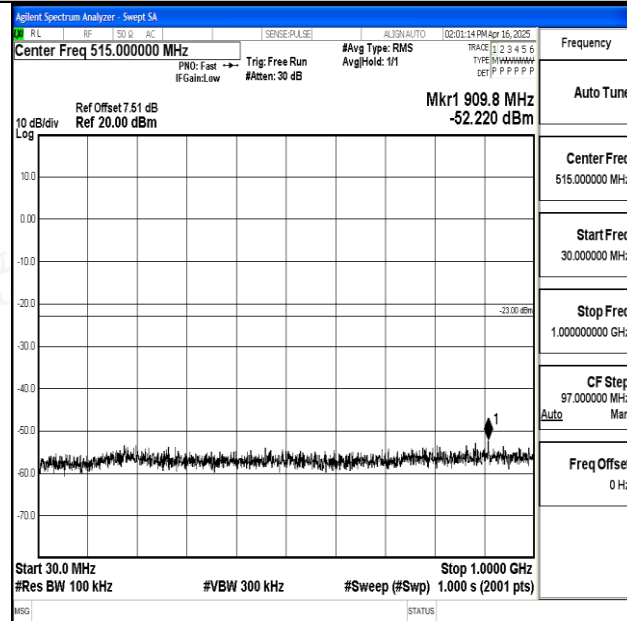
Band25_1.4MHz_16QAM_26683_1RB#0_30~1000_30~1000
