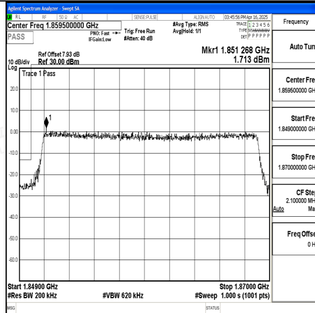
Band25_20MHz_16QAM_26140_100RB#0
