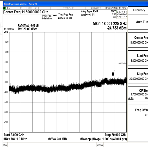
Band25_3MHz_QPSK_26055_1RB#0_3000~20000_3000~20000
