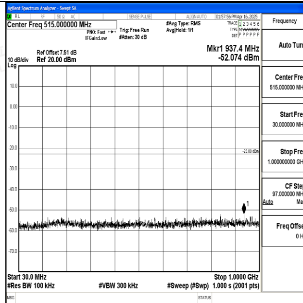
Band25_1.4MHz_QPSK_26047_1RB#0_30~1000_30~1000
