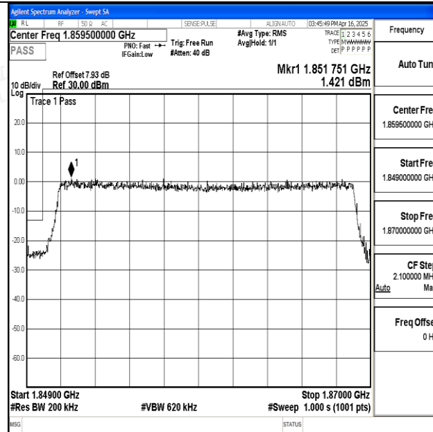
Band25_20MHz_QPSK_26140_100RB#0
