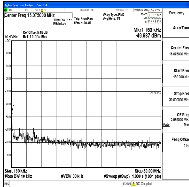
Band25_1.4MHz_16QAM_26683_1RB#0_0.15~30_0.15~30
