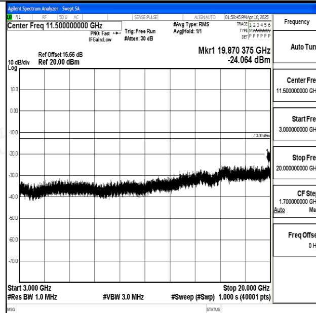
Band25_1.4MHz_16QAM_26047_1RB#0_3000~20000_3000~20000
