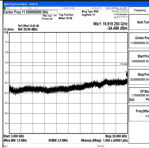
Band25_1.4MHz_16QAM_26683_1RB#0_3000~20000_3000~20000
