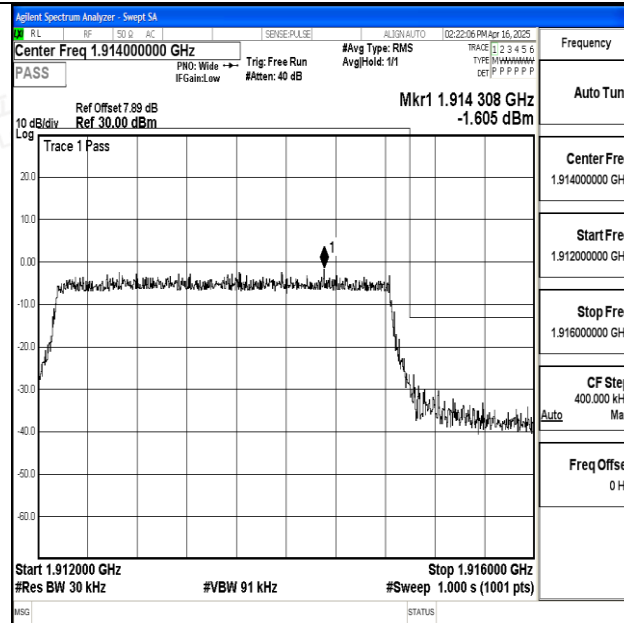
Band25_3MHz_QPSK_26675_15RB#0
