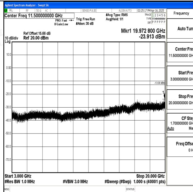
Band25_3MHz_QPSK_26675_1RB#0_3000~20000_3000~20000
