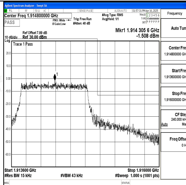
Band25_1.4MHz_16QAM_26683_6RB#0
