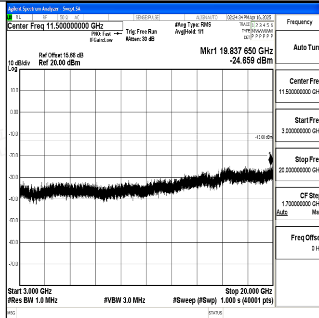
Band25_3MHz_16QAM_26365_1RB#0_3000~20000_3000~20000
