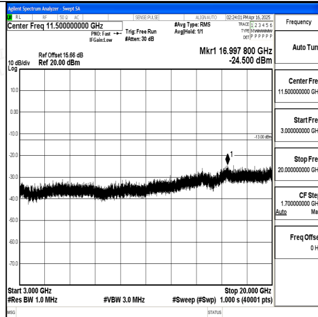
Band25_3MHz_QPSK_26365_1RB#0_3000~20000_3000~20000
