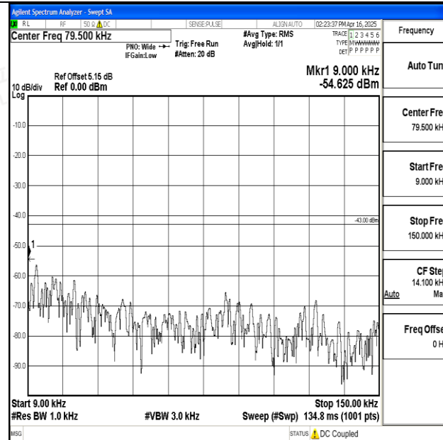
Band25_3MHz_QPSK_26365_1RB#0_0.009~0.15_0.009~0.15
