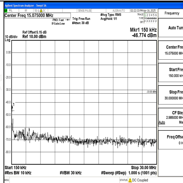
Band25_3MHz_QPSK_26055_1RB#0_0.15~30_0.15~30
