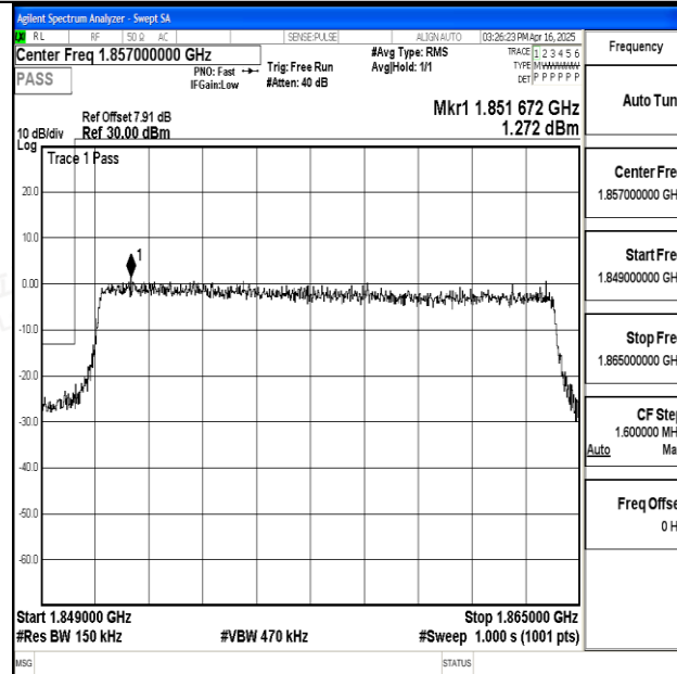
Band25_15MHz_16QAM_26115_75RB#0
