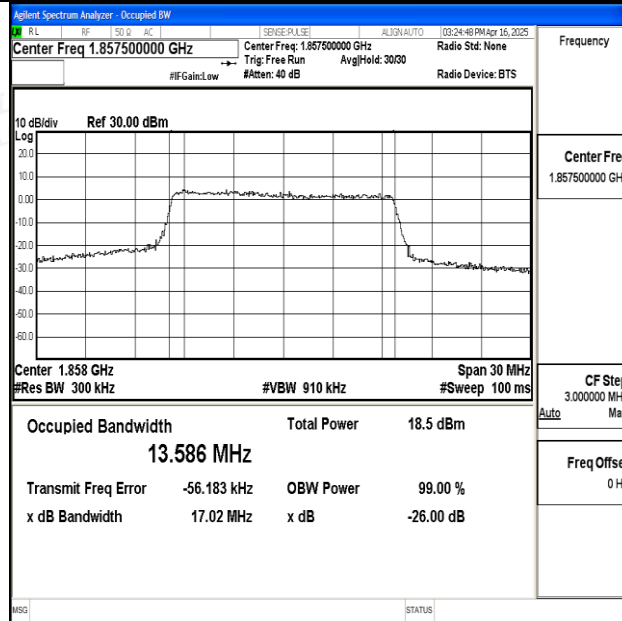
Band25-15MHz-QPSK-26115-75RB#0-PASS
