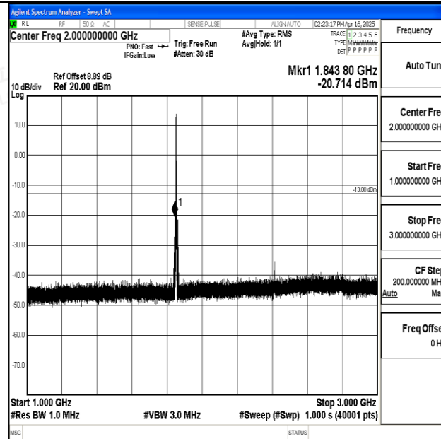
Band25_3MHz_16QAM_26055_1RB#0_1000~3000_1000~3000
