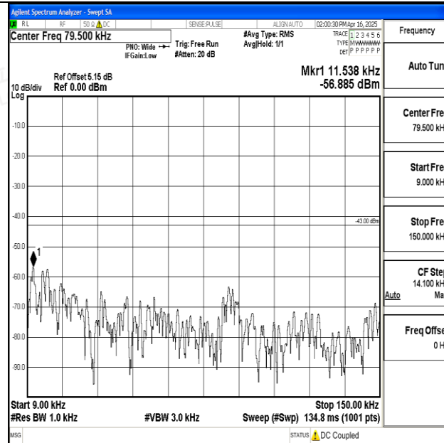
Band25_1.4MHz_QPSK_26683_1RB#0_0.009~0.15_0.009~0.15
