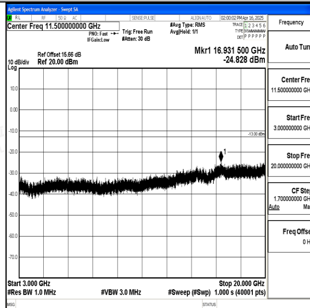
Band25_1.4MHz_16QAM_26365_1RB#0_3000~20000_3000~20000
