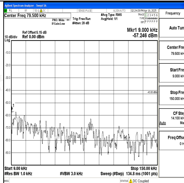
Band25_3MHz_16QAM_26365_1RB#0_0.009~0.15_0.009~0.15
