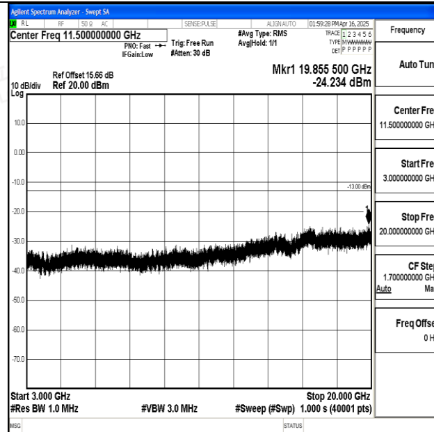
Band25_1.4MHz_QPSK_26365_1RB#0_3000~20000_3000~20000
