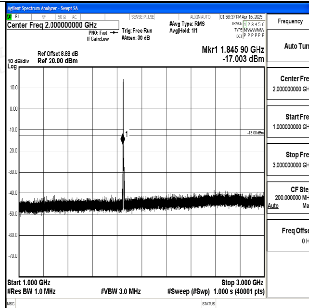
Band25_1.4MHz_16QAM_26047_1RB#0_1000~3000_1000~3000
