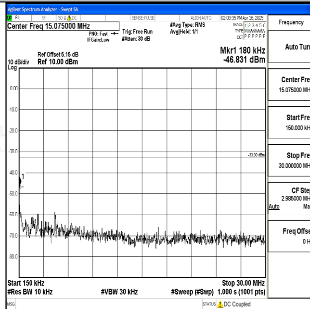
Band25_1.4MHz_QPSK_26683_1RB#0_0.15~30_0.15~30
