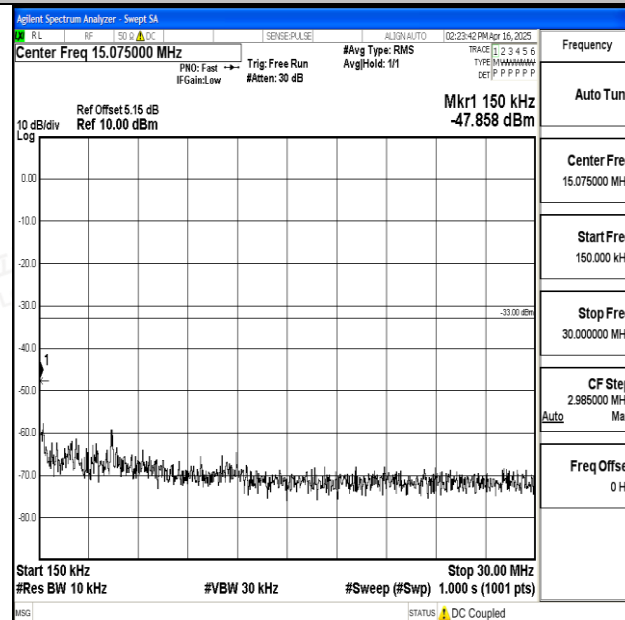
Band25_3MHz_QPSK_26365_1RB#0_0.15~30_0.15~30
