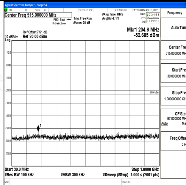
Band25_1.4MHz_16QAM_26365_1RB#0_30~1000_30~1000
