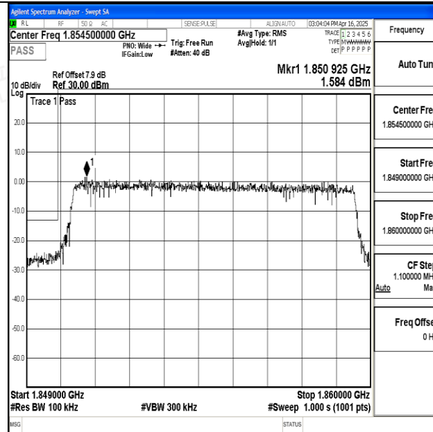
Band25_10MHz_QPSK_26090_50RB#0
