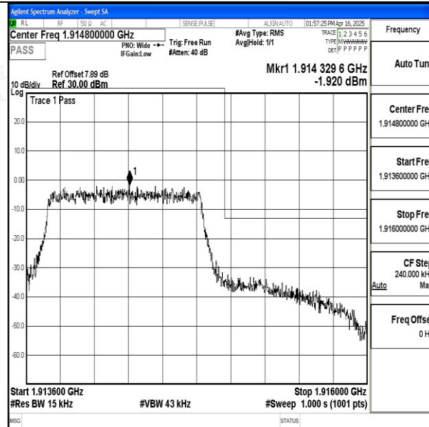
Band25_1.4MHz_QPSK_26683_6RB#0
