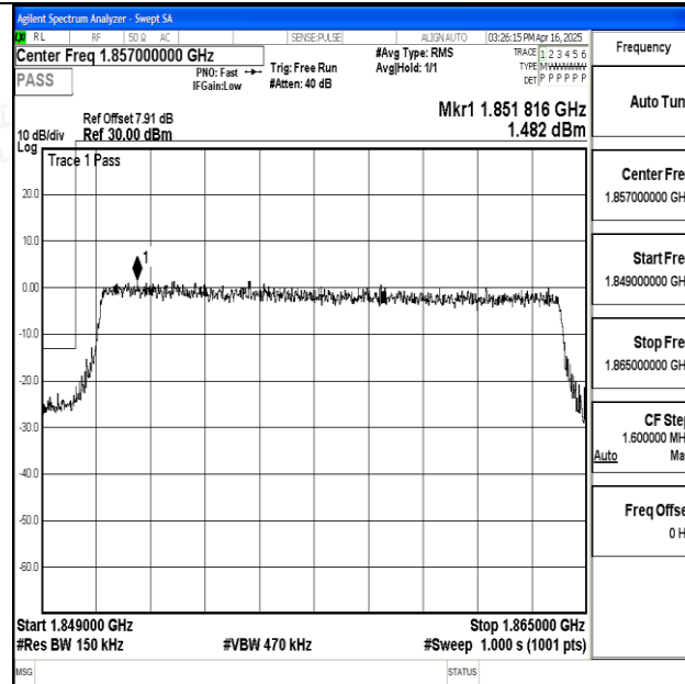
Band25_15MHz_QPSK_26115_75RB#0
