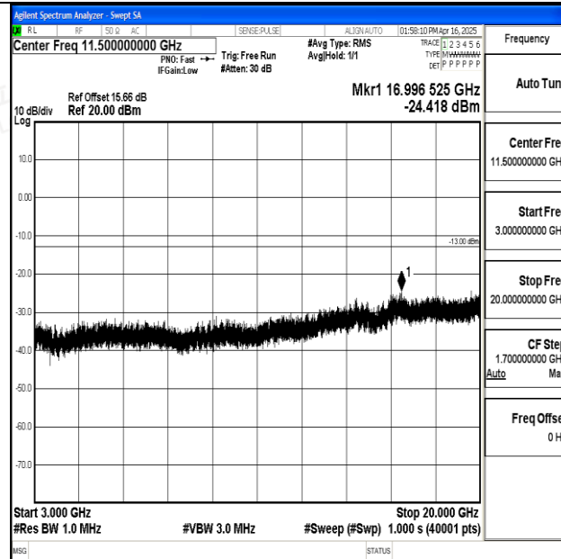
Band25_1.4MHz_QPSK_26047_1RB#0_3000~20000_3000~20000
