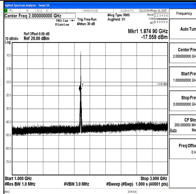
Band25_3MHz_QPSK_26365_1RB#0_1000~3000_1000~3000
