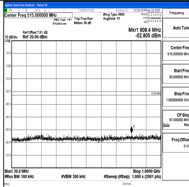
Band25_1.4MHz_16QAM_26047_1RB#0_30~1000_30~1000
