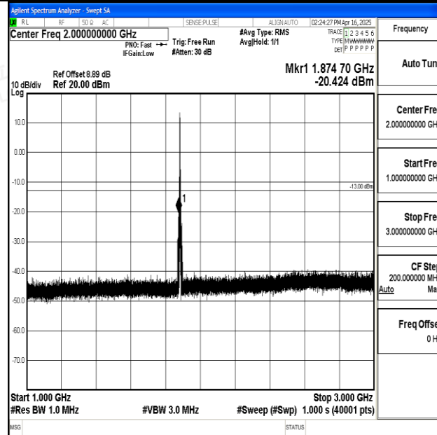
Band25_3MHz_16QAM_26365_1RB#0_1000~3000_1000~3000
