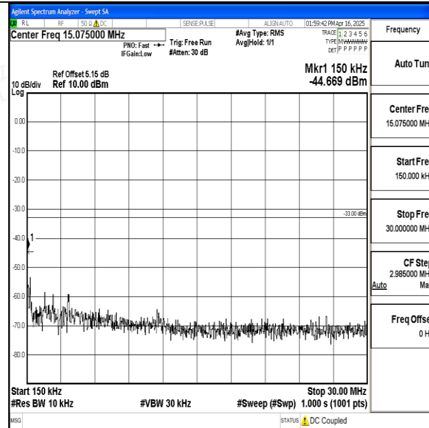
Band25_1.4MHz_16QAM_26365_1RB#0_0.15~30_0.15~30
