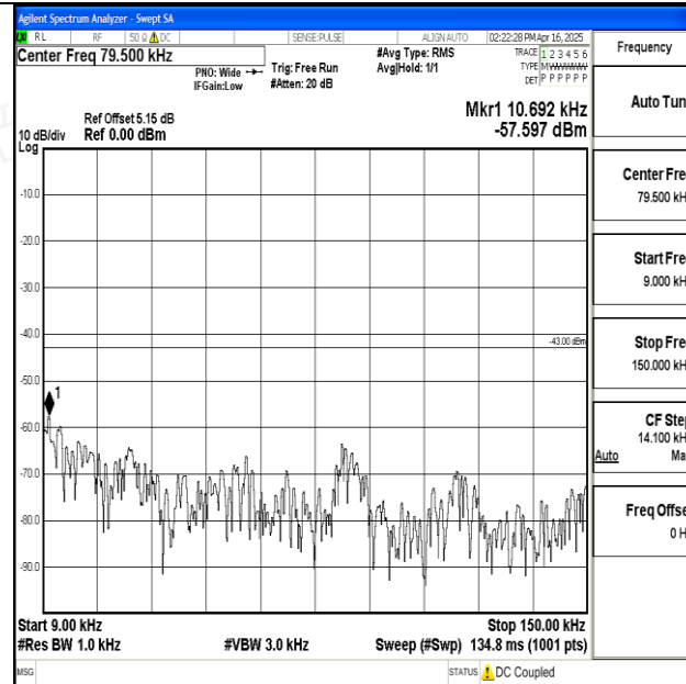
Band25_3MHz_QPSK_26055_1RB#0_0.009~0.15_0.009~0.15
