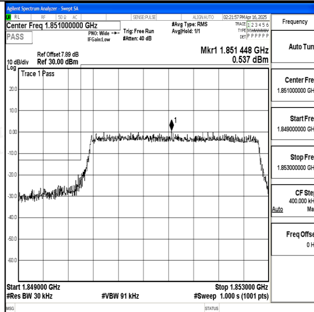
Band25_3MHz_16QAM_26055_15RB#0
