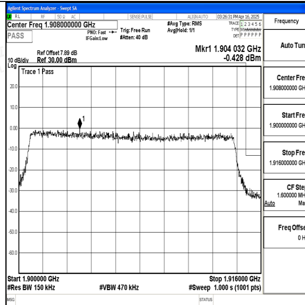
Band25_15MHz_QPSK_26615_75RB#0
