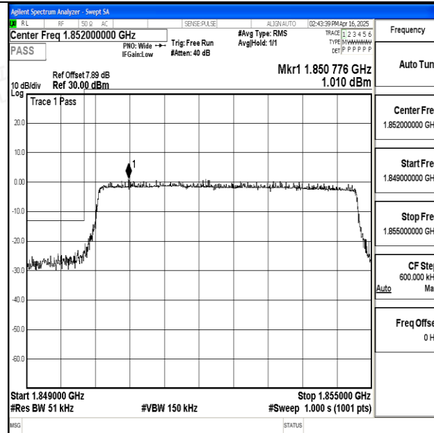
Band25_5MHz_QPSK_26065_25RB#0
