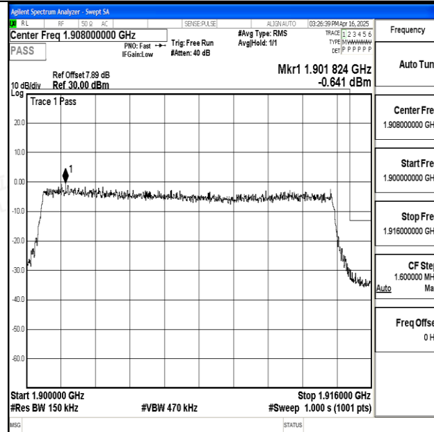
Band25_15MHz_16QAM_26615_75RB#0
