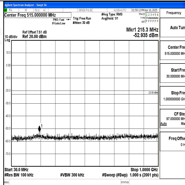
Band25_1.4MHz_QPSK_26365_1RB#0_30~1000_30~1000
