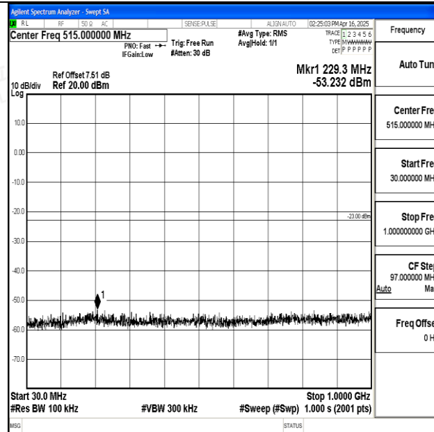
Band25_3MHz_QPSK_26675_1RB#0_30~1000_30~1000
