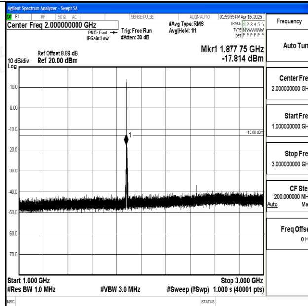
Band25_1.4MHz_16QAM_26365_1RB#0_1000~3000_1000~3000
