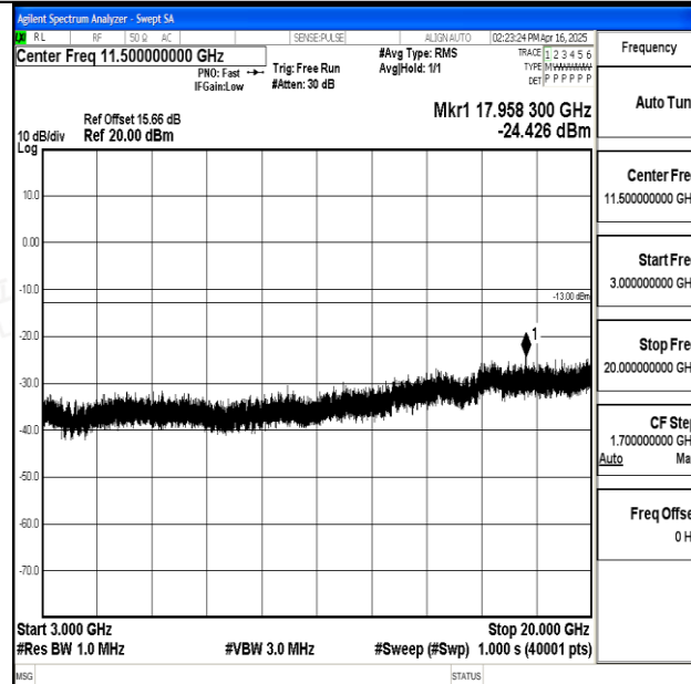
Band25_3MHz_16QAM_26055_1RB#0_3000~20000_3000~20000
