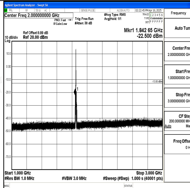
Band25_3MHz_QPSK_26055_1RB#0_1000~3000_1000~3000
