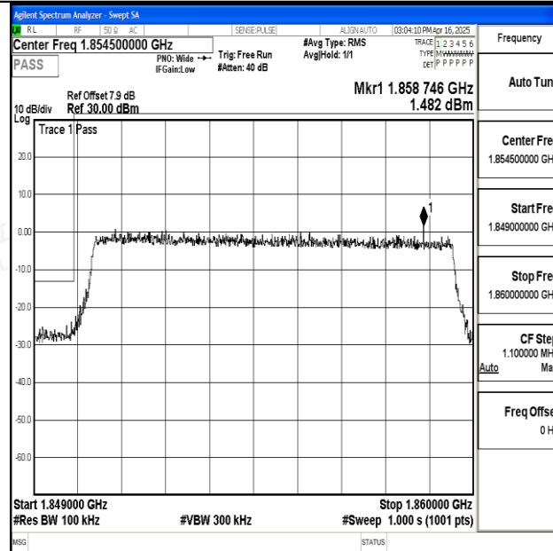
Band25_10MHz_16QAM_26090_50RB#0
