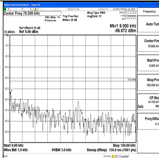
Band25_1.4MHz_16QAM_26365_1RB#0_0.009~0.15_0.009~0.15
