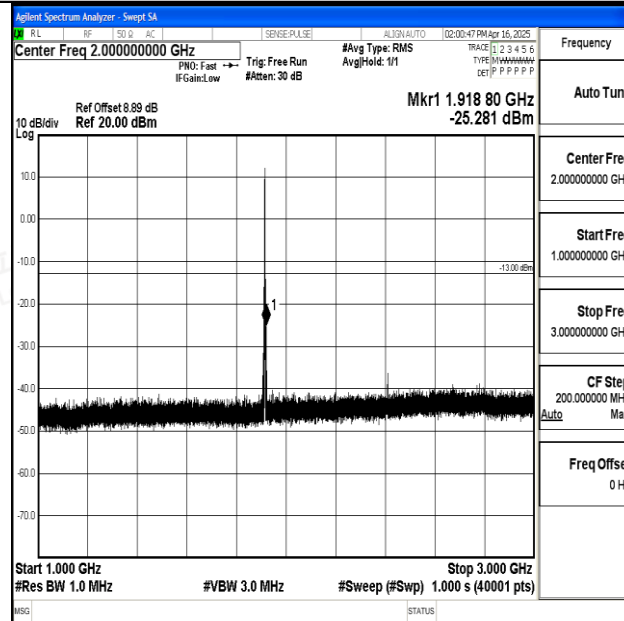
Band25_1.4MHz_QPSK_26683_1RB#0_1000~3000_1000~3000
