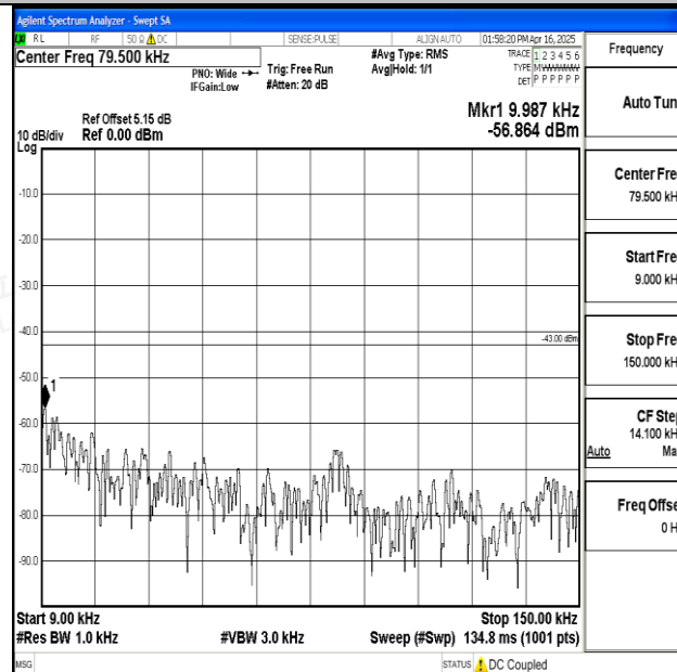
Band25_1.4MHz_16QAM_26047_1RB#0_0.009~0.15_0.009~0.15
