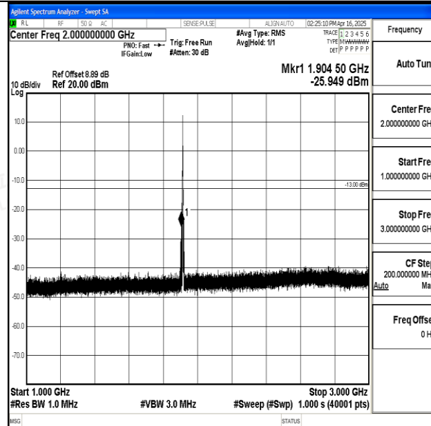
Band25_3MHz_QPSK_26675_1RB#0_1000~3000_1000~3000
