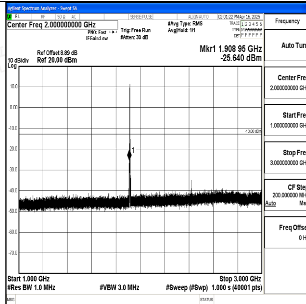
Band25_1.4MHz_16QAM_26683_1RB#0_1000~3000_1000~3000
