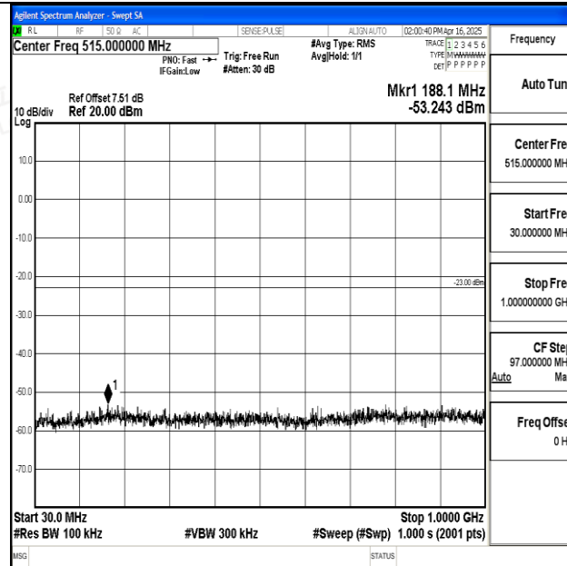
Band25_1.4MHz_QPSK_26683_1RB#0_30~1000_30~1000
