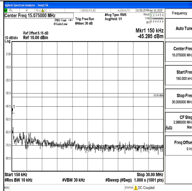
Band25_1.4MHz_16QAM_26047_1RB#0_0.15~30_0.15~30
