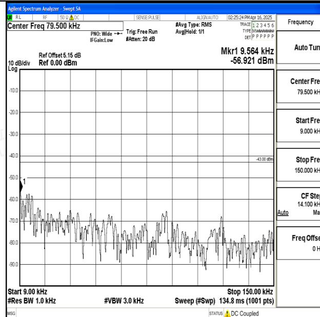
Band25_3MHz_16QAM_26675_1RB#0_0.009~0.15_0.009~0.15
