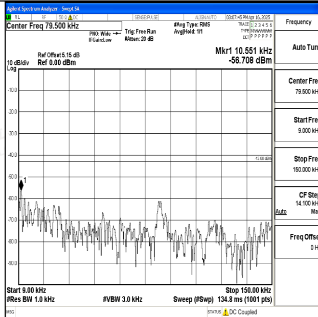
Band25_10MHz_16QAM_26640_1RB#0_0.009~0.15_0.009~0.15
