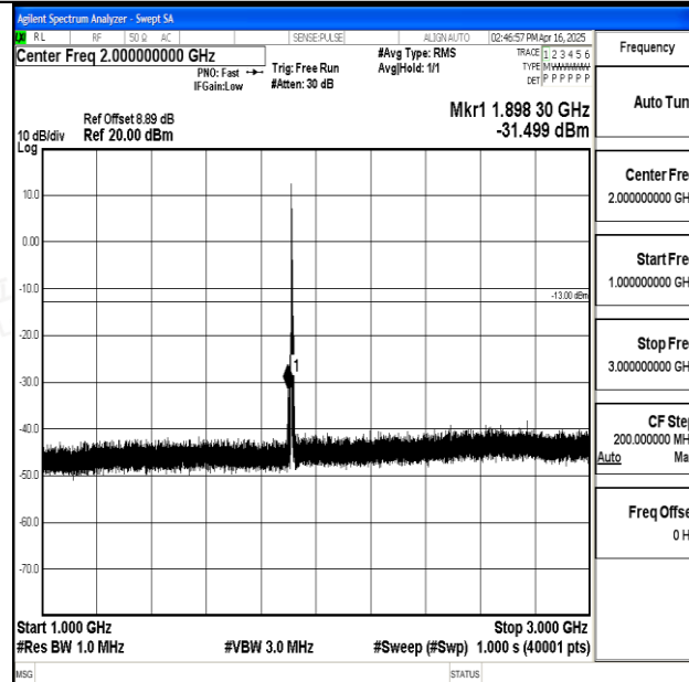
Band25_5MHz_QPSK_26665_1RB#0_1000~3000_1000~3000
