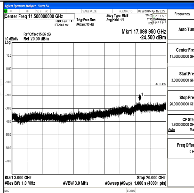
Band25_15MHz_16QAM_26365_1RB#0_3000~20000_3000~20000
