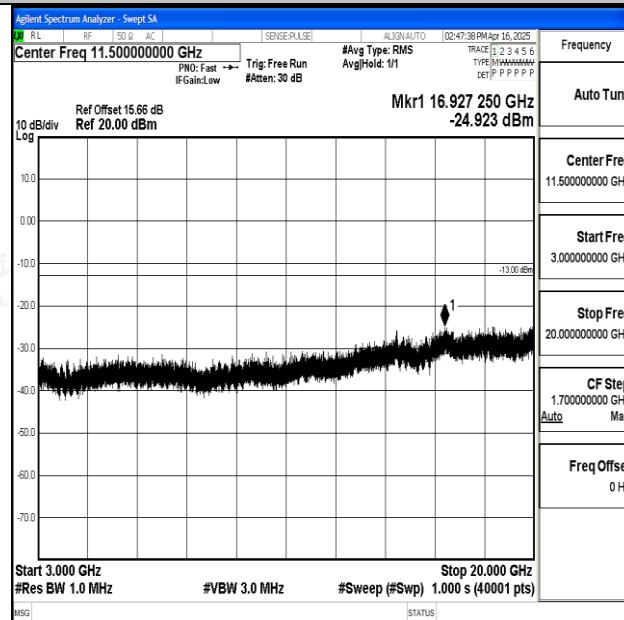
Band25_5MHz_16QAM_26665_1RB#0_3000~20000_3000~20000
