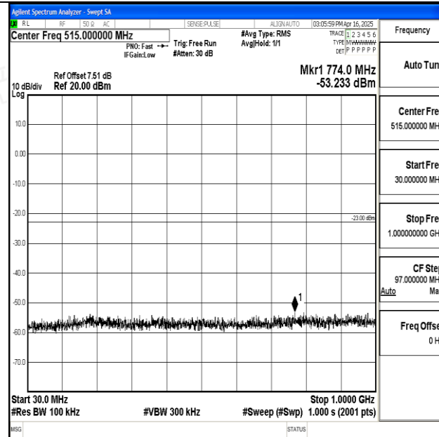
Band25_10MHz_QPSK_26365_1RB#0_30~1000_30~1000
