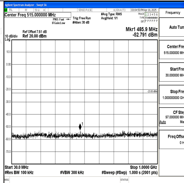
Band25_10MHz_QPSK_26090_1RB#0_30~1000_30~1000
