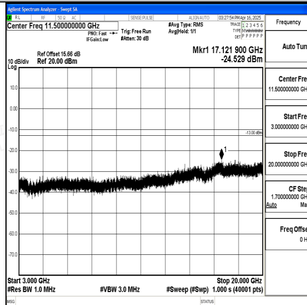
Band25_15MHz_16QAM_26115_1RB#0_3000~20000_3000~20000
