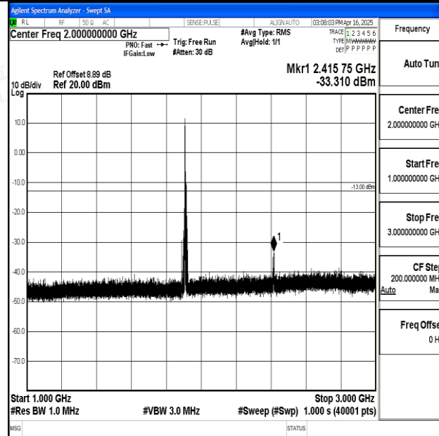
Band25_10MHz_16QAM_26640_1RB#0_1000~3000_1000~3000
