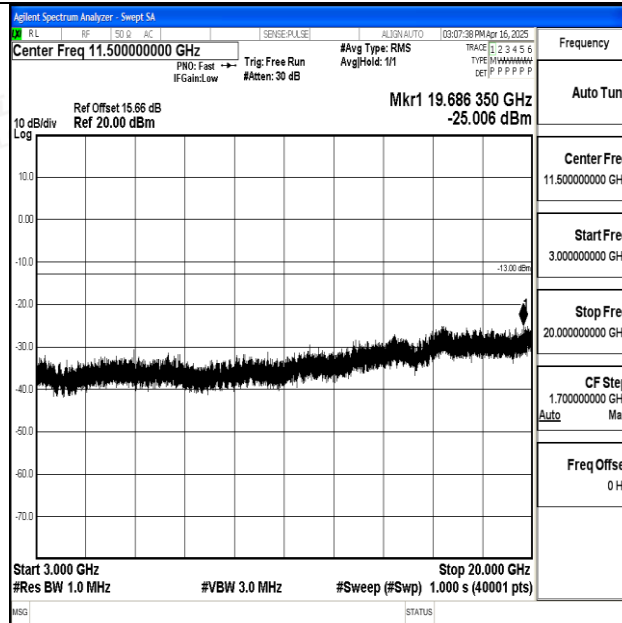
Band25_10MHz_QPSK_26640_1RB#0_3000~20000_3000~20000
