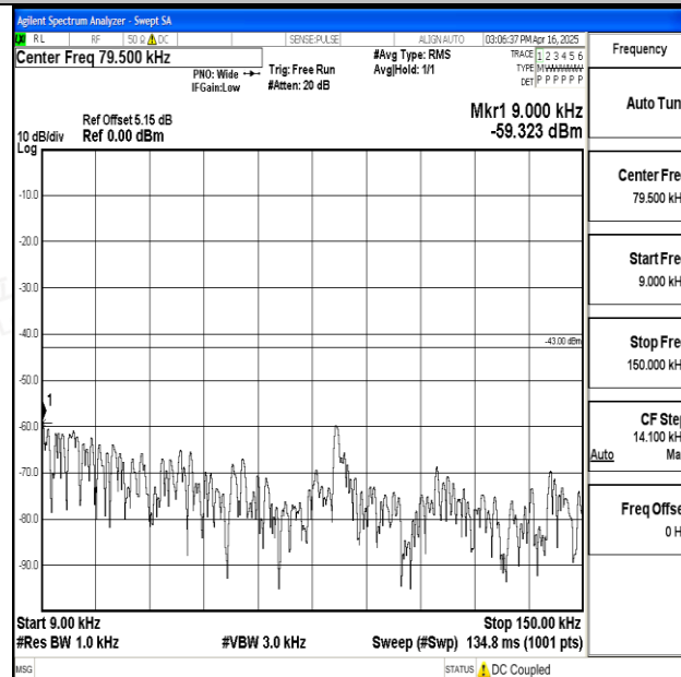
Band25_10MHz_16QAM_26365_1RB#0_0.009~0.15_0.009~0.15
