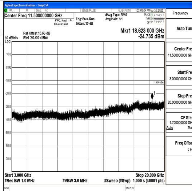
Band25_10MHz_QPSK_26090_1RB#0_3000~20000_3000~20000
