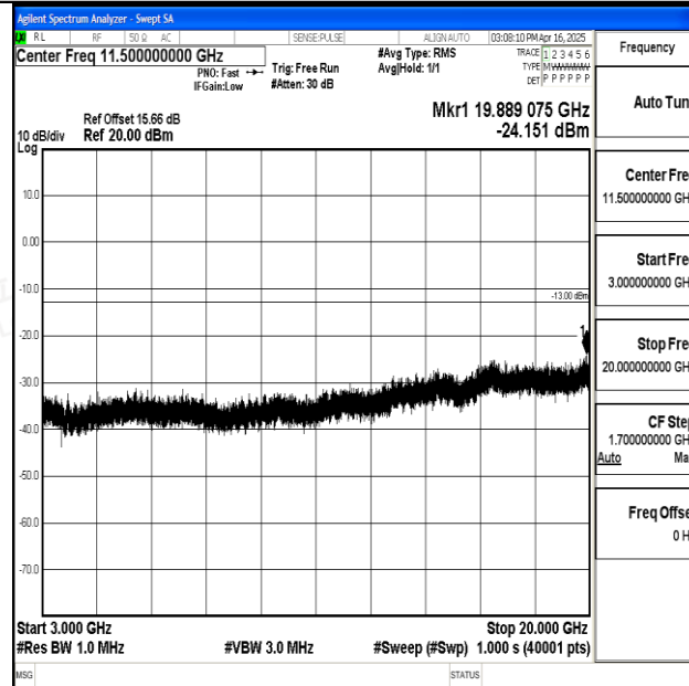
Band25_10MHz_16QAM_26640_1RB#0_3000~20000_3000~20000
