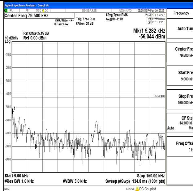
Band25_15MHz_16QAM_26365_1RB#0_0.009~0.15_0.009~0.15
