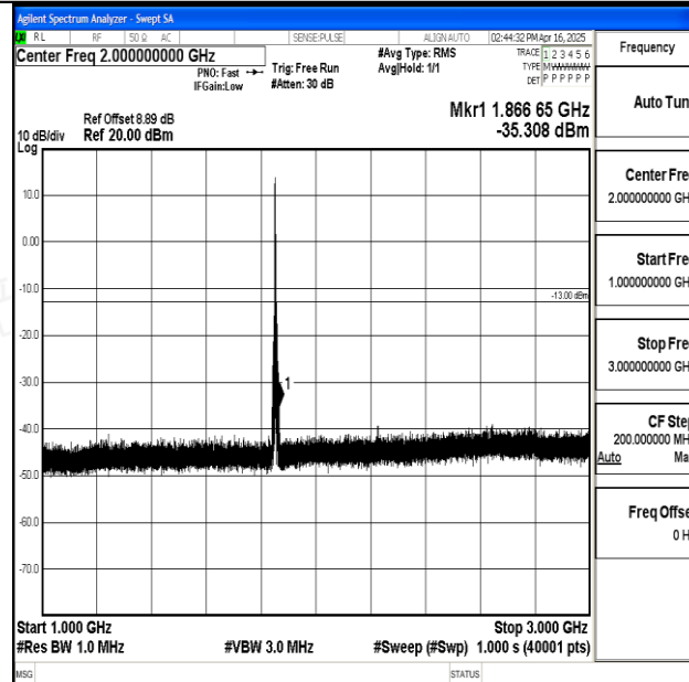
Band25_5MHz_QPSK_26065_1RB#0_1000~3000_1000~3000
