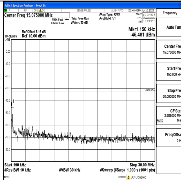
Band25_5MHz_QPSK_26665_1RB#0_0.15~30_0.15~30
