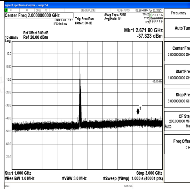
Band25_15MHz_QPSK_26615_1RB#0_1000~3000_1000~3000
