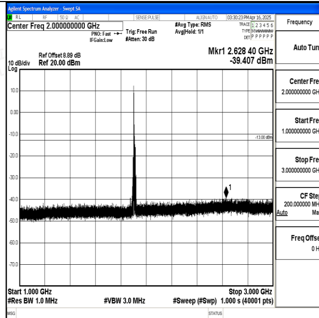
Band25_15MHz_16QAM_26615_1RB#0_1000~3000_1000~3000
