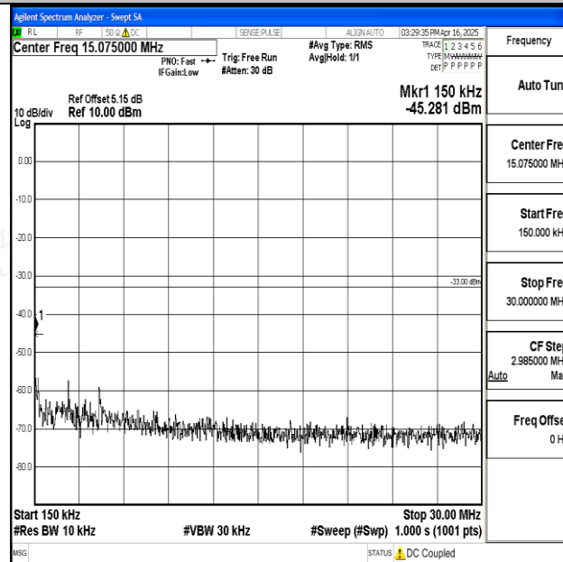
Band25_15MHz_QPSK_26615_1RB#0_0.15~30_0.15~30
