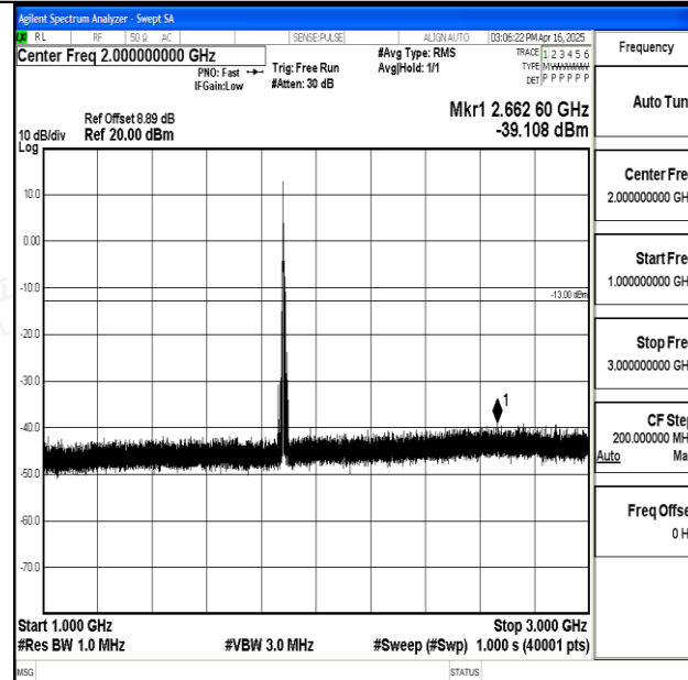
Band25_10MHz_QPSK_26365_1RB#0_1000~3000_1000~3000
