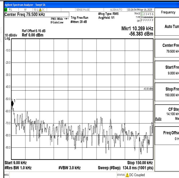
Band25_15MHz_QPSK_26115_1RB#0_0.009~0.15_0.009~0.15
