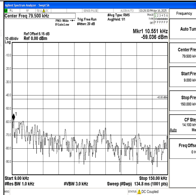
Band25_15MHz_QPSK_26615_1RB#0_0.009~0.15_0.009~0.15
