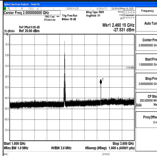
Band25_5MHz_QPSK_26365_1RB#0_1000~3000_1000~3000
