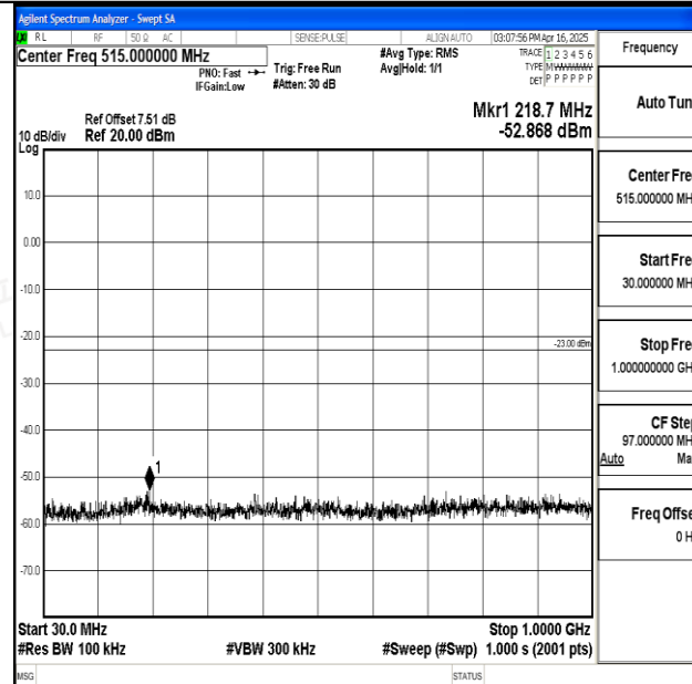
Band25_10MHz_16QAM_26640_1RB#0_30~1000_30~1000
