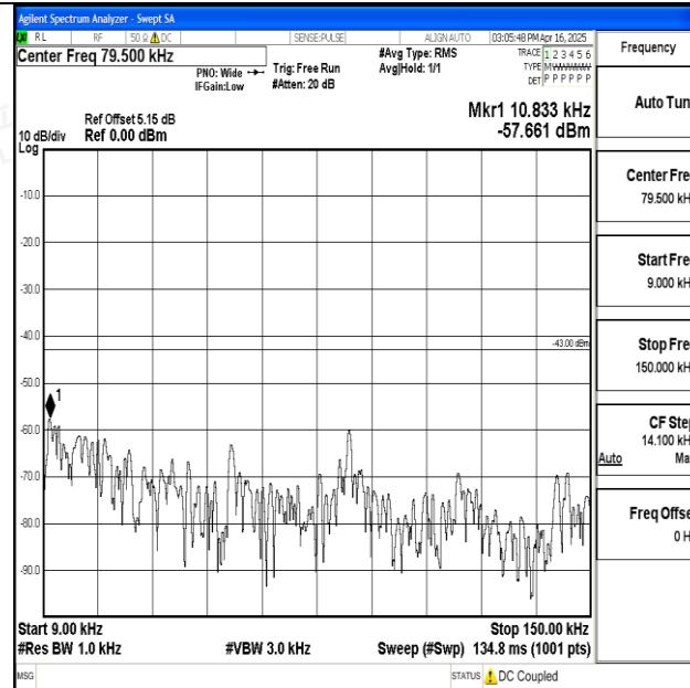
Band25_10MHz_QPSK_26365_1RB#0_0.009~0.15_0.009~0.15
