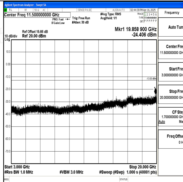
Band25_5MHz_QPSK_26065_1RB#0_3000~20000_3000~20000
