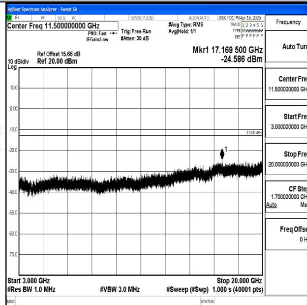
Band25_10MHz_16QAM_26365_1RB#0_3000~20000_3000~20000
