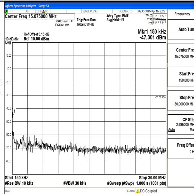
Band25_5MHz_QPSK_26365_1RB#0_0.15~30_0.15~30
