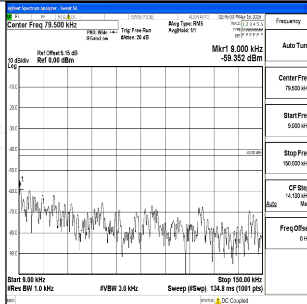
Band25_5MHz_16QAM_26365_1RB#0_0.009~0.15_0.009~0.15
