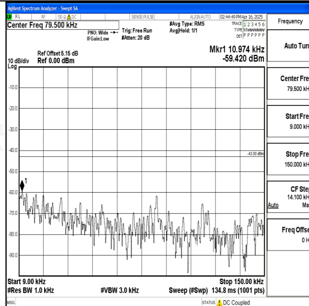
Band25_5MHz_16QAM_26065_1RB#0_0.009~0.15_0.009~0.15
