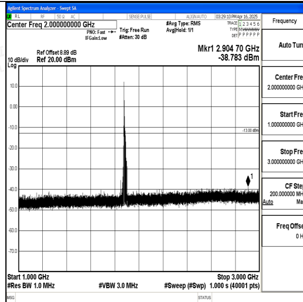
Band25_15MHz_16QAM_26365_1RB#0_1000~3000_1000~3000
