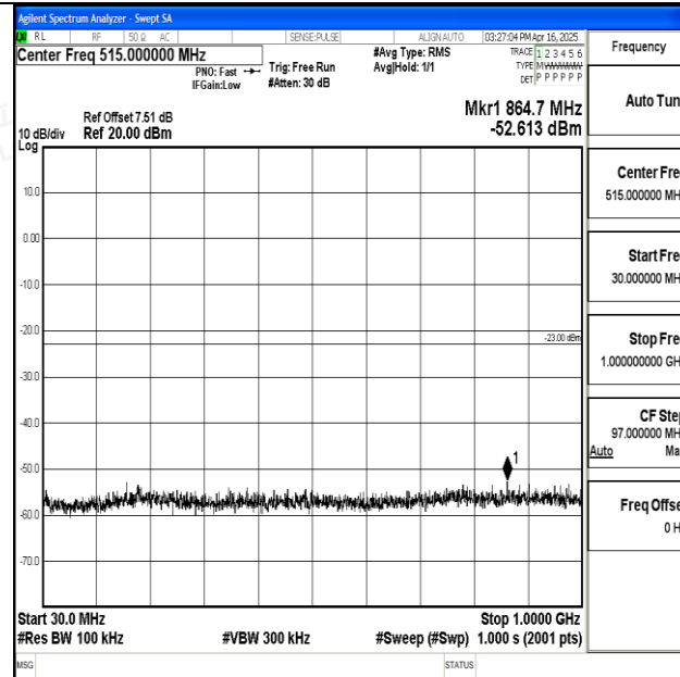
Band25_15MHz_QPSK_26115_1RB#0_30~1000_30~1000
