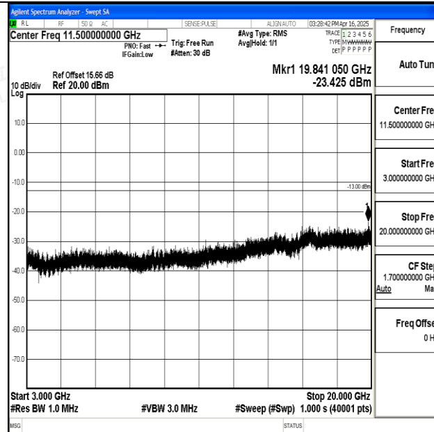
Band25_15MHz_QPSK_26365_1RB#0_3000~20000_3000~20000
