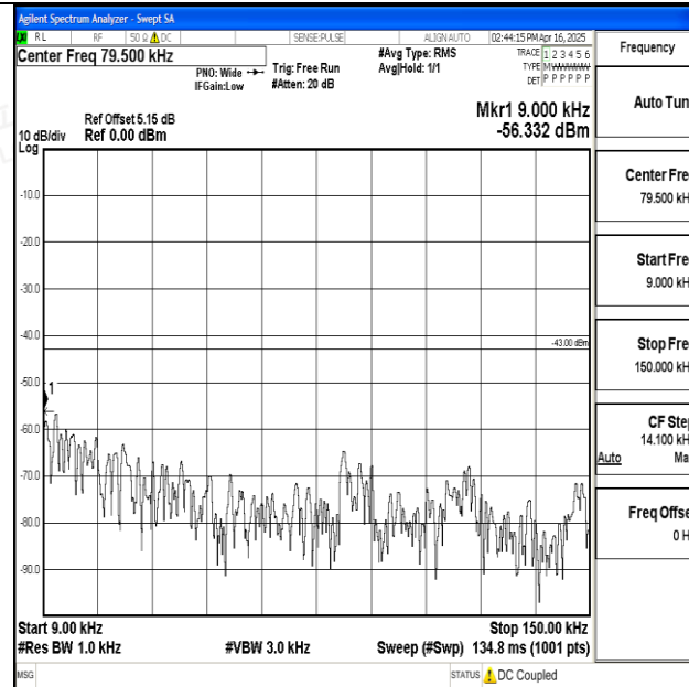
Band25_5MHz_QPSK_26065_1RB#0_0.009~0.15_0.009~0.15
