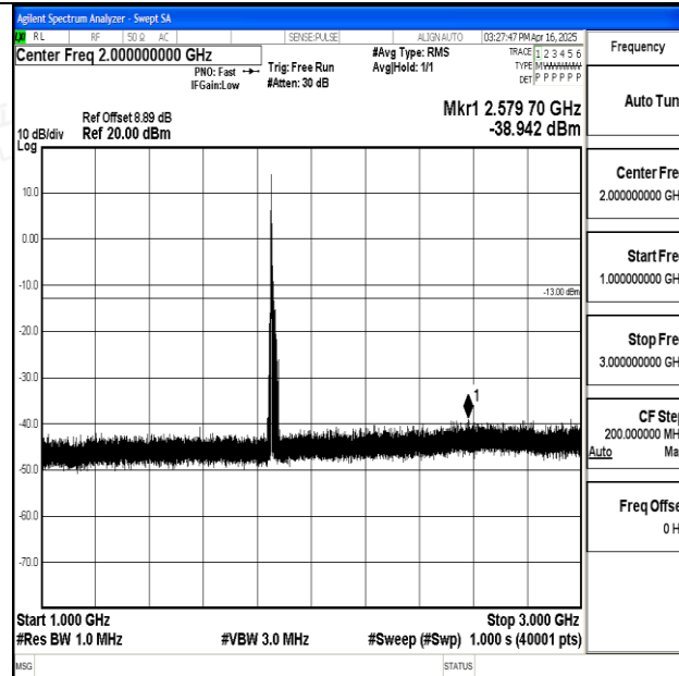
Band25_15MHz_16QAM_26115_1RB#0_1000~3000_1000~3000
