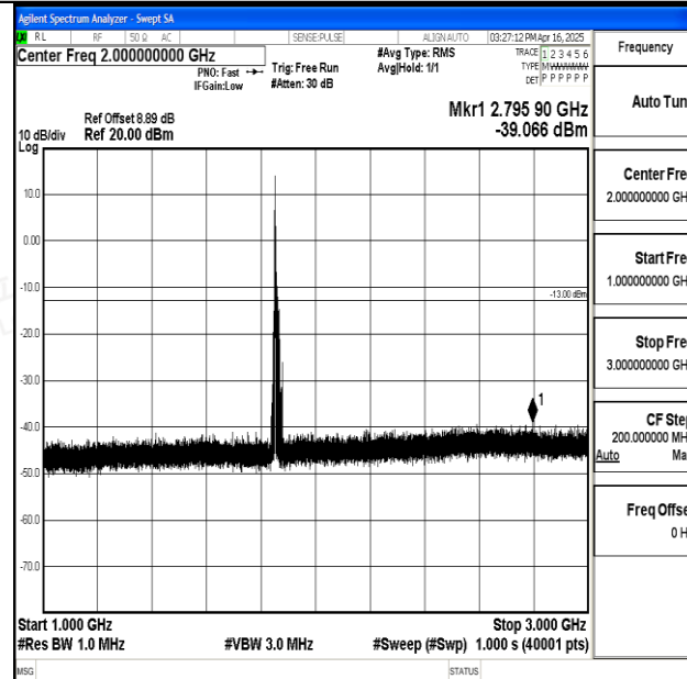
Band25_15MHz_QPSK_26115_1RB#0_1000~3000_1000~3000
