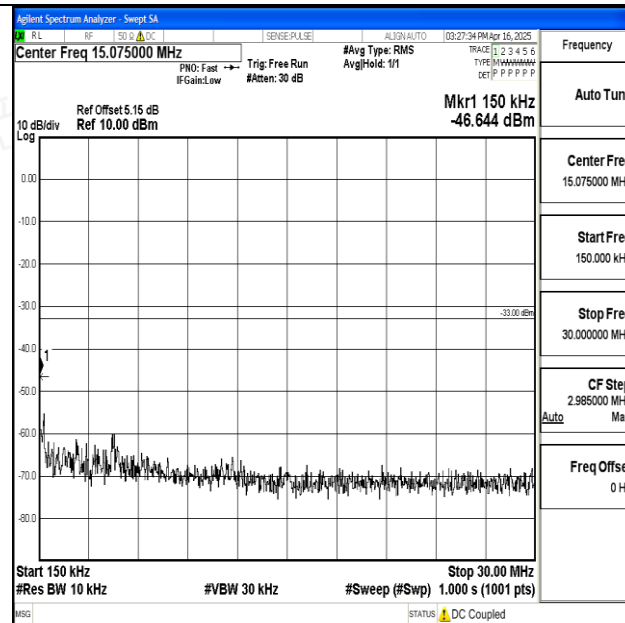
Band25_15MHz_16QAM_26115_1RB#0_0.15~30_0.15~30
