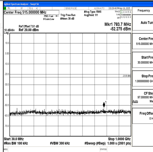
Band25_15MHz_QPSK_26615_1RB#0_30~1000_30~1000
