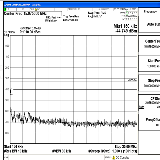
Band25_10MHz_QPSK_26365_1RB#0_0.15~30_0.15~30
