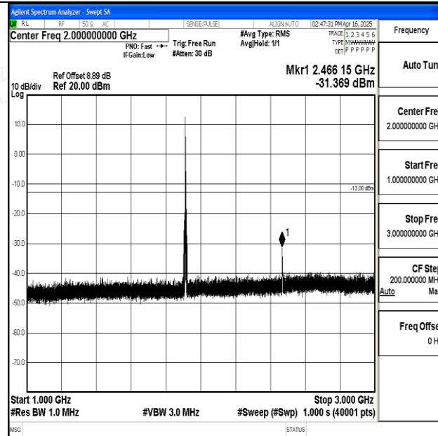
Band25_5MHz_16QAM_26665_1RB#0_1000~3000_1000~3000
