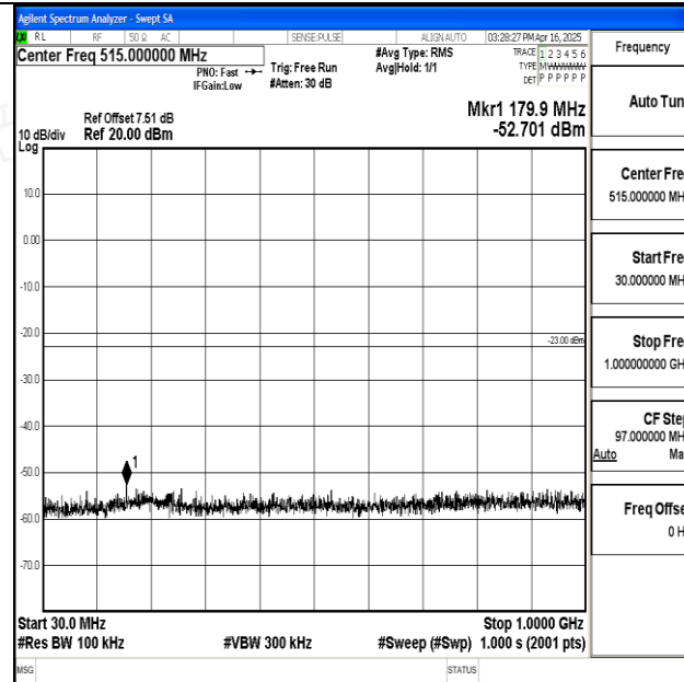
Band25_15MHz_QPSK_26365_1RB#0_30~1000_30~1000
