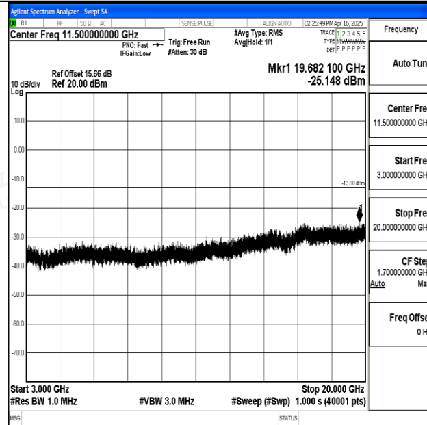
Band25_3MHz_16QAM_26675_1RB#0_3000~20000_3000~20000
