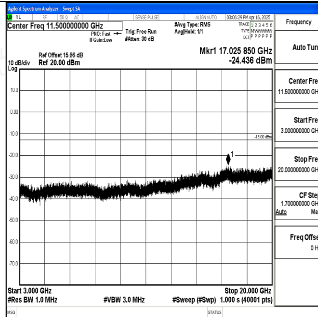
Band25_10MHz_QPSK_26365_1RB#0_3000~20000_3000~20000
