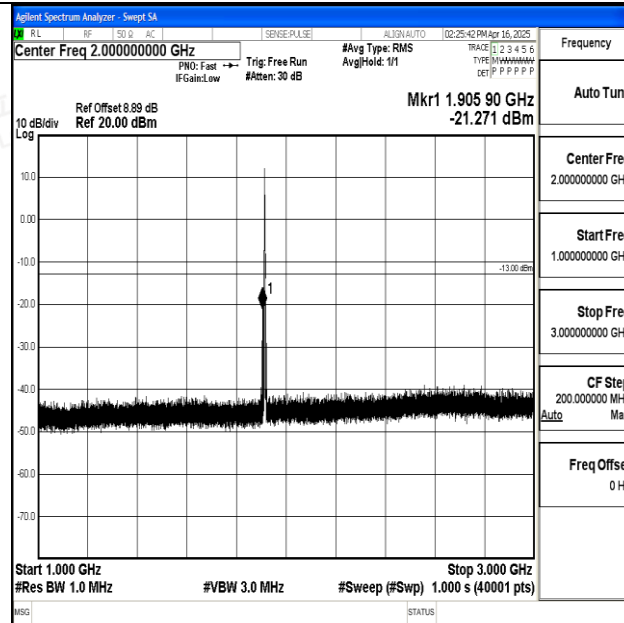
Band25_3MHz_16QAM_26675_1RB#0_1000~3000_1000~3000
