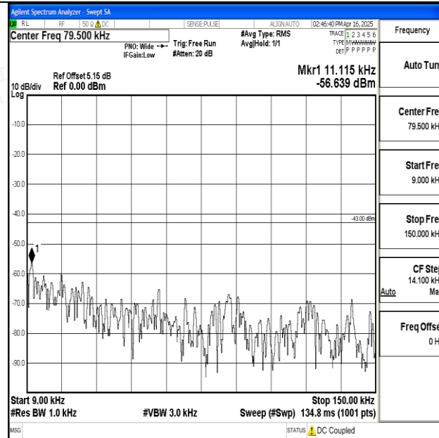
Band25_5MHz_QPSK_26665_1RB#0_0.009~0.15_0.009~0.15
