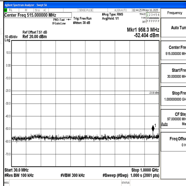
Band25_5MHz_QPSK_26065_1RB#0_30~1000_30~1000
