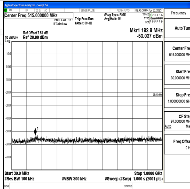
Band25_5MHz_QPSK_26665_1RB#0_30~1000_30~1000
