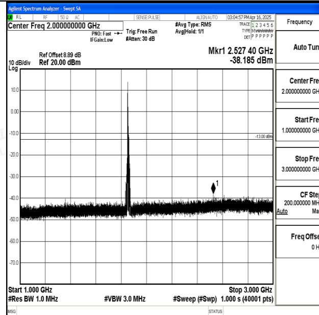
Band25_10MHz_QPSK_26090_1RB#0_1000~3000_1000~3000
