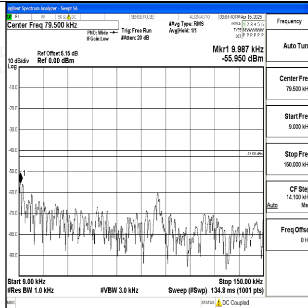
Band25_10MHz_QPSK_26090_1RB#0_0.009~0.15_0.009~0.15
