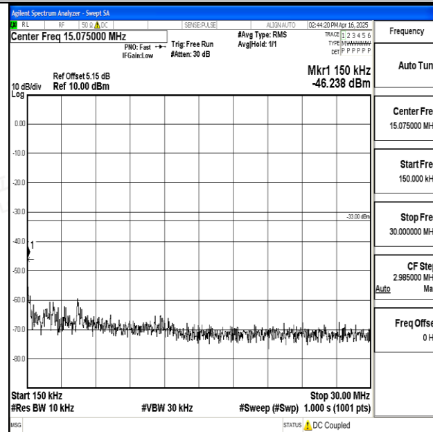
Band25_5MHz_QPSK_26065_1RB#0_0.15~30_0.15~30
