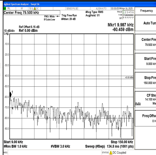
Band25_15MHz_16QAM_26615_1RB#0_0.009~0.15_0.009~0.15
