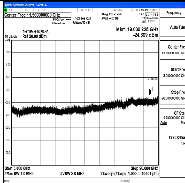
Band25_15MHz_16QAM_26615_1RB#0_3000~20000_3000~20000
