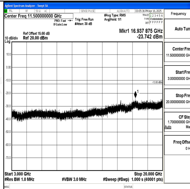
Band25_10MHz_16QAM_26090_1RB#0_3000~20000_3000~20000
