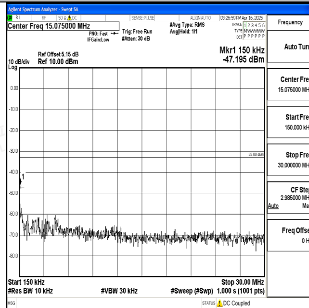
Band25_15MHz_QPSK_26115_1RB#0_0.15~30_0.15~30
