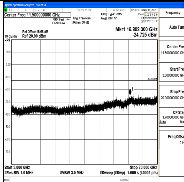
Band25_5MHz_16QAM_26065_1RB#0_3000~20000_3000~20000
