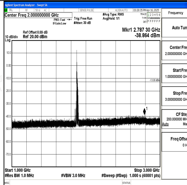
Band25_15MHz_QPSK_26365_1RB#0_1000~3000_1000~3000
