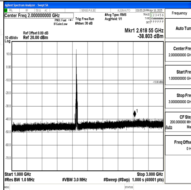
Band25_10MHz_16QAM_26090_1RB#0_1000~3000_1000~3000
