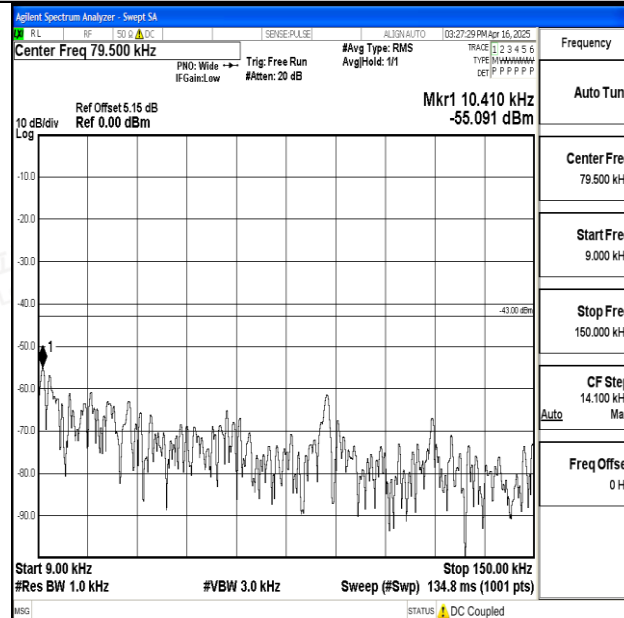
Band25_15MHz_16QAM_26115_1RB#0_0.009~0.15_0.009~0.15
