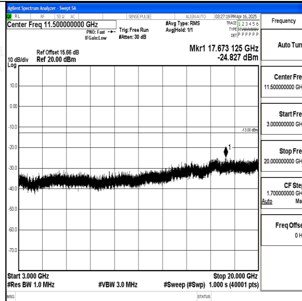
Band25_15MHz_QPSK_26115_1RB#0_3000~20000_3000~20000
