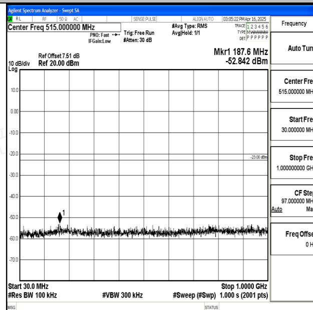
Band25_10MHz_16QAM_26090_1RB#0_30~1000_30~1000
