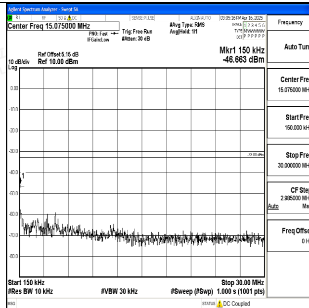
Band25_10MHz_16QAM_26090_1RB#0_0.15~30_0.15~30
