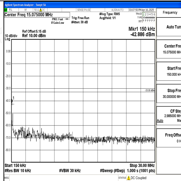
Band25_10MHz_16QAM_26640_1RB#0_0.15~30_0.15~30
