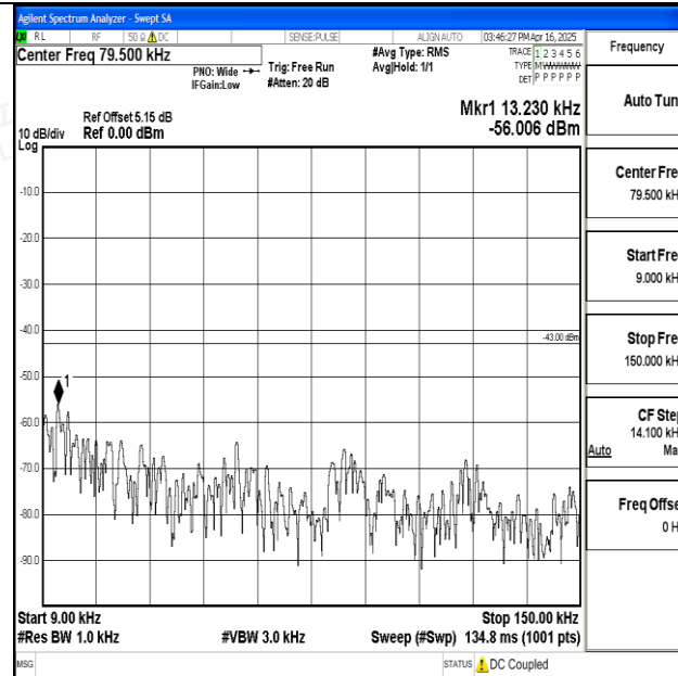
Band25_20MHz_QPSK_26140_1RB#0_0.009~0.15_0.009~0.15
