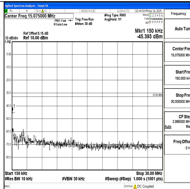
Band25_5MHz_16QAM_26065_1RB#0_0.15~30_0.15~30
