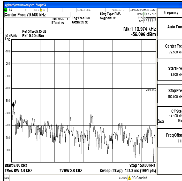
Band25_5MHz_QPSK_26365_1RB#0_0.009~0.15_0.009~0.15
