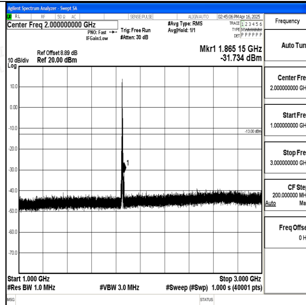
Band25_5MHz_16QAM_26065_1RB#0_1000~3000_1000~3000
