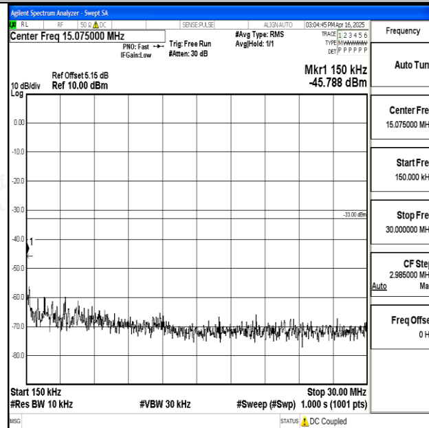
Band25_10MHz_QPSK_26090_1RB#0_0.15~30_0.15~30
