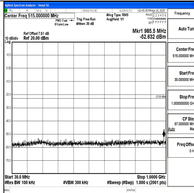
Band25_5MHz_QPSK_26365_1RB#0_30~1000_30~1000
