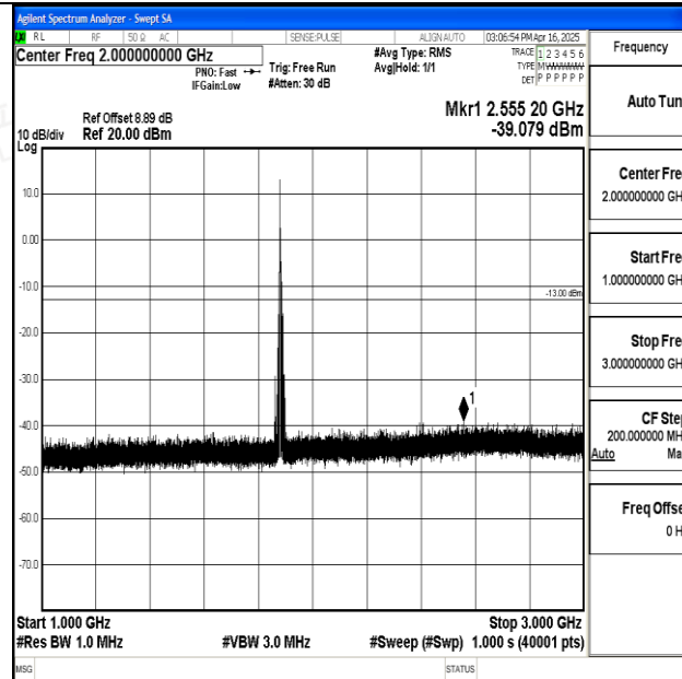
Band25_10MHz_16QAM_26365_1RB#0_1000~3000_1000~3000
