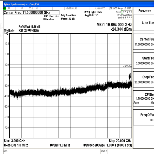
Band25_15MHz_QPSK_26615_1RB#0_3000~20000_3000~20000
