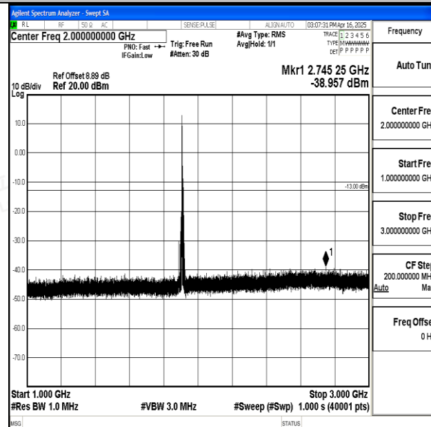
Band25_10MHz_QPSK_26640_1RB#0_1000~3000_1000~3000
