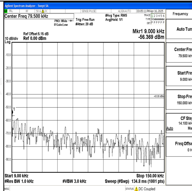
Band25_10MHz_16QAM_26090_1RB#0_0.009~0.15_0.009~0.15
