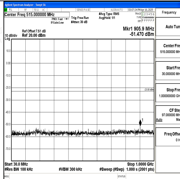
Band25_10MHz_QPSK_26640_1RB#0_30~1000_30~1000
