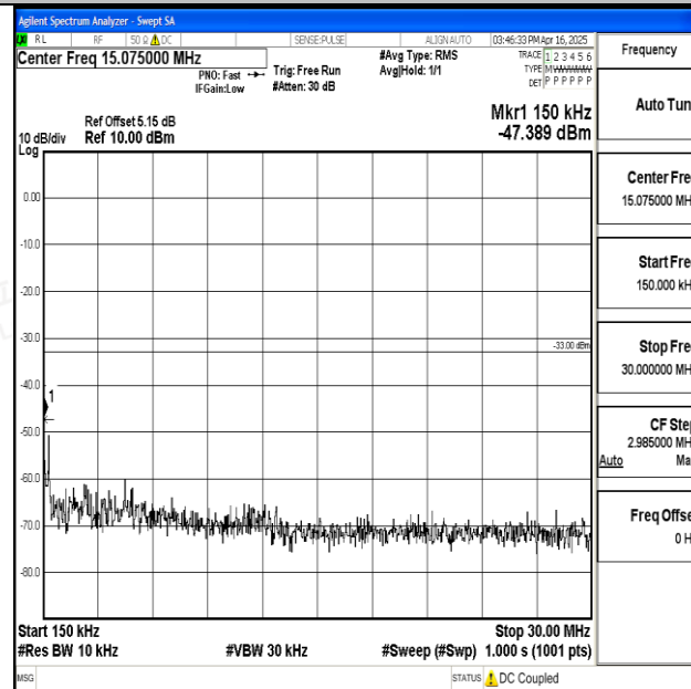
Band25_20MHz_QPSK_26140_1RB#0_0.15~30_0.15~30
