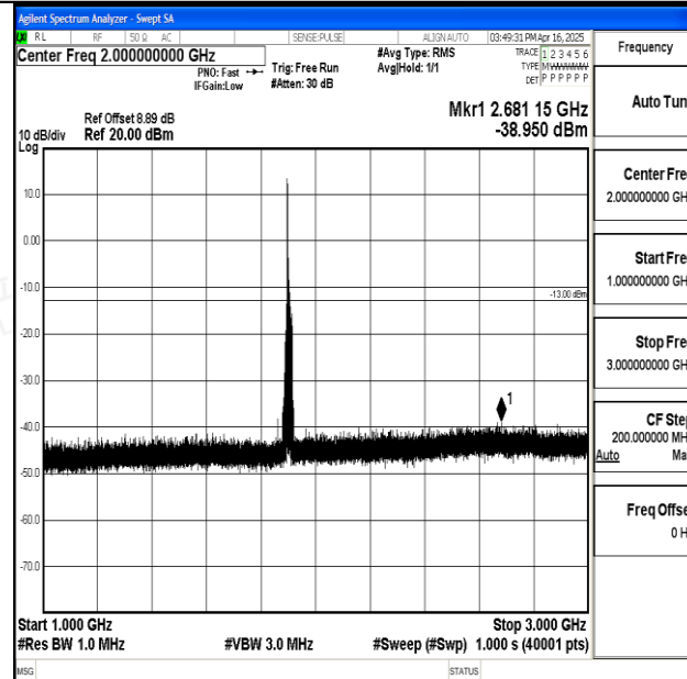
Band25_20MHz_QPSK_26590_1RB#0_1000~3000_1000~3000
