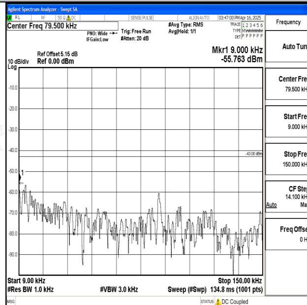
Band25_20MHz_16QAM_26140_1RB#0_0.009~0.15_0.009~0.15
