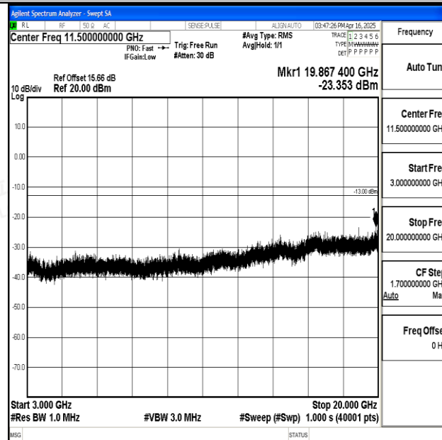
Band25_20MHz_16QAM_26140_1RB#0_3000~20000_3000~20000
