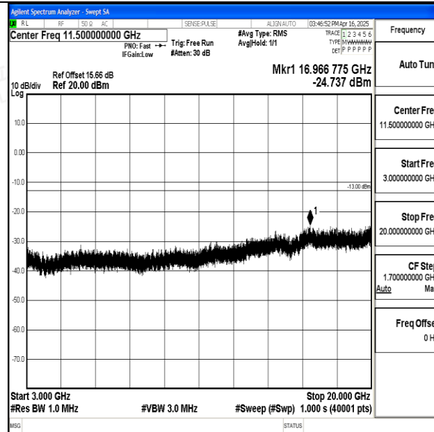
Band25_20MHz_QPSK_26140_1RB#0_3000~20000_3000~20000
