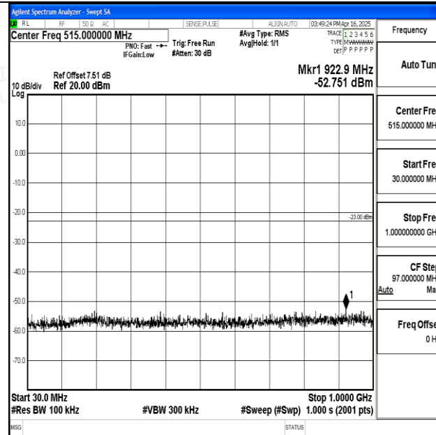
Band25_20MHz_QPSK_26590_1RB#0_30~1000_30~1000
