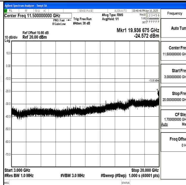
Band25_20MHz_16QAM_26365_1RB#0_3000~20000_3000~20000
