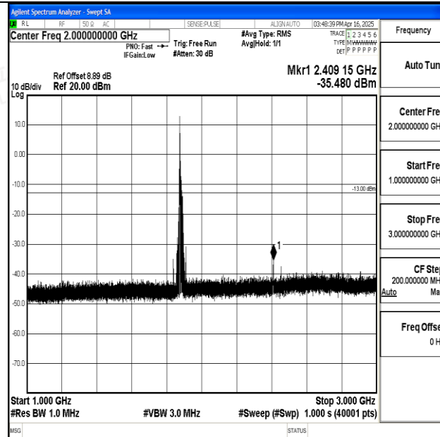
Band25_20MHz_16QAM_26365_1RB#0_1000~3000_1000~3000
