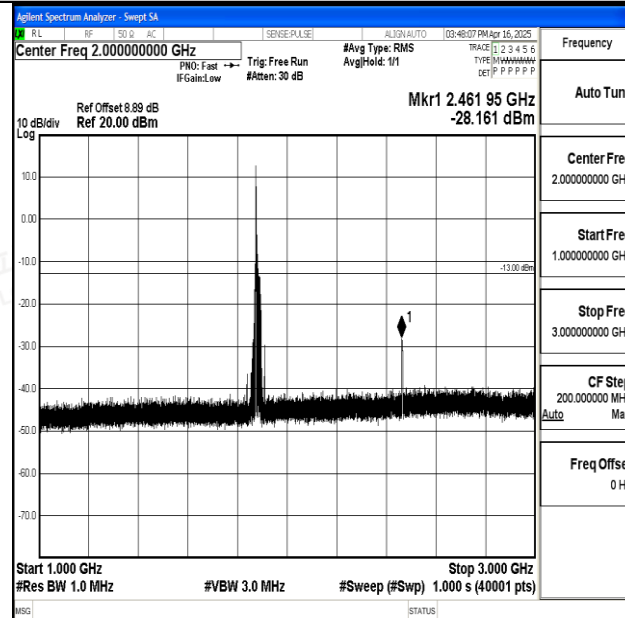
Band25_20MHz_QPSK_26365_1RB#0_1000~3000_1000~3000
