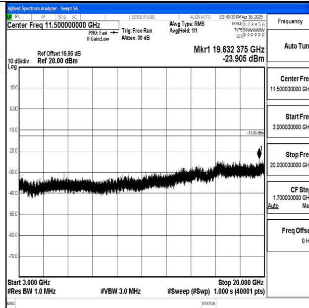
Band25_20MHz_QPSK_26590_1RB#0_3000~20000_3000~20000
