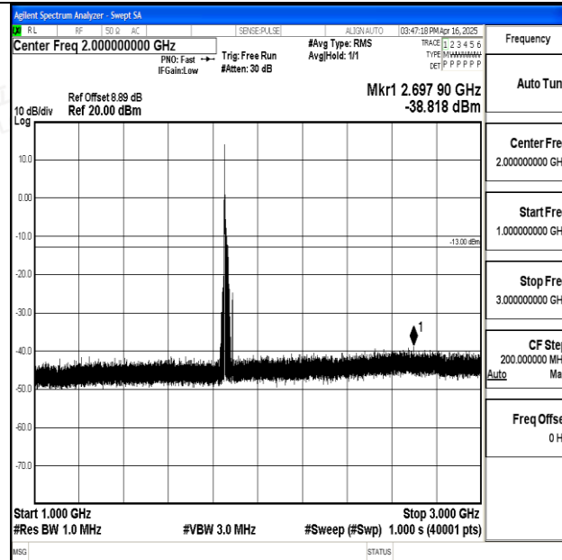
Band25_20MHz_16QAM_26140_1RB#0_1000~3000_1000~3000
