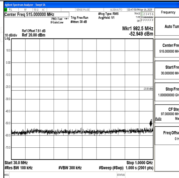
Band25_20MHz_QPSK_26365_1RB#0_30~1000_30~1000
