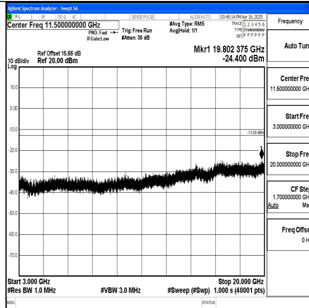
Band25_20MHz_QPSK_26365_1RB#0_3000~20000_3000~20000
