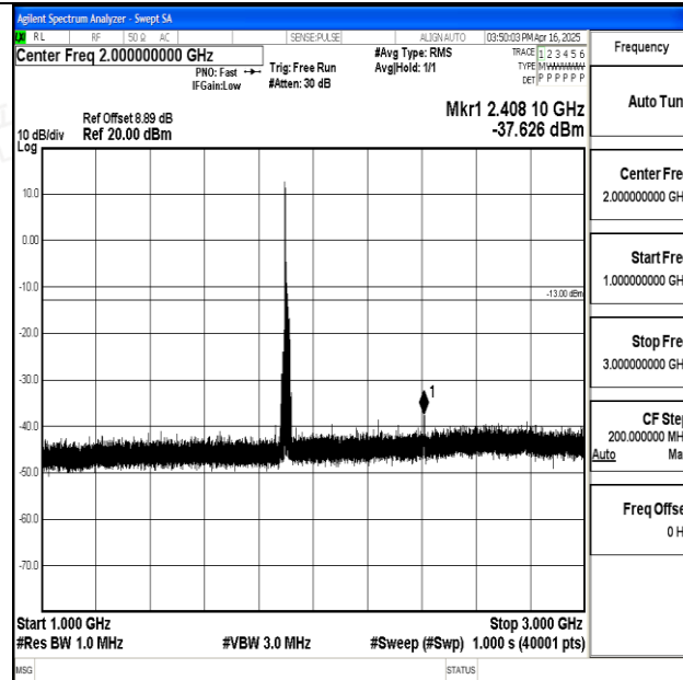
Band25_20MHz_16QAM_26590_1RB#0_1000~3000_1000~3000
