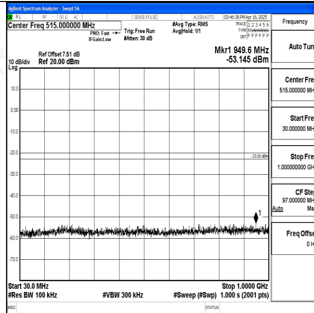
Band25_20MHz_QPSK_26140_1RB#0_30~1000_30~1000
