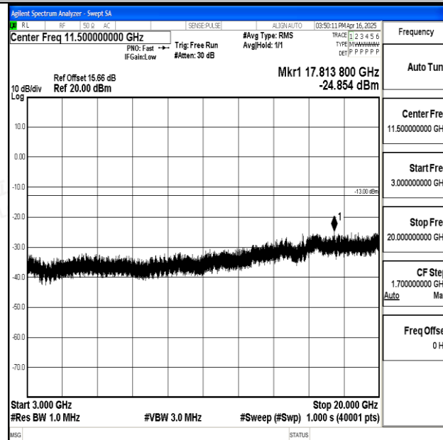
Band25_20MHz_16QAM_26590_1RB#0_3000~20000_3000~20000
