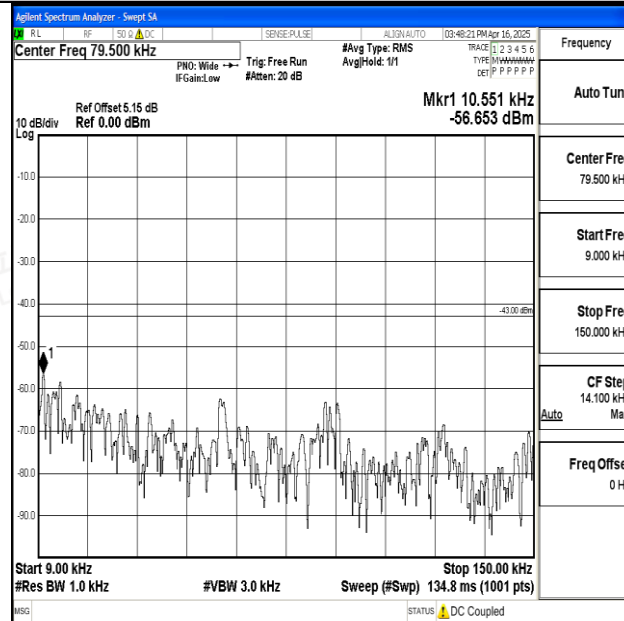
Band25_20MHz_16QAM_26365_1RB#0_0.009~0.15_0.009~0.15
