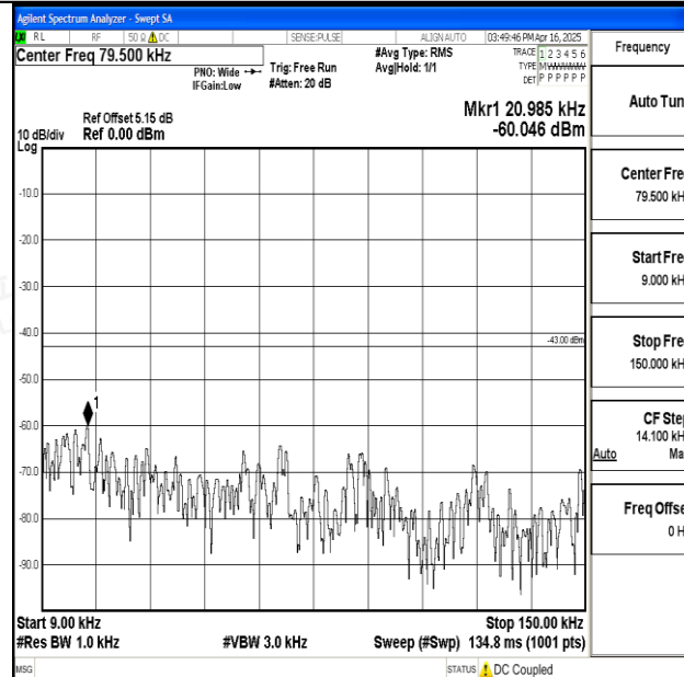
Band25_20MHz_16QAM_26590_1RB#0_0.009~0.15_0.009~0.15
