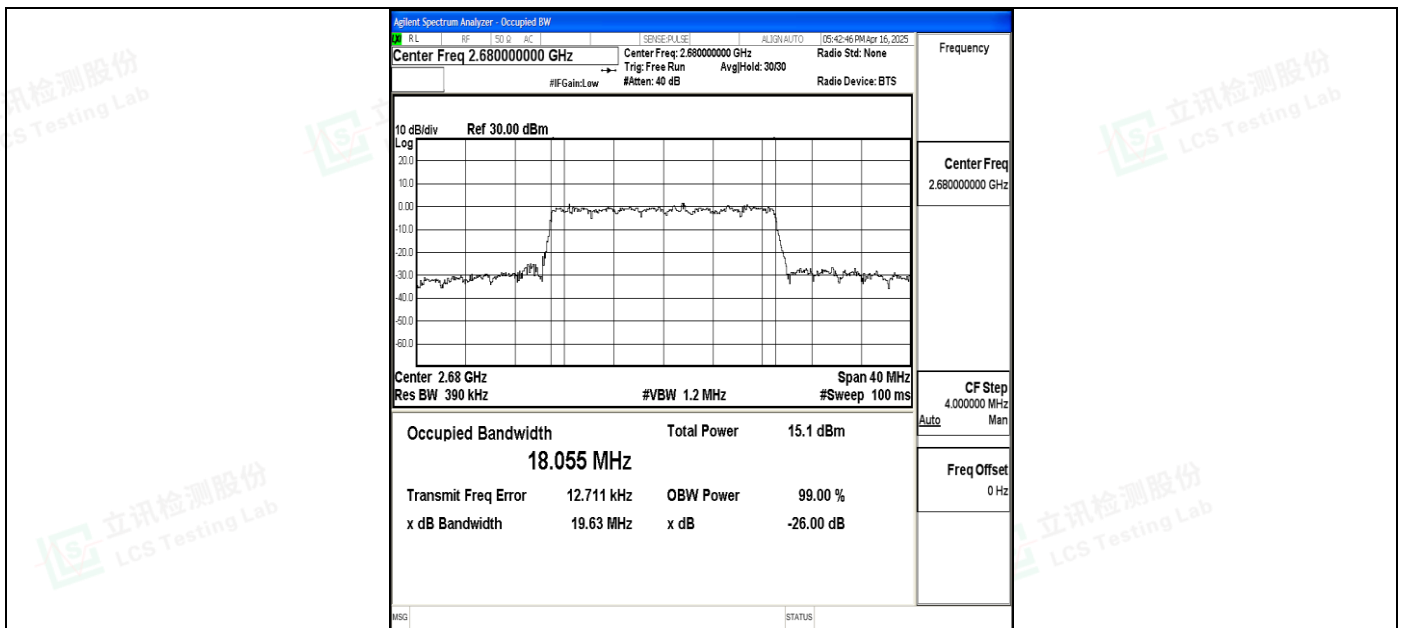
Band41-20MHz-QPSK-41490-100RB#0-PASS
