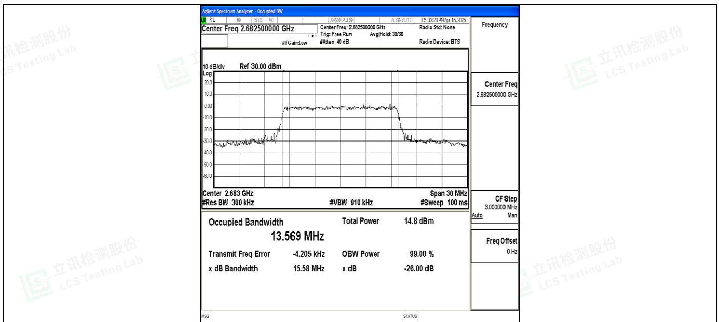
Band41-15MHz-QPSK-41515-75RB#0-PASS
