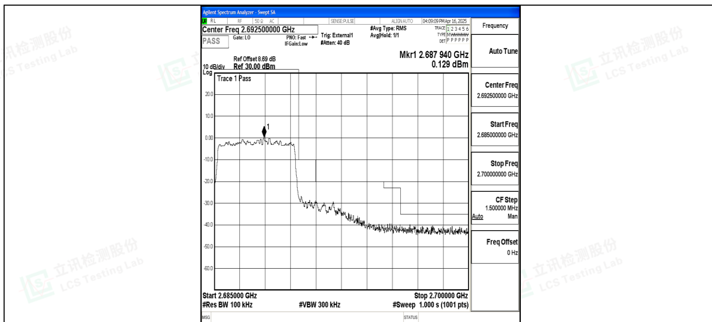
Band41_5MHz_16QAM_41565_25RB#0
