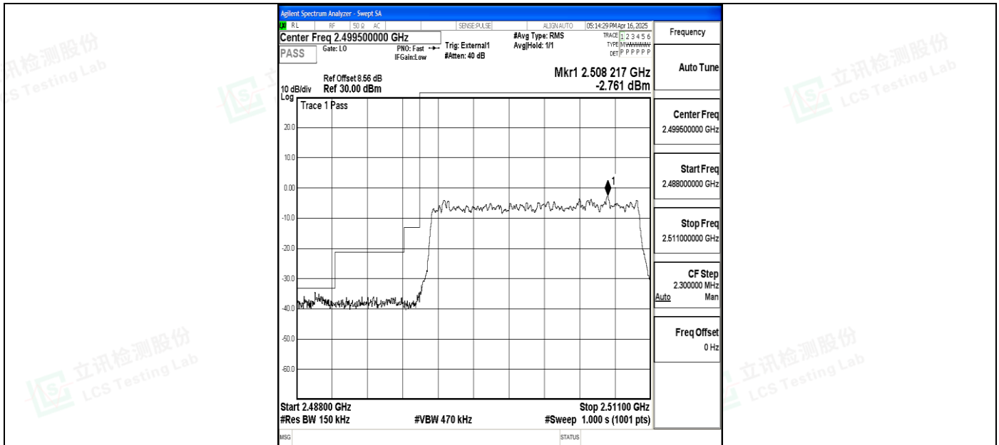
Band41_15MHz_16QAM_39725_75RB#0
