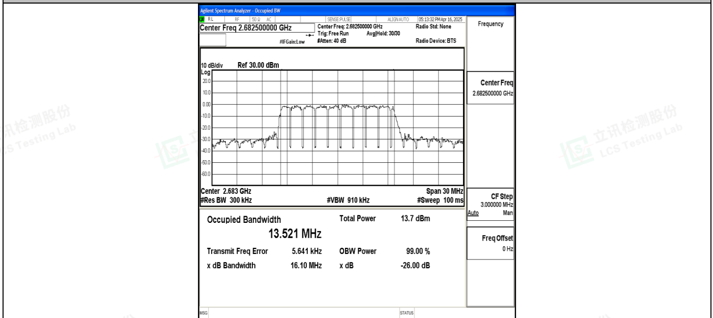
Band41-15MHz-16QAM-41515-75RB#0-PASS
