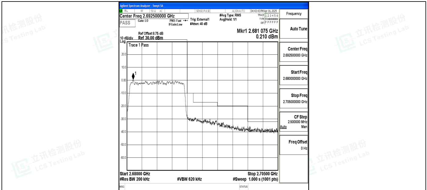
Band41_10MHz_16QAM_41540_50RB#0
