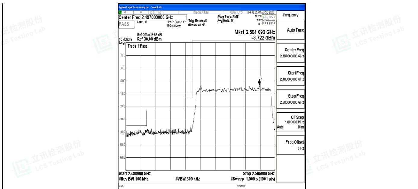
Band41_10MHz_16QAM_39700_50RB#0
