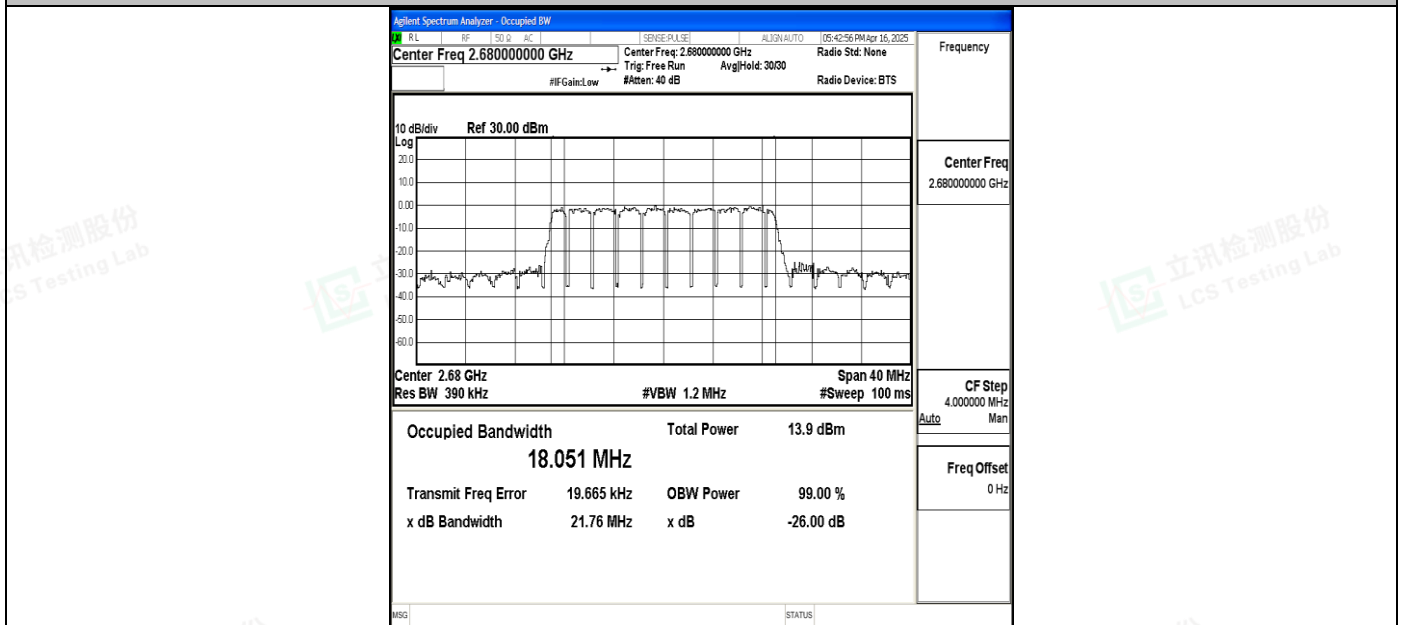
Band41-20MHz-16QAM-41490-100RB#0-PASS
