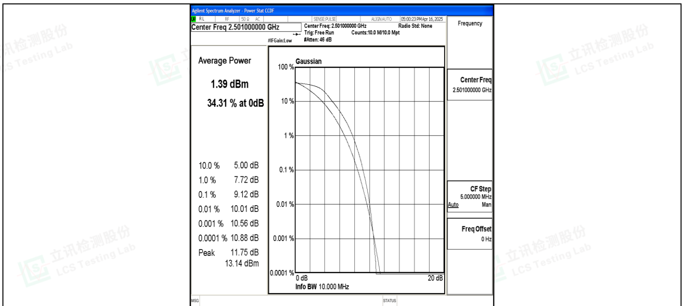
Band41-10MHz-QPSK-39700-50RB#0-PASS
