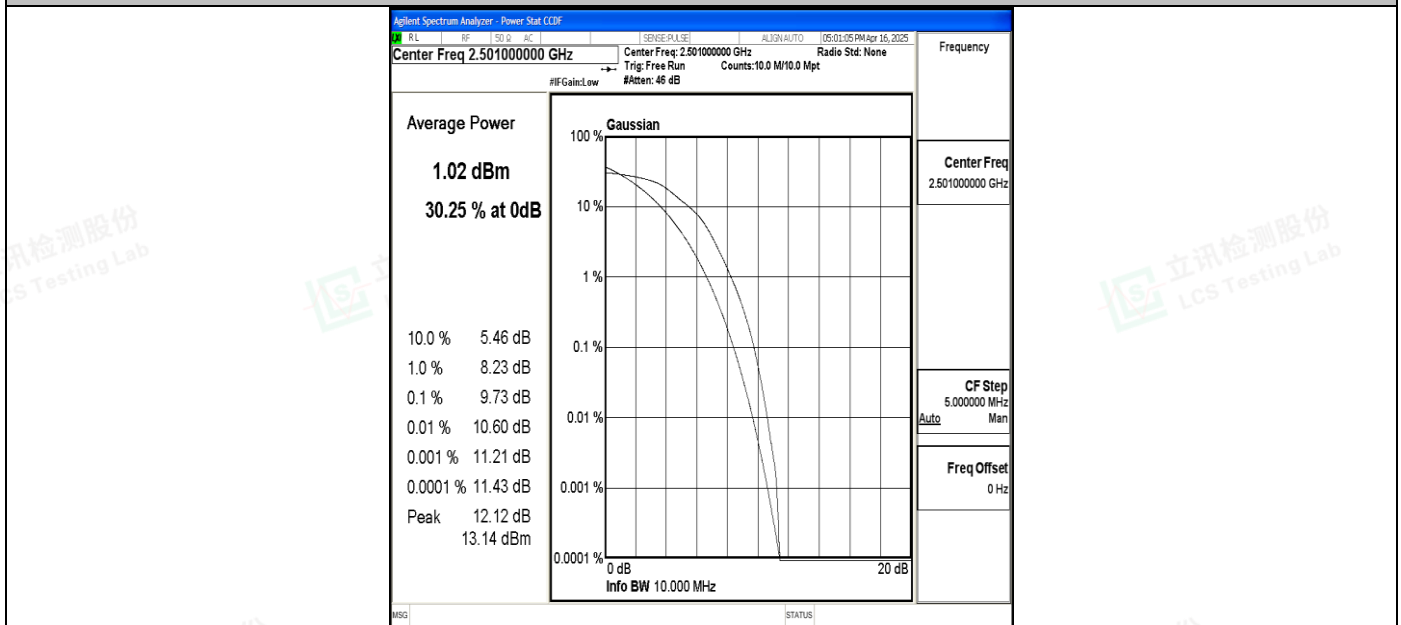
Band41-10MHz-16QAM-39700-50RB#0-PASS
