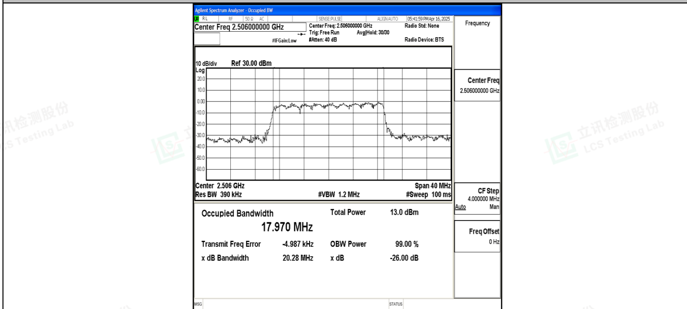
Band41-20MHz-16QAM-39750-100RB#0-PASS
