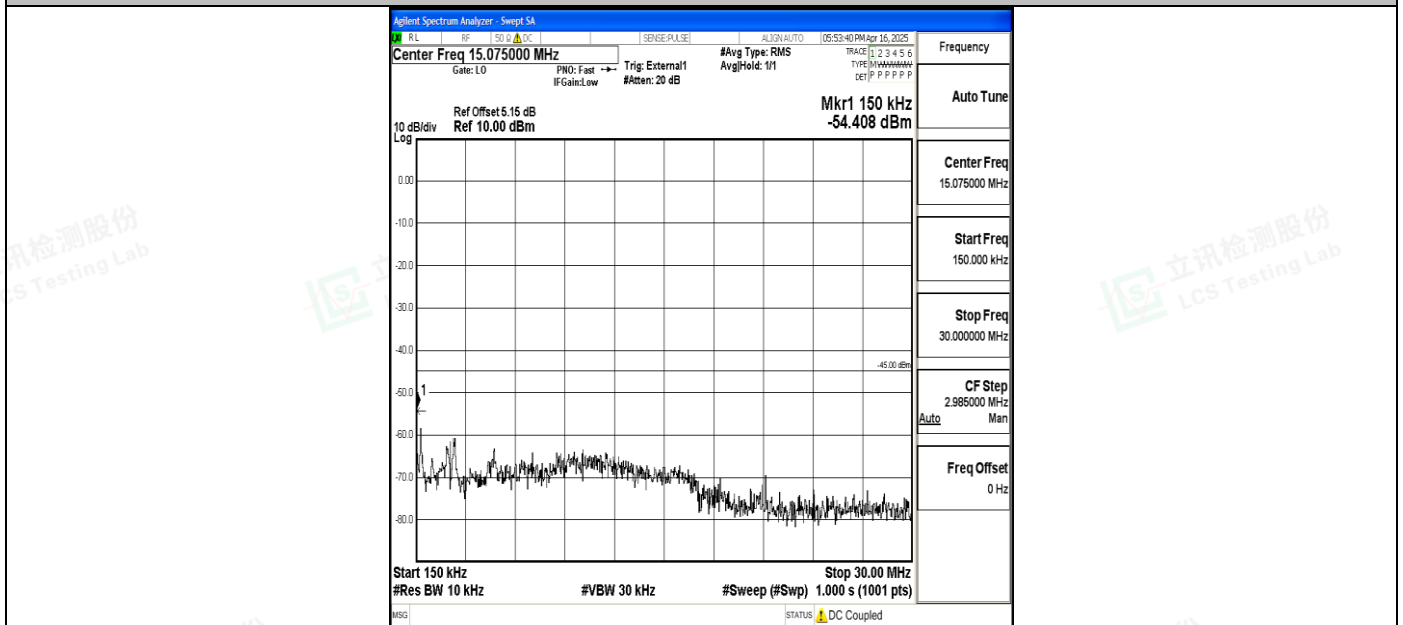
Band41_20MHz_QPSK_41490_1RB#0_0.15~30_0.15~30
