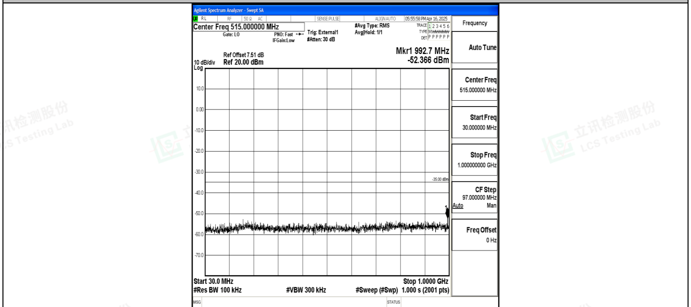
Band41_20MHz_16QAM_41490_1RB#0_30~1000_30~1000
