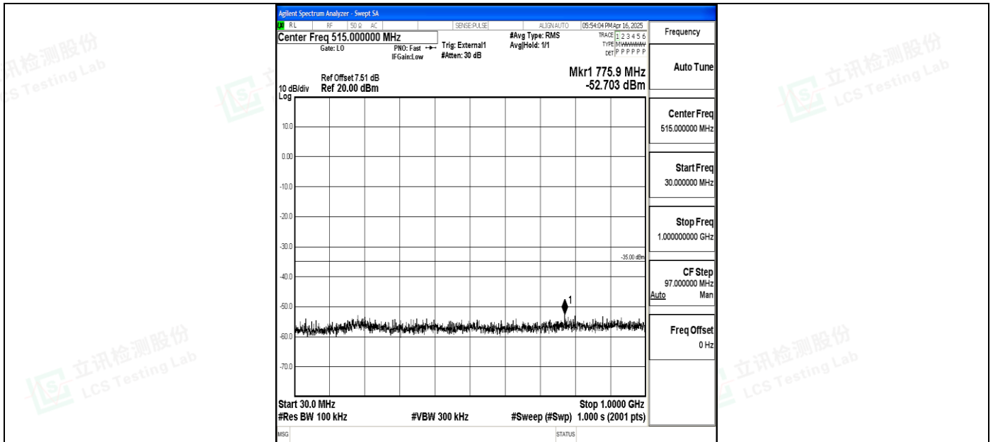
Band41_20MHz_QPSK_41490_1RB#0_30~1000_30~1000
