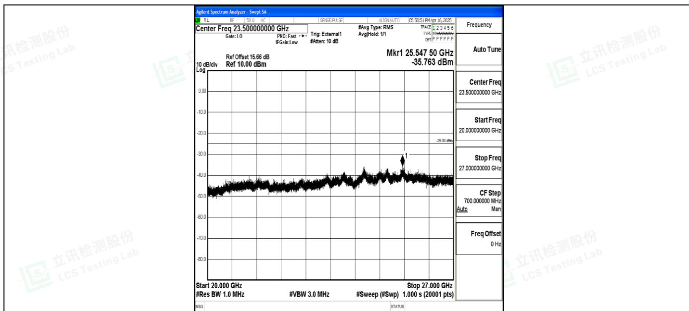
Band41_20MHz_QPSK_40620_1RB#0_20000~27000_20000~27000
