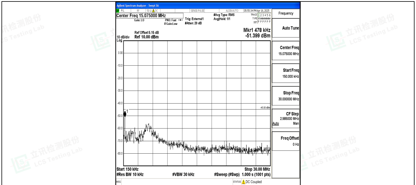
Band41_20MHz_16QAM_41490_1RB#0_0.15~30_0.15~30
