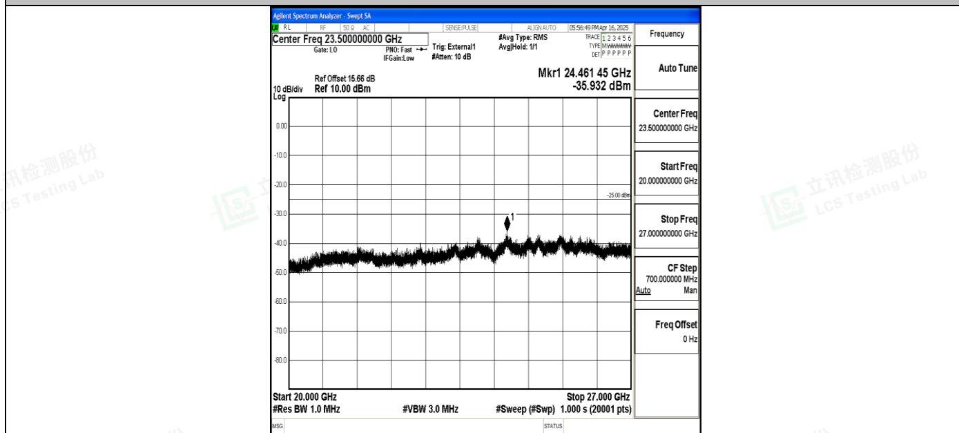
Band41_20MHz_16QAM_41490_1RB#0_20000~27000_20000~27000
