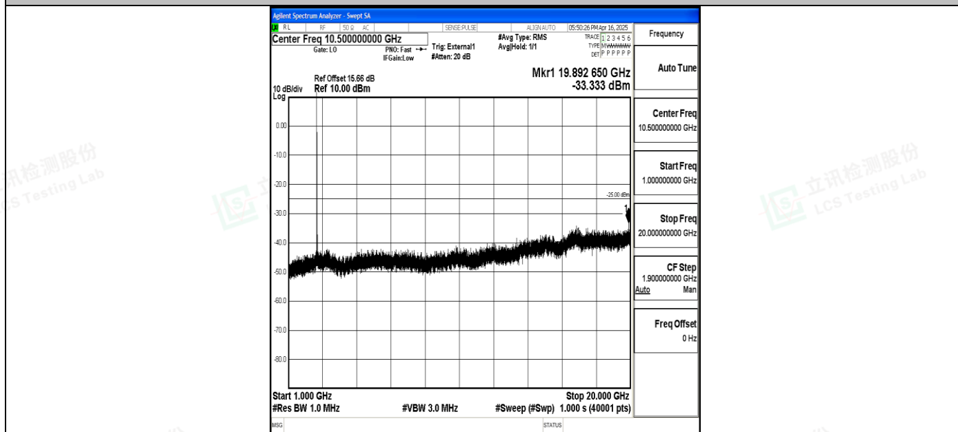
Band41_20MHz_QPSK_40620_1RB#0_1000~20000_1000~20000
