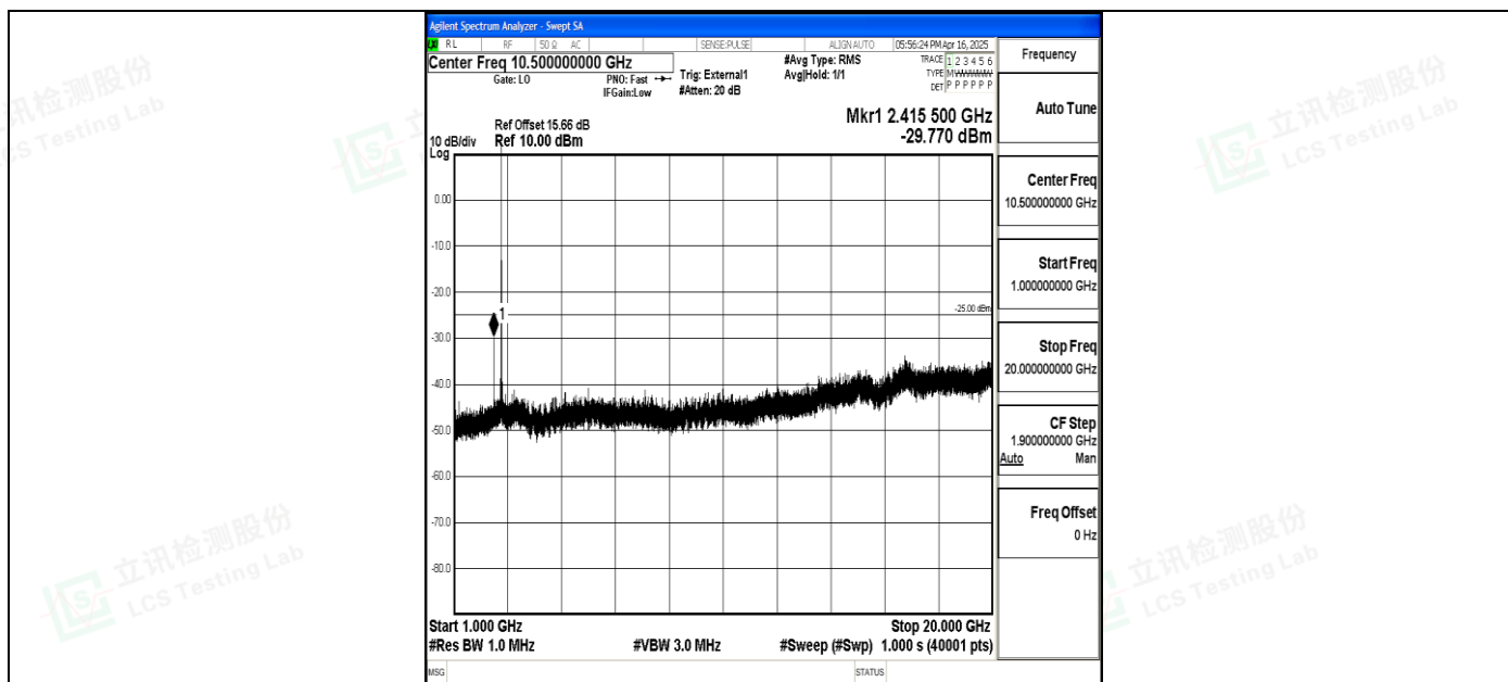
Band41_20MHz_16QAM_41490_1RB#0_1000~20000_1000~20000
