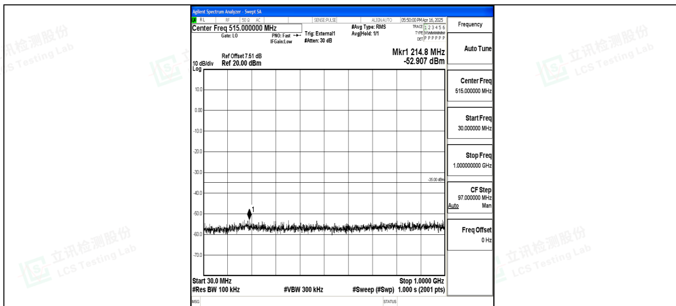
Band41_20MHz_QPSK_40620_1RB#0_30~1000_30~1000
