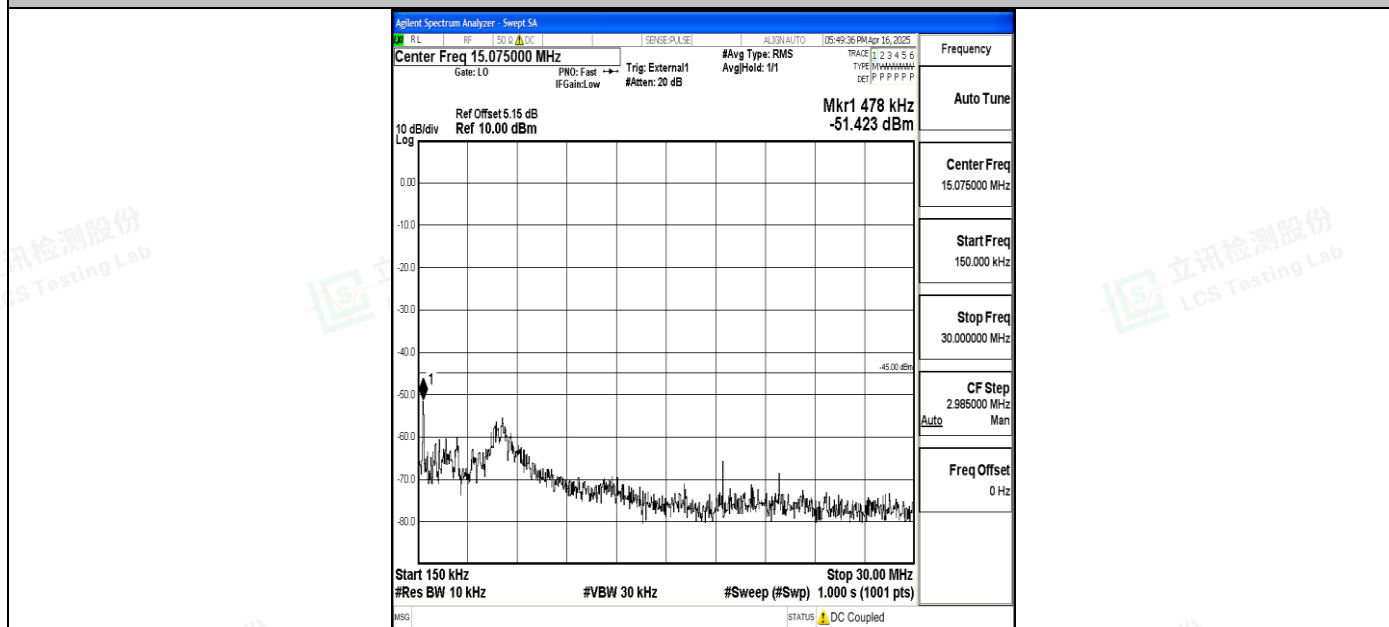
Band41_20MHz_QPSK_40620_1RB#0_0.15~30_0.15~30
