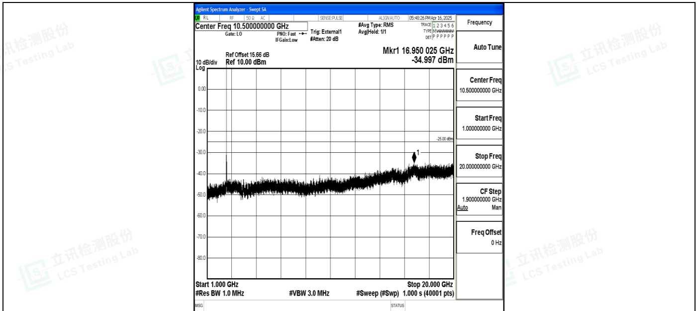
Band41_20MHz_16QAM_39750_1RB#0_1000~20000_1000~20000
