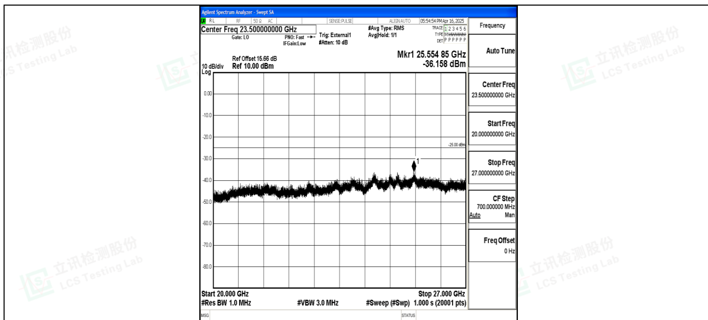
Band41_20MHz_QPSK_41490_1RB#0_20000~27000_20000~27000
