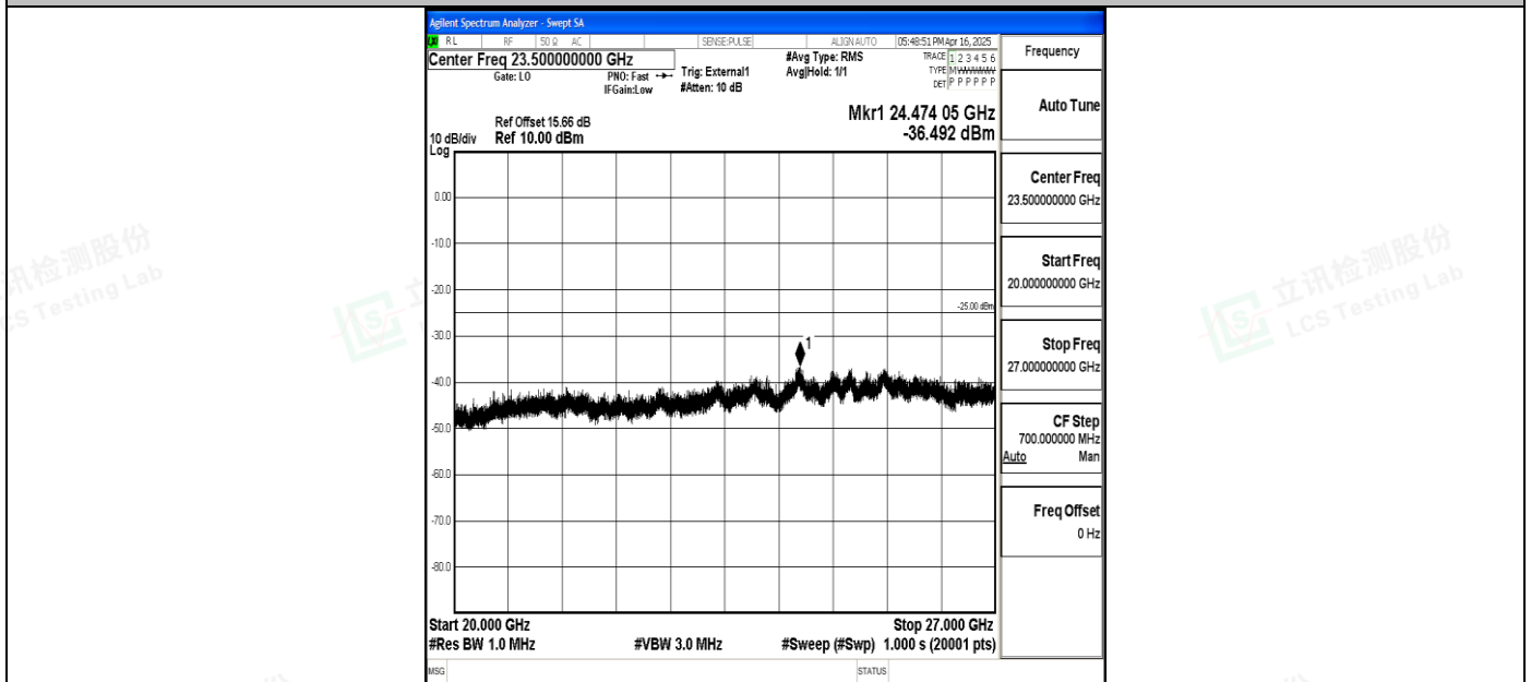
Band41_20MHz_16QAM_39750_1RB#0_20000~27000_20000~27000
