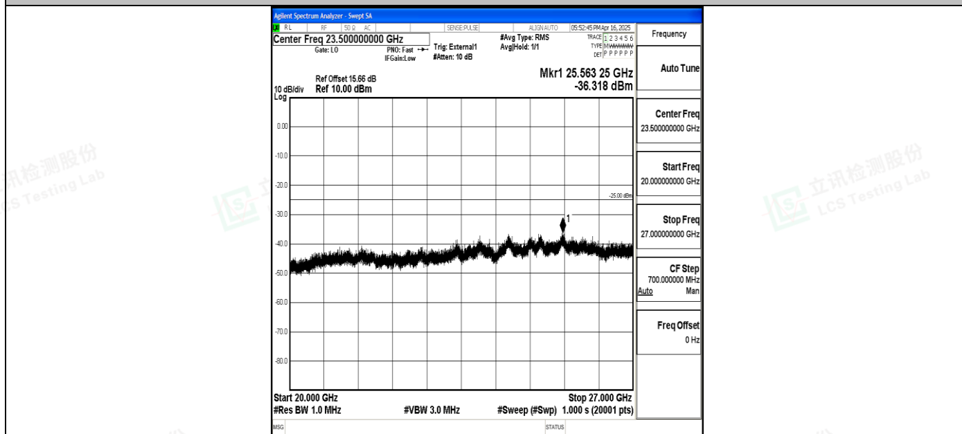
Band41_20MHz_16QAM_40620_1RB#0_20000~27000_20000~27000
