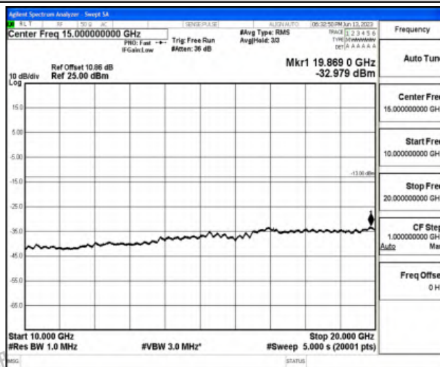
Band25-3MHz-16QAM-26365-1RB#0-Range5:10000~20000MHz
