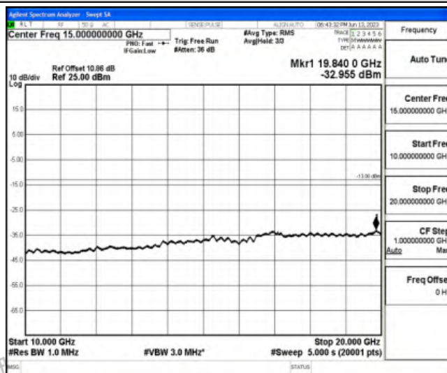
Band25-5MHz-16QAM-26365-1RB#0-Range5:10000~20000MHz
