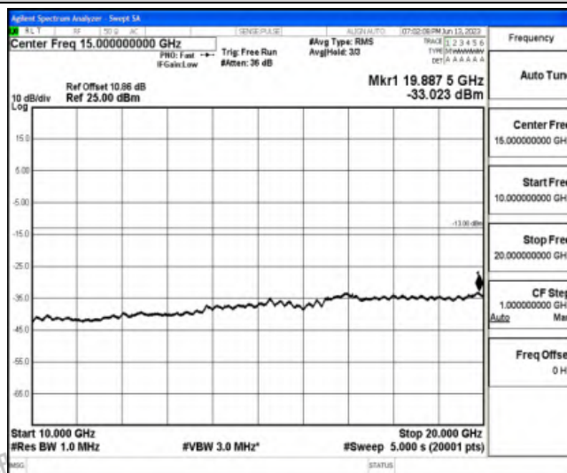
Band25-15MHz-QPSK-26365-1RB#0-Range5:10000~20000MHz
