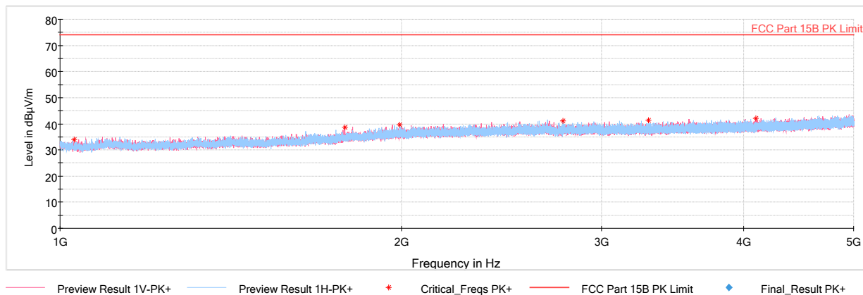
Plot 7-2. Radiated Spurious Plot Above 1GHz
