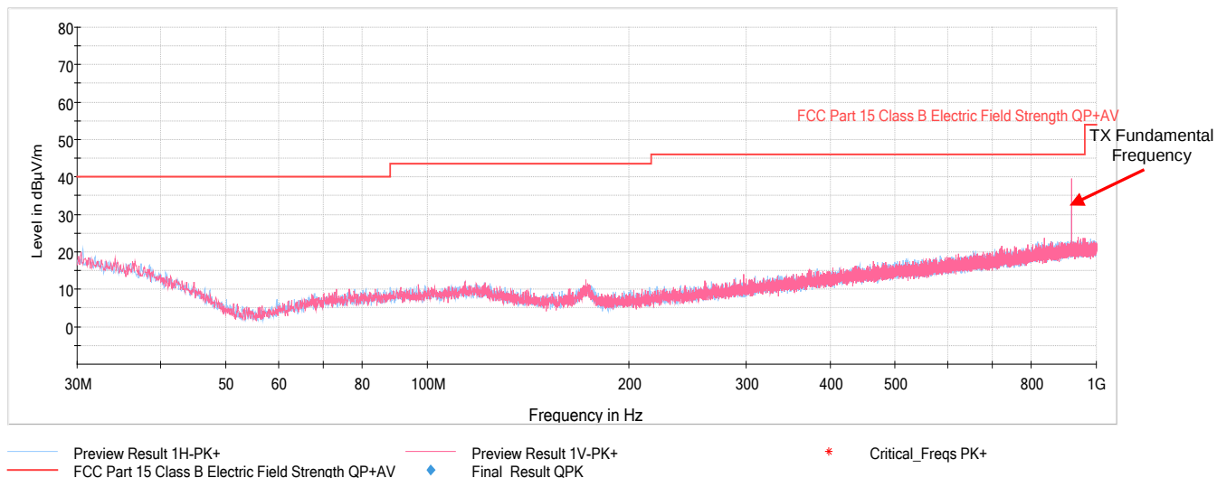
Plot 7-1. Radiated Spurious Plot Below 1GHz
