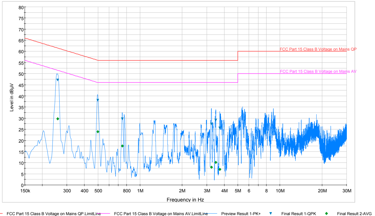
Plot 6-2. Line-Conducted Test Plot (L1)
