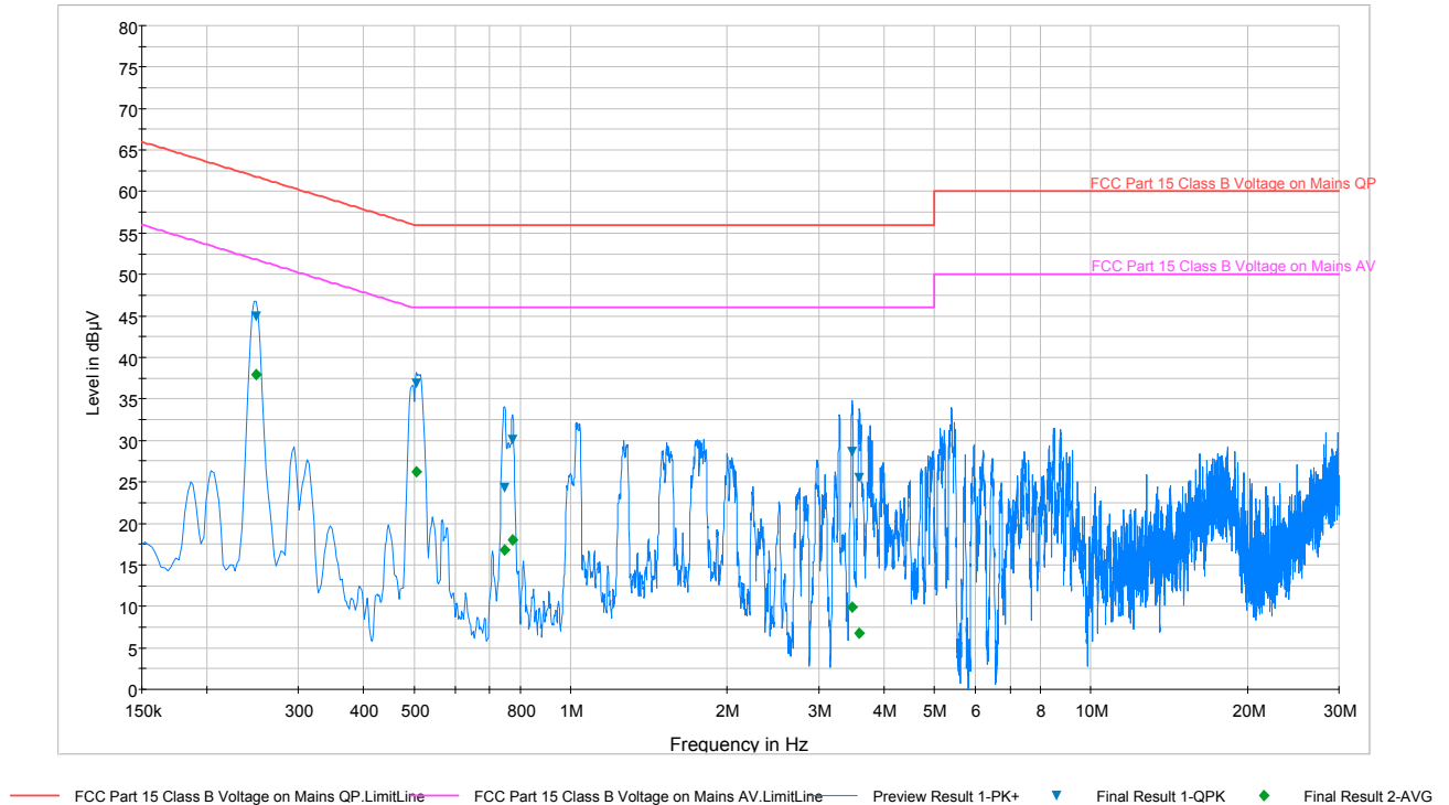
Plot 6-3. Line-Conducted Test Plot (N)
