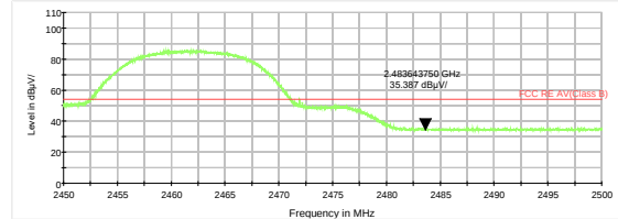
802.11b-Channel 11 Average
