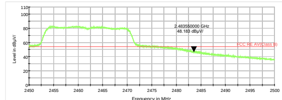
802.11g-Channel 11 Average
