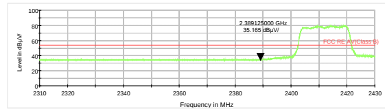
802.11g-Channel 1 Average
