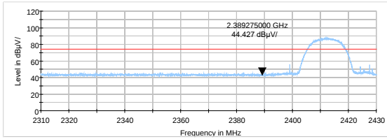
802.11b-Channel 1 Peak
