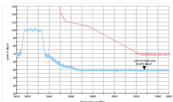
802.11a-Channel 165: Peak
