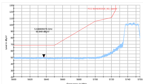
802.11a-Channel 149: Peak
