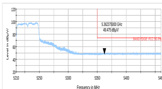
802.11n HT40-Channel 46: Average
