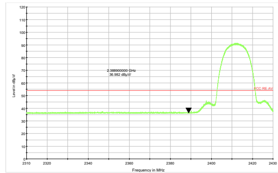
802.11b-Channel 1 Average
