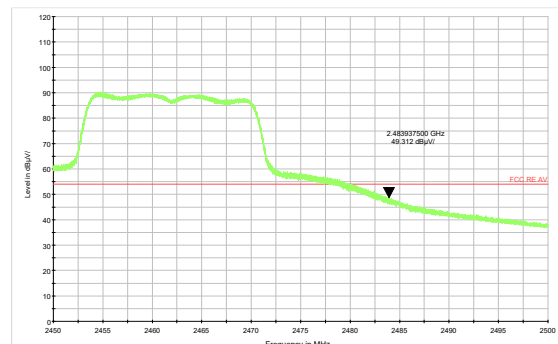
802.11g-Channel 11 Average
