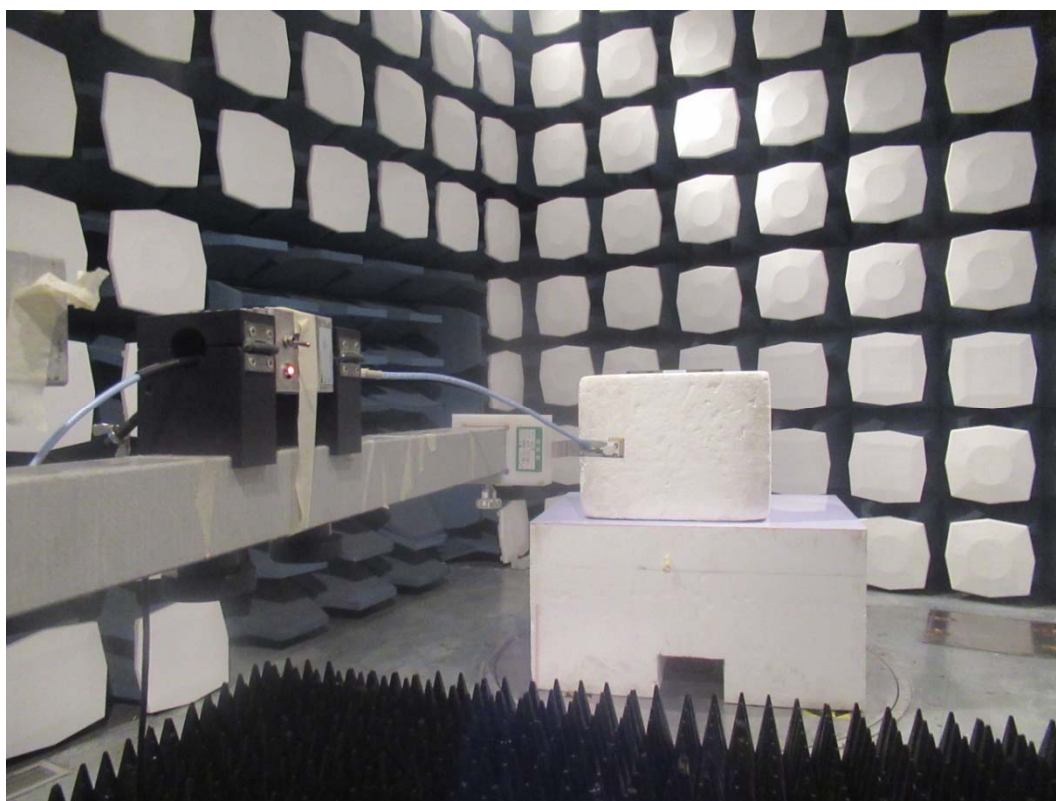
26GHz-40GHz
