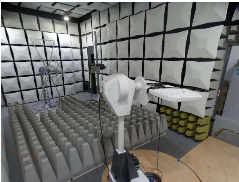
Photo 3: Test Antenna
