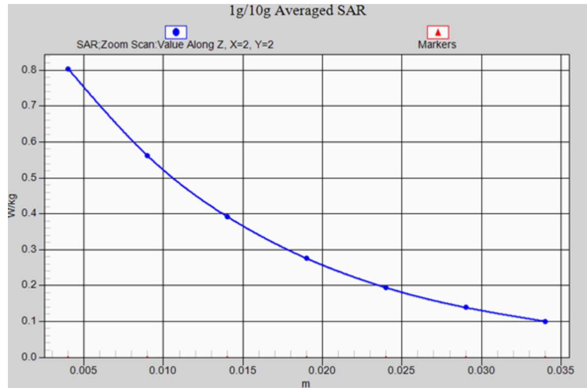
WCDMA Band V- LEFT/CHEEK-Mid- axis scan
