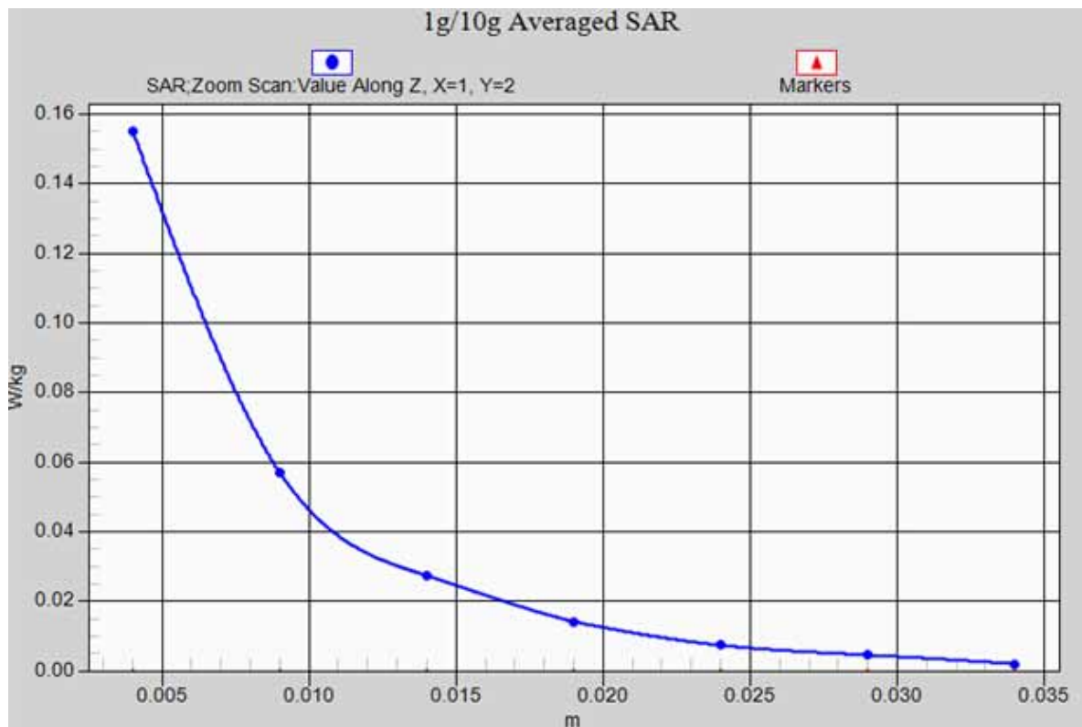
WiFi 802.11b(Body)/Back side High -axis scan
