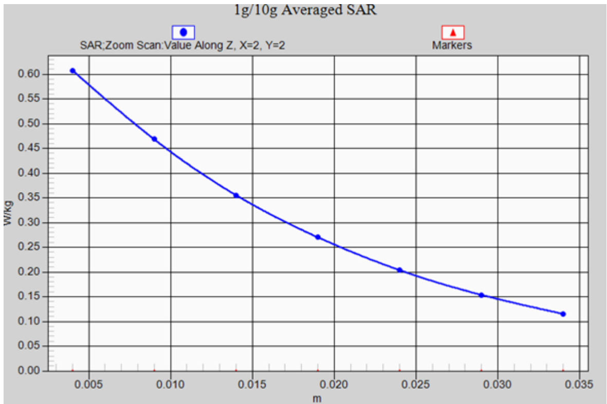
WCDMA Band V(Body)/Back side Low-axis scan
