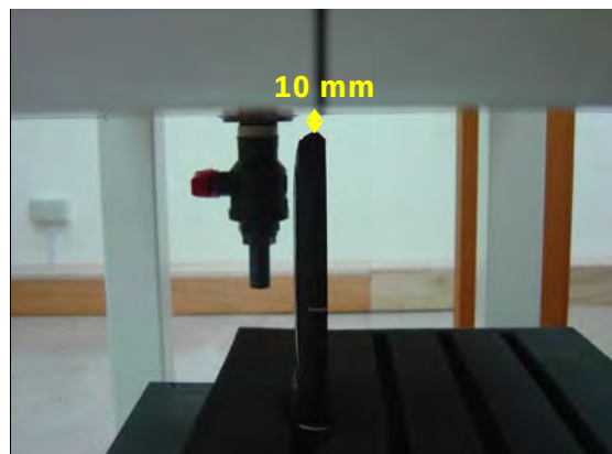
Fig.10 EUT bottom to flat phantom
