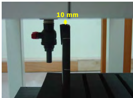
Fig.9 EUT top to flat phantom
