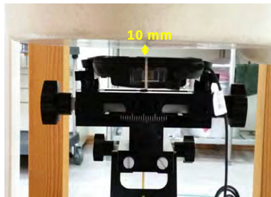
Fig.13 EUT front with headset to flat phantom
