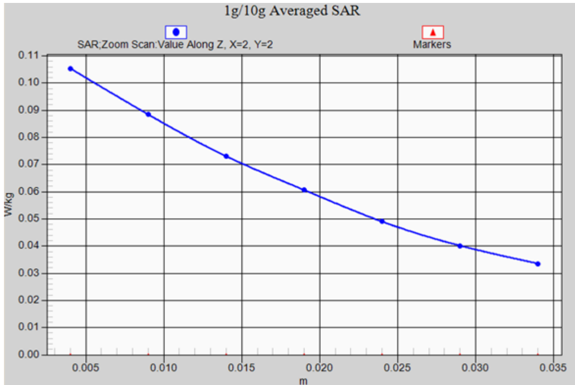
GSM850 LEFT/CHEEK-Low -axis scan
