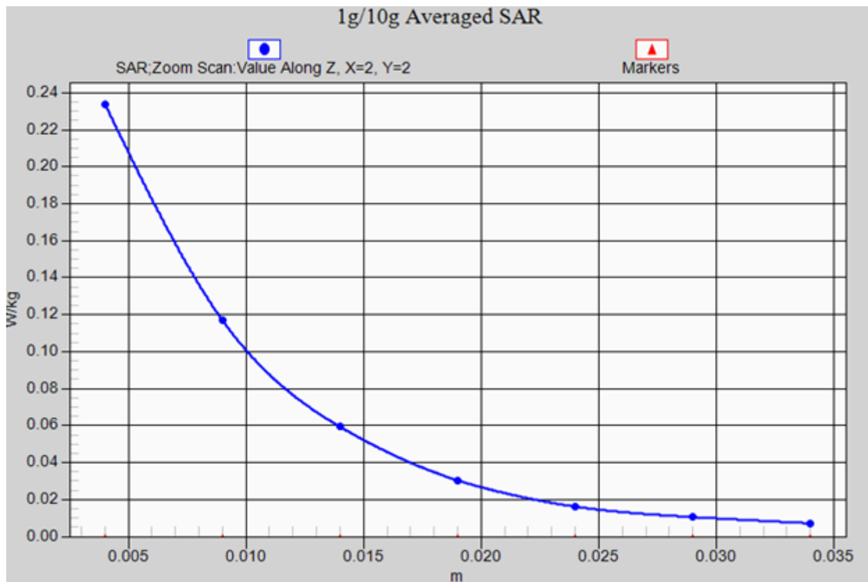
WiFi 802.11b LEFT/CHEEK-Low-axis scan
