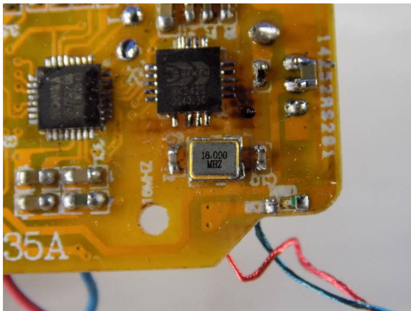
Oscillator view 1
