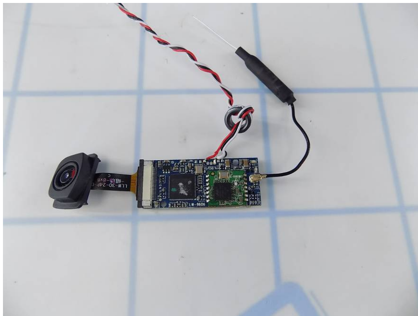
Antenna view
