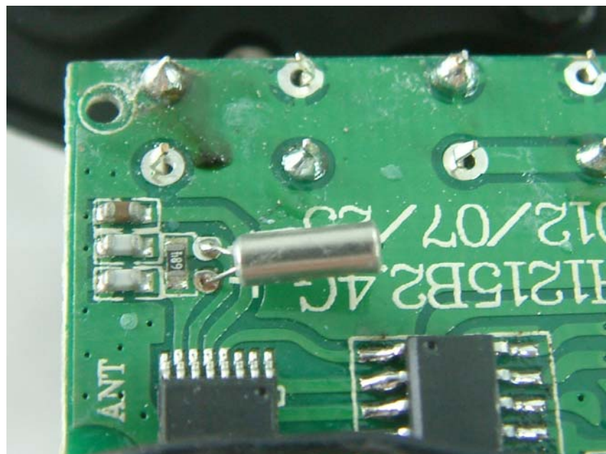
Oscillator view
