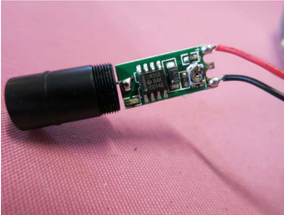
Red Laser Light PCB comp side
