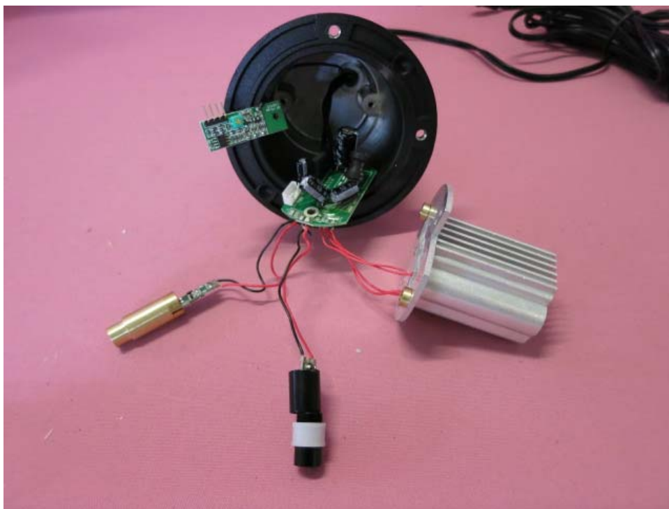
Receiver Unit assembly (4)
