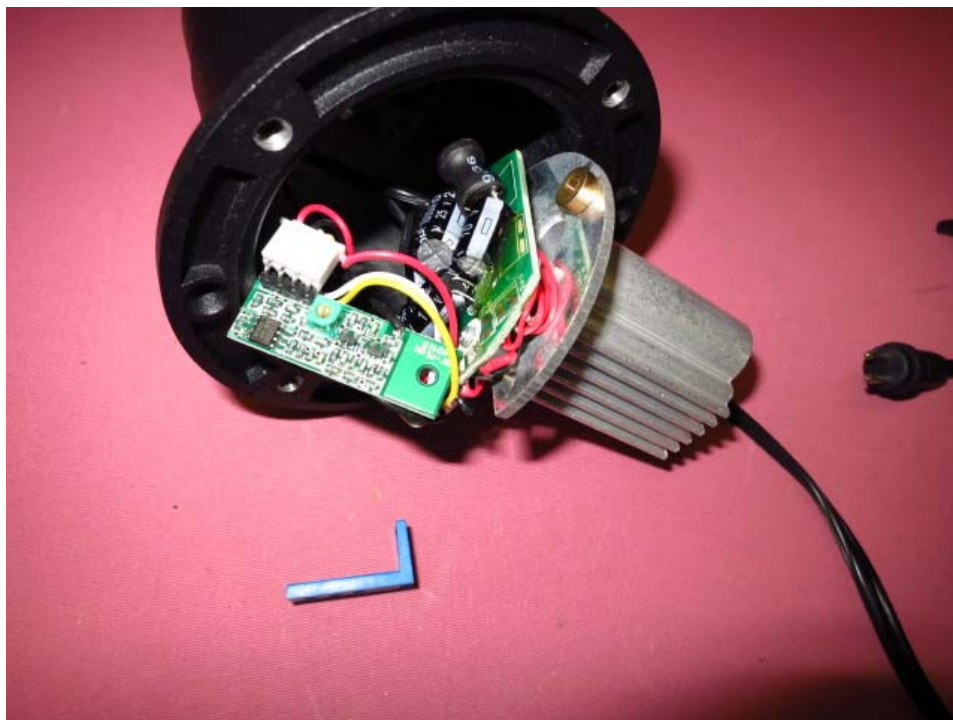
Receiver Unit assembly (3)
