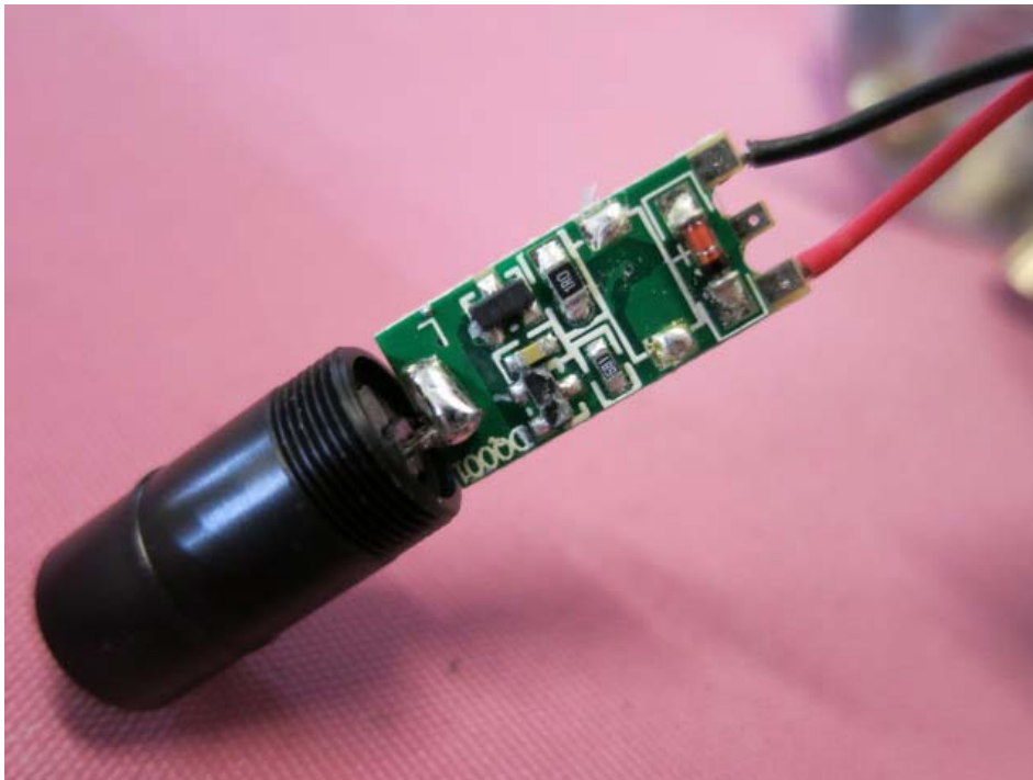
Red Laser Light PCB solder side
