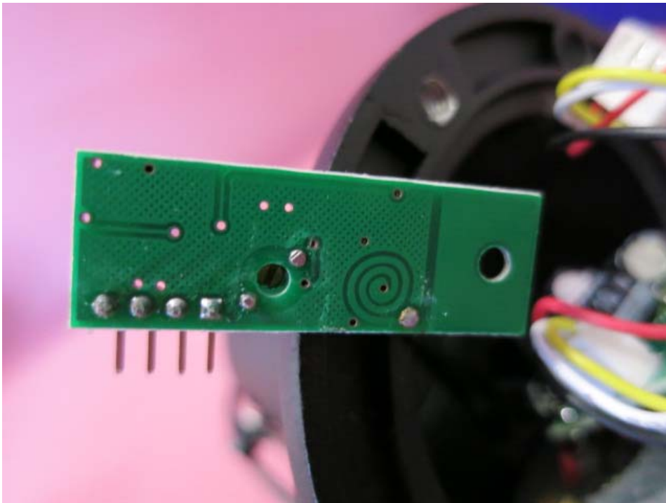
Receiver Unit Oscillator solder side
