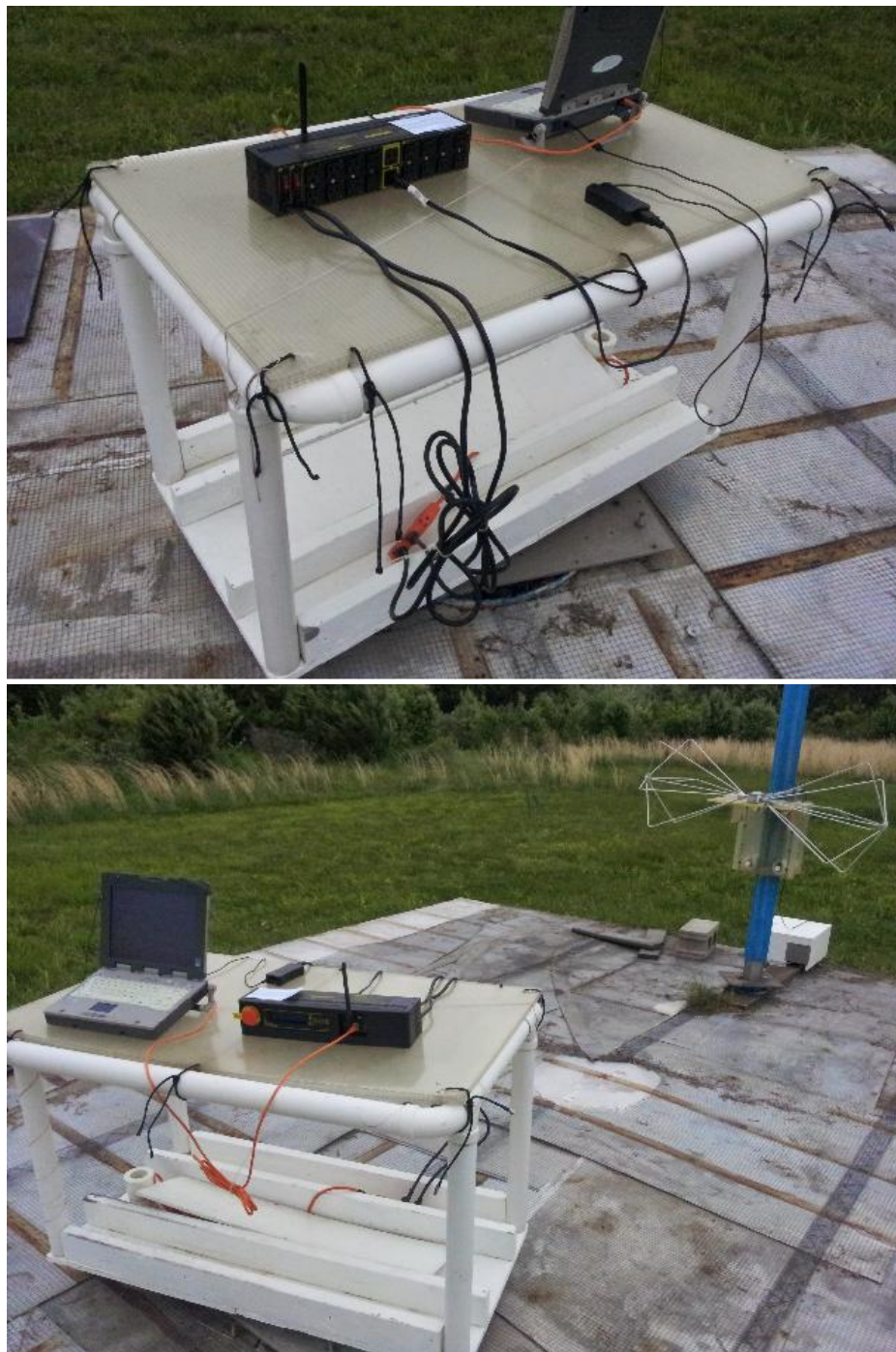
Figure 4: Radiated Emissions Test Setup Photograph(s).
