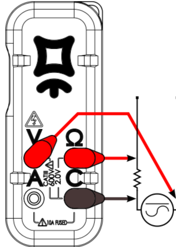
FIGURE 8 POWER FACTOR WITH EXTERNAL CURRENT SHUNT
