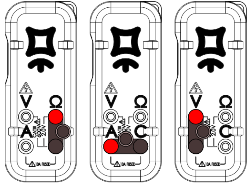
FIGURE 6 BNC ADAPTORS FOR \Omega , V, A INPUTS
