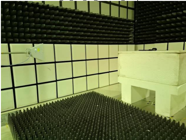
FCC_15_247_BT_Radiated_Setup
