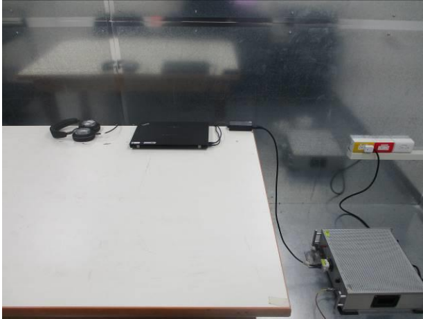
FCC_15_247_QHS_Conduction_Setup
