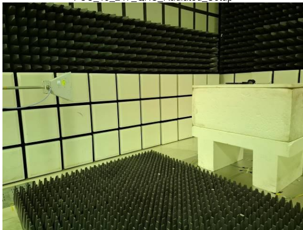
FCC_15_247_QHS_Radiated_Setup
