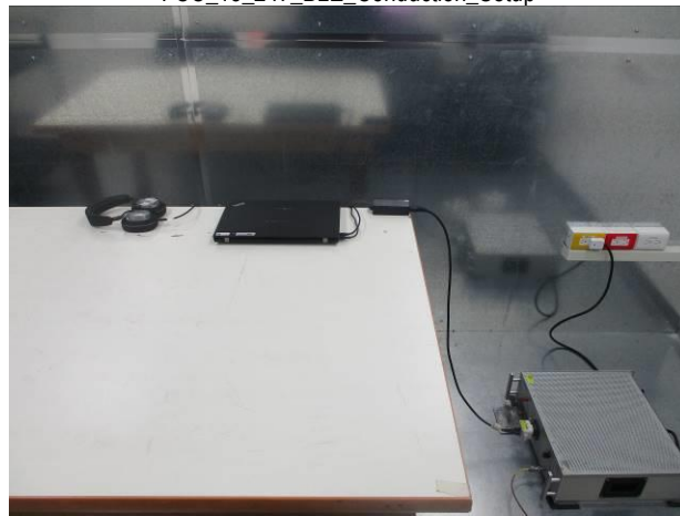
FCC_15_247_BLE_Conduction_Setup
