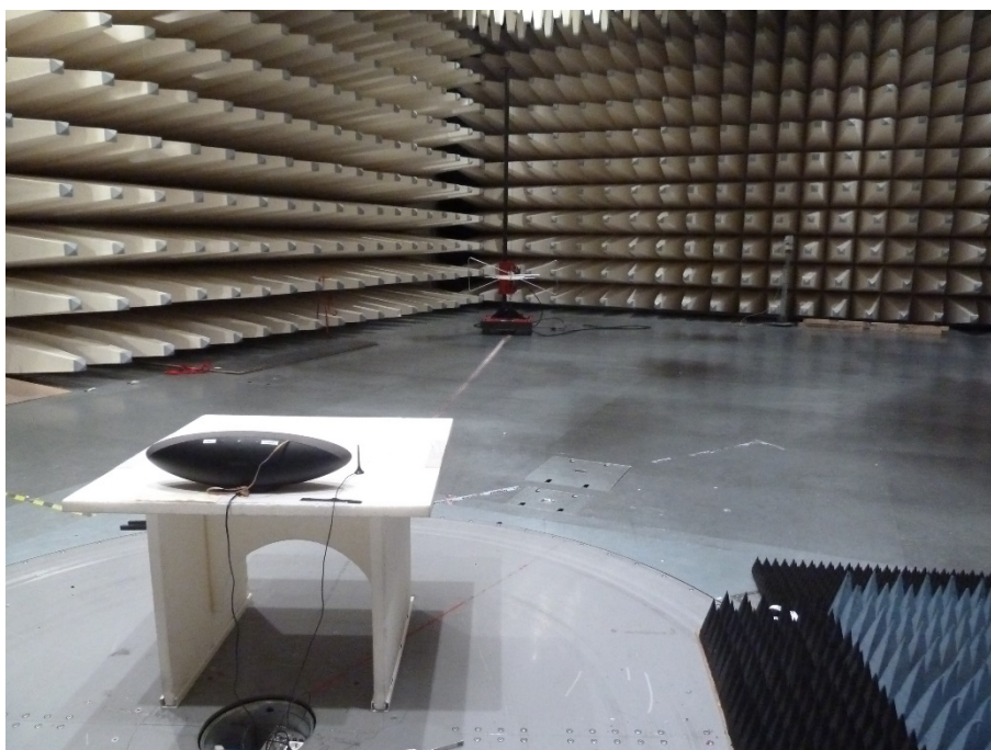
Photo 6: EUT at the semi anechoic chamber
