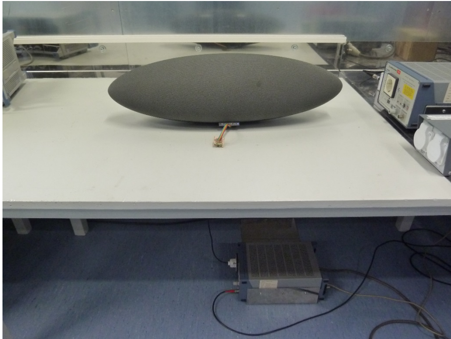
Photo 7: AC conducted emission measurement
