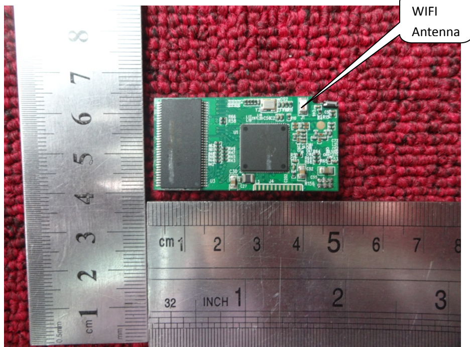
Internal photograph of EUT
