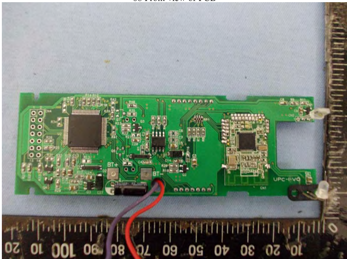
08 Front view of PCB
