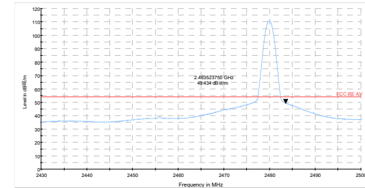
Bluetooth LE (1M) Channel 39 Peak+Average
