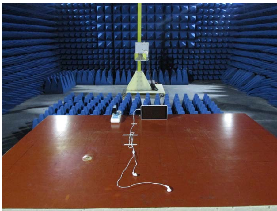
RADIATED EMISSION TEST ABOVE 1GHz (Mode 1, Mode 2, Mode 3)
