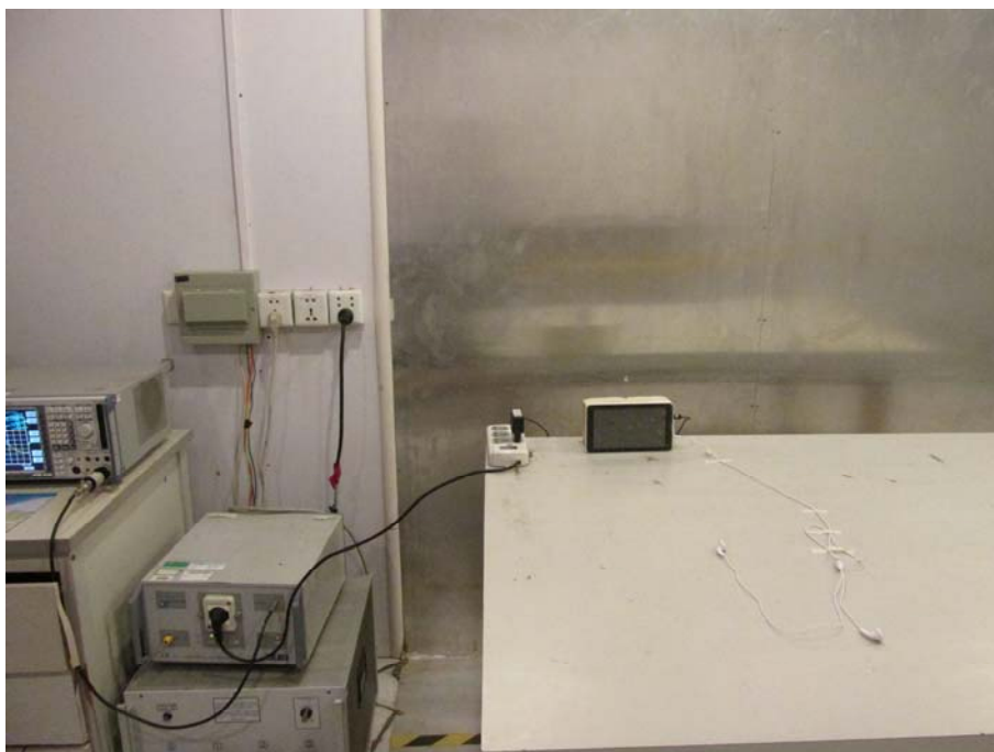
Conducted emission test (Mode 1, Mode 2, Mode 3)
