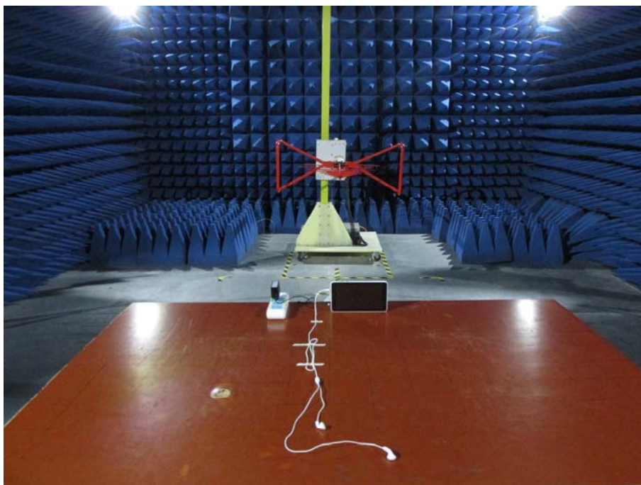
RADIATED EMISSION TEST BELOW 1GHz (Mode 1, Mode 2, Mode 3)
