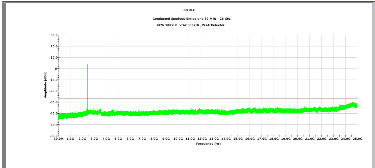
Plot 4.40 Ant 1, Tx @ 2412MHz 802.11n 40MHz
