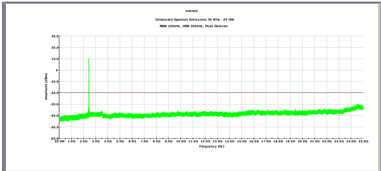
Plot 4.27 Ant 0, Tx @ 2462MHz 802.11n 20MHz
