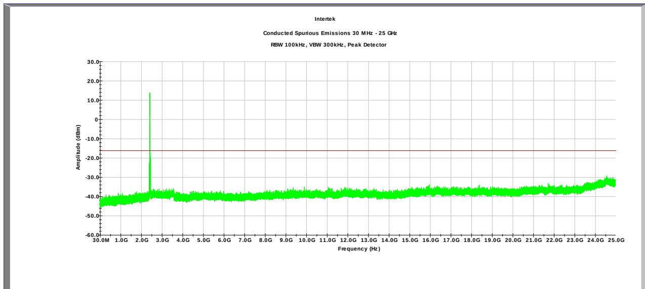
Plot 4.26 Ant 0, Tx @ 2437MHz 802.11n 20MHz
