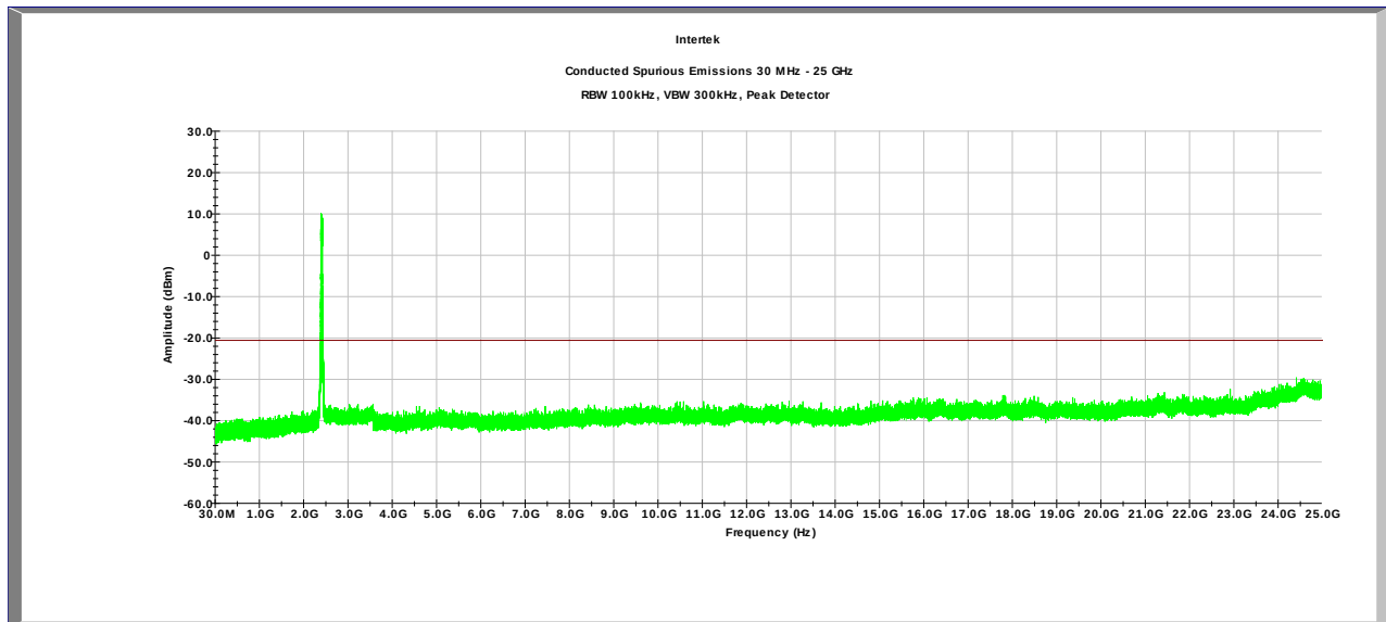
Plot 4.41 Ant 1, Tx @ 2437MHz 802.11n 40MHz
