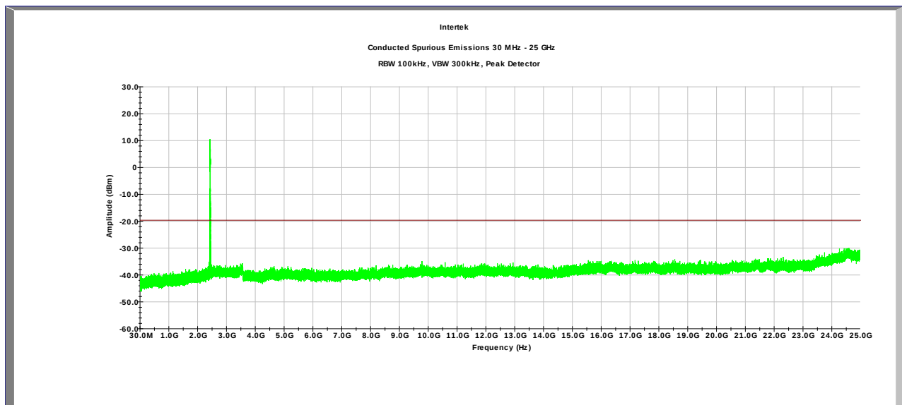
Plot 4.28 Ant 1, Tx @ 2412MHz 802.11n 20MHz
