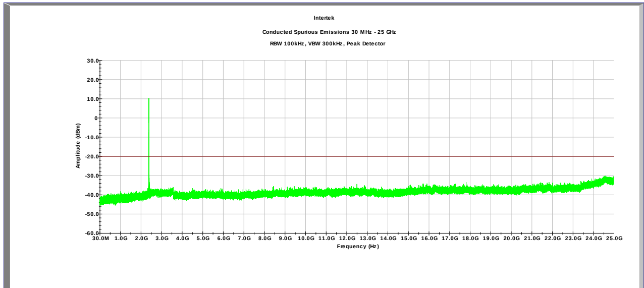
Plot 4.34 Ant 3, Tx @ 2412MHz 802.11n 20MHz
