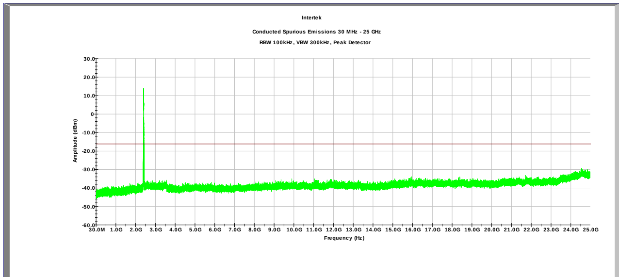
Plot 4.32 Ant 2, Tx @ 2437MHz 802.11n 20MHz
