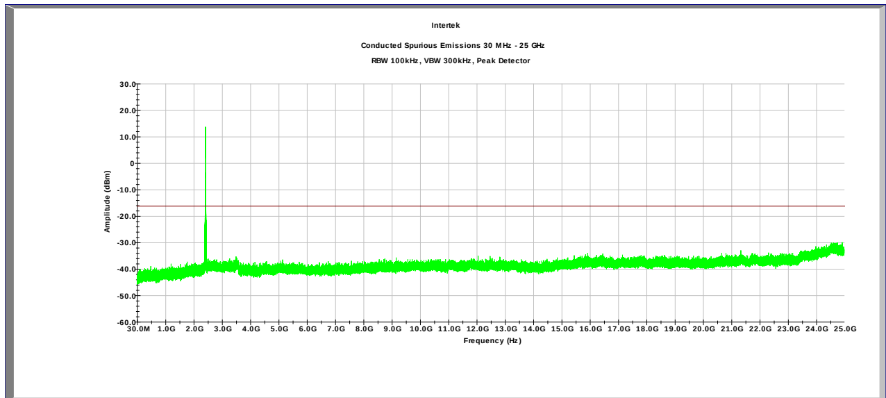
Plot 4.29 Ant 1, Tx @ 2437MHz 802.11n 20MHz
