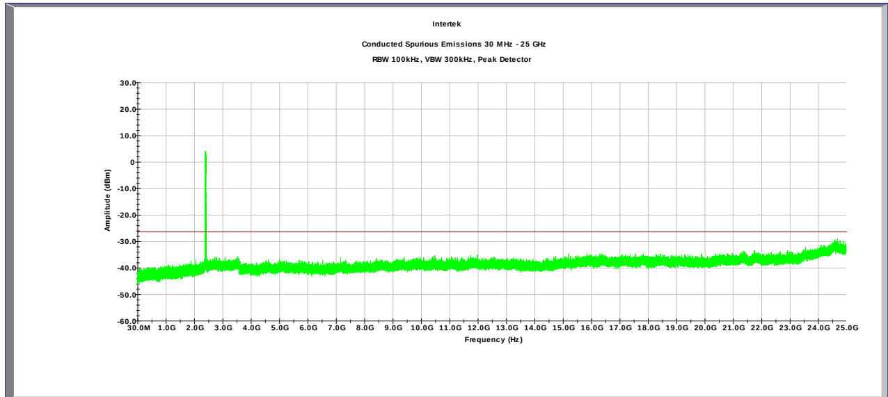
Plot 4.37 Ant 0, Tx @ 2412MHz 802.11n 40MHz
