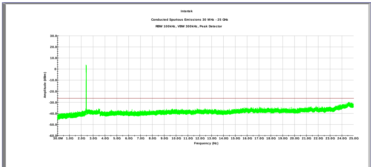
Plot 4.42 Ant 1, Tx @ 2462MHz 802.11n 40MHz
