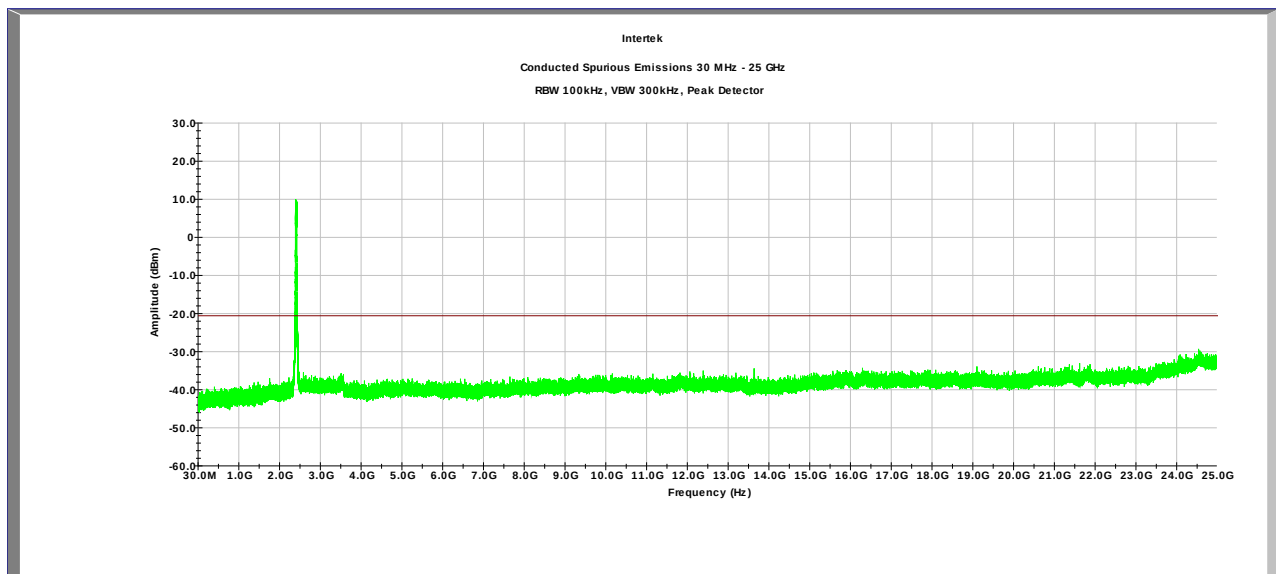
Plot 4.38 Ant 0, Tx @ 2437MHz 802.11n 40MHz
