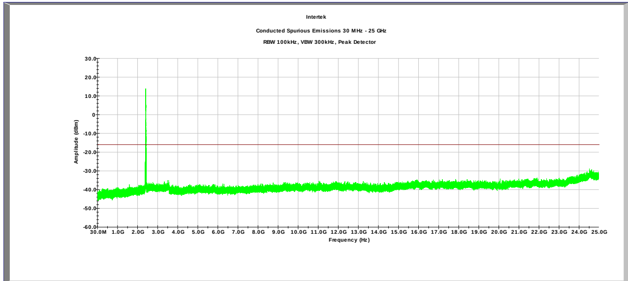
Plot 4.36 Ant 3, Tx @ 2462MHz 802.11n 20MHz
