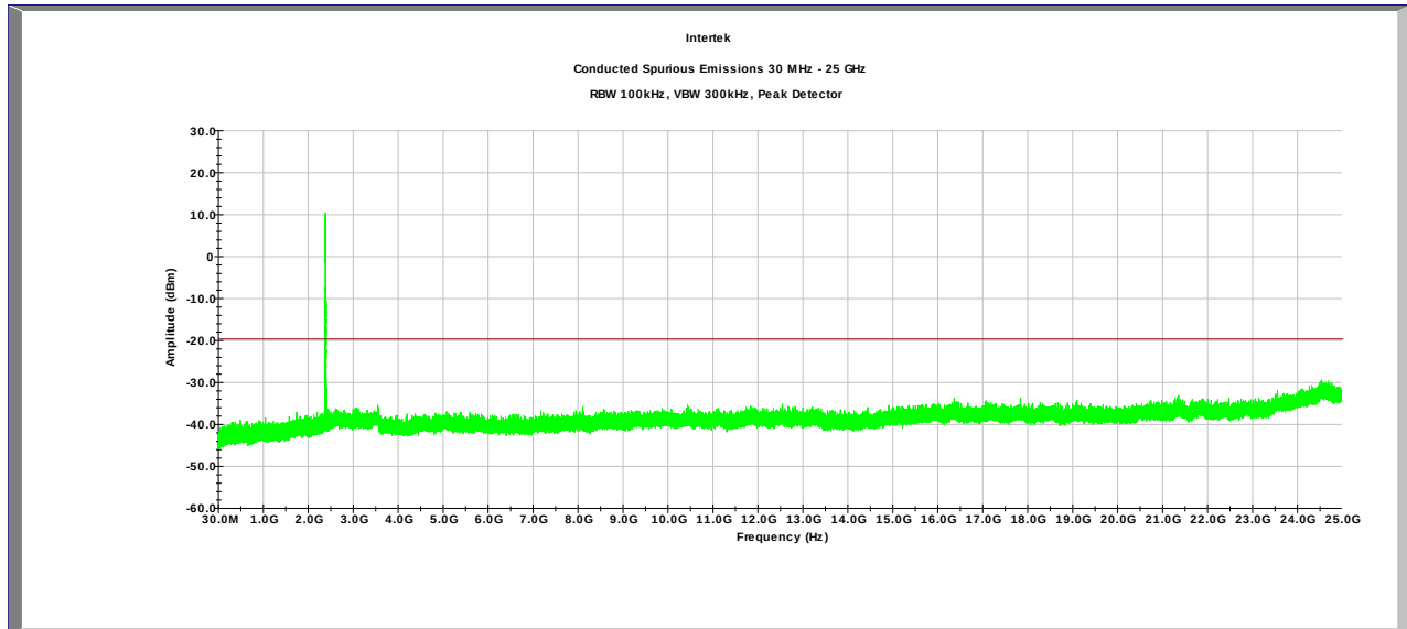
Plot 4.31 Ant 2, Tx @ 2412MHz 802.11n 20MHz
