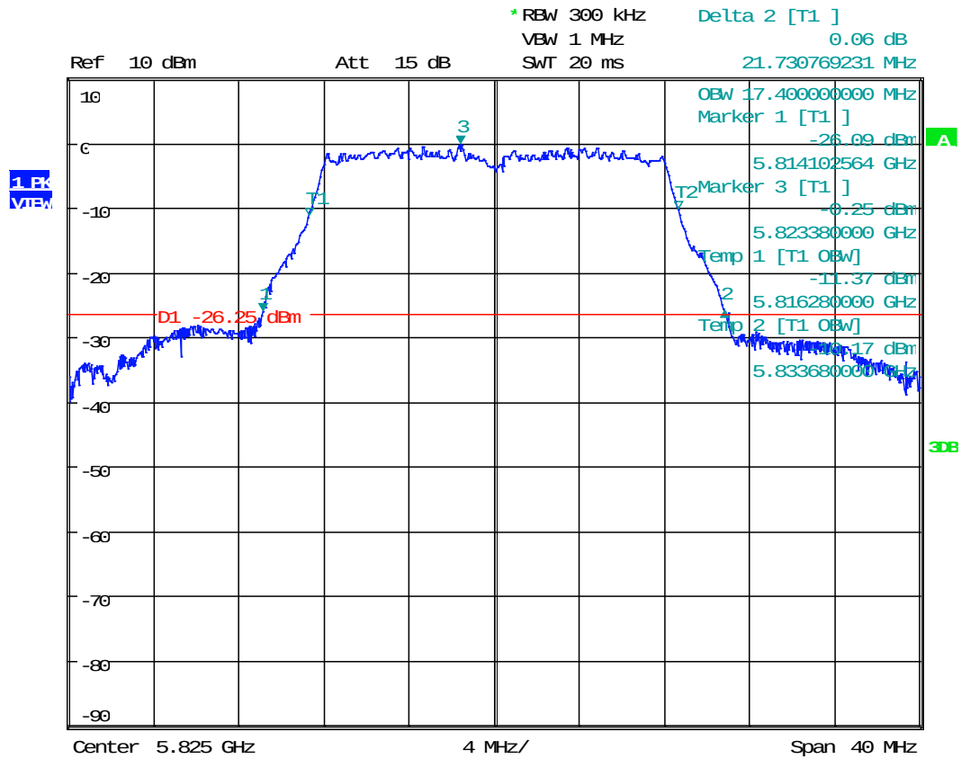
Plot 1.3 802.11a, 5825MHz
