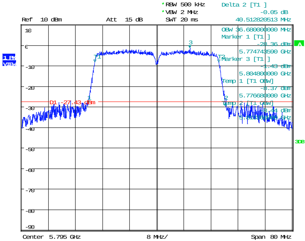
Plot 1. 8 802.11n 40MHz, 5795MHz
