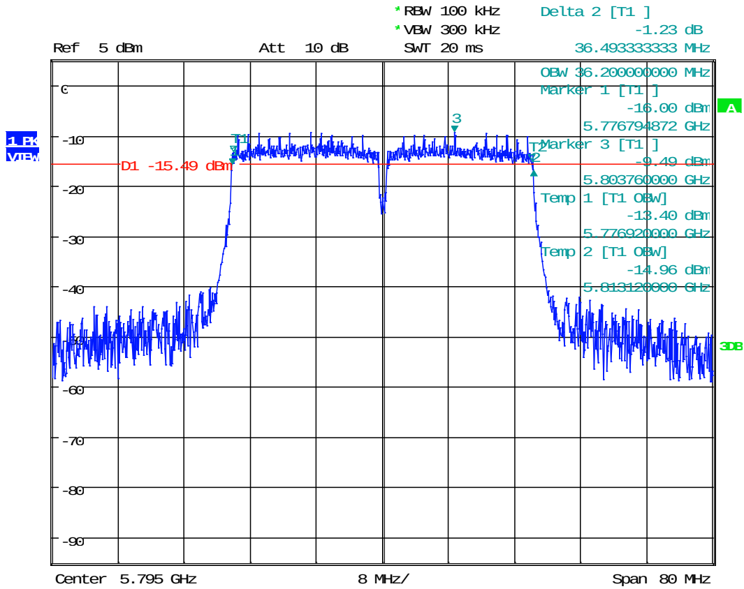
Plot 1. 17 802.11n 40MHz, 5795MHz
